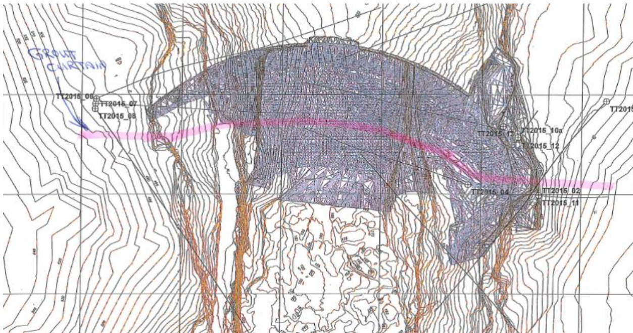
Exhibit 3E-1: Grout curtain drilling through dam from downstream dam face, plan view
