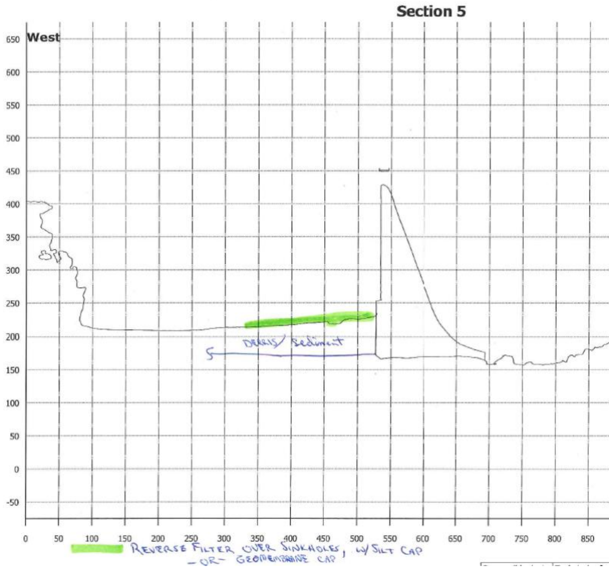
Exhibit Alt 1A-4: Blanket over forebay depressions, section perpendicular to dam
