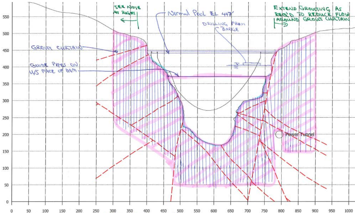
Exhibit Alt 3D-3: Grout curtain drilling from barge through upstream dam face, cross section (grout holes shown vertical—grout holes may be inclined and grout holes in adjacent grout curtain lines drilled at different orientations)
