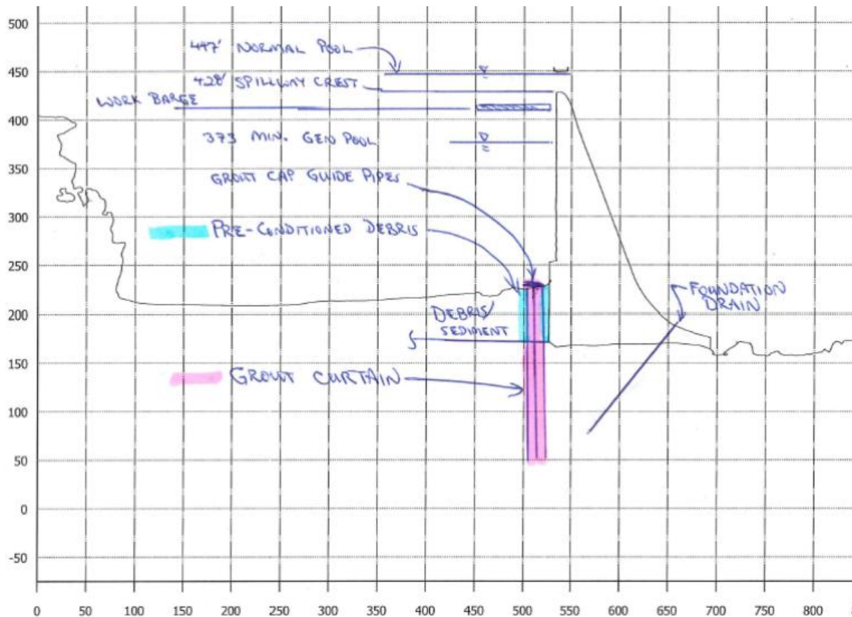
Exhibit Alt 3F-2: Grout curtain upstream of dam, drilling from barge upstream of dam, section perpendicular to dam
