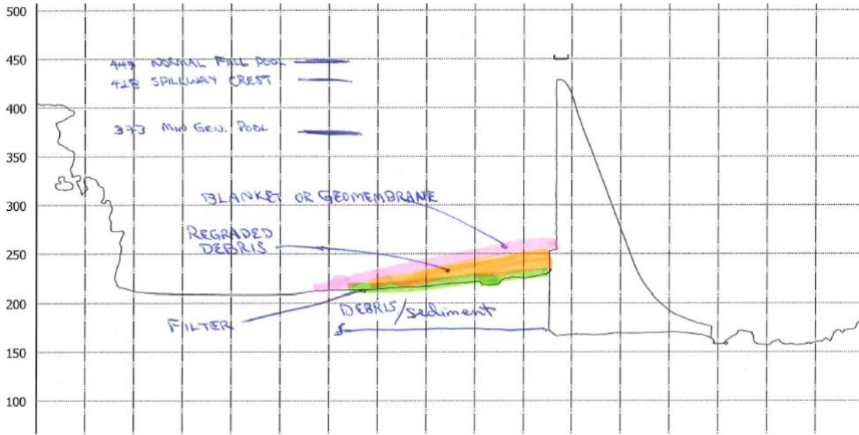
Exhibit A-Alt 1B-3: Filter over depressions and sinkholes, debris regrading, and blanket; section perpendicular to dam
