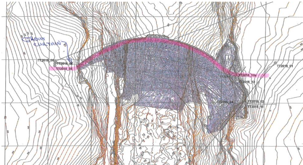
Exhibit Alt 3A-1: Grout curtain drilling through dam crest, plan view
