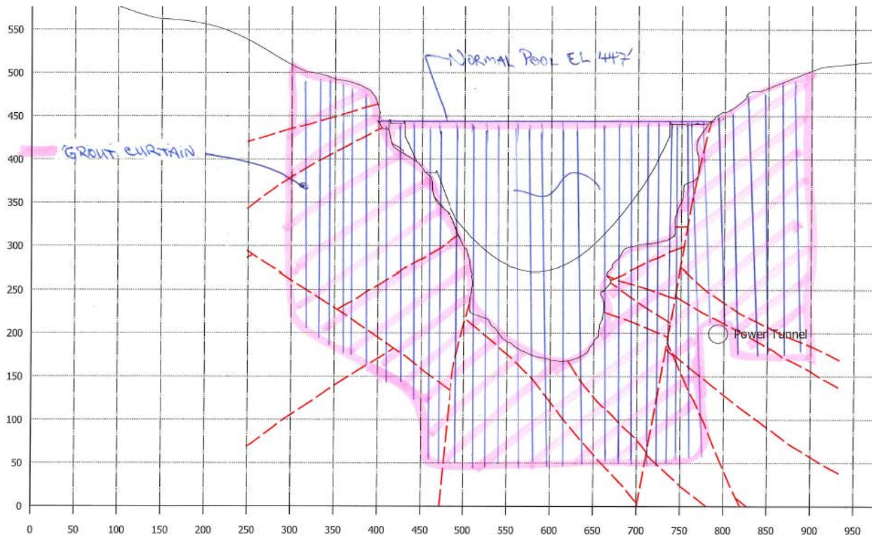
Exhibit Alt 3A-3: Grout curtain drilling through dam crest, cross section (grout holes shown vertical—grout holes may be inclined and grout holes in adjacent grout curtain lines drilled at different orientations)
