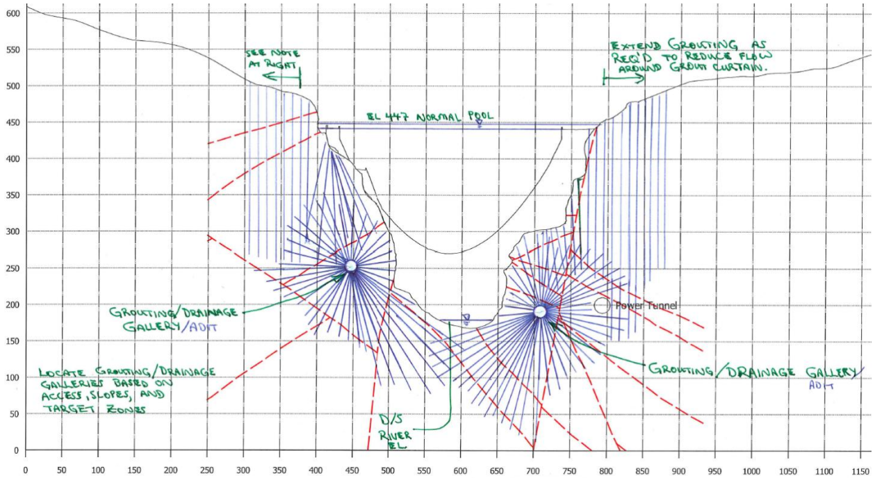
Exhibit A-Alt 3B-1: Grout curtain – drilling from adits; cross section (vertical and horizontal grout holes shown for convenience—grout hole orientations would vary and would be different on adjacent grout lines)
