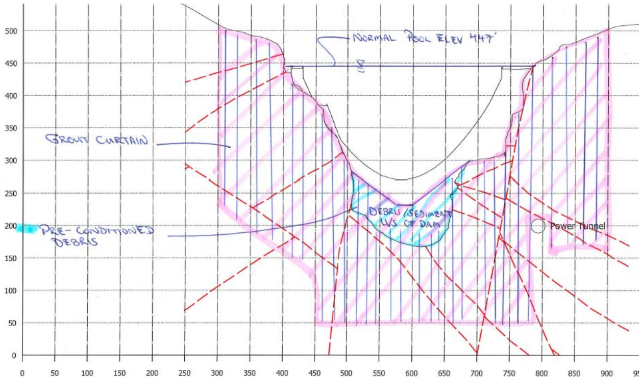
Exhibit Alt 3F-3: Grout curtain upstream of dam, drilling from barge upstream of dam, cross section (grout holes shown vertical—grout holes may be inclined and grout holes in adjacent grout curtain lines drilled at different orientations)
