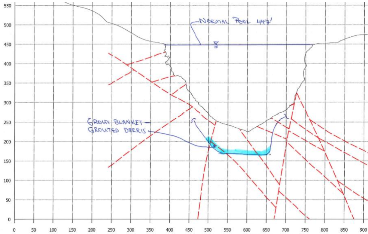
Exhibit Alt 4-4: Grout blanket in debris upstream of LBD, cross section
