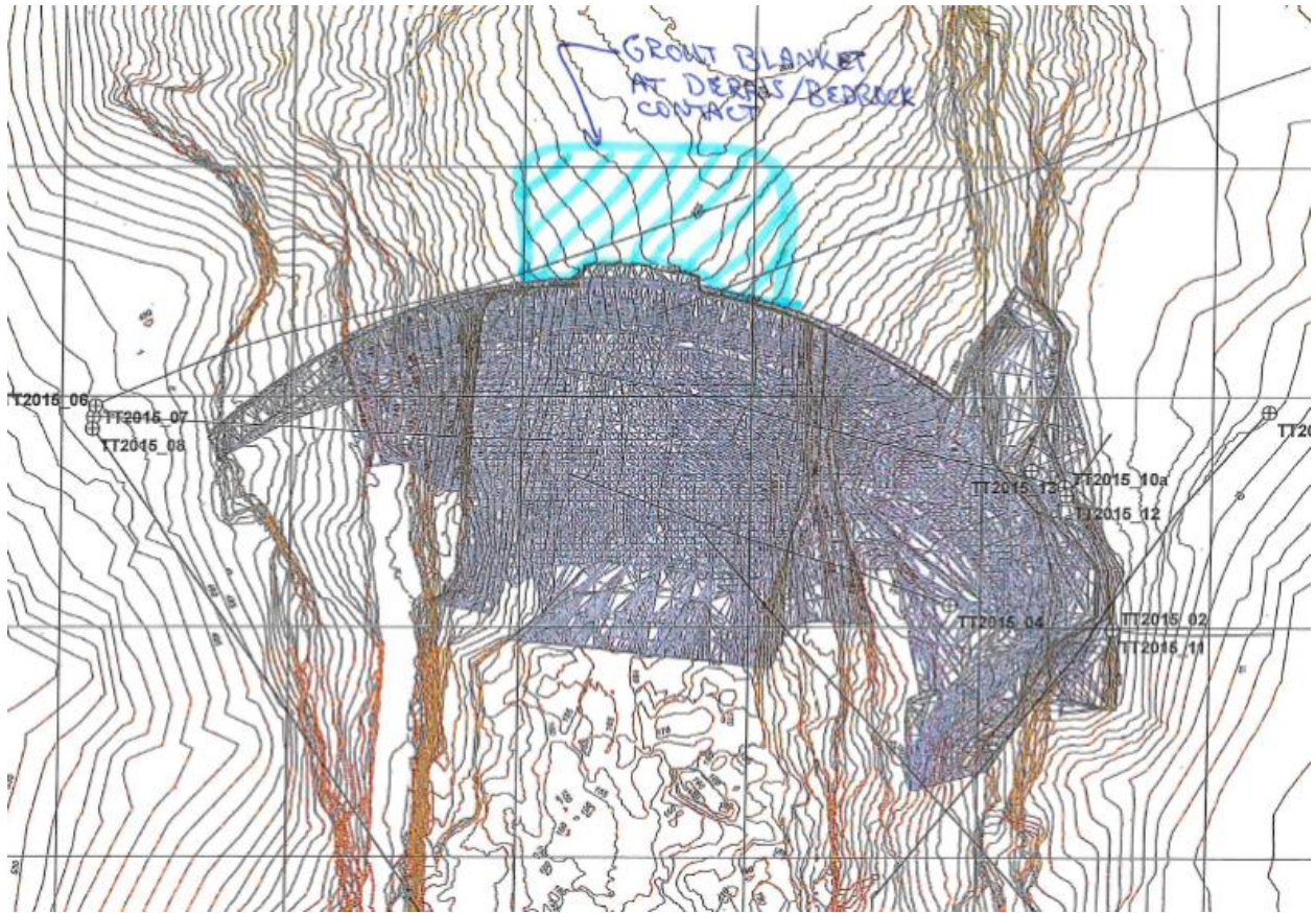
Exhibit Alt 4-2: Grout blanket in debris upstream of LBD, plan view
