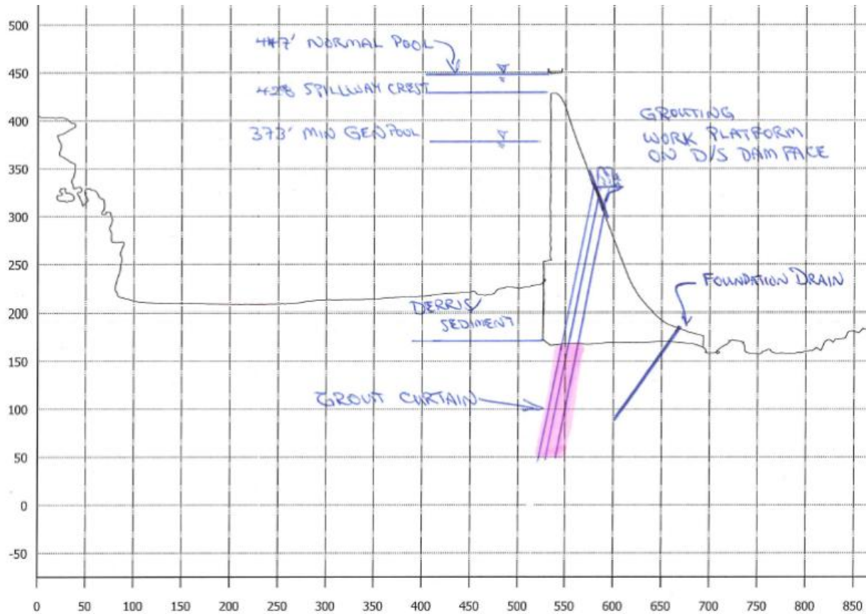
Exhibit 3E-2: Grout curtain drilling through dam from downstream dam face, section perpendicular to dam
