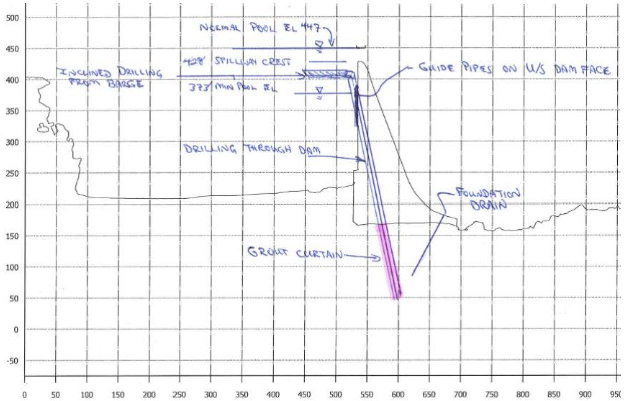
Exhibit Alt 3D-2: Grout curtain drilling from barge through upstream dam face, section perpendicular to dam
