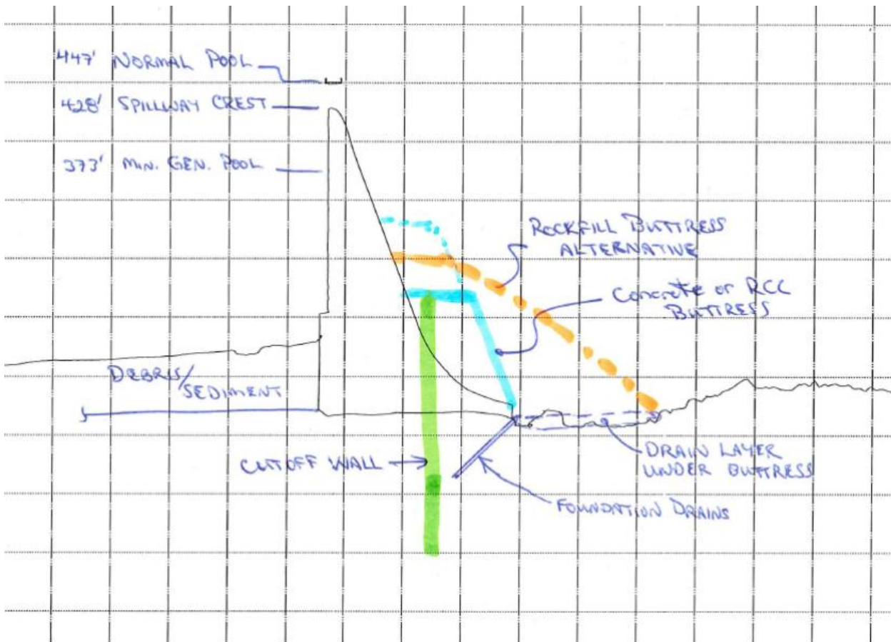
Exhibit A-Alt 2A-1: Cutoff wall downstream of dam; section perpendicular to dam.
