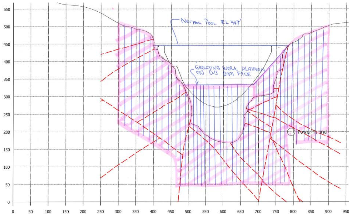
Exhibit 3E-3: Grout curtain drilling through dam from downstream dam face, cross section (grout holes shown vertical—grout holes may be inclined and grout holes in adjacent grout curtain lines drilled at different orientations)
