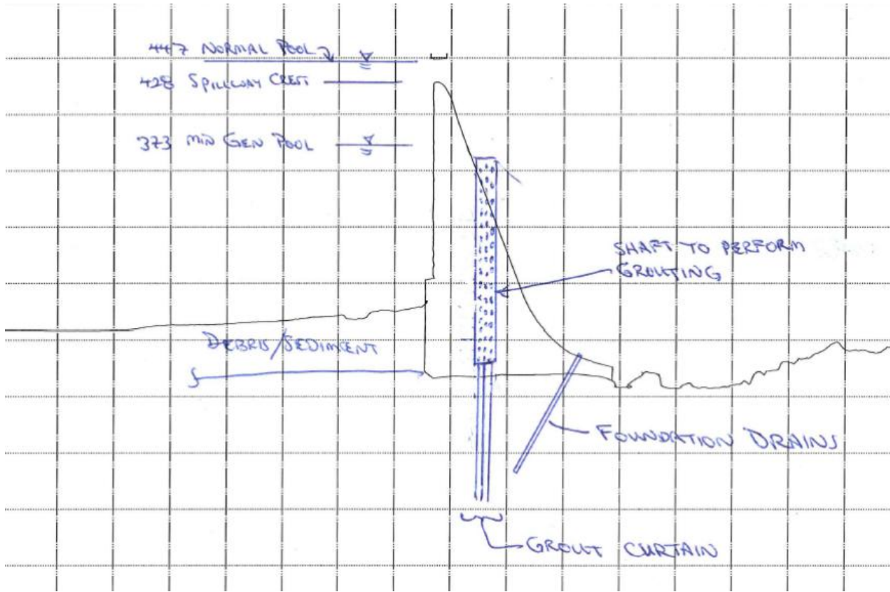
Exhibit A-Alt 3C-2: Grout curtain – drilling from shafts; section perpendicular to dam
