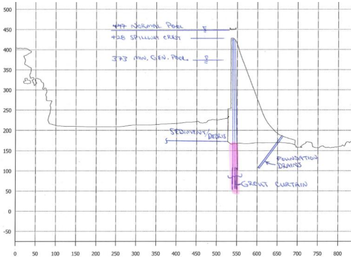
Exhibit Alt 3A-2: Grout curtain drilling through dam crest, section perpendicular to dam
