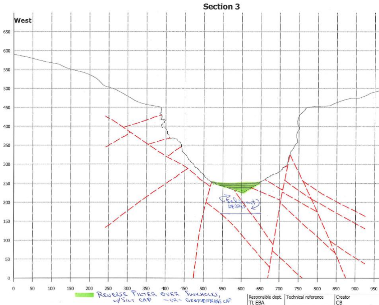
Exhibit Alt 1A-5: Blanket over forebay depressions, cross section
