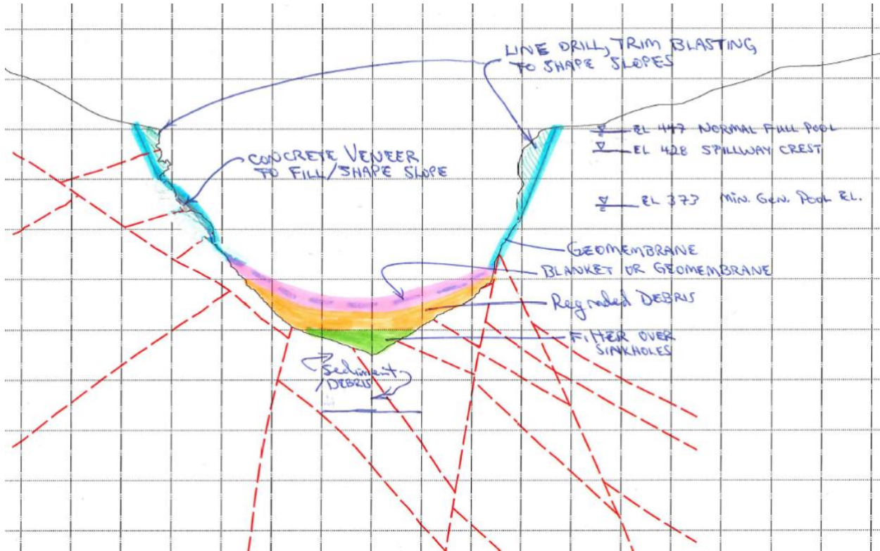
Exhibit A-Alt 1C-2: Filter over depressions and sinkholes, debris regrading, blanket, and geomembrane on slope; cross section
