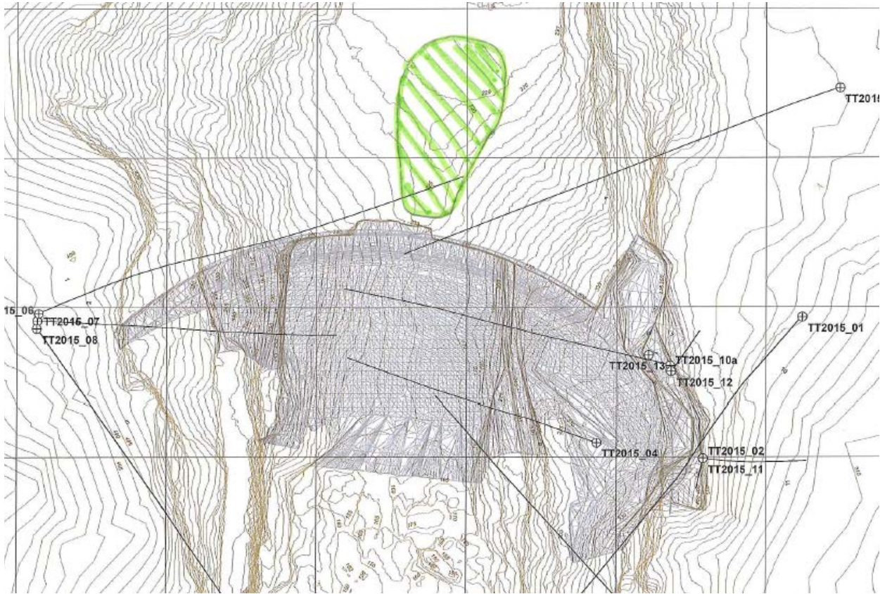
Exhibit Alt 1A-2: Blanket over forebay depressions, plan view
