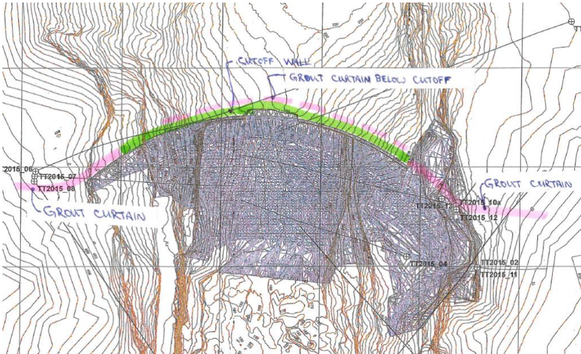
Exhibit Alt 2D-1: Cutoff wall and grout curtain upstream of dam, plan view
