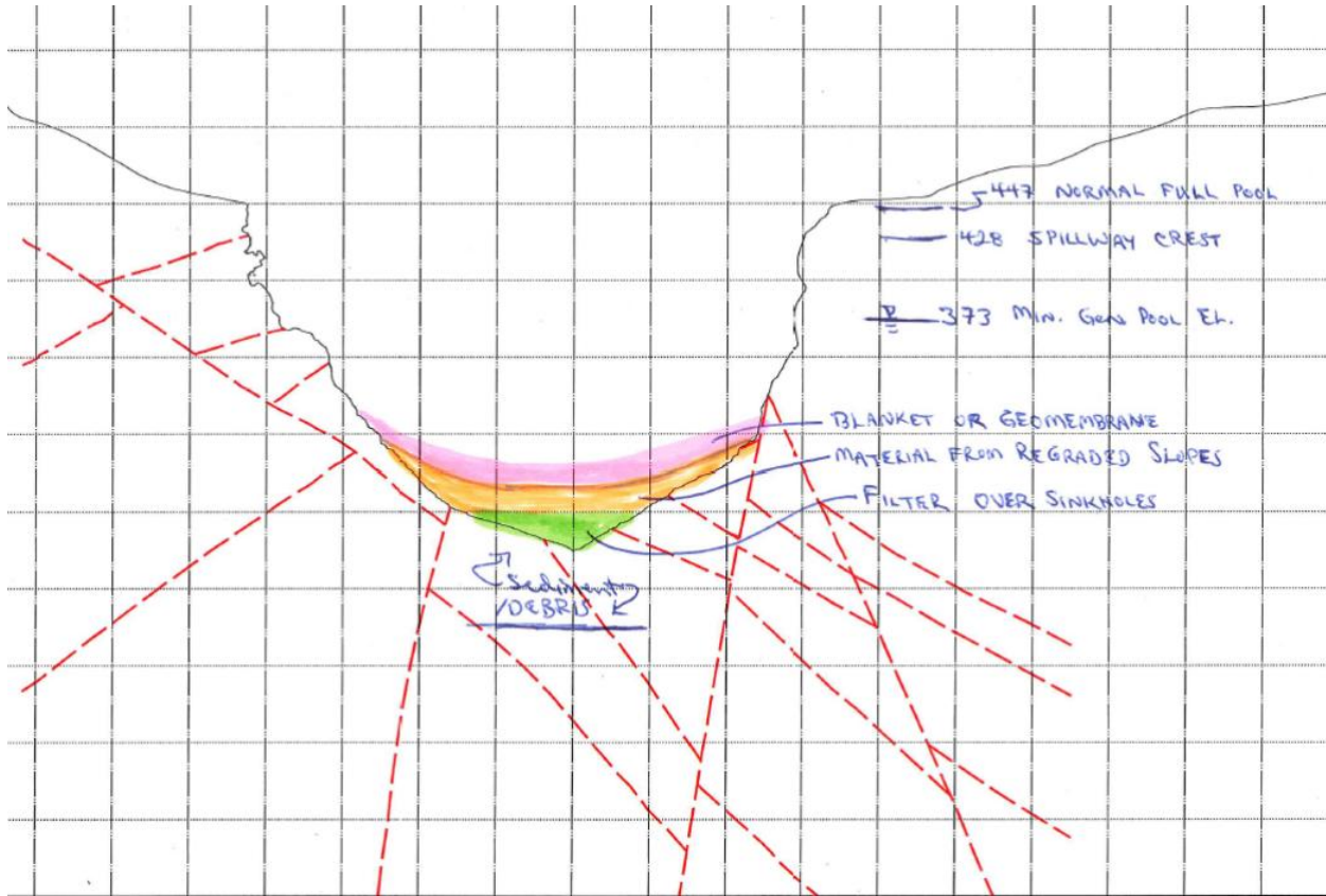
Exhibit A-Alt 1B-2: Filter over depressions and sinkholes, debris regrading, and blanket; cross section
