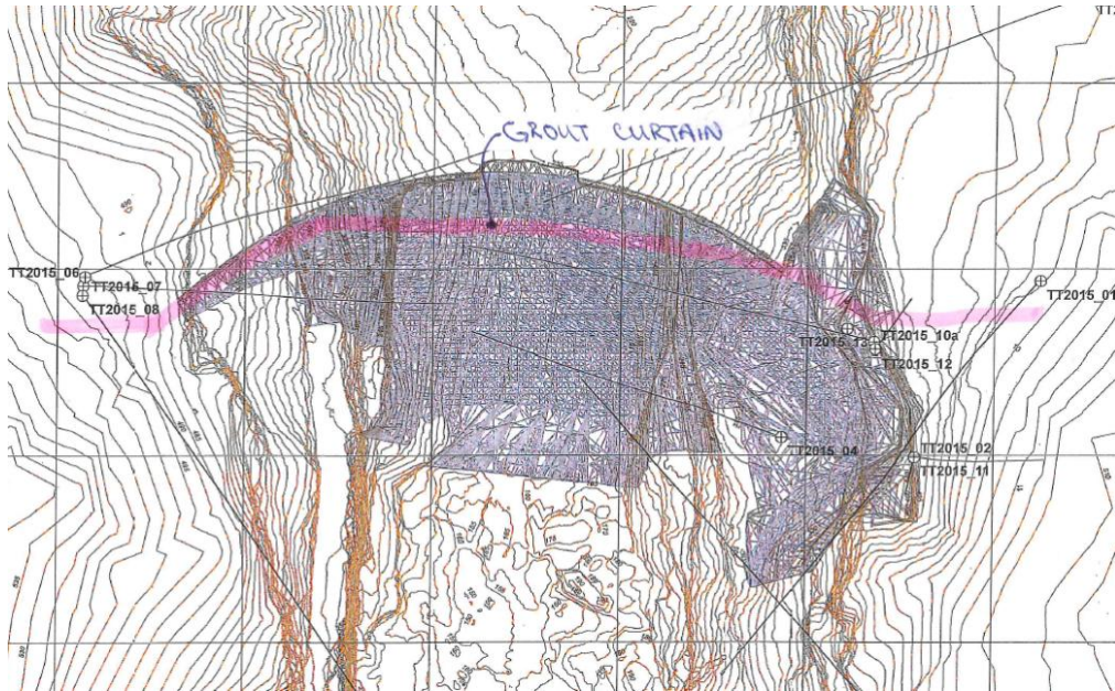
Exhibit Alt 3D-1: Grout curtain drilling from barge through upstream dam face, plan view
