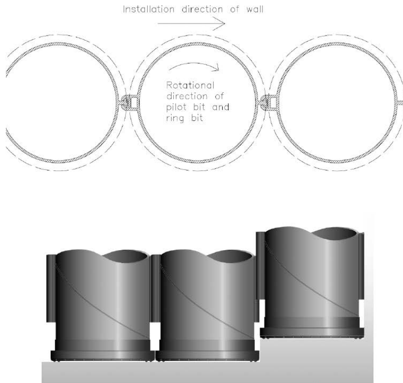
Exhibit Alt 2D-5: Principle of RD piles, interlock, and installation (Uotinen and Jokiniemi, 2012)
