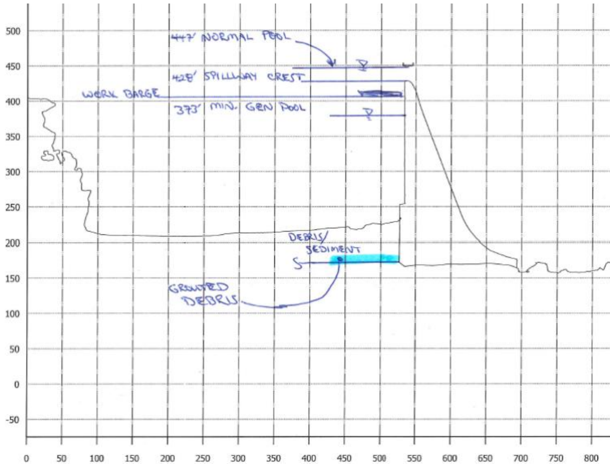
Exhibit Alt 4-3: Grout blanket in debris upstream of LBD, section perpendicular to dam
