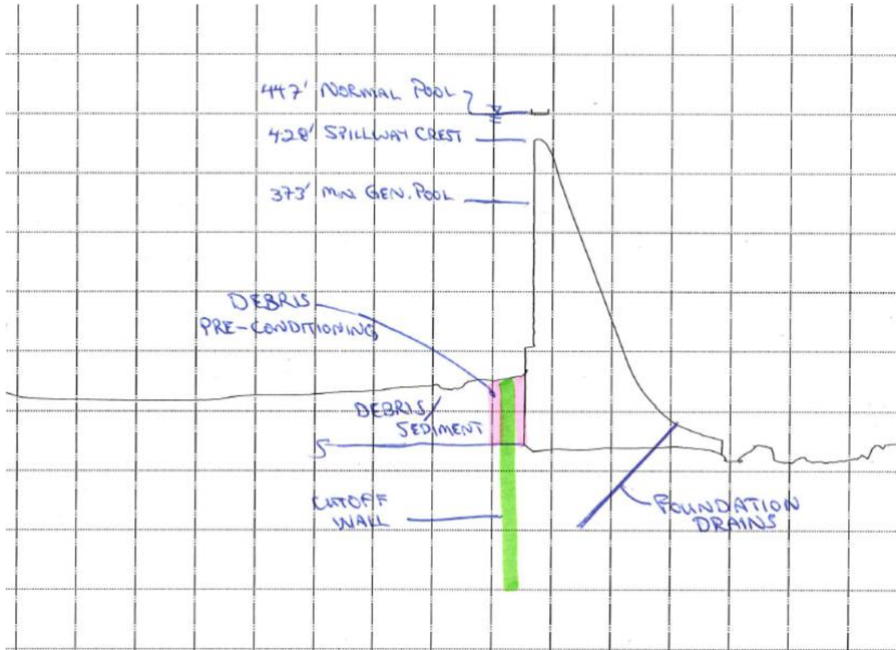
Exhibit A-Alt 2C-1: Cutoff wall upstream of dam; section perpendicular to dam
