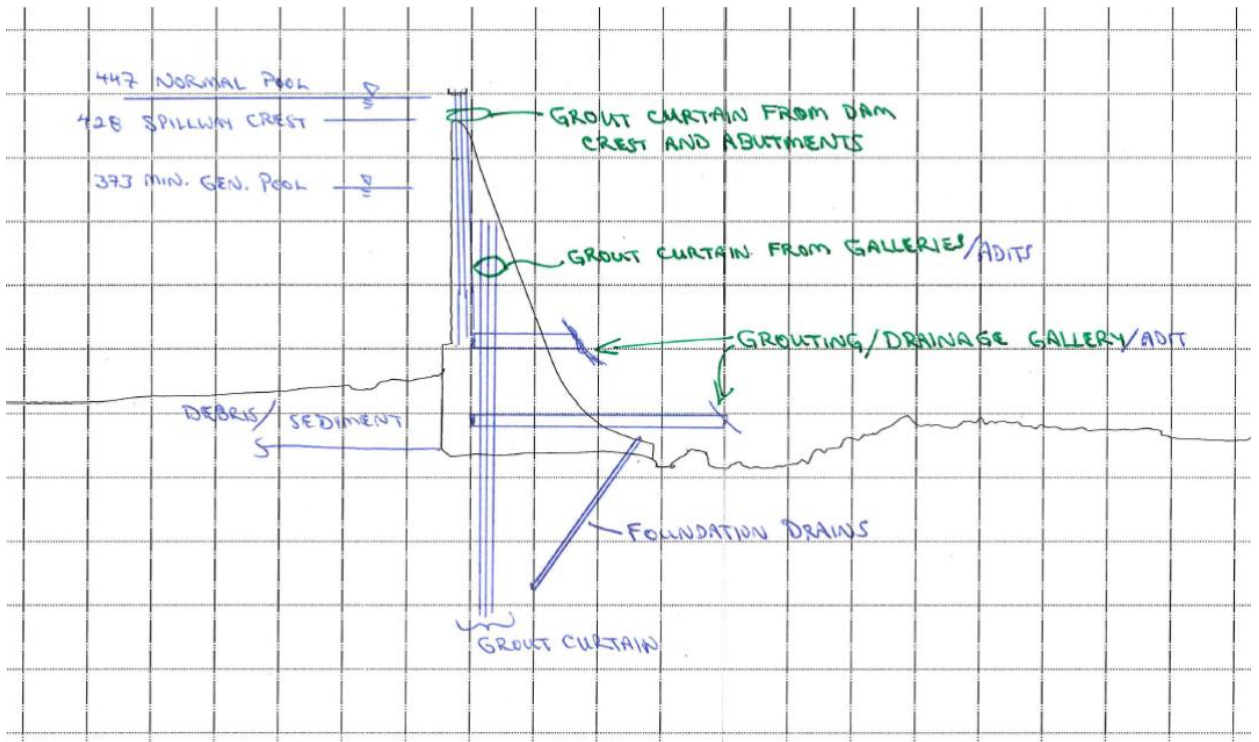
Exhibit A-Alt 3B-2: Grout curtain – drilling from adits; section perpendicular to dam
