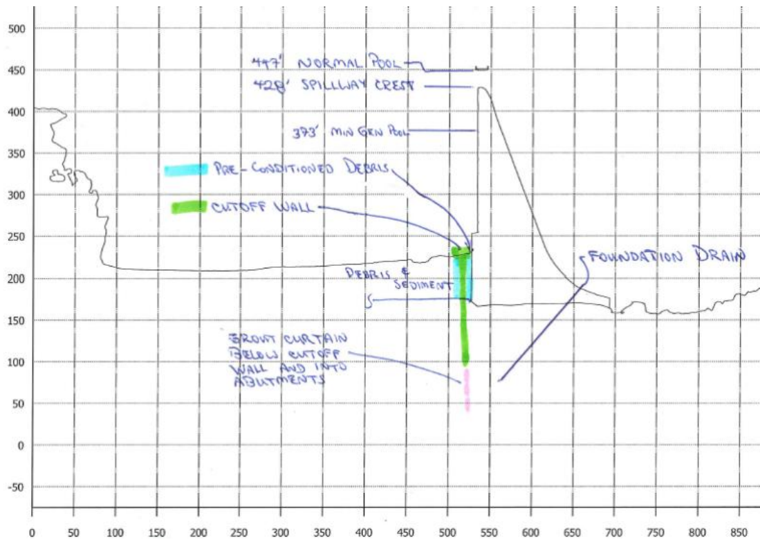
Exhibit Alt 2D-2: Cutoff wall and grout curtain upstream of dam, section perpendicular to dam
