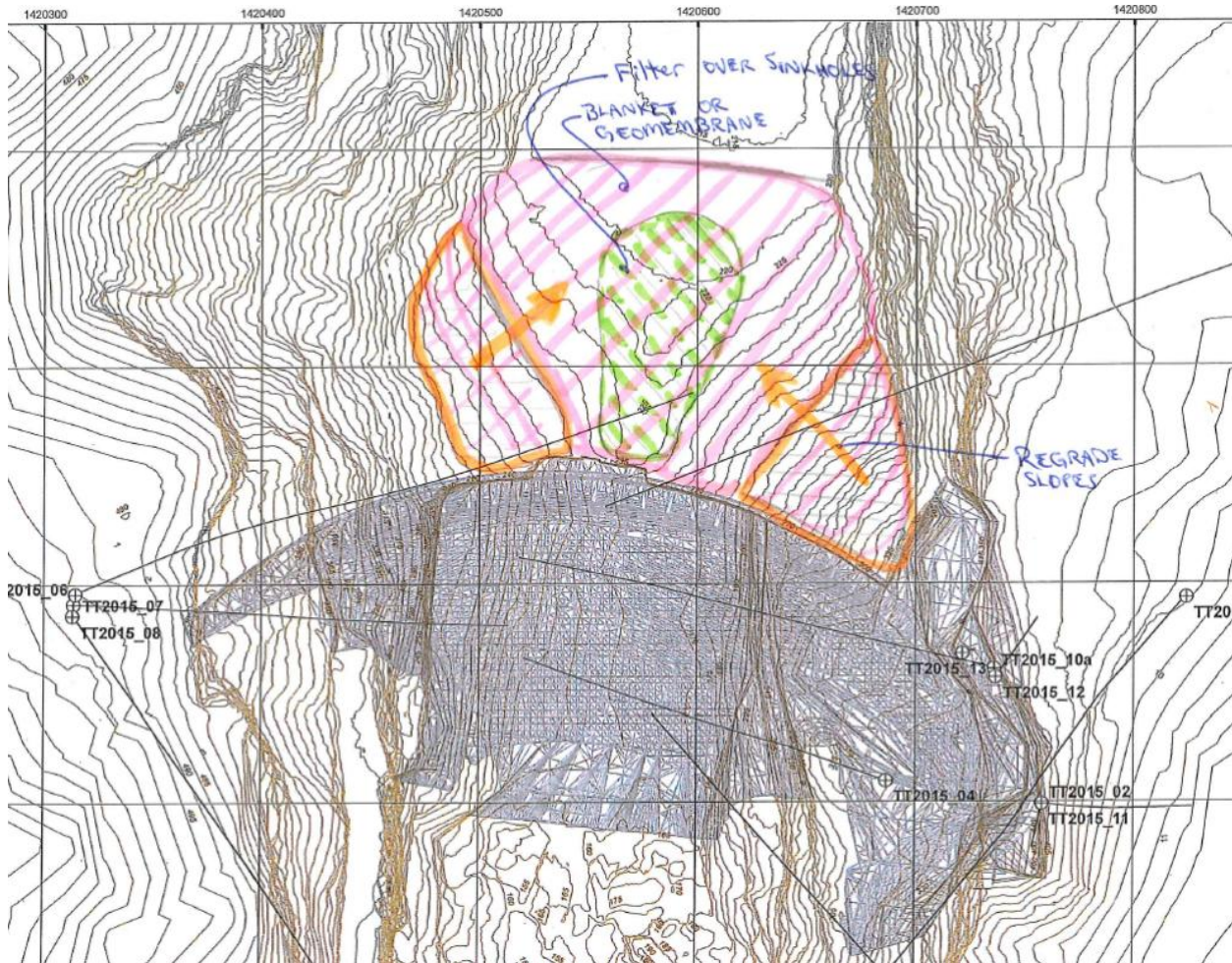
Exhibit A-Alt 1B-1: Filter over depressions and sinkholes, debris regrading, and blanket; plan view
