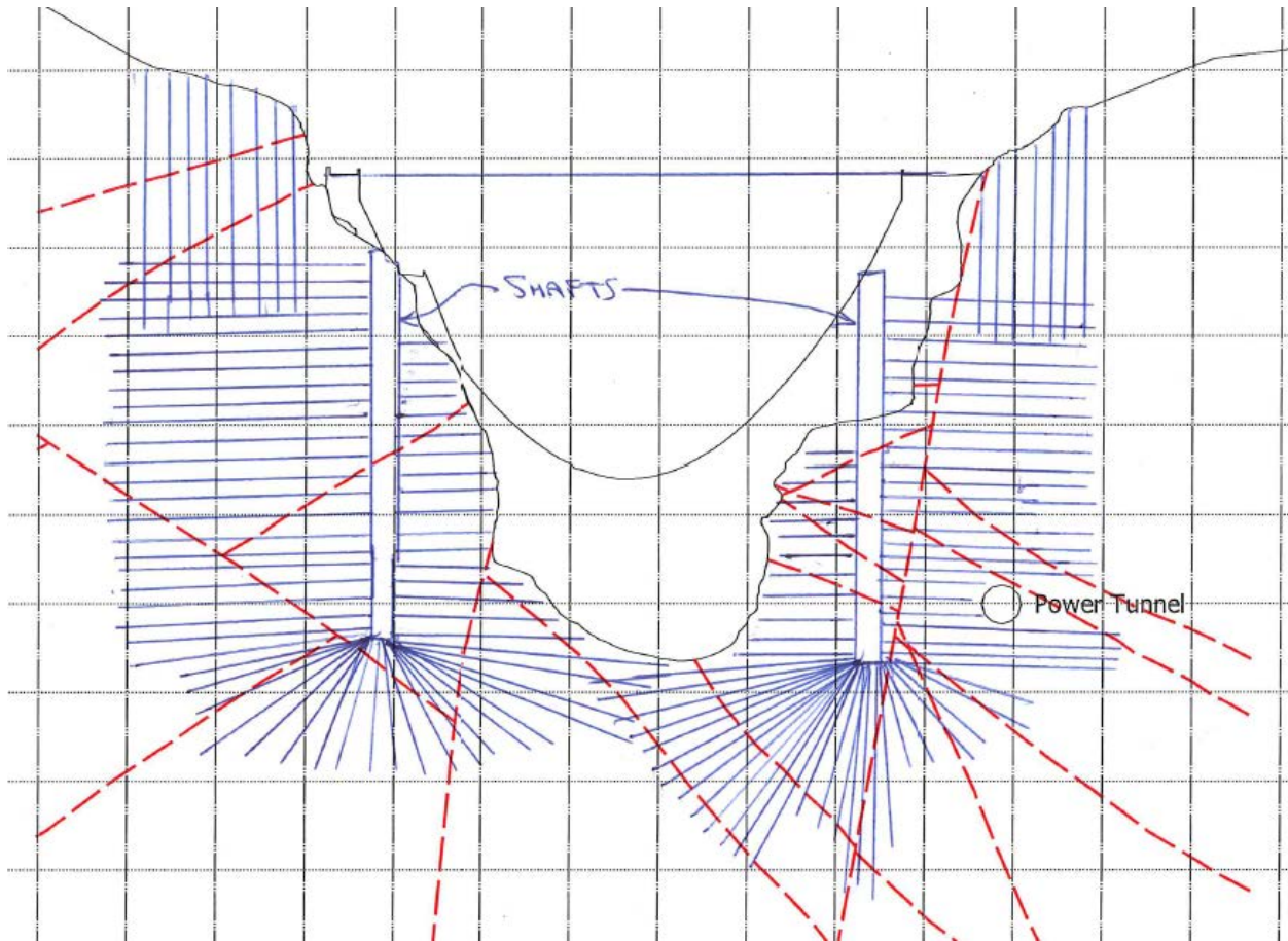
Exhibit A-Alt 3C-1: Grout curtain – drilling from shafts; cross section (vertical and horizontal grout holes shown for convenience—grout hole orientations would vary and would be different on adjacent grout lines.)
