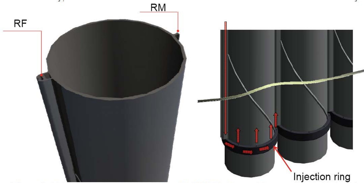
Exhibit Alt 2D-7: RD pile interlock details (left) and grout injection ring (right) (Uotinen and Jokiniemi, 2012)
