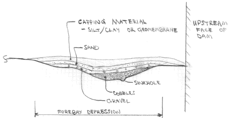
Exhibit Alt 1A-3: Blanket over forebay depression, detail
