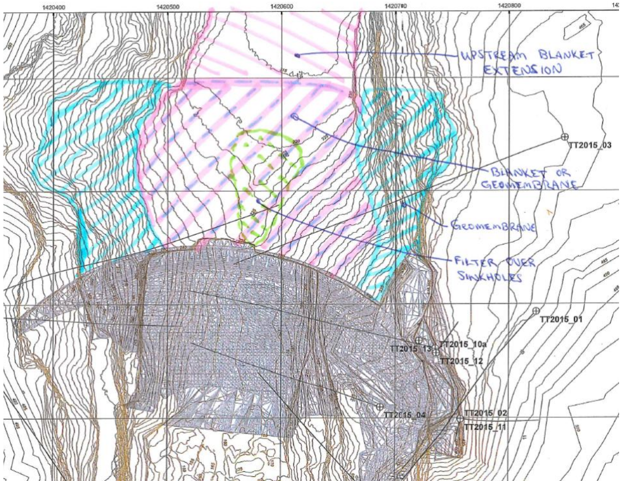
Exhibit A-Alt 1C-1: Filter over depressions and sinkholes, debris regrading, blanket, and geomembrane on slope; plan view
