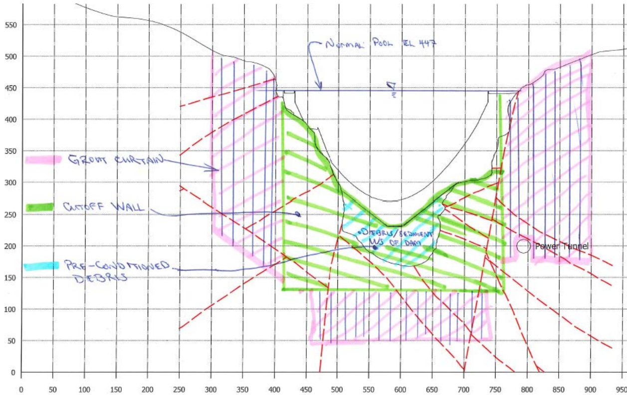
Exhibit Alt 2D-3: Cutoff wall and grout curtain upstream of dam, cross section (grout holes shown vertical—grout holes may be inclined and grout holes in adjacent grout curtain lines drilled at different orientations)
