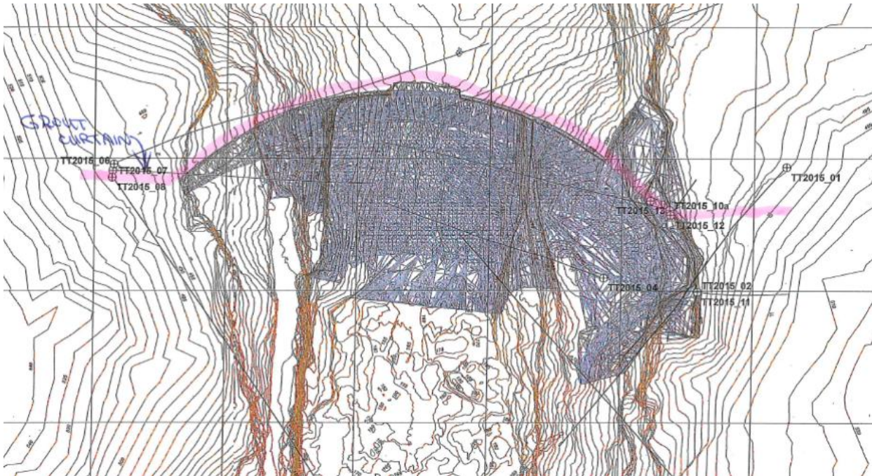
Exhibit Alt 3F-1: Grout curtain upstream of dam, drilling from barge upstream of dam, plan view
