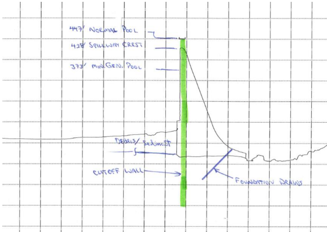
Exhibit A-Alt 2B-1: Cutoff wall through dam; section perpendicular to dam
