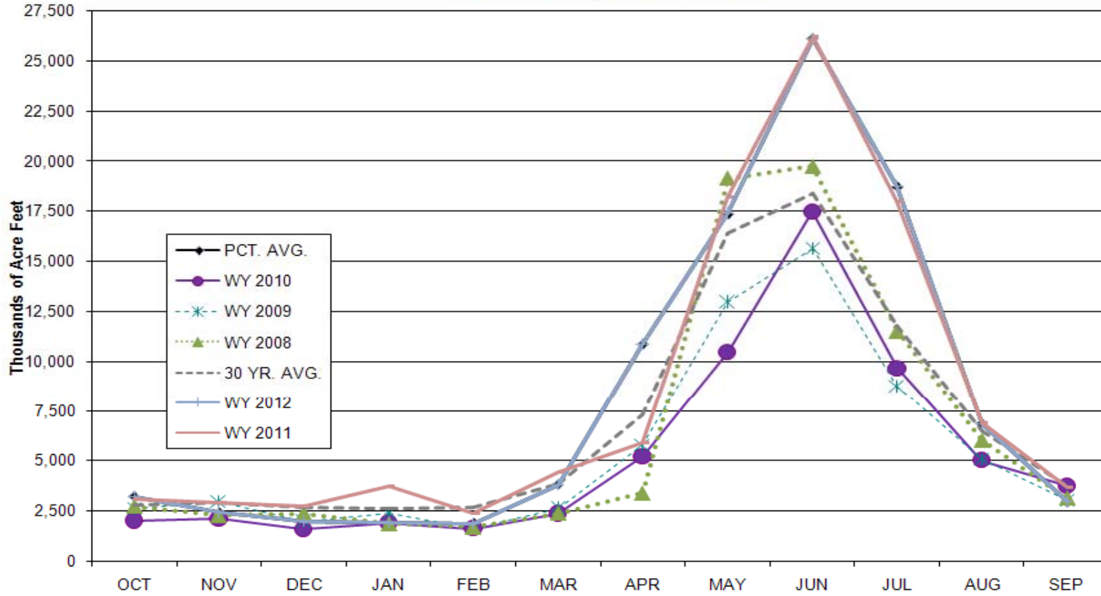
Monthly Runoff Volumes Grand Coulee Water Years 2008 through September 2012 Actuals and 30 Yr Average for 1971-2000
