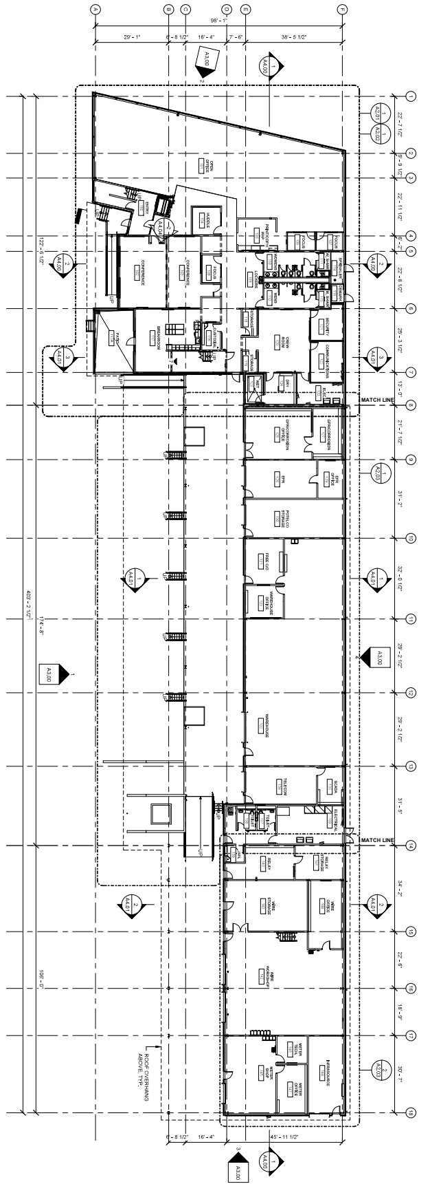
1 OVERALL FLOOR PLAN 1/16" = 1'-0"
