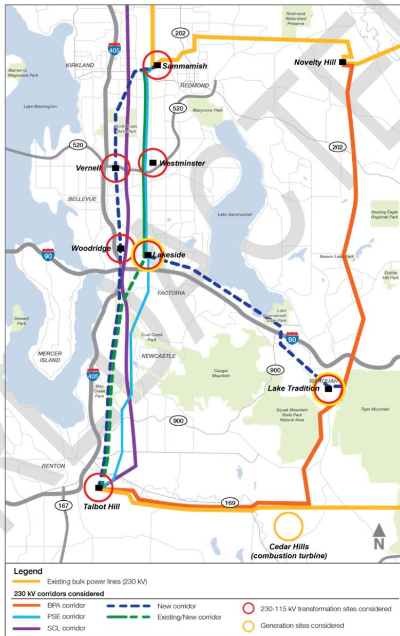
Figure 4-2: Locations of Transformer and Generation Alternatives Studied
