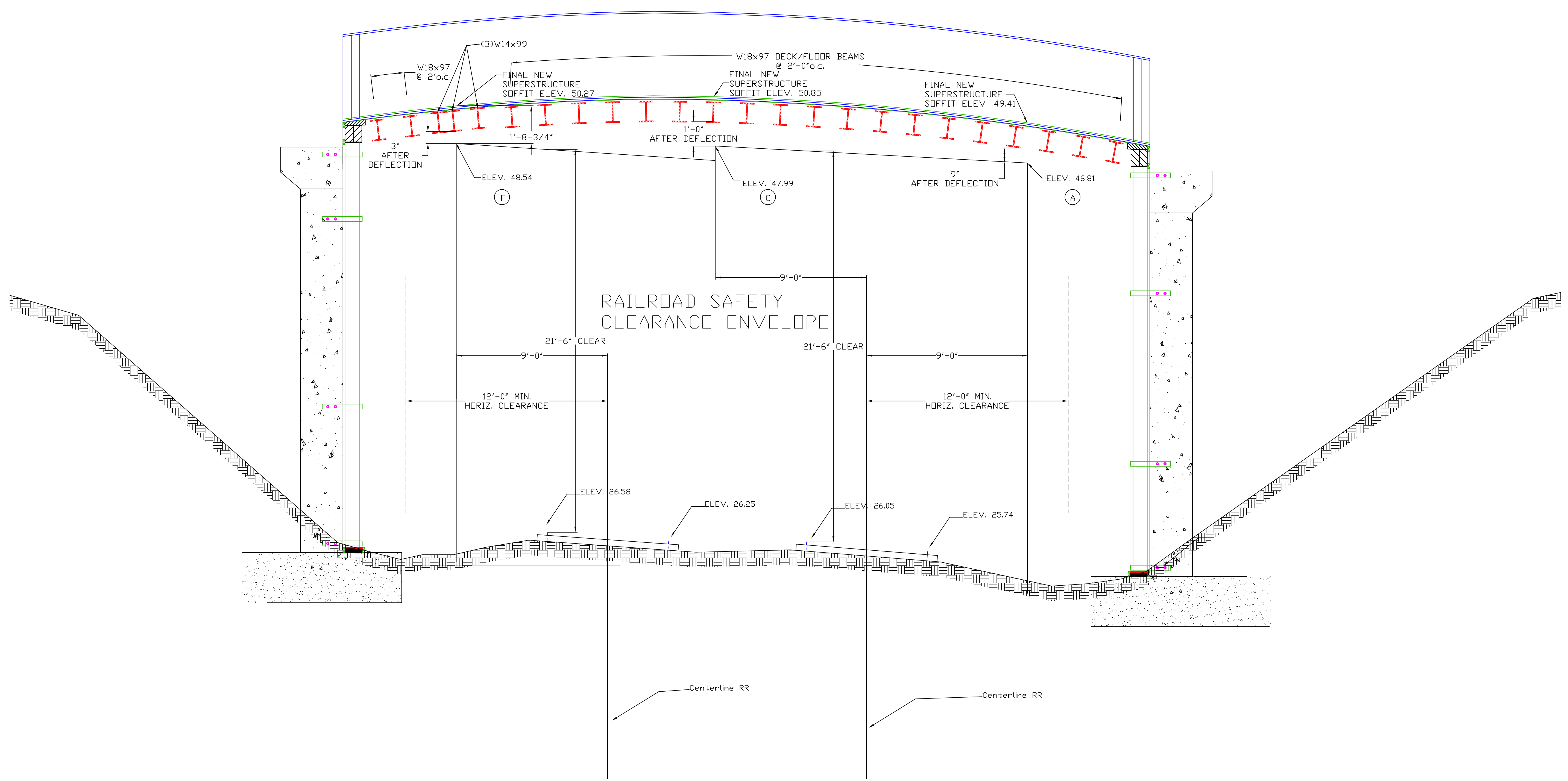
FALSEWORK ELEVATION
