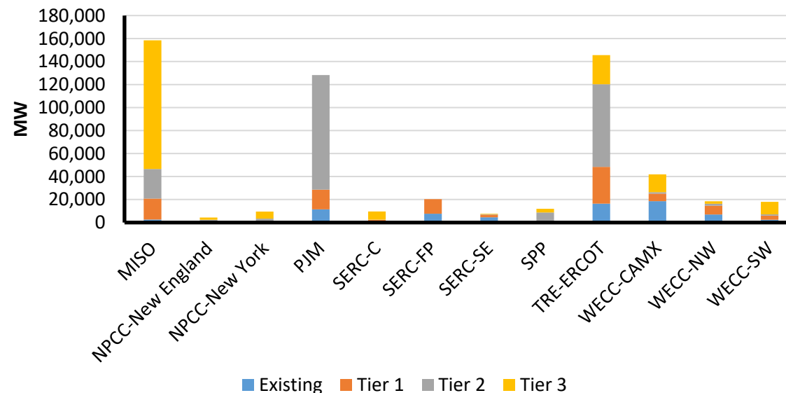
Figure 17: Solar Capacity Existing and Planned through 2033
