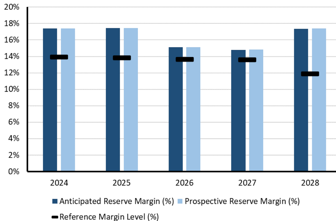
Figure 13: WECC-BC Five-Year Planning Reserve Margin
