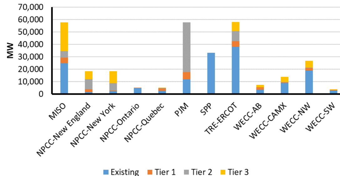
Figure 18: Wind Capacity Existing and Planned through 2033
