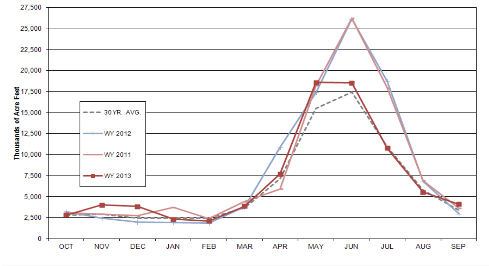
Grand Coulee Monthly Runoff Volumes Water Years 2011-2013 (Oct-Sep) Actuals and 30 Yr Average 1981-2010
