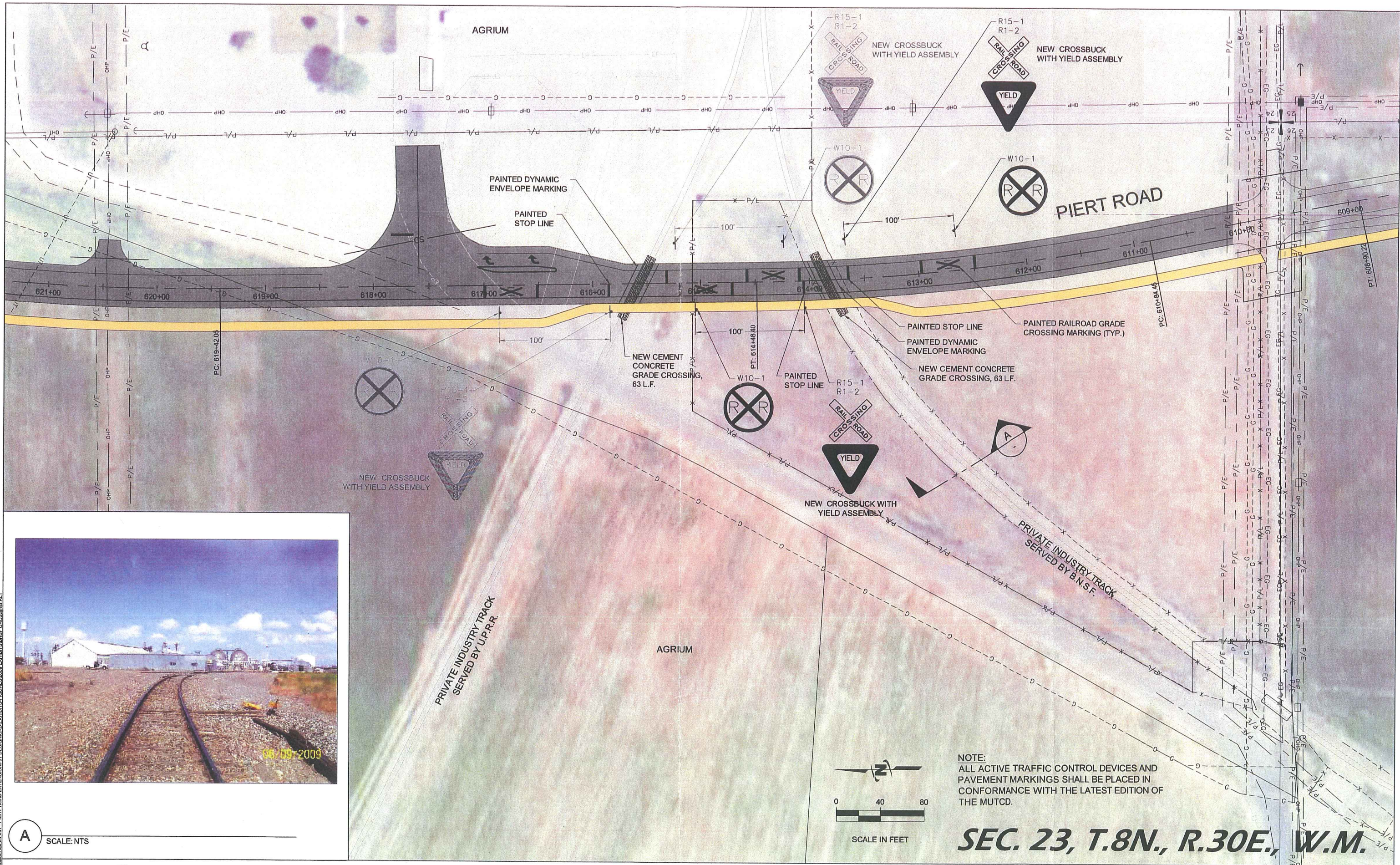
FIGURE 1 B.N.S.F. CROSSING UPGRADE BENTON COUNTY - PIERT ROAD EXTENSION
