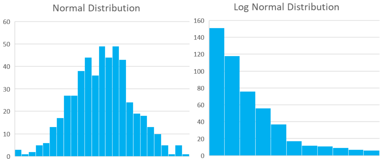
Figure 7.4: Monte Carlo Example - 500 Draws
