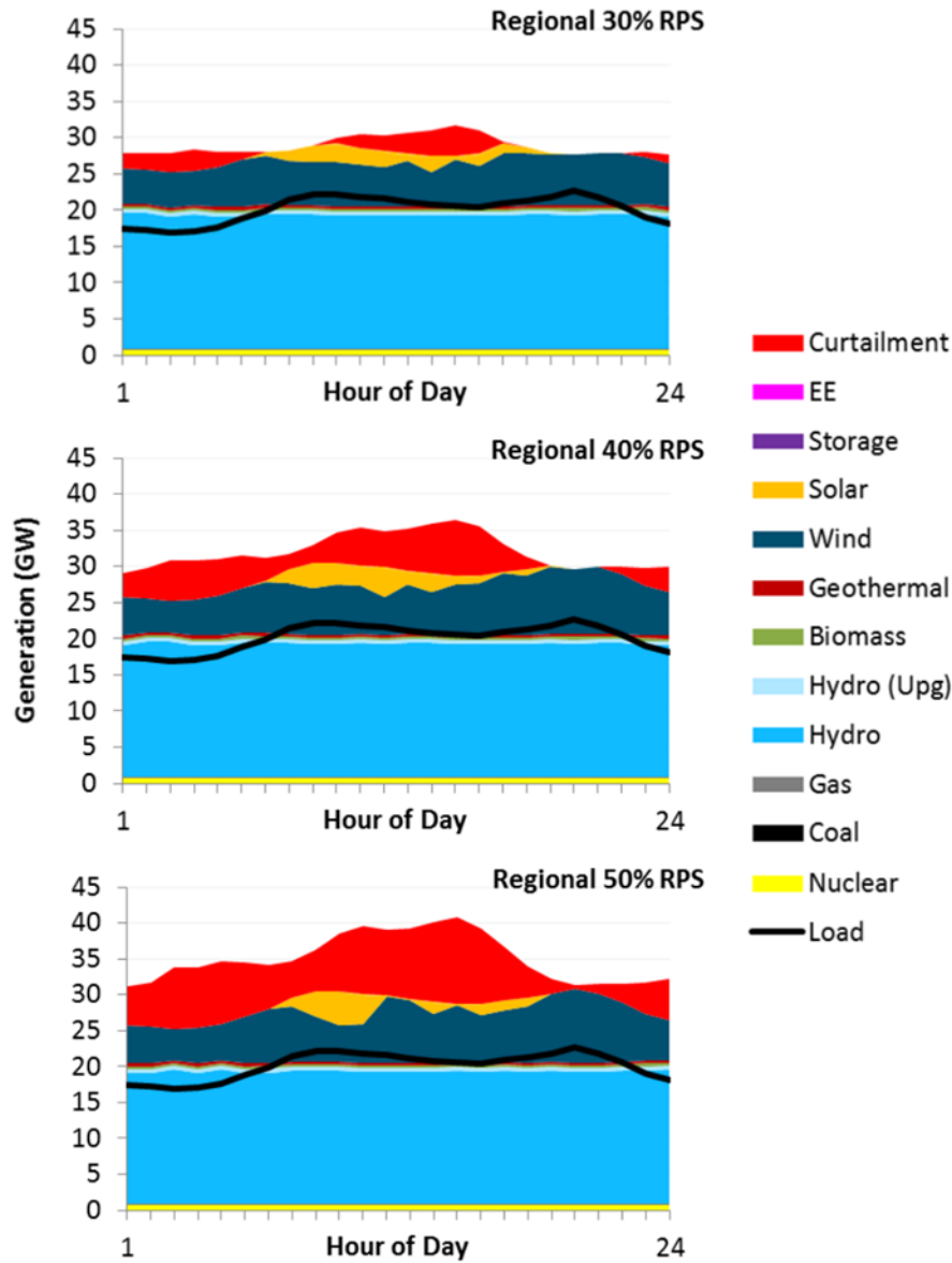
Figure 6.8: Increasing renewable curtailment observed with increasing regional RPS goals 124
