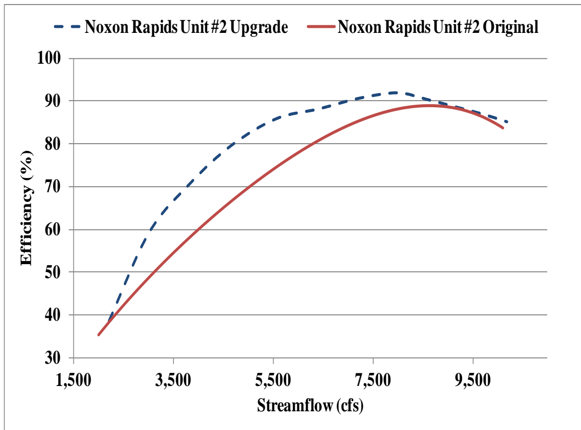
Illustration 5: Noxon Rapids Unit #2 Turbine Curves
