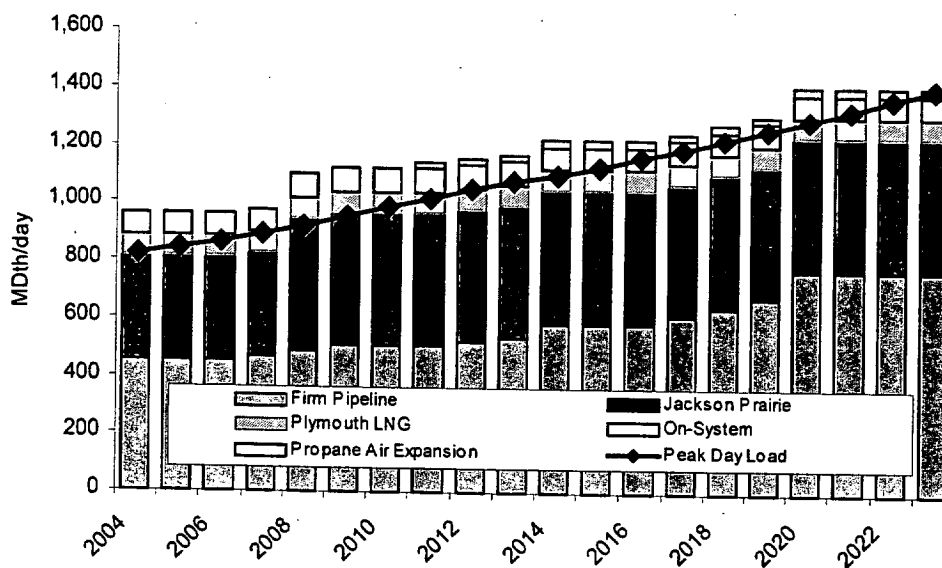
Exhibit XVI-4 PSE Peak Day Load and Delivery Capacity High Load Growth
