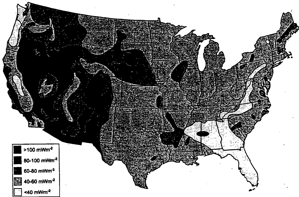
Figure 1. Geothermal resource quality in the United States.
