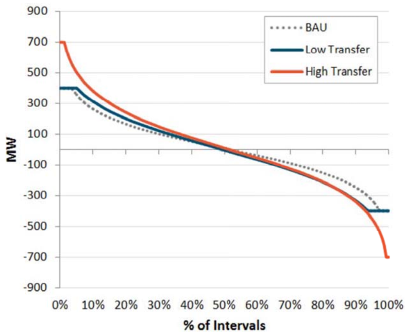
Figure 7. PSE plus PacifiCorp Imbalance Duration Curve
