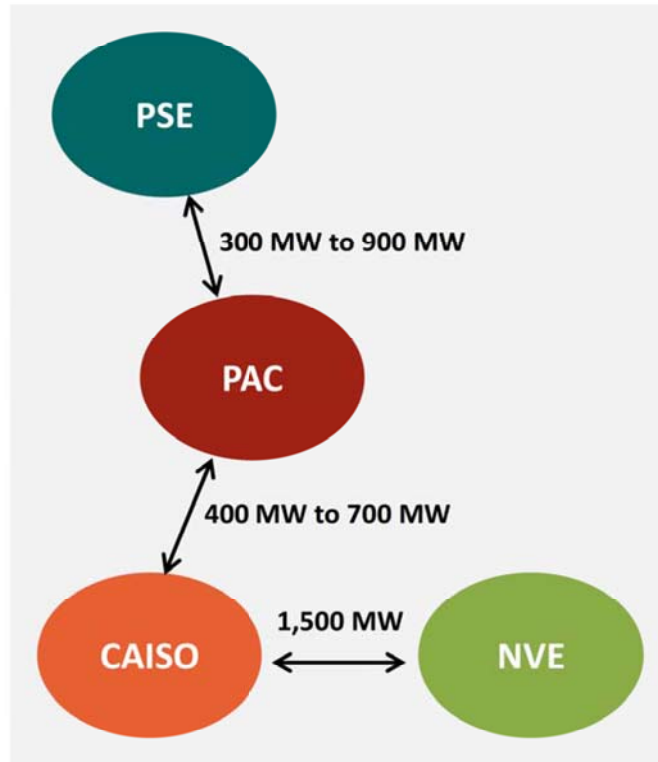
Figure 1. Real-time Transfer Capabilities across the EIM Footprint
