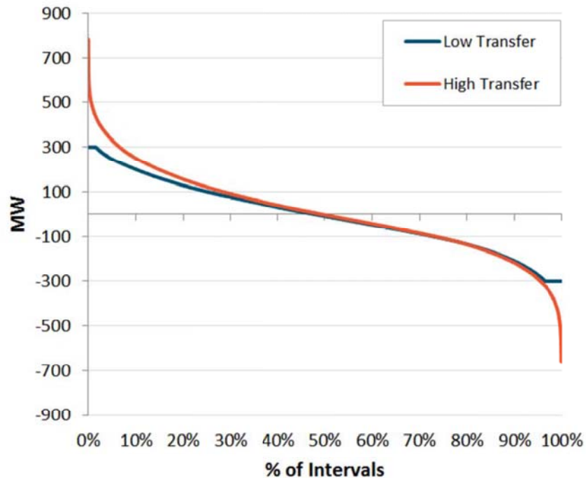
Figure 6. PSE Imbalance Duration Curve
