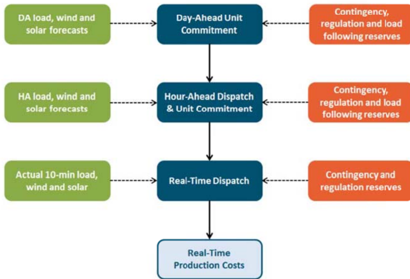
Figure 2. PLEXOS Three-Stage Sequential Simulation Process
