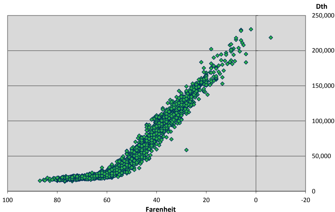
Figure 2.2: Example Demand vs. Average Temperature – WA/ID
