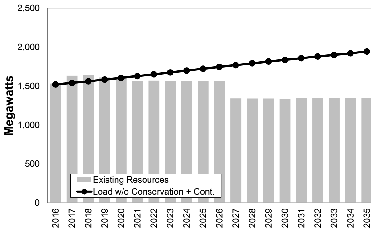
Figure 6.7: Summer 18-Hour Capacity Load and Resources
