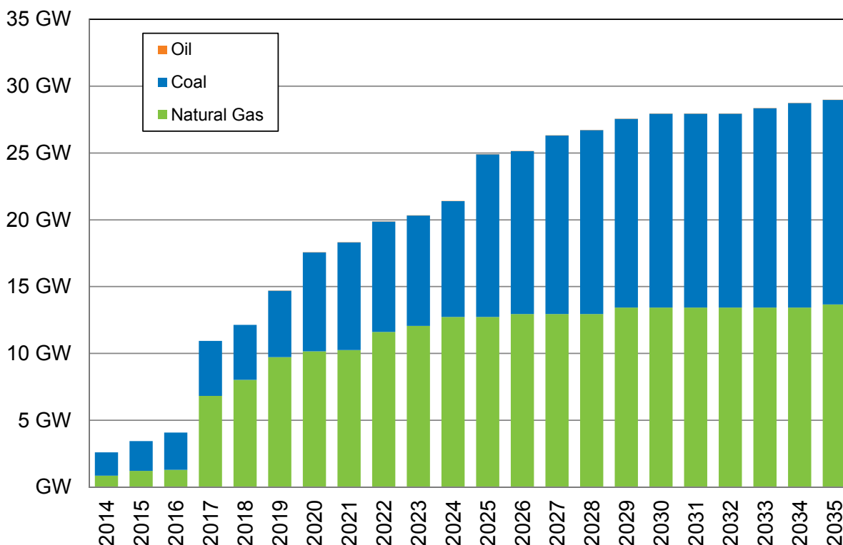
Figure 10.3: Resource Retirements (Nameplate Capacity)
