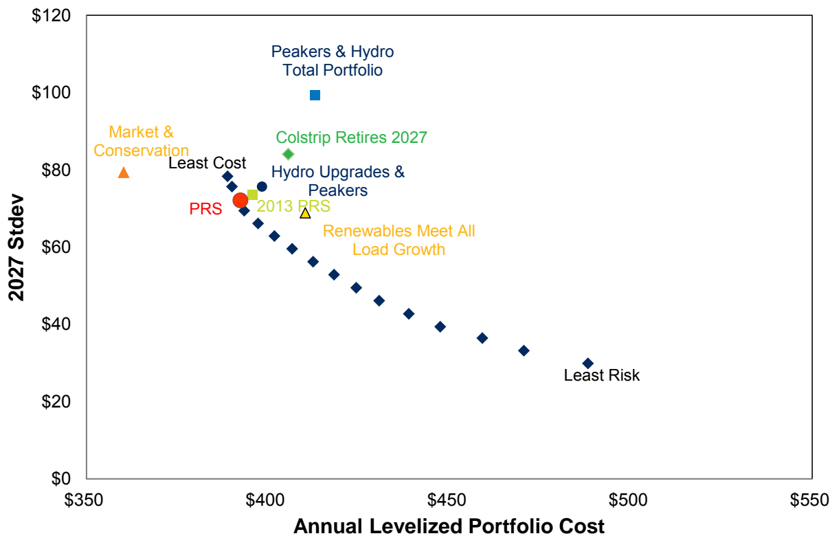
Figure 12.10: Other Resource Strategy Portfolio Cost and Risk (Millions)
