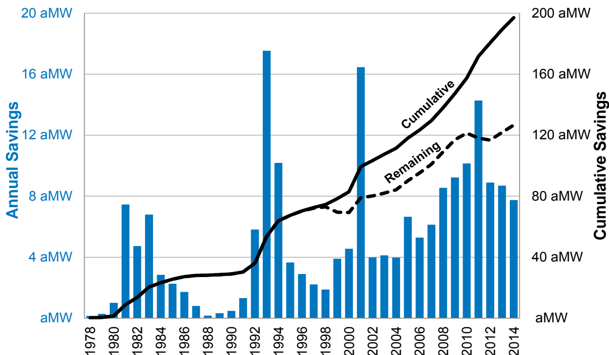
Figure 5.1: Historical and Forecast Conservation Acquisition (system)
