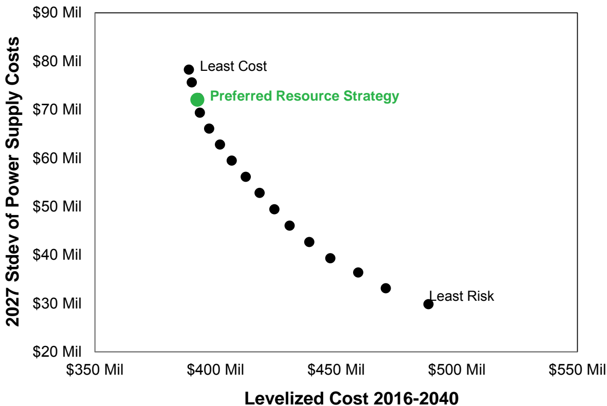
Figure 1.5: Efficient Frontier
