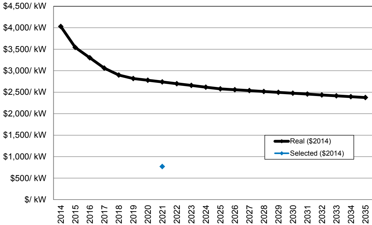
Figure 12.13: Utility Scale Storage Tipping Point Analysis (2014 $)
