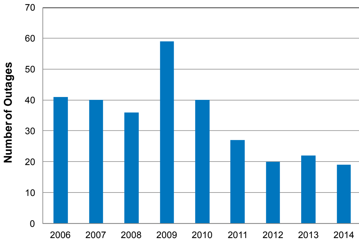
Figure 8.3: Spokane's 9th and Central Feeder (9CE12F4) Outage History
