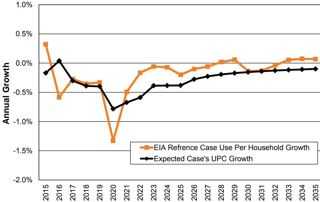
Figure 3.15: UPC Growth Forecast Comparison to EIA
