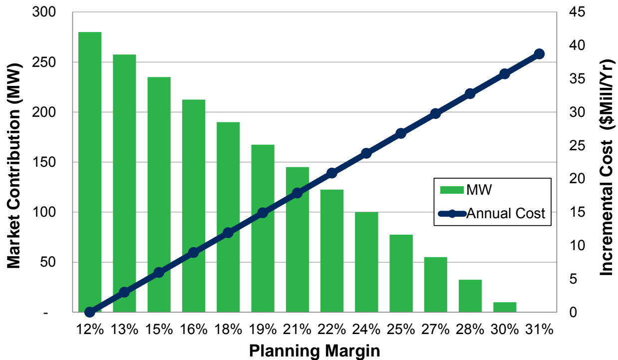
Figure 6.1: 2020 Market Reliance & Capacity Cost Tradeoffs
