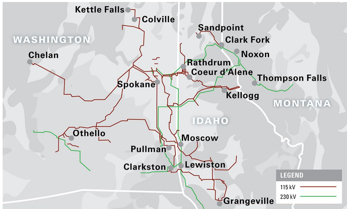
Figure 8.2: Avista Transmission Map
