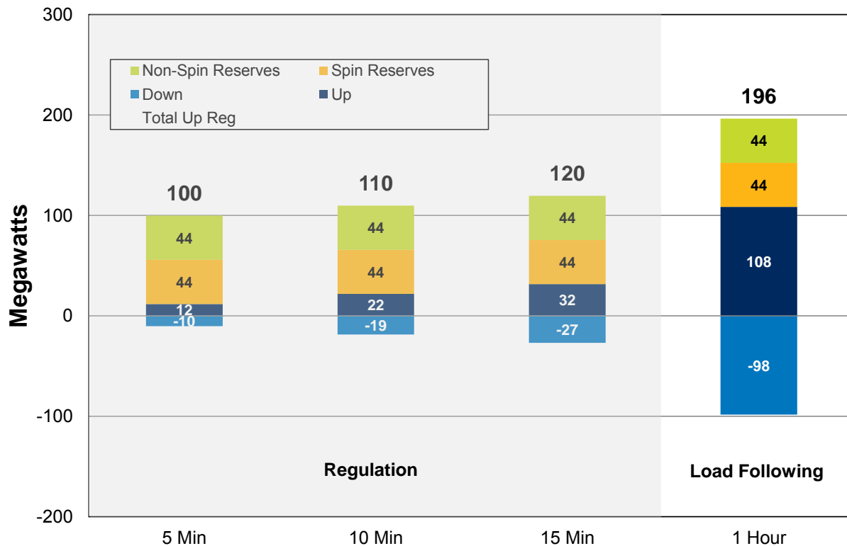
Figure 6.4: 95th Percentile Capacity Requirements
