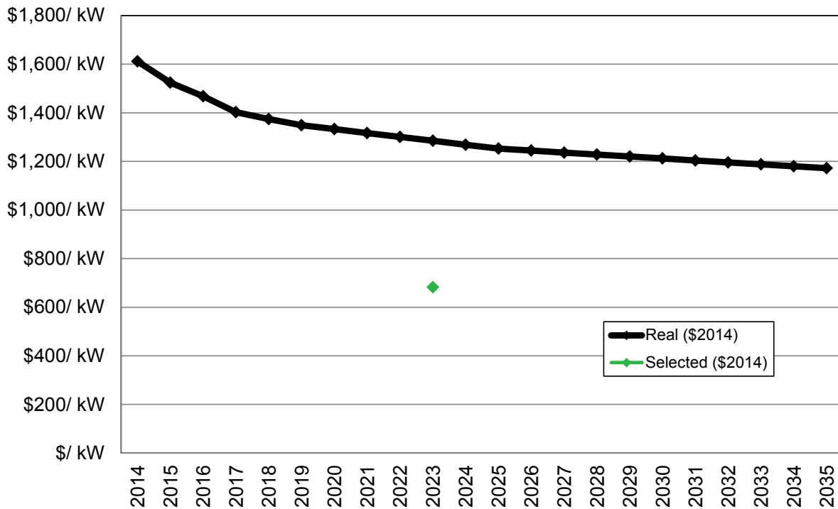
Figure 12.12: Utility Scale Solar Tipping Point Analysis (2014 $)
