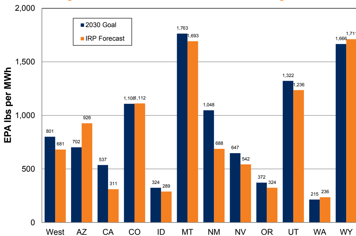
Figure 10.17: EPA’s CPP 2030 State Goal vs. Modeling Result
