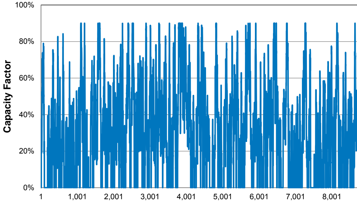
Figure 10.12: Wind Model Output for the Northwest Region
