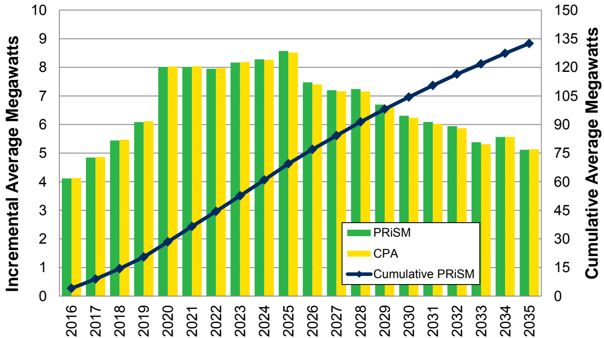
Figure 11.6: Energy Efficiency Annual Expected Acquisition Comparison 6
