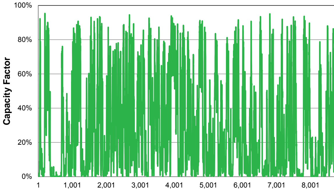
Figure 10.13: 2014 Actual Wind Output BPA Balancing Authority 3
