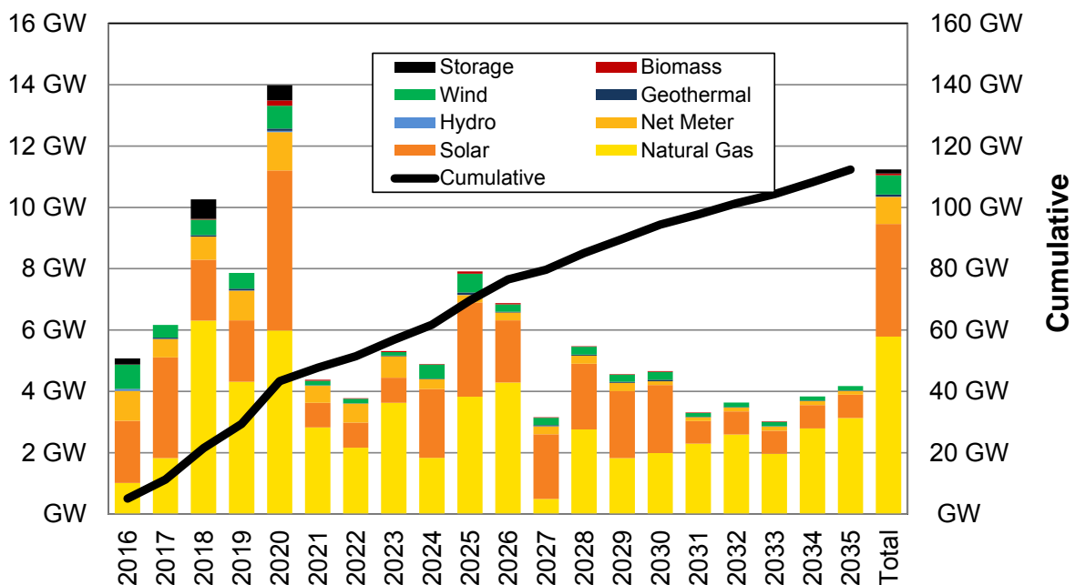
Figure 10.4: Cumulative Generation Resource Additions (Nameplate Capacity)
