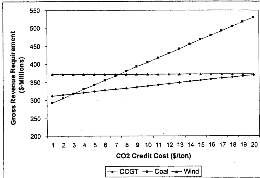
Impact of CO2 Credit Prices on Generation Technologies
