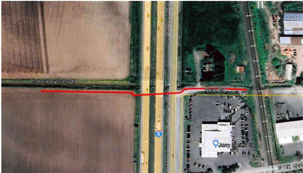
Figure 1: Overall view of the proposed 3” Burlington HP Replacement (Red) pipeline alignment.
