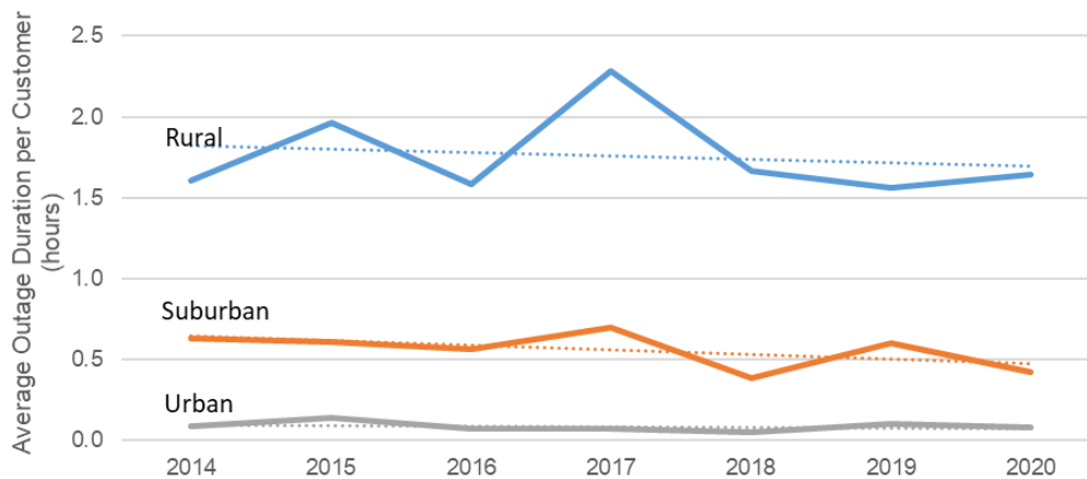
Figure 9: SAIDI by Feeder Classification 2014-2020
