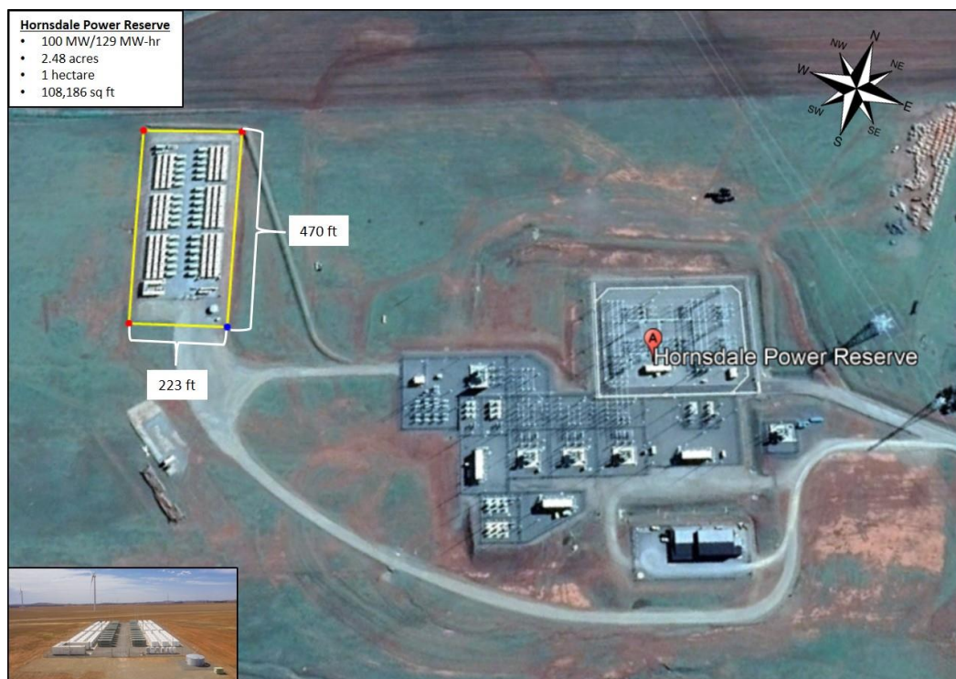
Figure 1.1 Hornsdale Power Reserve ESS
