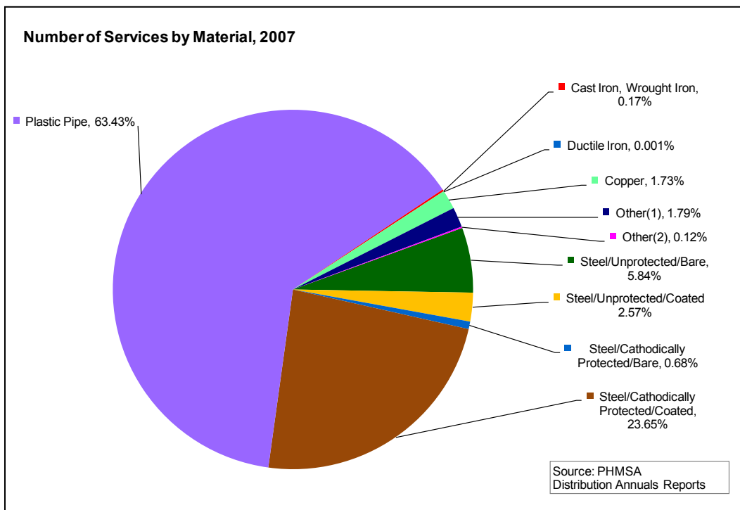
Figure 2. Piping Materials of Mains and Service Lines in Distribution Systems*
