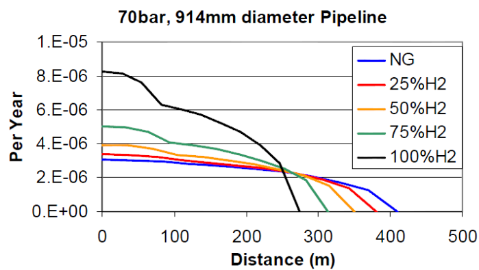
Figure 12. Risk to an individual per year as a function of distance from the pipeline. Risk shown is individual risk: the likelihood of a person becoming a fatality in a given year. Source: Lowesmith 2009. Displayed with permission.
