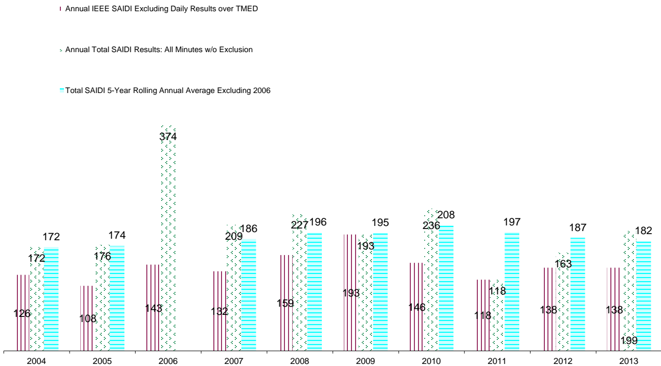
Chart 1: 2004-2013 AVA SAIDI Performance in Different Measurements by Year
