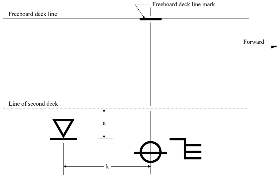
k = a distance between 21 inches and six feet six inches. a = the distance between the line of the second deck and the uppermost part of the load line grid.
