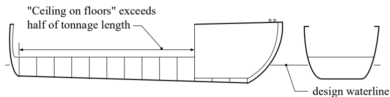
Example of vessel that fails the one-half tonnage length criterion
