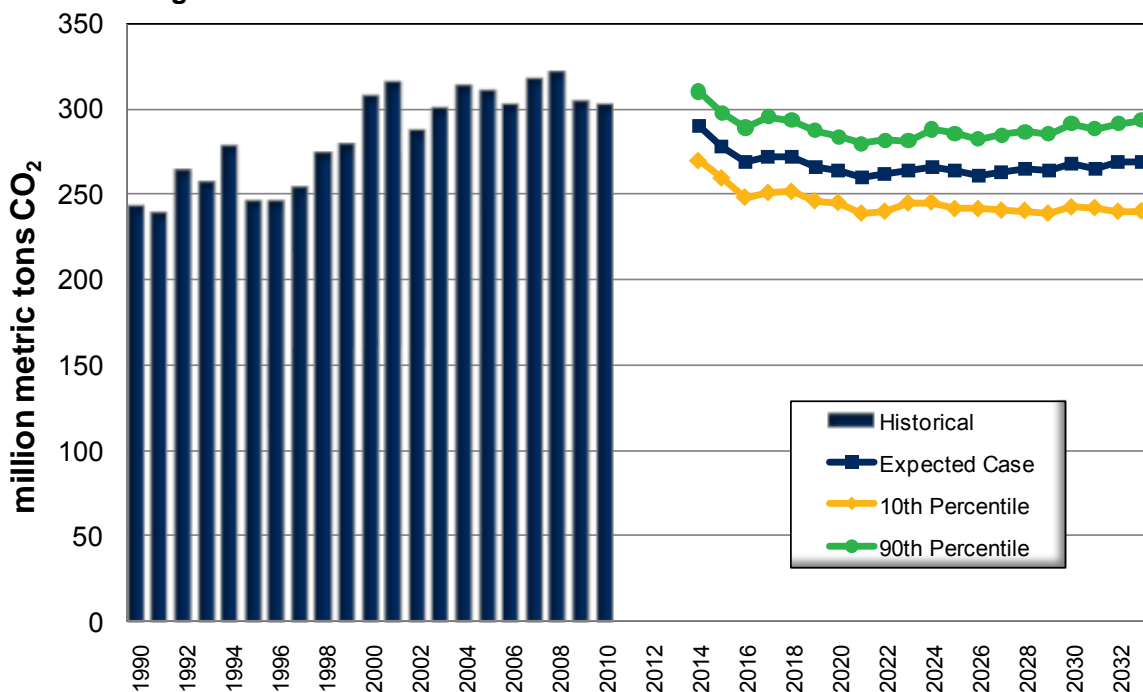
Figure 10: U.S. Western Interconnect Greenhouse Gas Emissions
