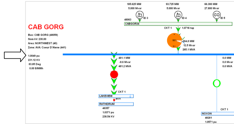
Figure 3: 2016 HT, Voltage Limit Violation, N-1: Cabinet – Noxon 230 kV
