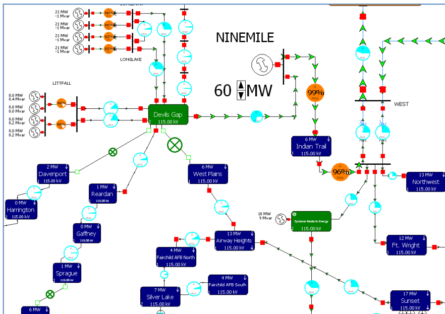
Figure 2. Limiting Contingency: N-1: Airway Heights - Devis Gap 115 kV Open @ DGP
