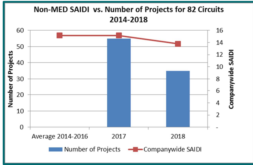
Figure 6: SAIDI Results and Projects Completed on 82 Circuits with Targeted Reliability Improvements
