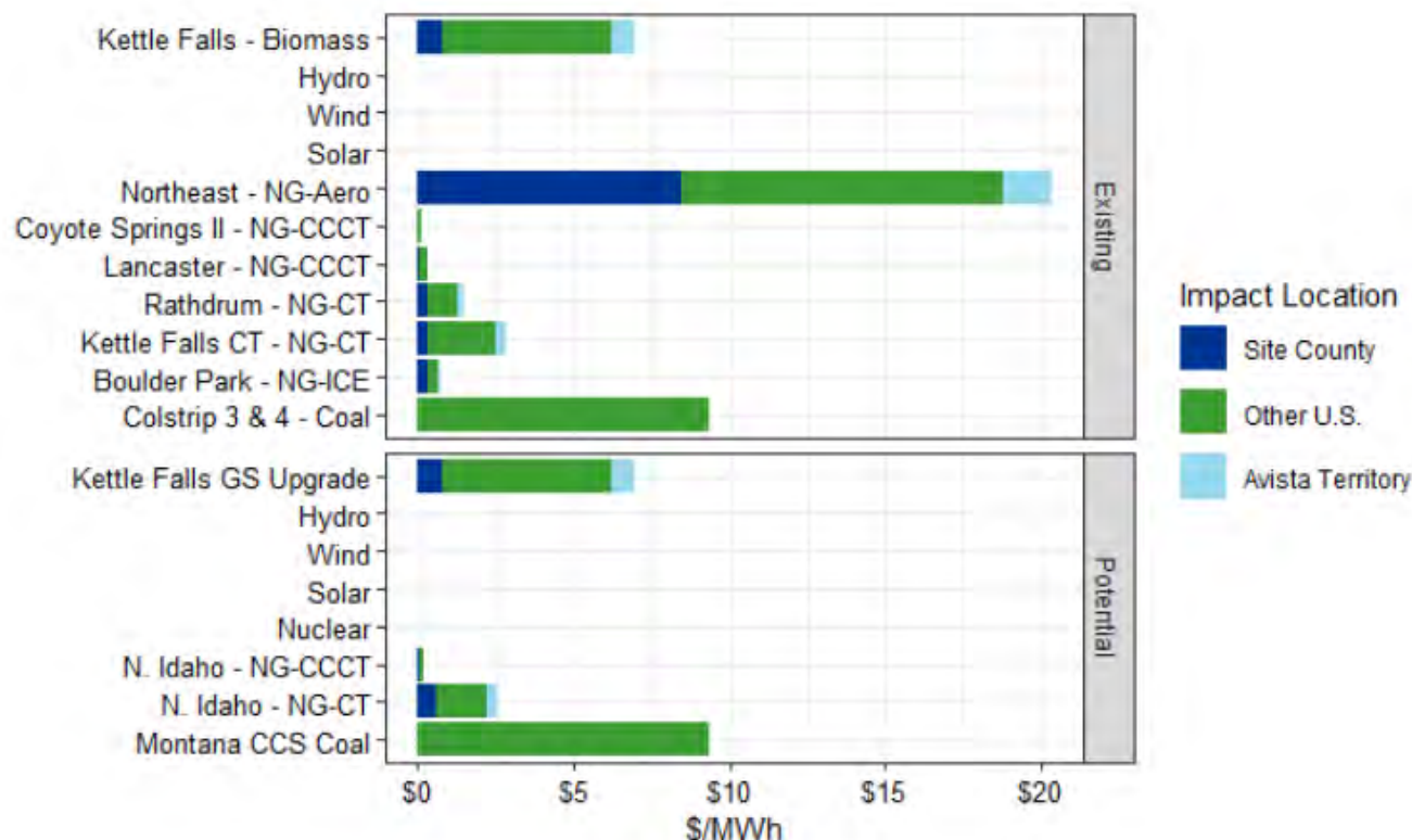
Figure 3-6. Operational NO x health costs per MWh by generation type
