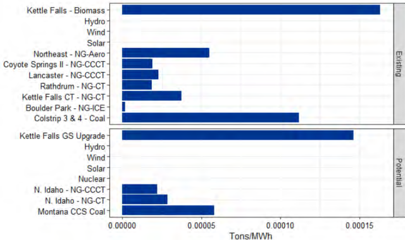
Figure 3-2. Operational SO 2 emissions per MWh by generation type
