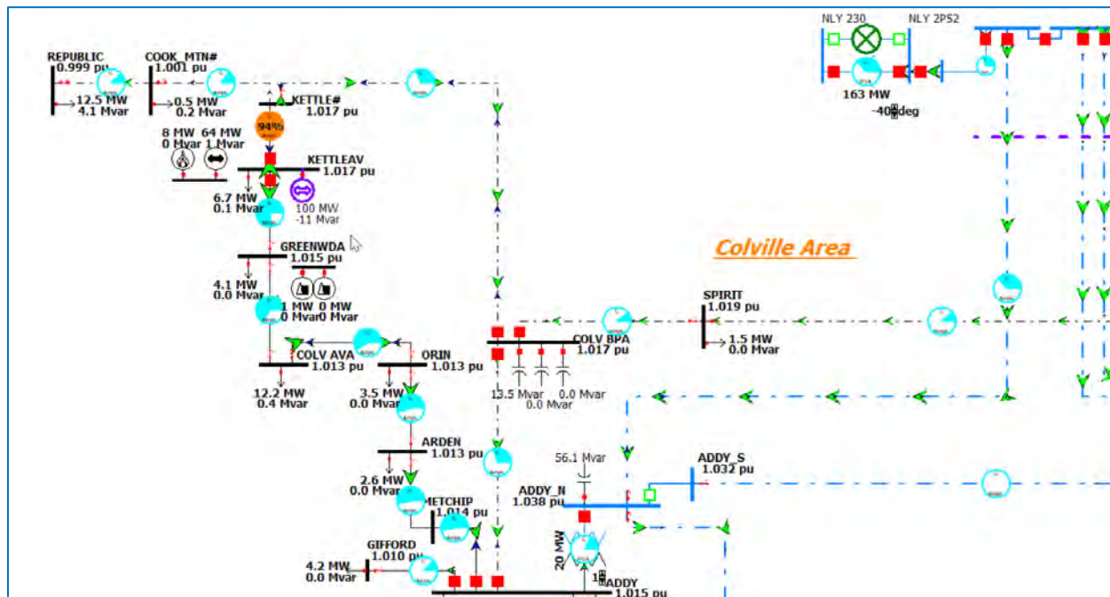
Figure 14: Proposed Generation at Kettle Falls, 2027 Heavy Spring
