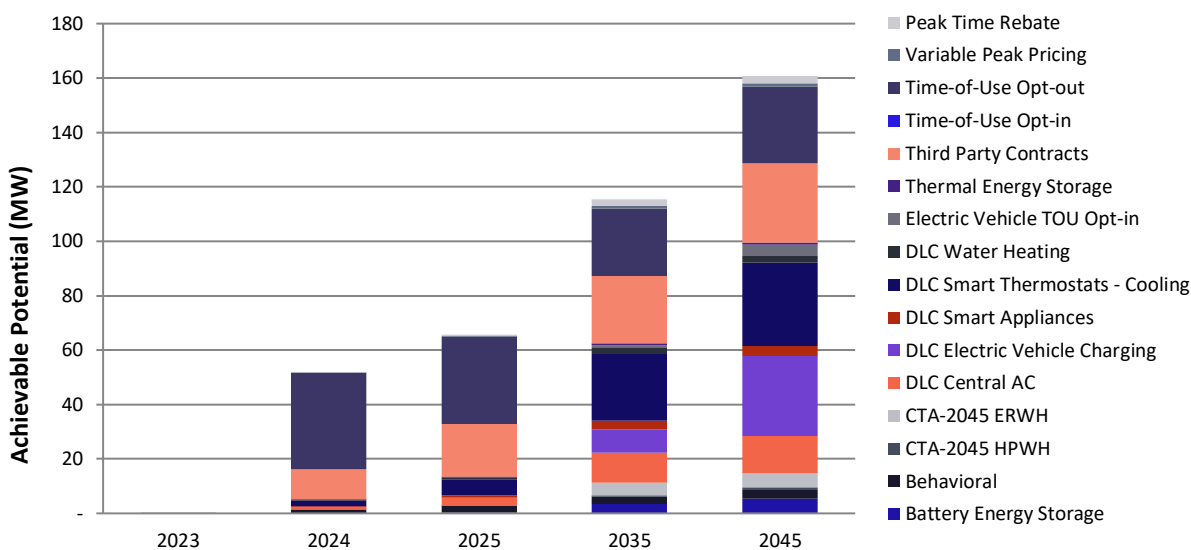
Figure D-1 Summary of Summer Potential by Option – TOU Opt-Out (MW @Generator)
