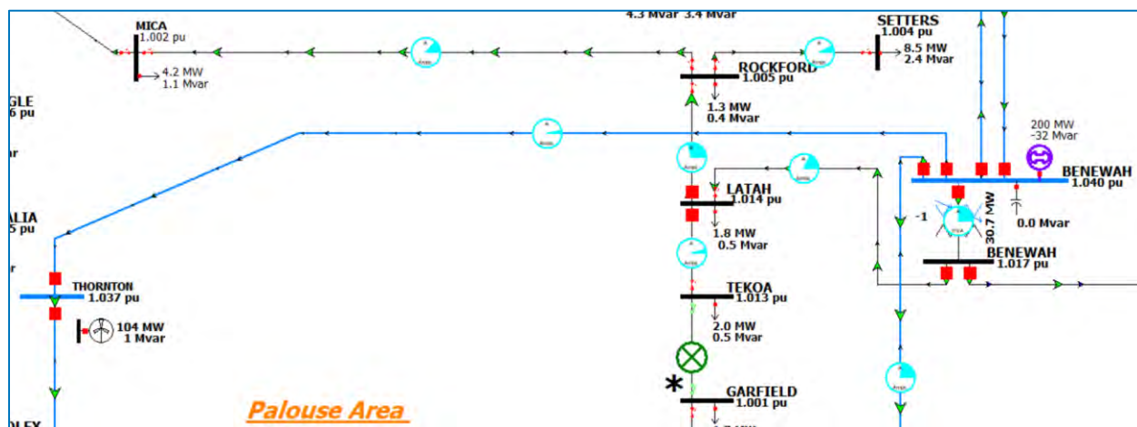
Figure 20: Proposed Generation at Benewah 230kV, 2027 Heavy Summer
