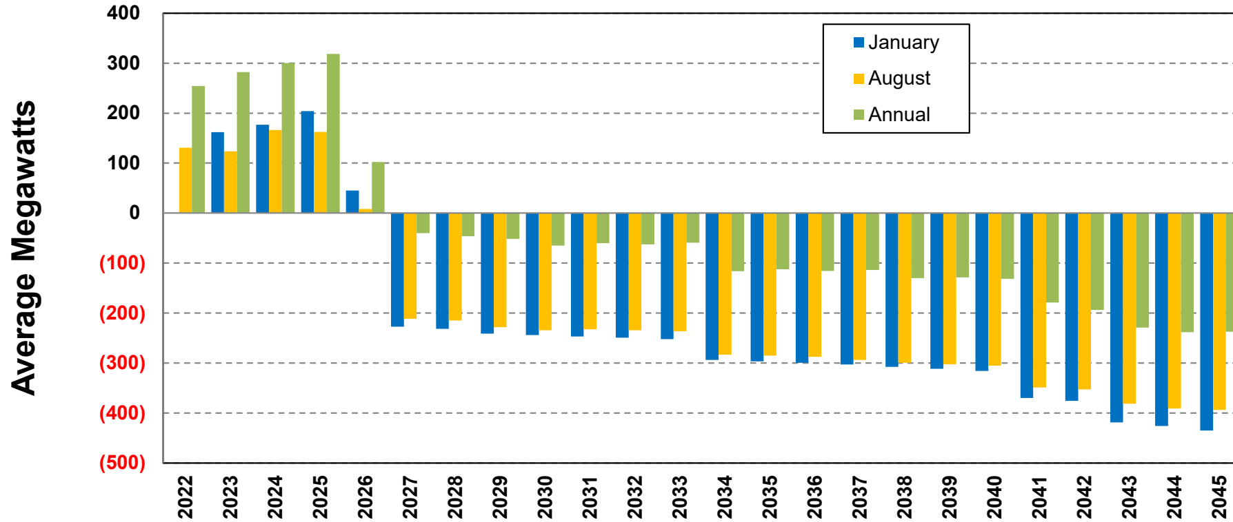
Energy Load & Resource Position
