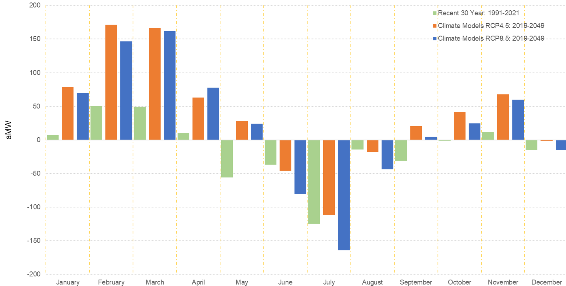
Impact of Climate Change Forecasted River Flows on Monthly Median Avista Hydro Generation
