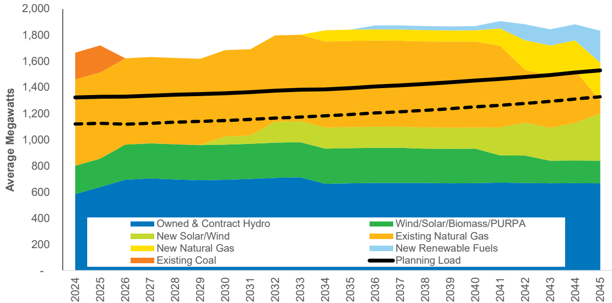
Figure 9.7: System Annual Energy Load &amp; Resources
