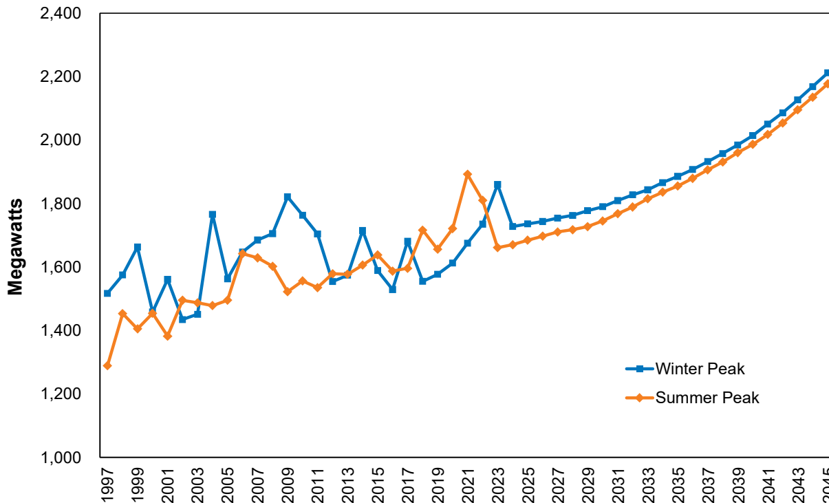
Figure 2.17: Peak Load Forecast
