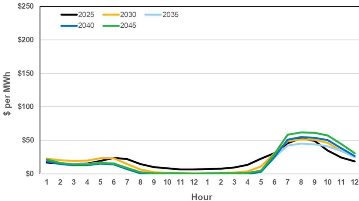
Figure 8.18: Spring Average Hourly Electric Prices (March - June)
