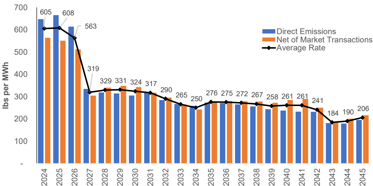
Figure 9.11: System Greenhouse Gas Emissions Intensity
