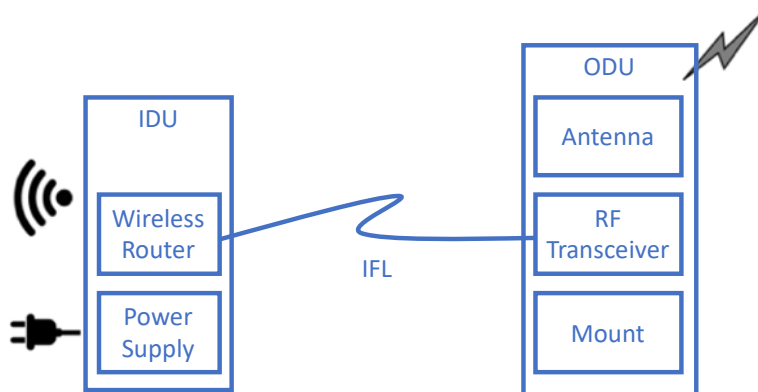
Figure 2: Viasat User Terminals
