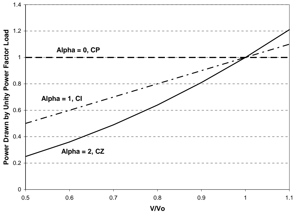
Figure 2.1: Power Versus Voltage Curve for Different Load Characteristics
