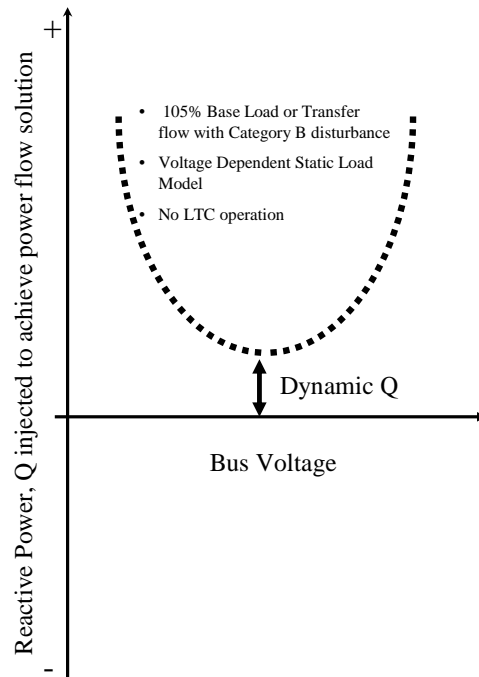
Figure 2.5: Determination of the dynamic reactive power resource requirement.
