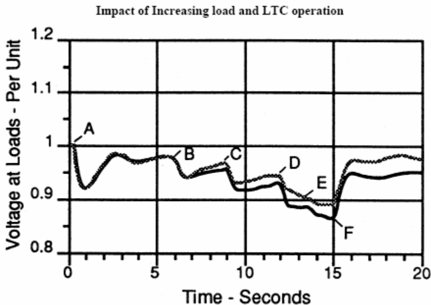
Figure 4-7 Voltage at loads: Gray curve is for industrial load, black curve for residential load. Trip one 500 kV line at Point A. Resistive load added at the residential load bus: 200 MW at points B, C, and D; 100 MW at Point E. At Point F, trip 5% of total load by UVLS with voltage setpoint at 0.9 pu and 1.5 second time delay.
