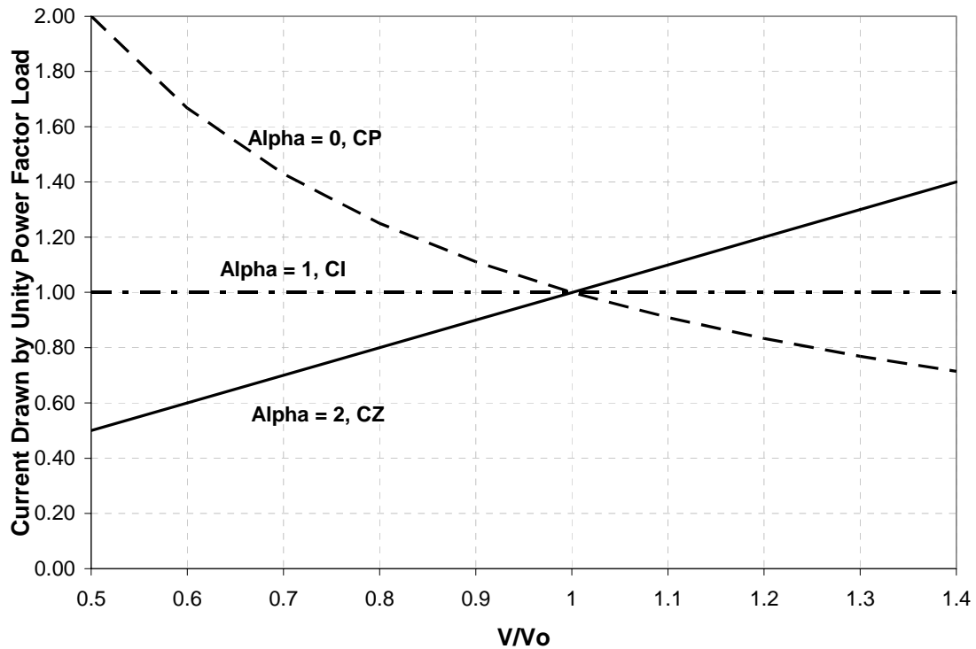
Figure 2.0: Current Versus Voltage Curve for Different Load Characteristics
