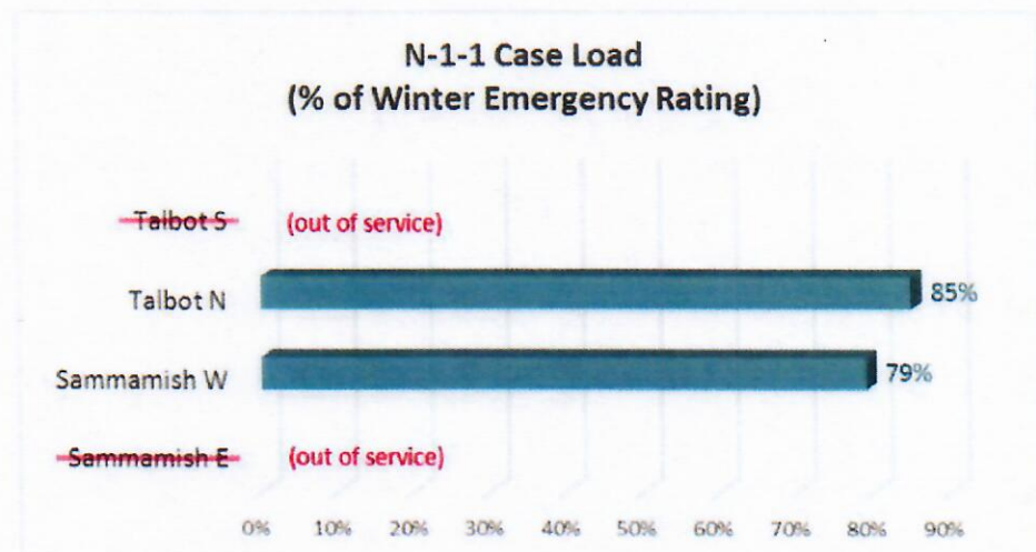
Figure 2: Loads on two remaining transformers are in a safe range.
