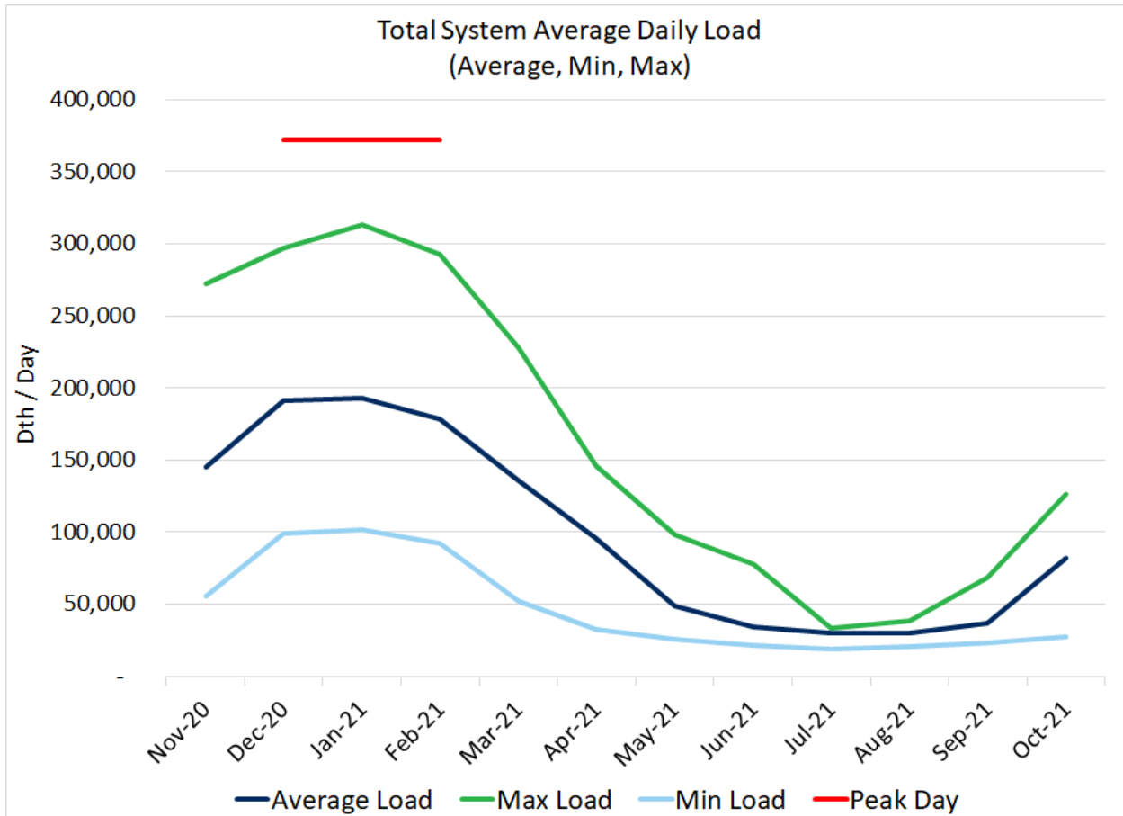
Figure 6.2: Total System Average Daily Load (Average, Minimum and Maximum)
