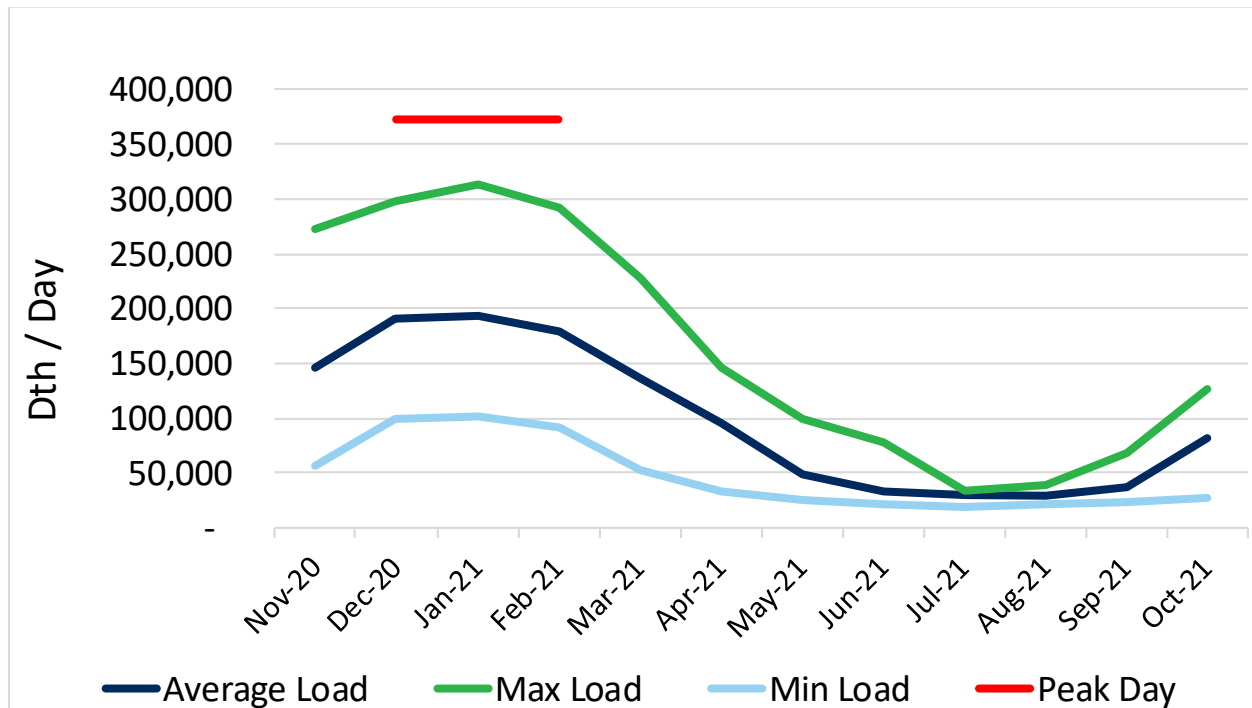
Figure 1.5: Total System Average Daily Load
