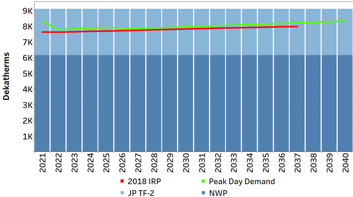
Figure 8: Expected Case – La Grande Existing Resources vs. Peak Day Demand (Net of DSM)
