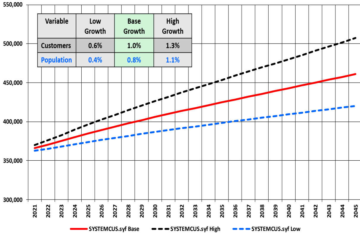
Figure 2.1: Customer Growth Scenarios
