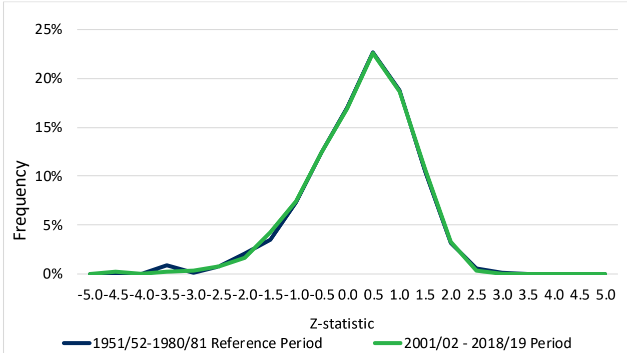
Figure 2.7: Klamath Falls
