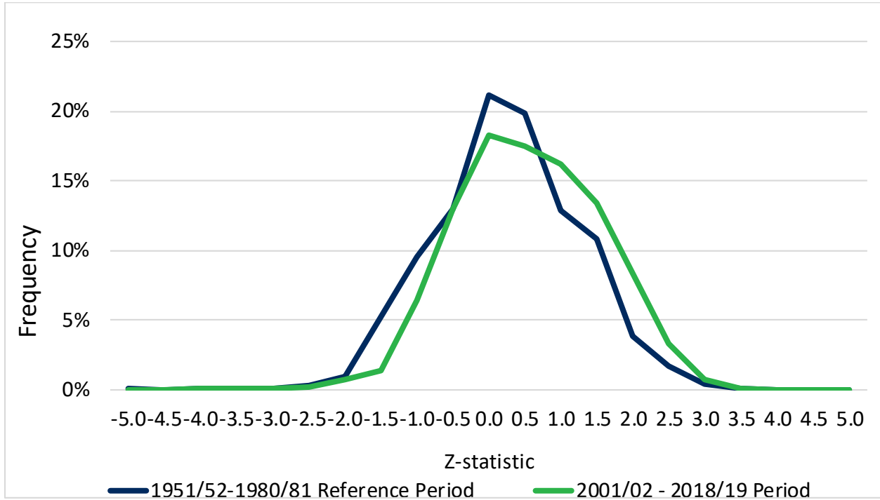
Figure 2.5: Medford
