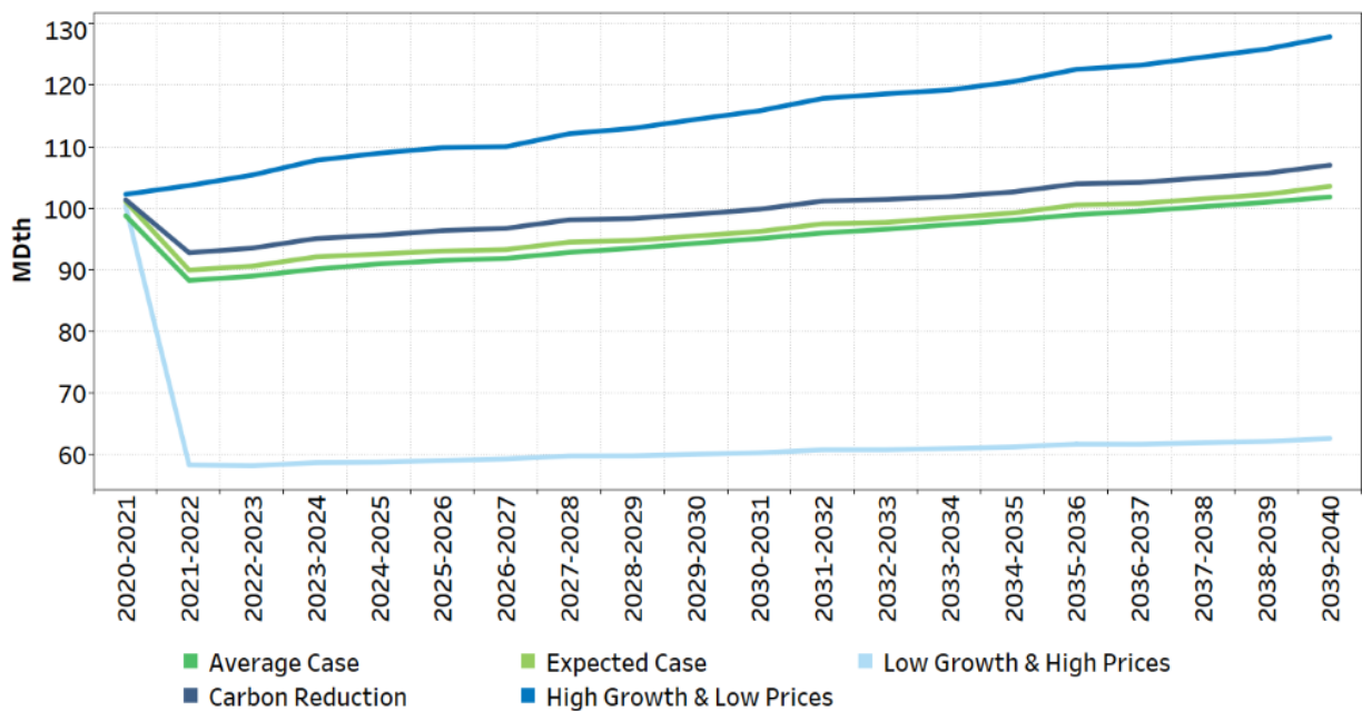
Figure 2.13: Average Daily Demand – 2021 IRP Scenarios
