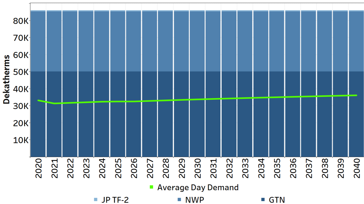
Figure 6.11: Average Case – Medford / Roseburg Existing Resources vs. Peak Day Demand – December 20 th
