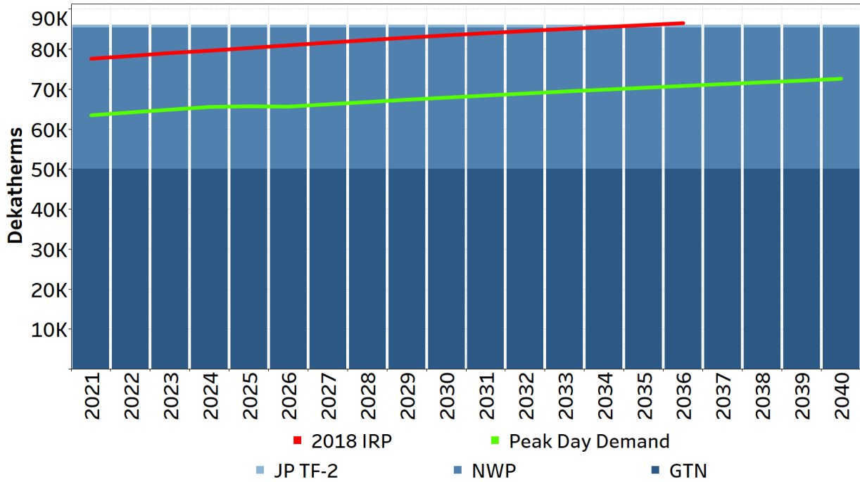
Figure 6: Expected Case – Medford/Roseburg Existing Resources vs. Peak Day Demand (Net of DSM)
