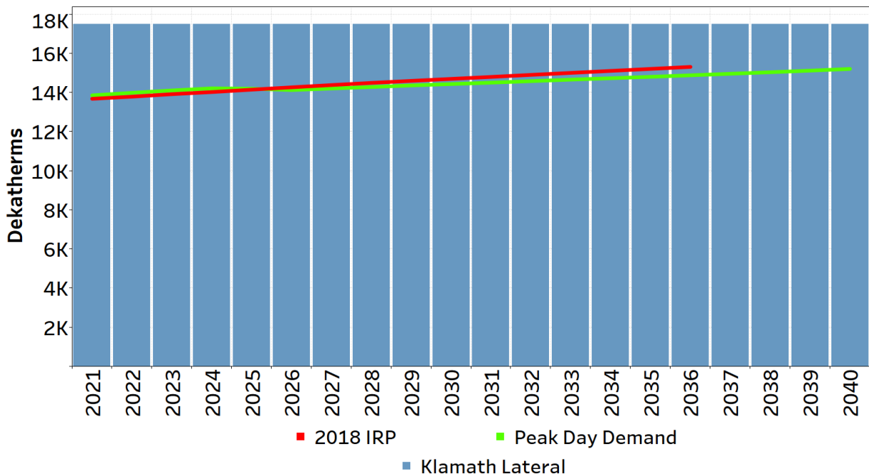
Figure 7: Expected Case – Klamath Falls Existing Resources vs. Peak Day Demand (Net of DSM)
