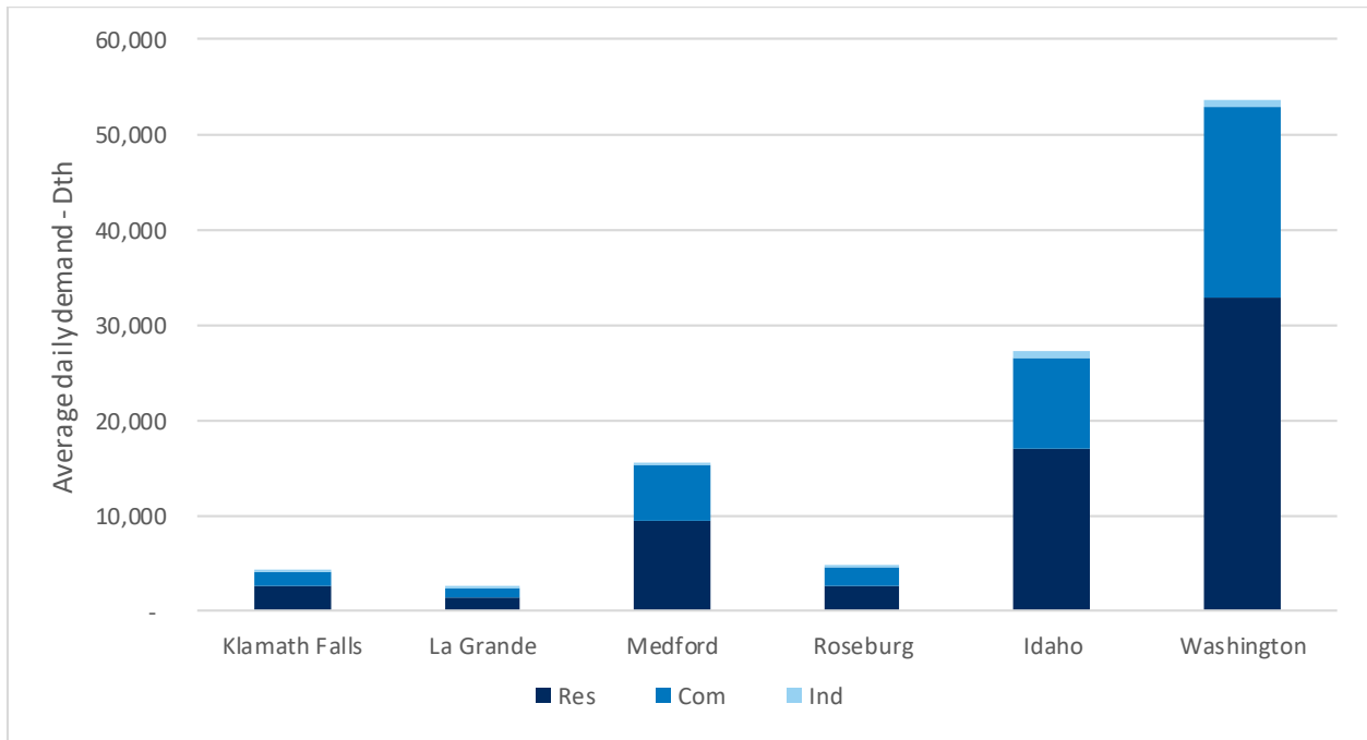
Figure 1.4 2019 daily demand by area and class
