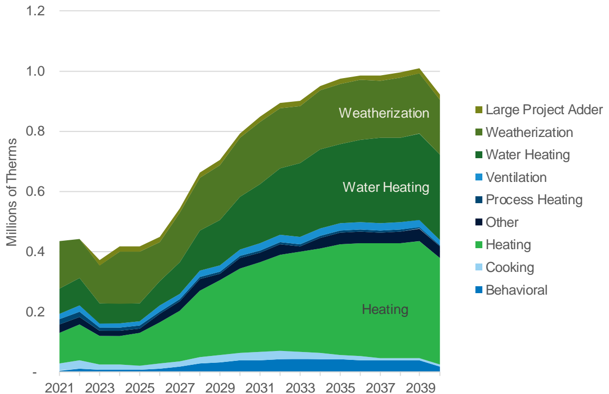
Figure 9 – Annual Deployed Final Savings Potential by End Use
