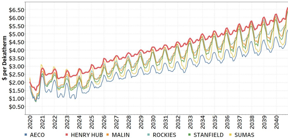
Figure 6.6: Regional Price as a compared to the Henry Hub Price
