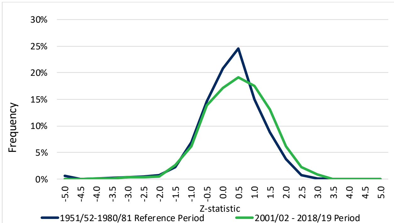
Figure 2.8: Roseburg
