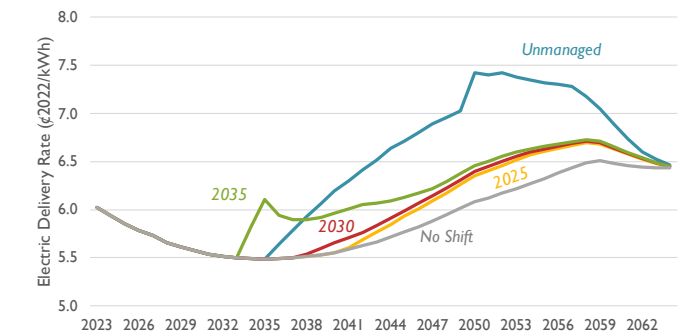
Figure 21. Electric delivery rate across the four transition management scenarios, if net income and depreciation costs can be shifted to the electric utility
