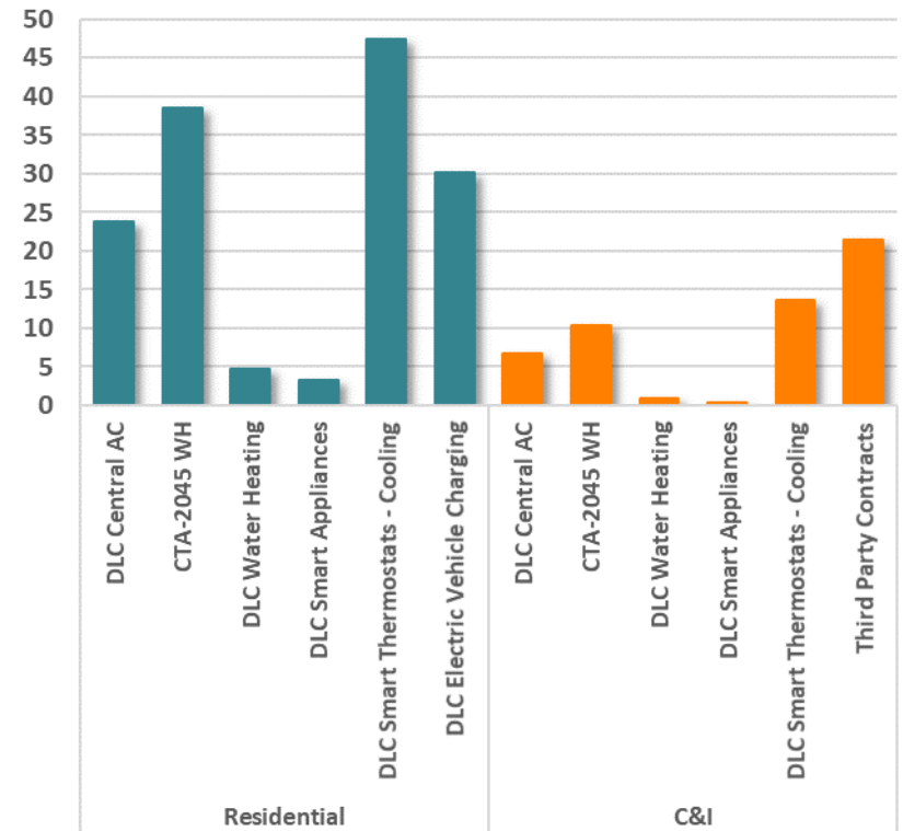
2045 Summer Potential (MW) - DLC Options
