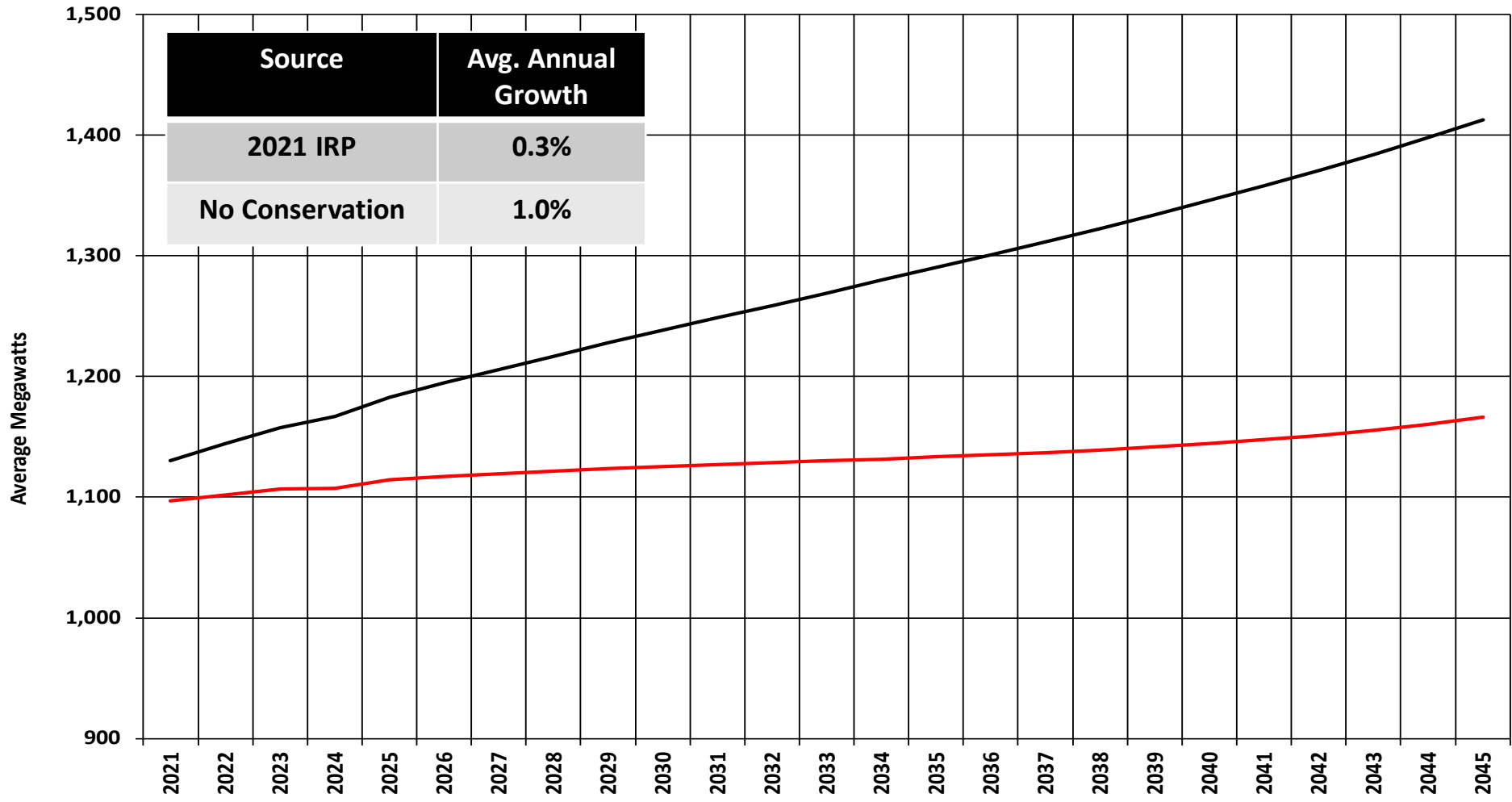
Average Megawatts Load Comparison with Conservation Adjustment
