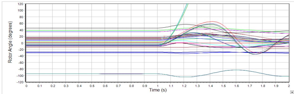
FIGURE 4: NINE MILE GENERATION OOS.
