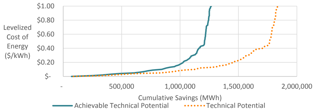
UCT Conservation Supply Curve, 2031
