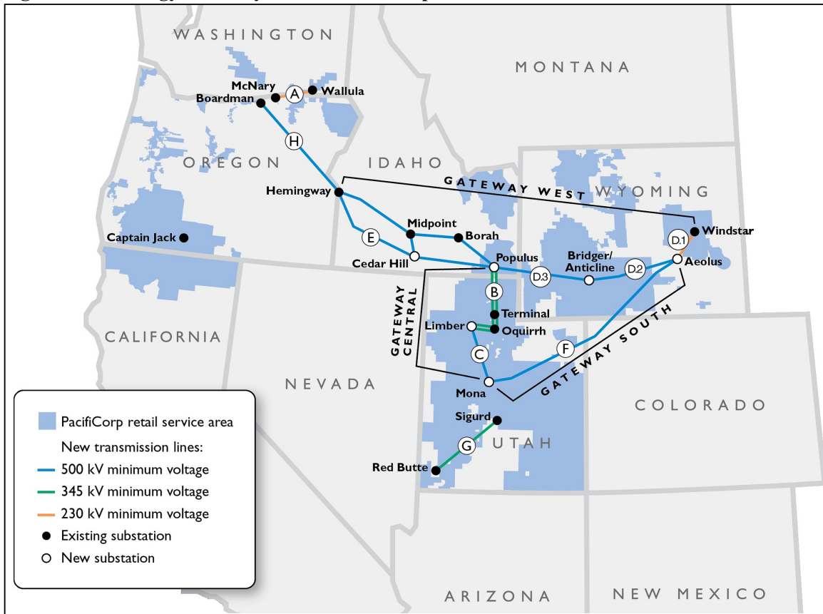
Figure 4.3 – Energy Gateway Transmission Expansion Plan
