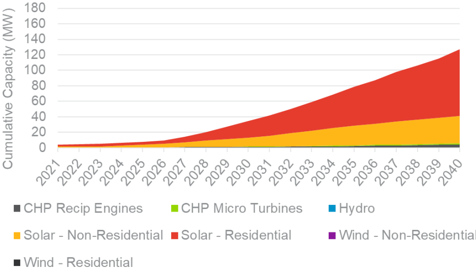
Figure 17. Cumulative Capacity Installations by Technology (MW AC), Idaho Base Case
