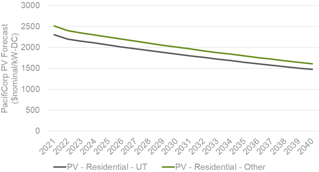
Figure 10 Residential Solar System Costs, 2021-2040
