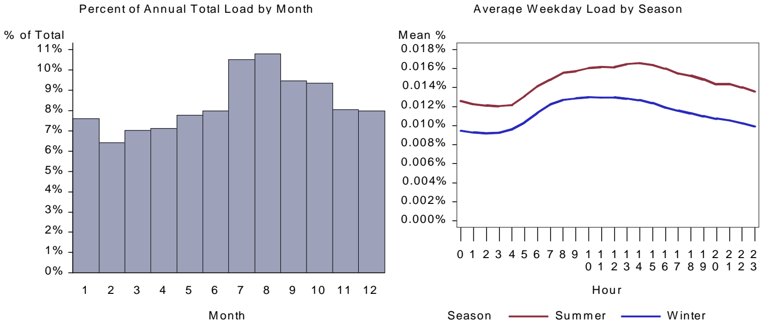
Figure 261. : WY Grocery Refrigeration Load by Month and Average Weekday
