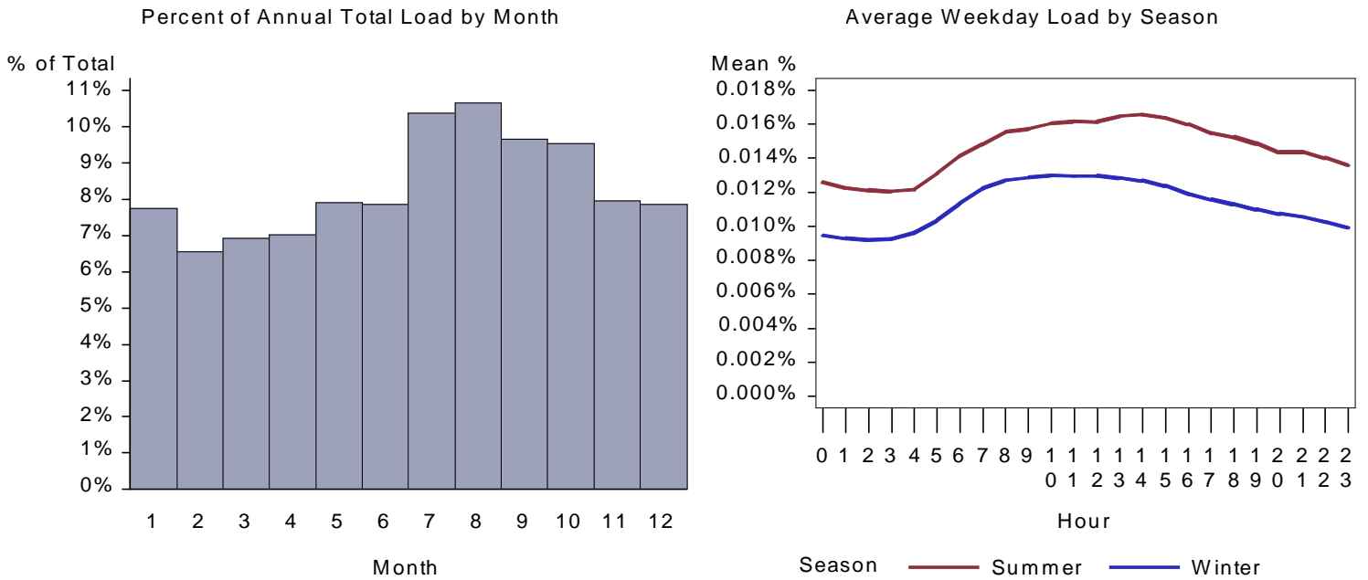
Figure 302. : UT Warehouse Refrigeration Load by Month and Average Weekday
