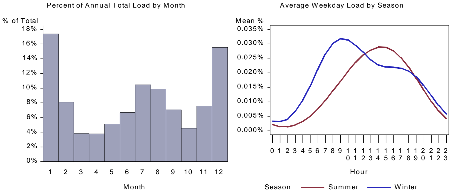
Figure 67. CA Large Retail HVAC Aux Load by Month and Average Weekday
