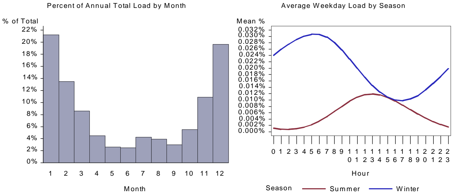
Figure 136. : CA School Heat Pump Load by Month and Average Weekday
