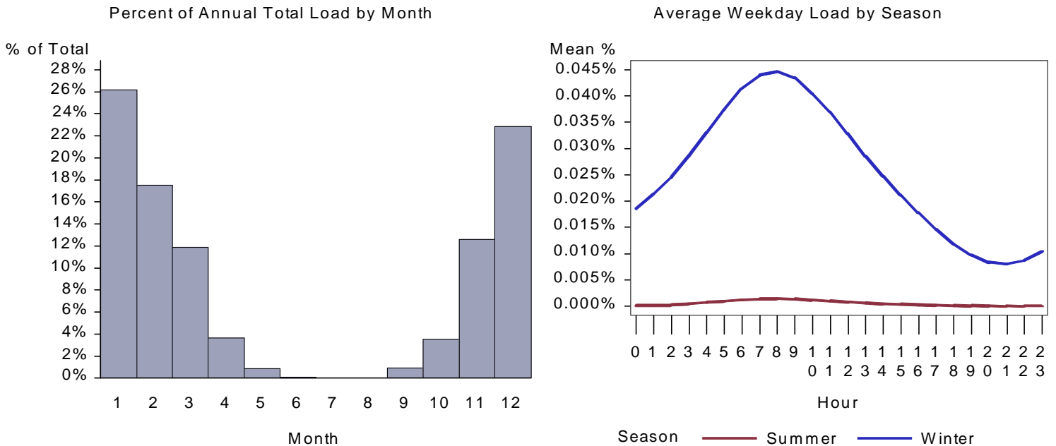
Figure 376. : WY Large Office Space Heat Load by Month and Average Weekday
