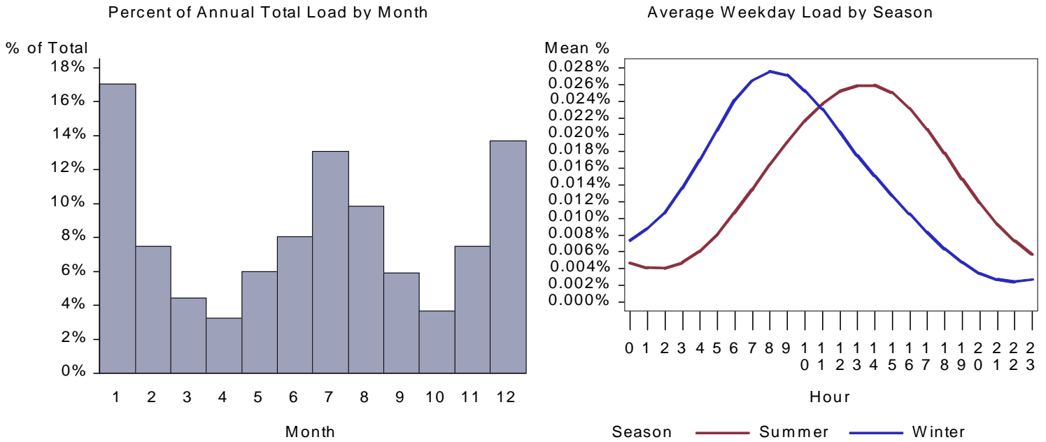
Figure 95. WA Small Office HVAC Aux Load by Month and Average Weekday
