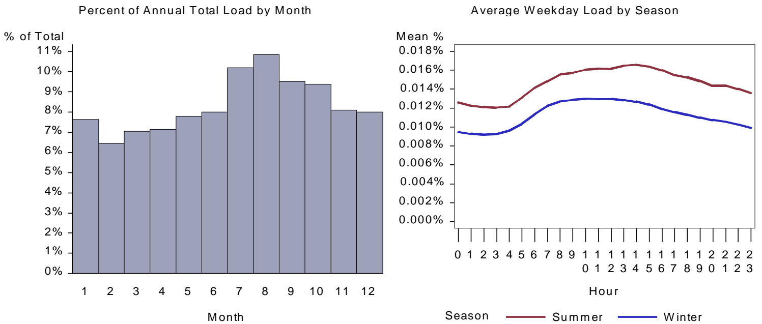
Figure 280. : CA Restaurant Refrigeration Load by Month and Average Weekday
