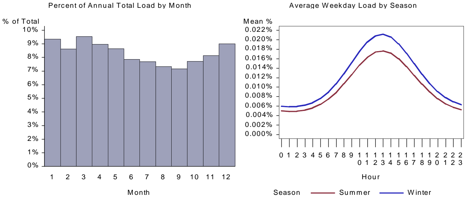
Figure 421. : WA Grocery Water Heat Load by Month and Average Weekday
