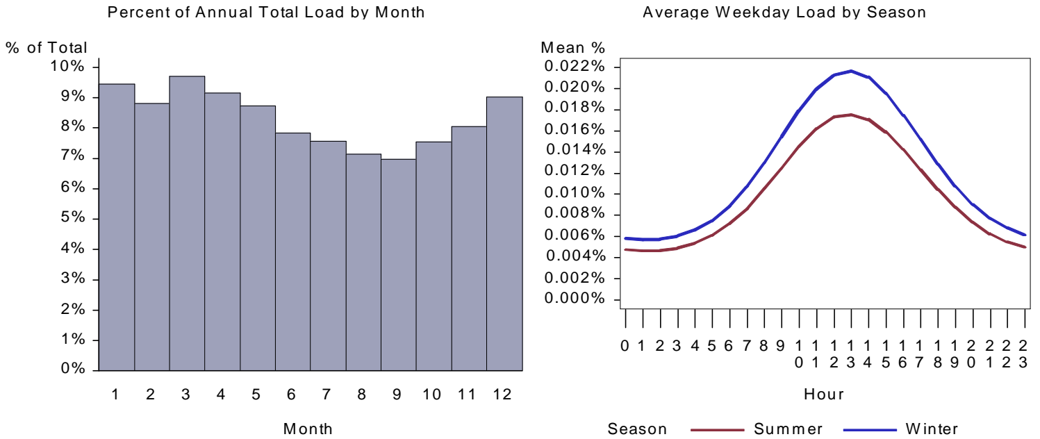
Figure 3. UT Grocery Cooking Load by Month and Average Weekday
