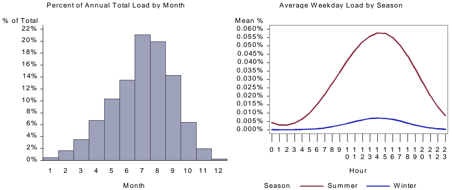
Figure 351. : CA Small Retail Space Cool Load by Month and Average Weekday
