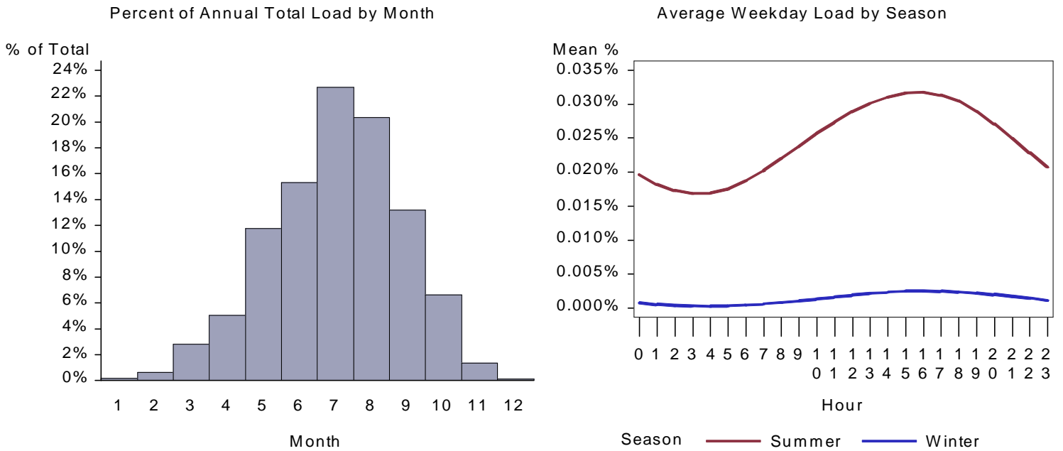
Figure 328. : UT Lodging Space Cool Load by Month and Average Weekday
