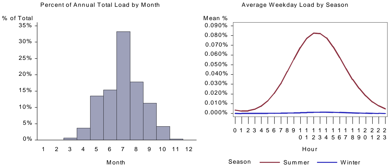
Figure 342. : ID School Space Cool Load by Month and Average Weekday
