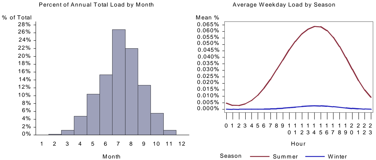
Figure 322. : ID Large Retail Space Cool Load by Month and Average Weekday
