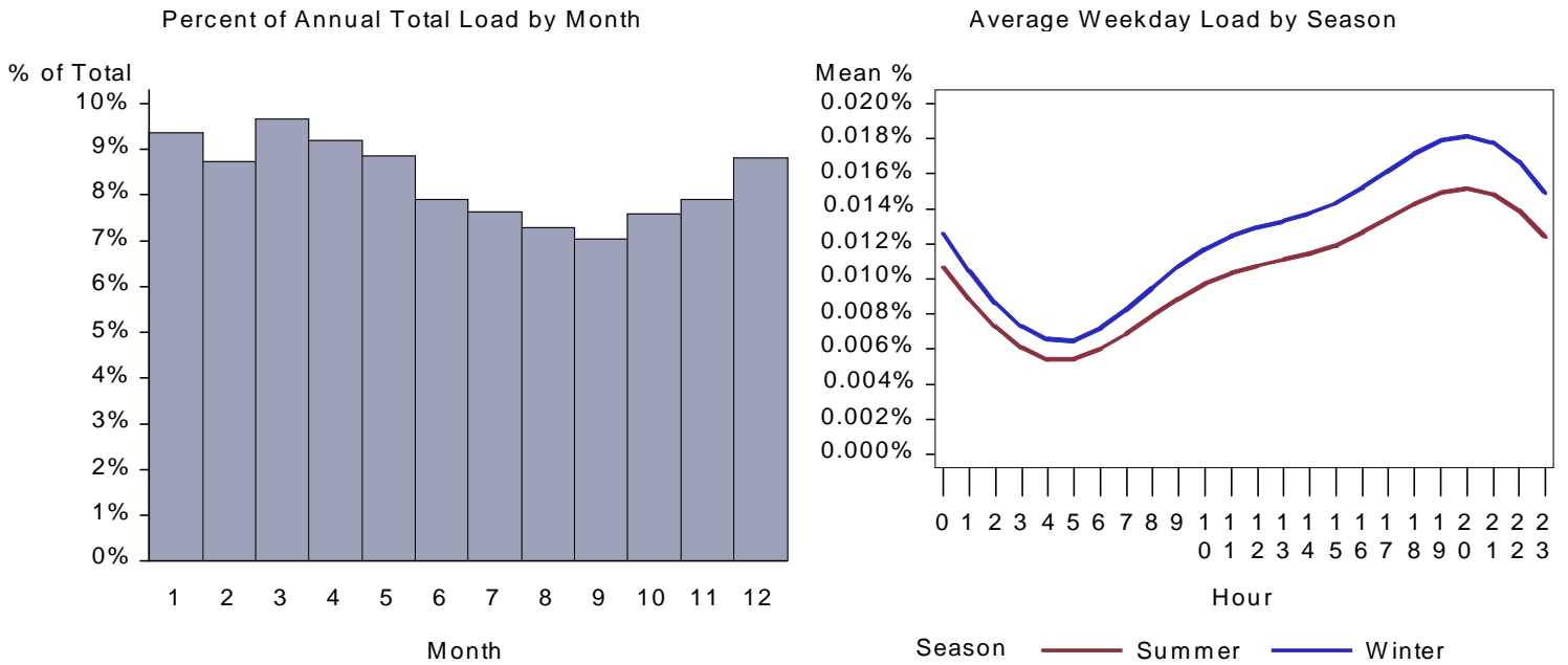
Figure 452. : WY Restaurant Water Heat Load by Month and Average Weekday
