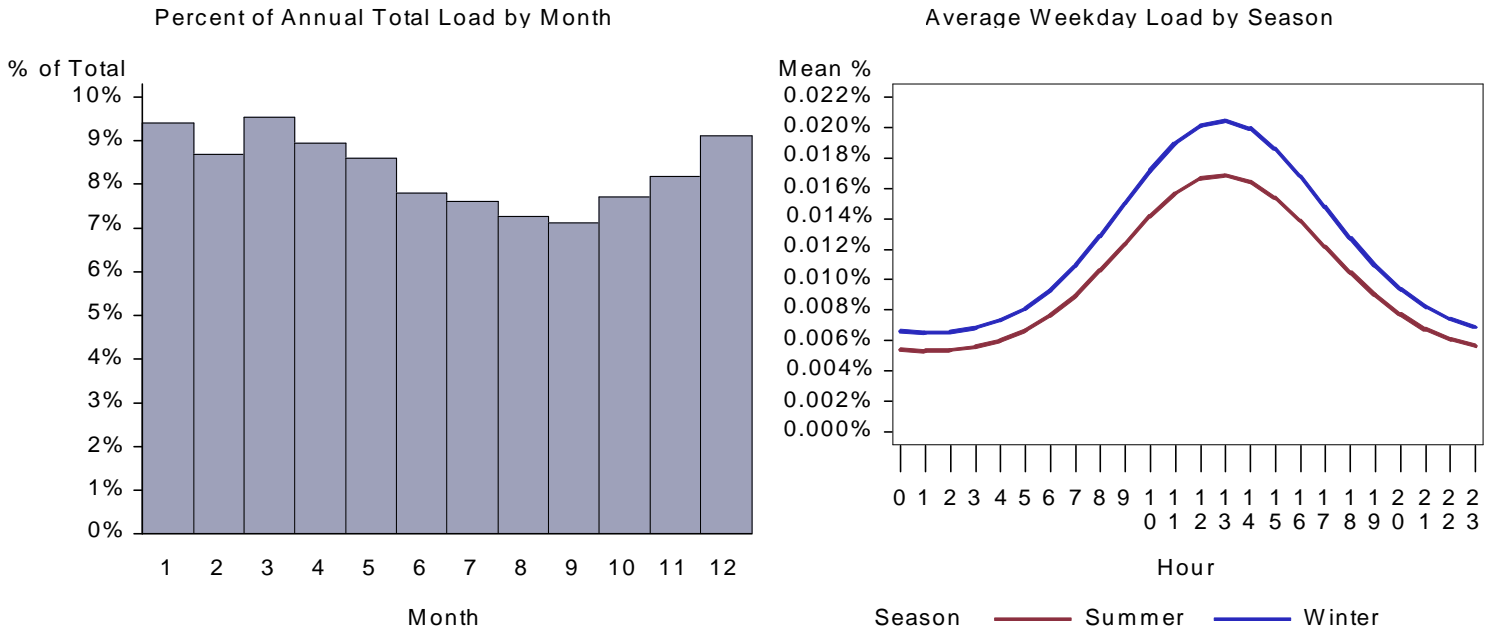
Figure 419. : ID Grocery Water Heat Load by Month and Average Weekday
