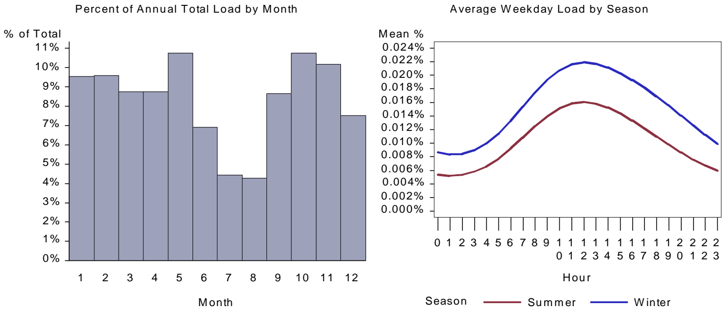
Figure 184. : UT School Lighting Load by Month and Average Weekday
