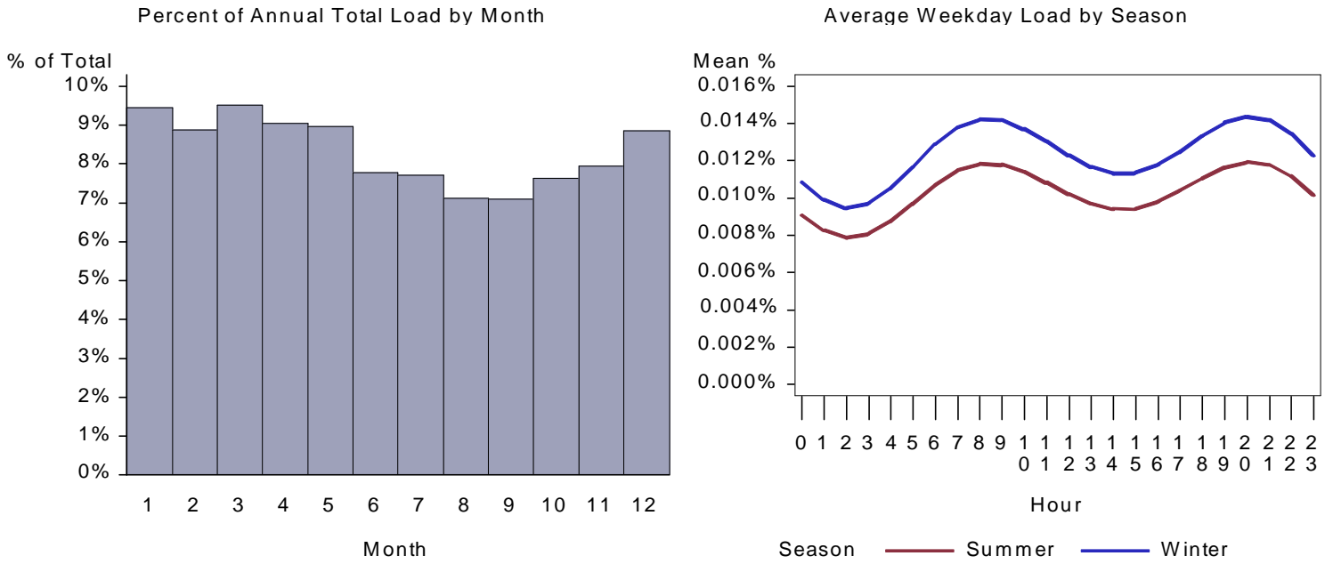
Figure 439. : ID Lodging Water Heat Load by Month and Average Weekday
