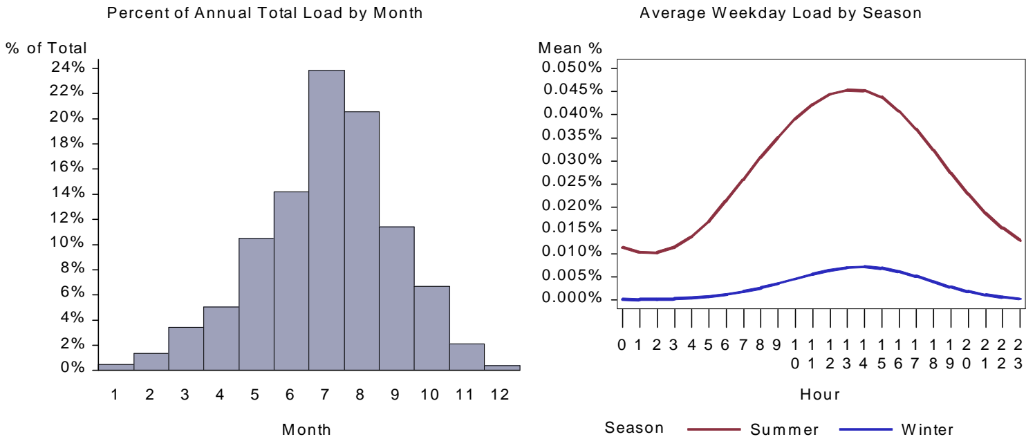
Figure 318. : UT Large Office Space Cool Load by Month and Average Weekday
