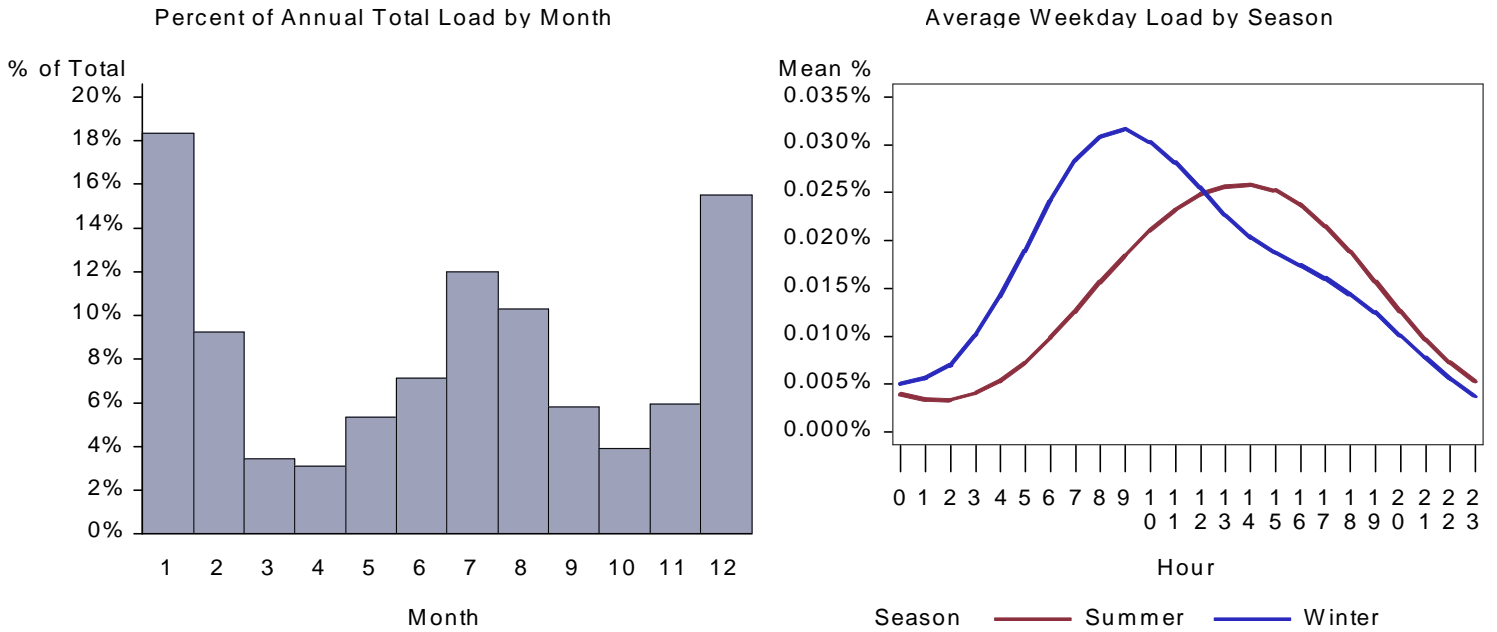
Figure 79. UT Miscellaneous HVAC Aux Load by Month and Average Weekday
