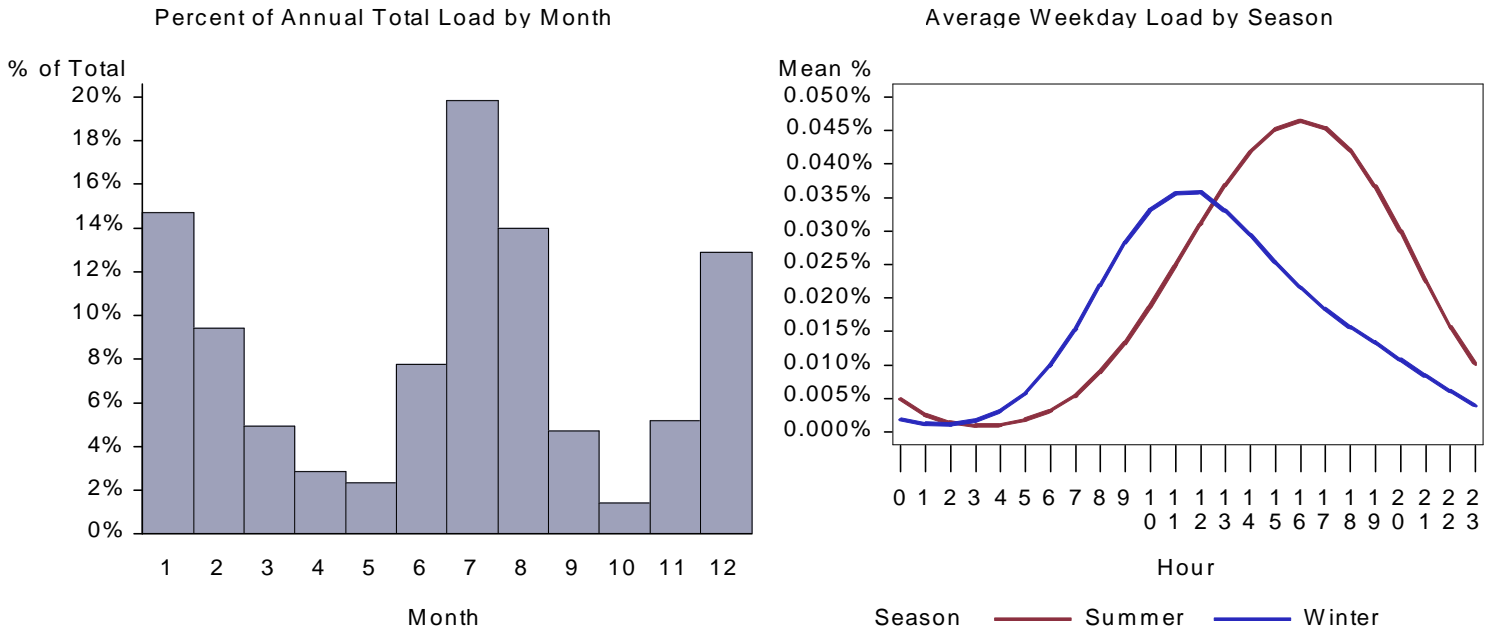
Figure 103. : ID Warehouse HVAC Aux Load by Month and Average Weekday
