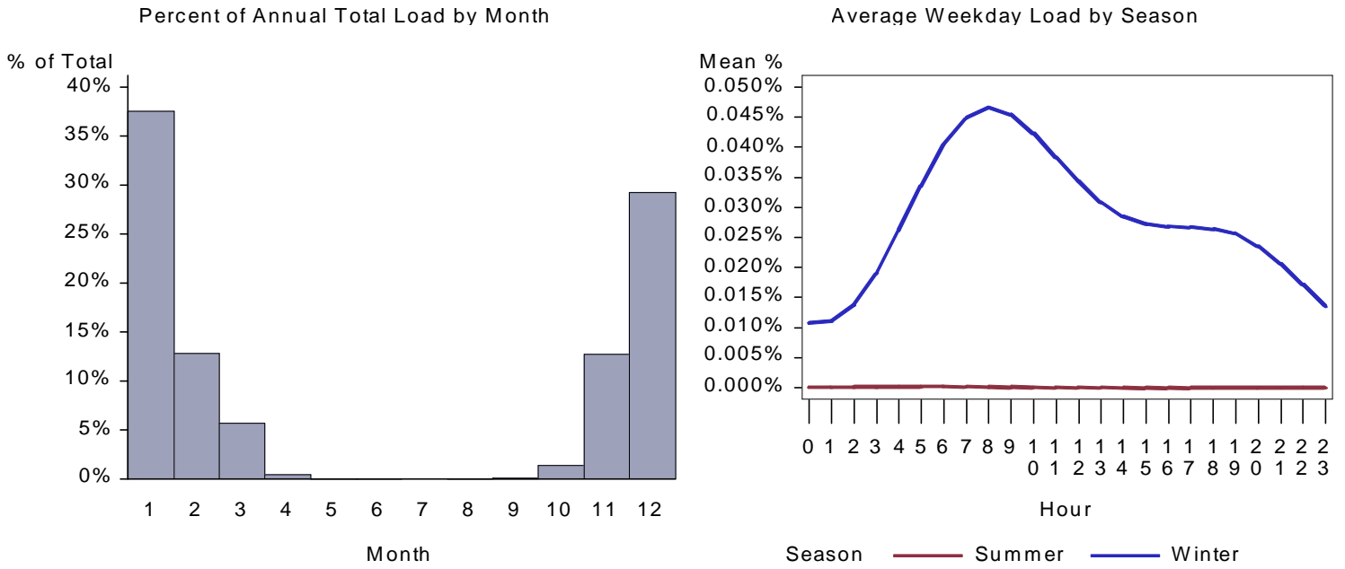
Figure 365. : WA Grocery Space Heat Load by Month and Average Weekday
