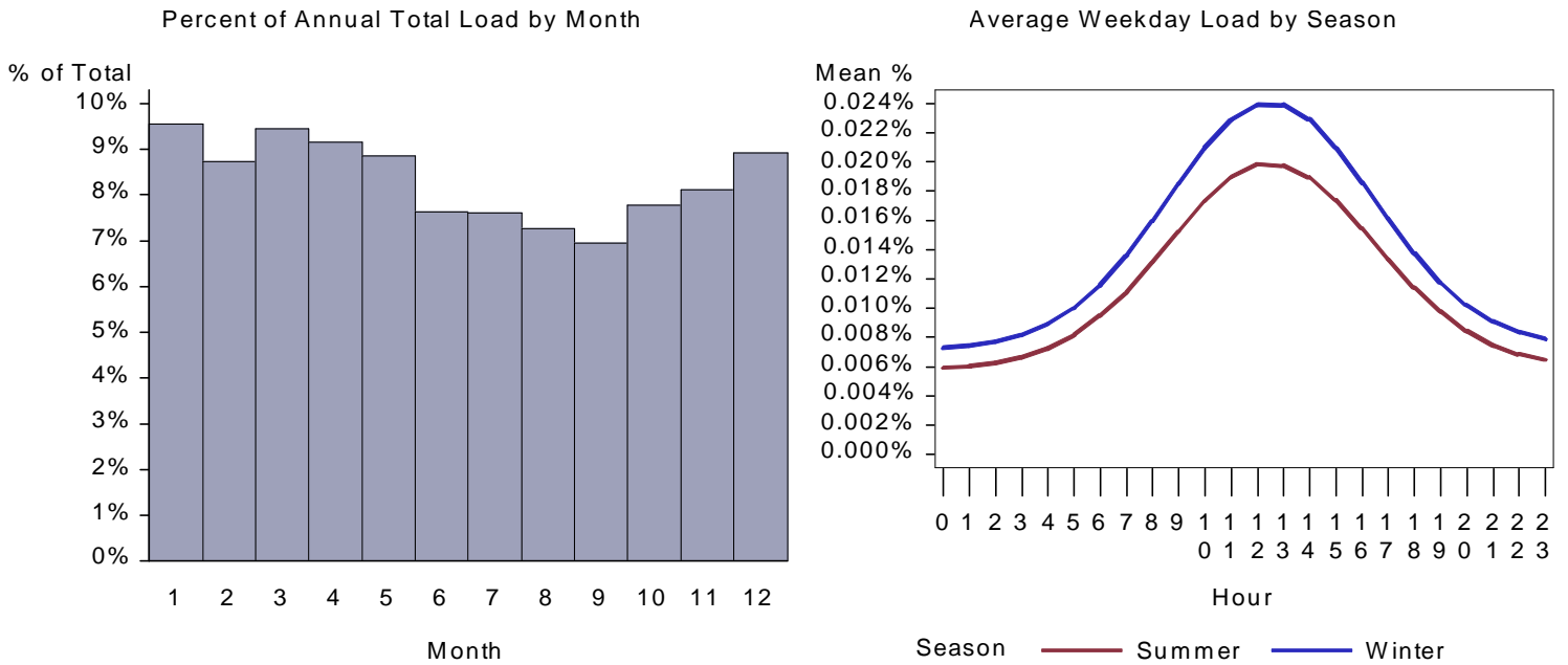
Figure 20. WY Large Retail Cooking Load by Month and Average Weekday
