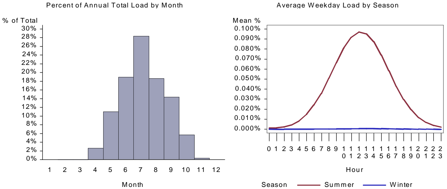
Figure 345. : WY School Space Cool Load by Month and Average Weekday
