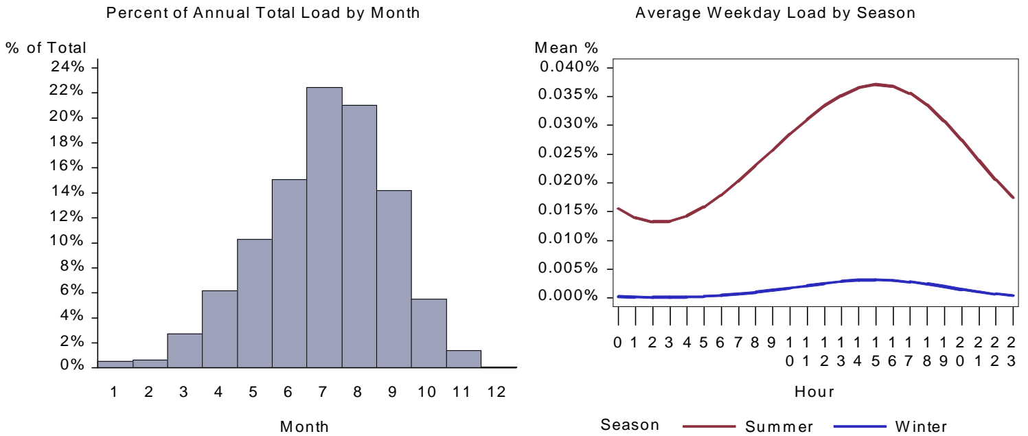
Figure 306. : CA Grocery Space Cool Load by Month and Average Weekday
