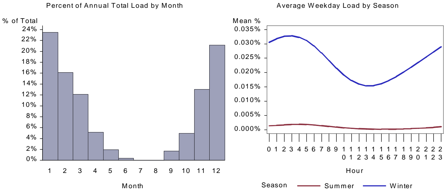
Figure 386. : WY Lodging Space Heat Load by Month and Average Weekday
