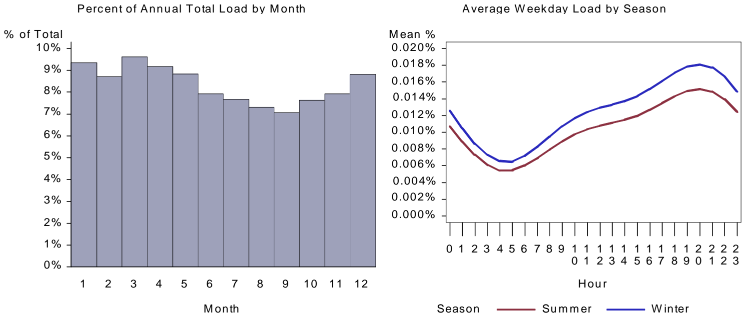
Figure 29. WA Restaurant Cooking Load by Month and Average Weekday
