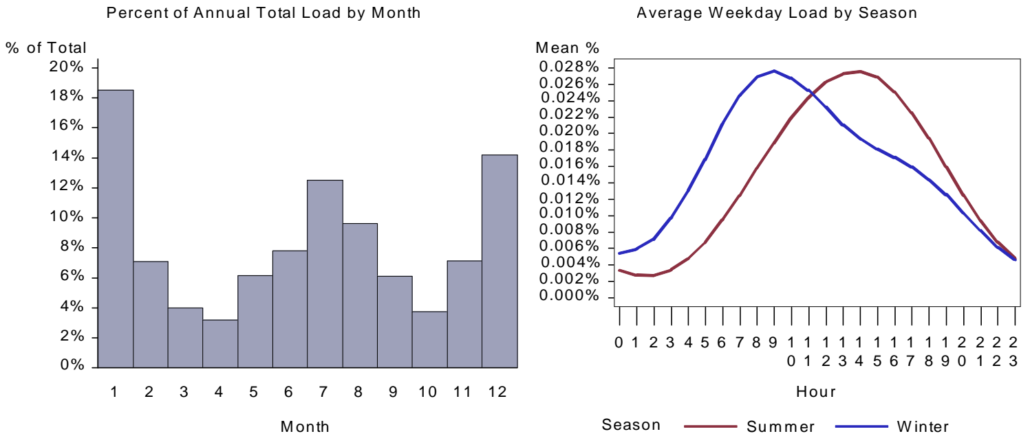
Figure 80. WA Miscellaneous HVAC Aux Load by Month and Average Weekday
