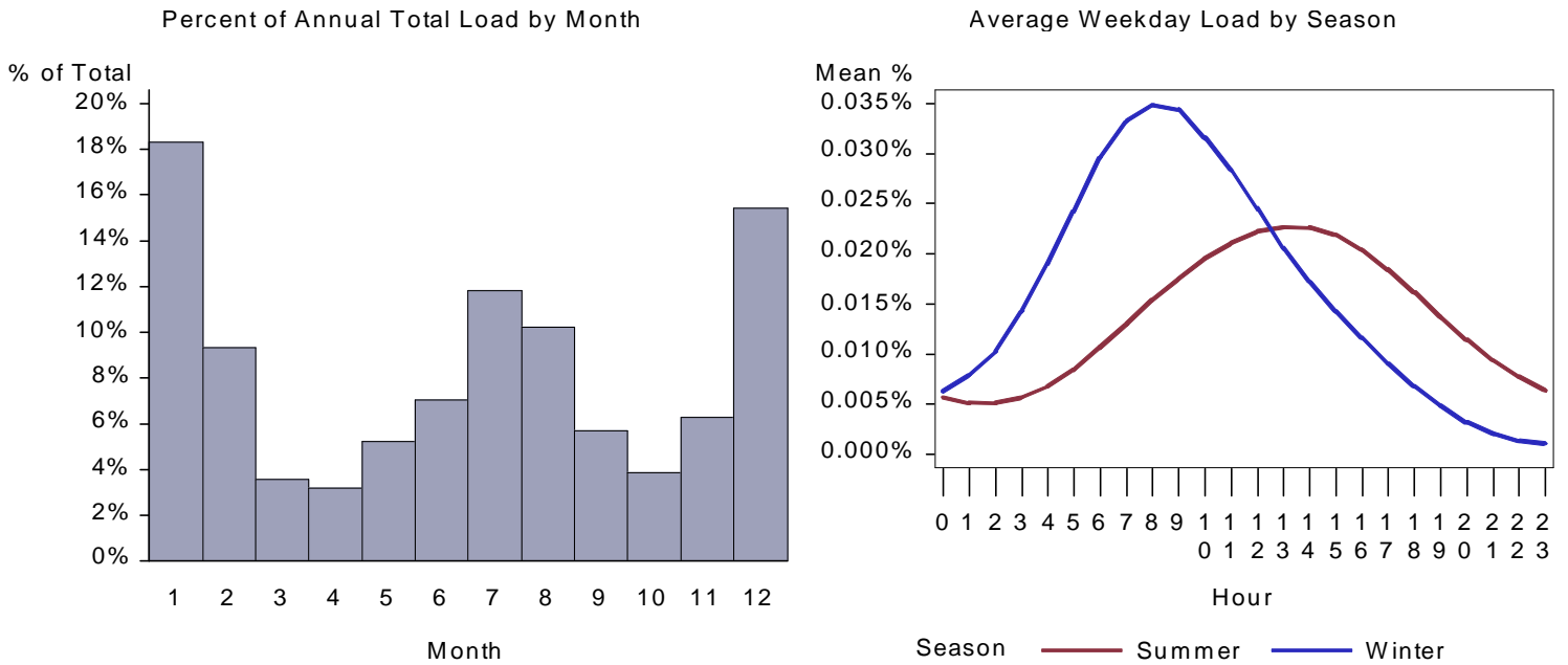
Figure 94. UT Small Office HVAC Aux Load by Month and Average Weekday
