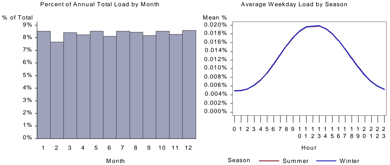
Figure 166. : WY Large Retail Lighting Load by Month and Average Weekday
