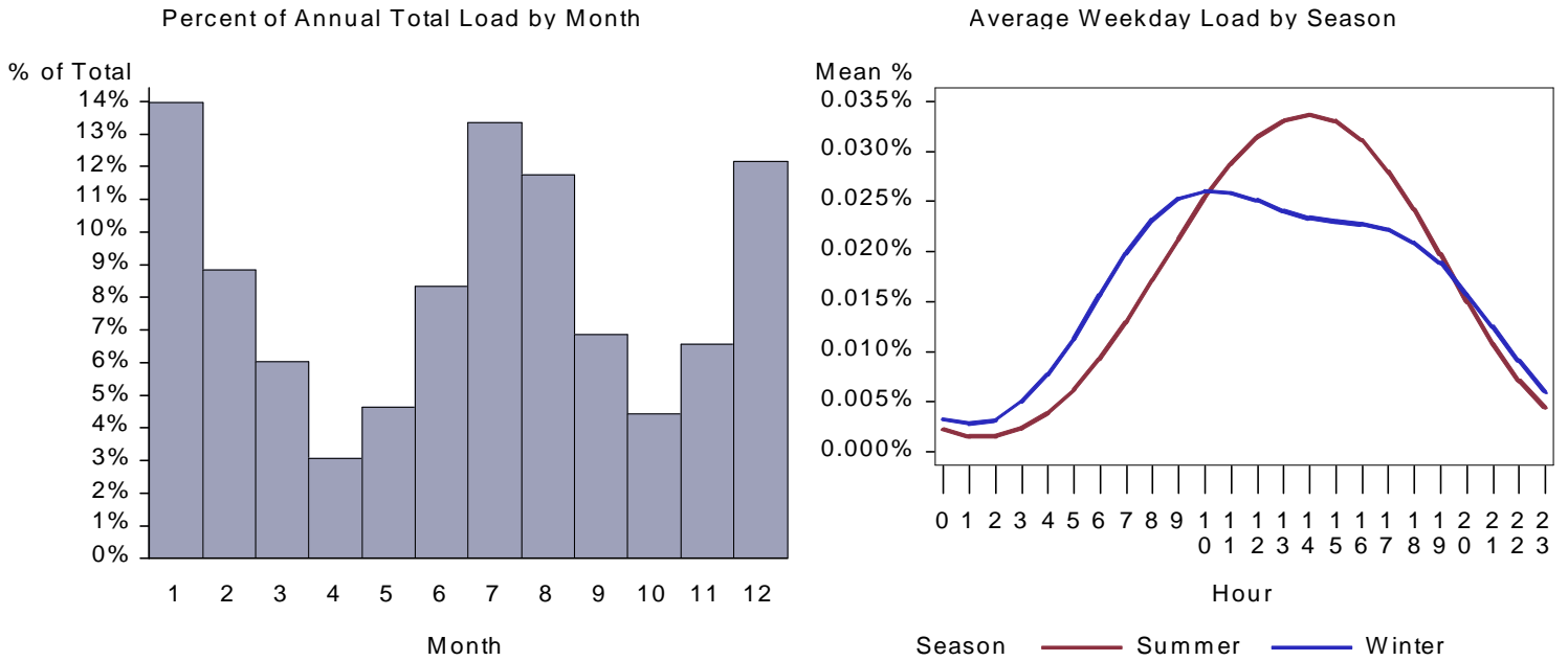
Figure 101. : WY Small Retail HVAC Aux Load by Month and Average Weekday
