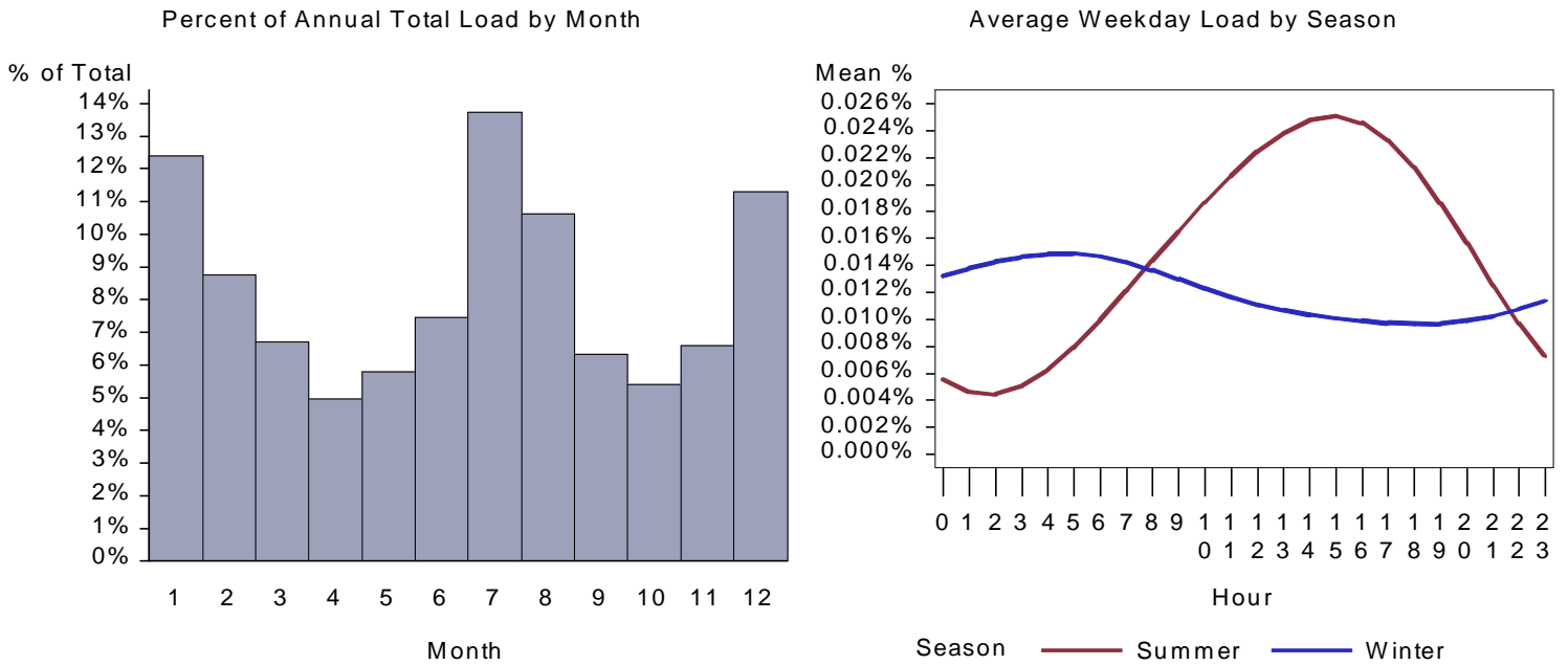
Figure 58. ID Health HVAC Aux Load by Month and Average Weekday
