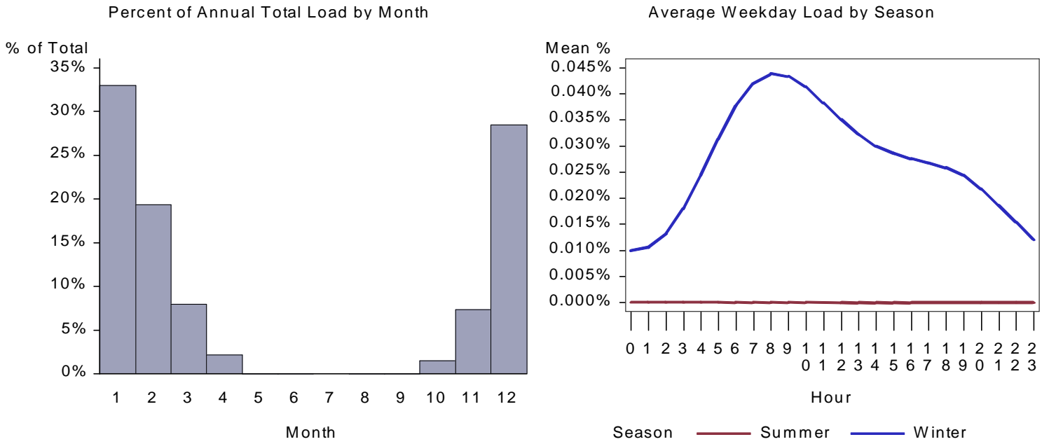
Figure 363. : ID Grocery Space Heat Load by Month and Average Weekday
