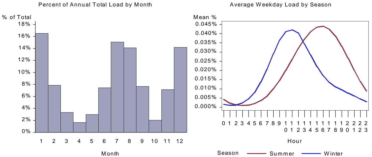
Figure 102. : CA Warehouse HVAC Aux Load by Month and Average Weekday
