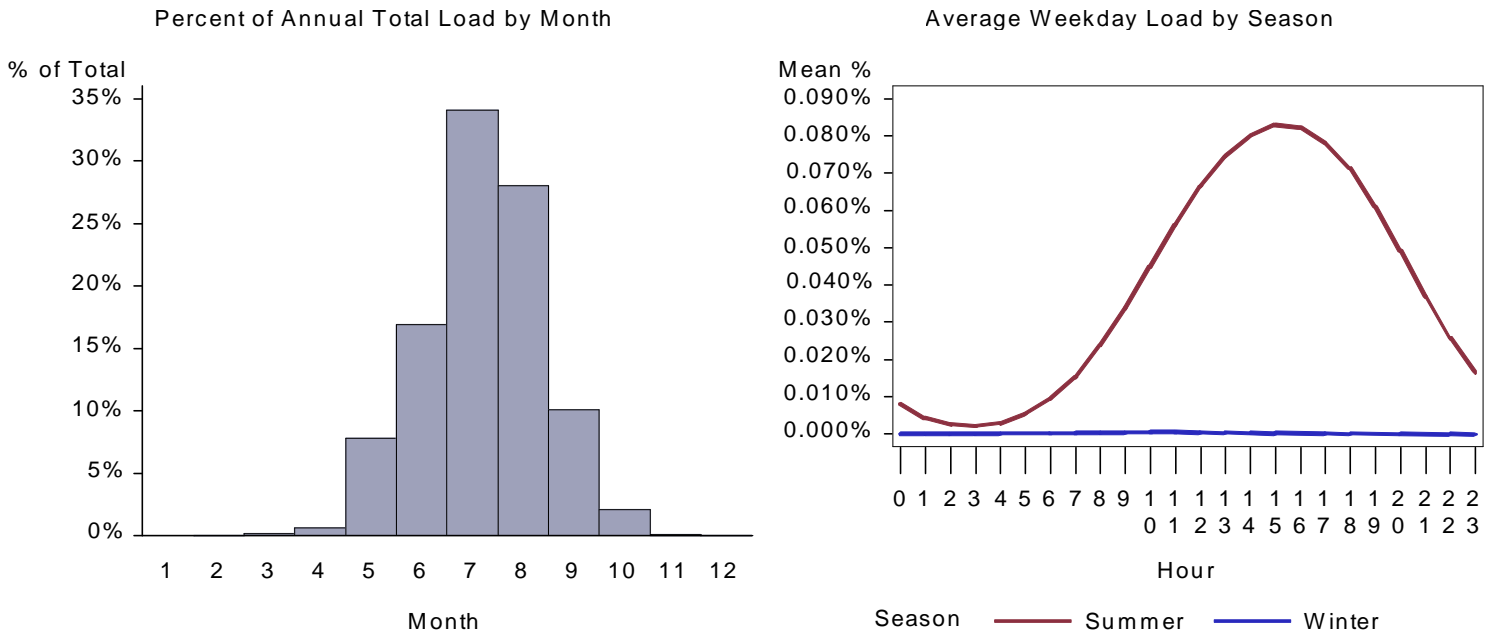
Figure 358. : UT Warehouse Space Cool Load by Month and Average Weekday
