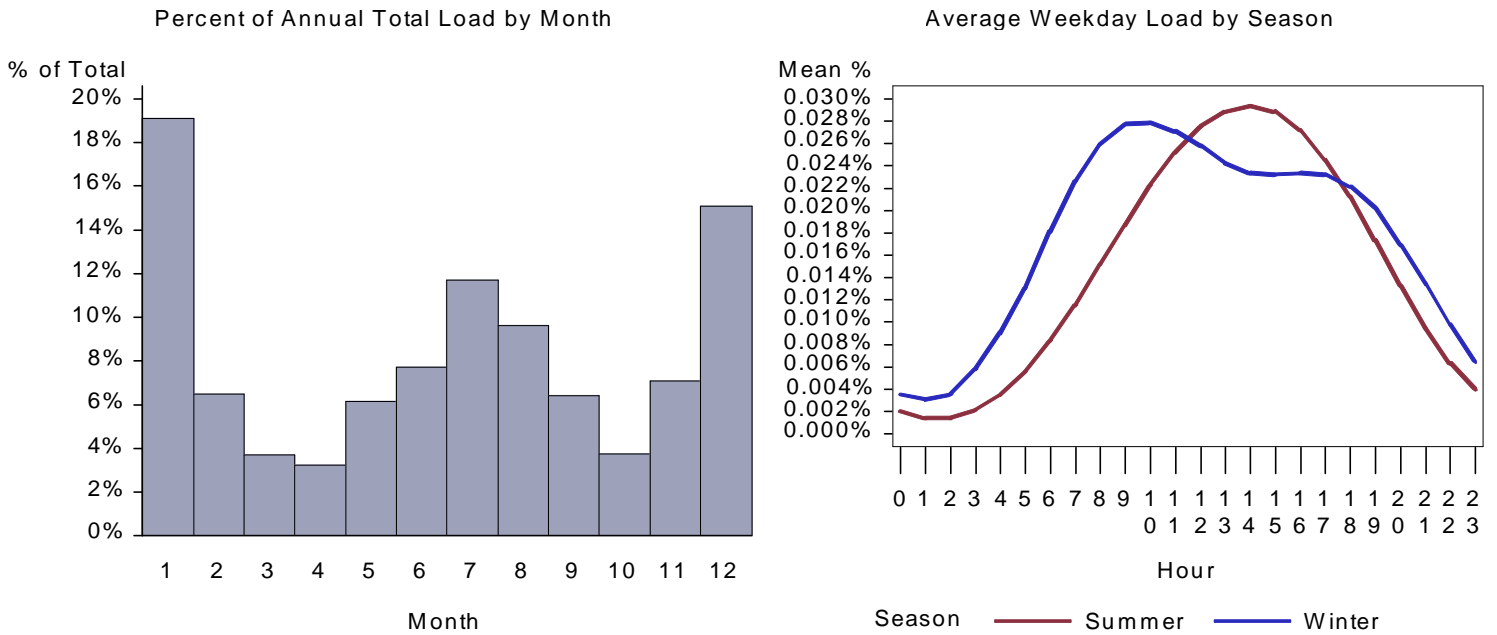
Figure 100. : WA Small Retail HVAC Aux Load by Month and Average Weekday
