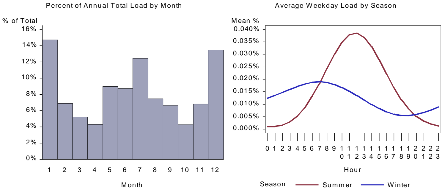
Figure 90. WA School HVAC Aux Load by Month and Average Weekday
