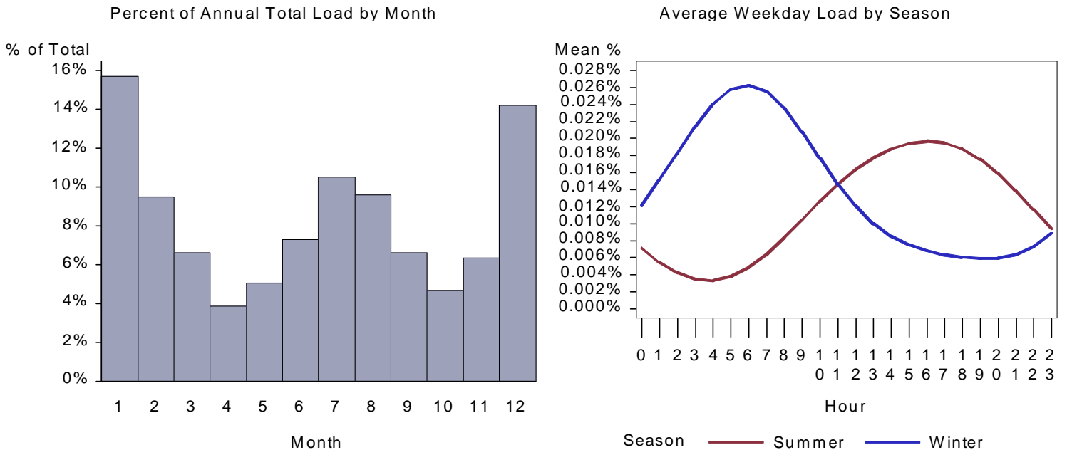
Figure 86. WY Restaurant HVAC Aux Load by Month and Average Weekday
