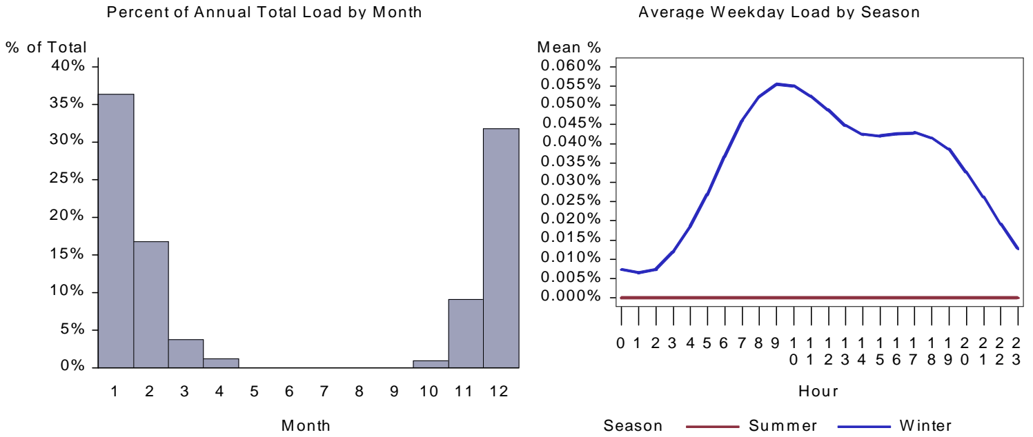
Figure 379. : UT Large Retail Space Heat Load by Month and Average Weekday
