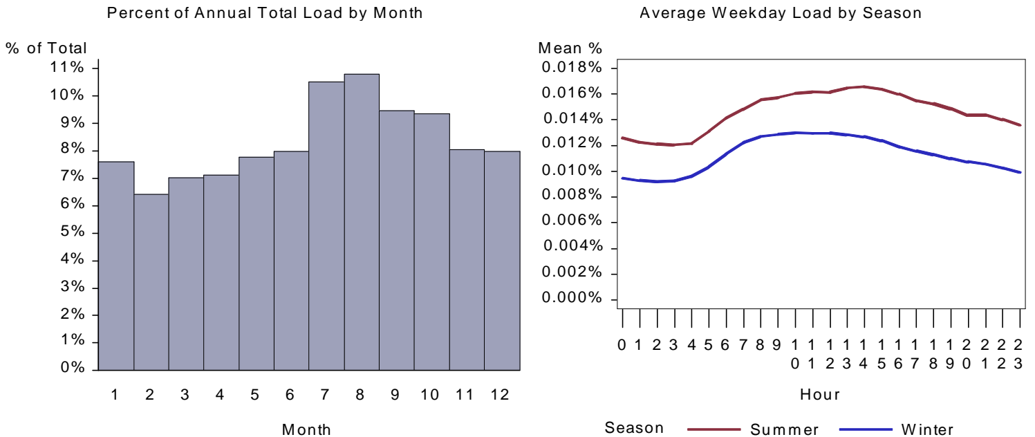
Figure 258. : ID Grocery Refrigeration Load by Month and Average Weekday
