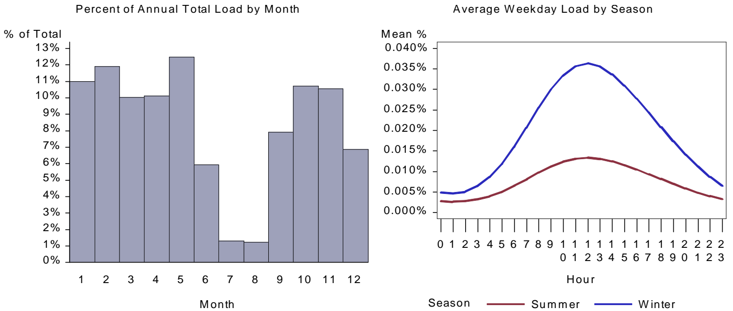
Figure 456. : WA School Water Heat Load by Month and Average Weekday
