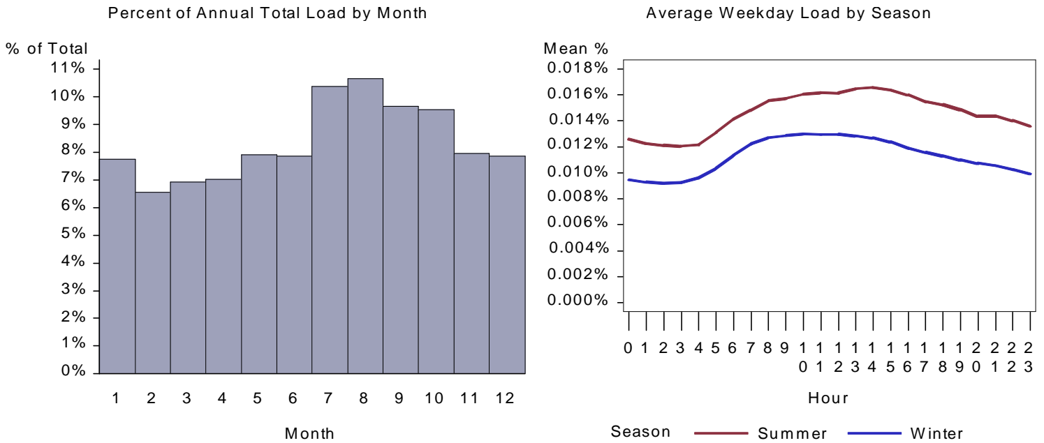
Figure 290. : CA Small Office Refrigeration Load by Month and Average Weekday
