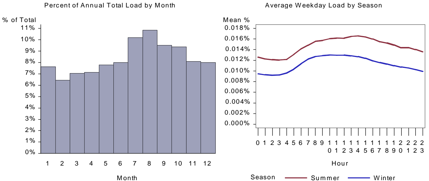
Figure 284. : WY Restaurant Refrigeration Load by Month and Average Weekday
