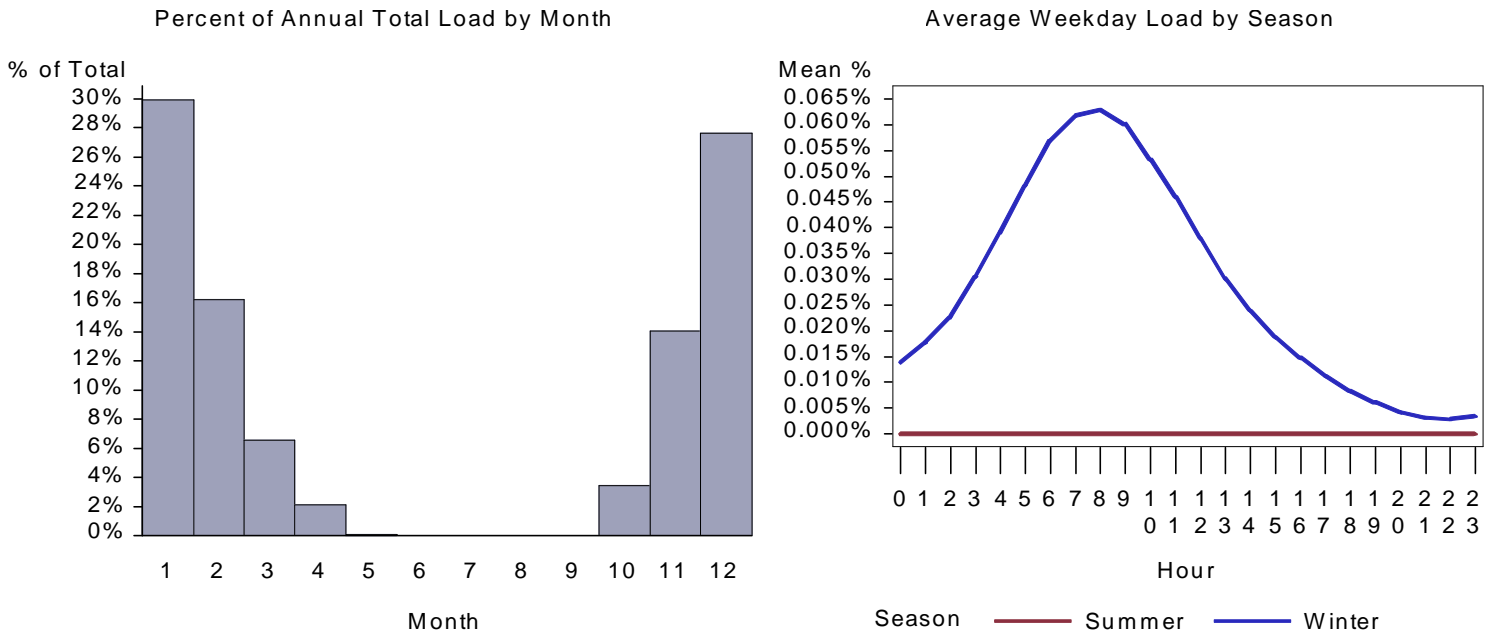
Figure 402. : CA Small Office Space Heat Load by Month and Average Weekday
