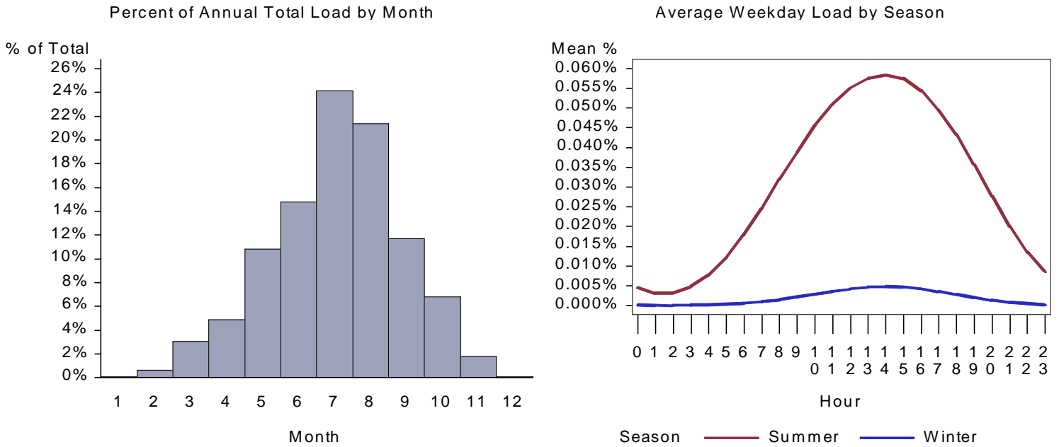
Figure 323. : UT Large Retail Space Cool Load by Month and Average Weekday
