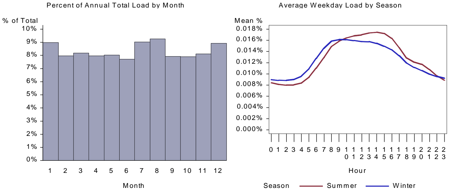
Figure 247. : ID Small Retail Plug Load Load by Month and Average Weekday
