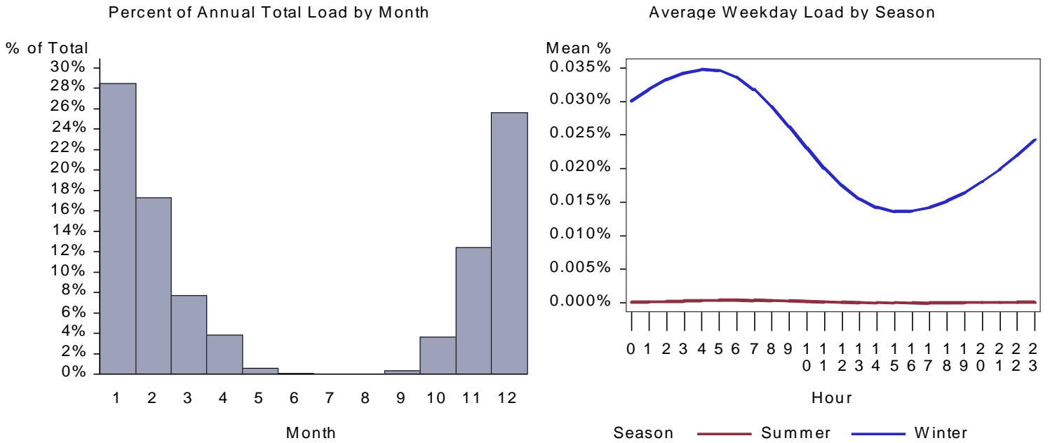
Figure 369. : UT Health Space Heat Load by Month and Average Weekday
