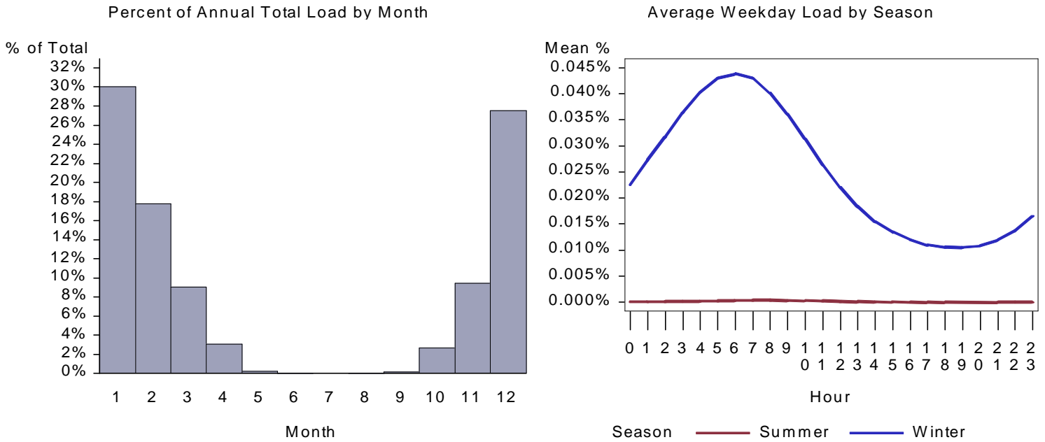
Figure 393. : ID Restaurant Space Heat Load by Month and Average Weekday
