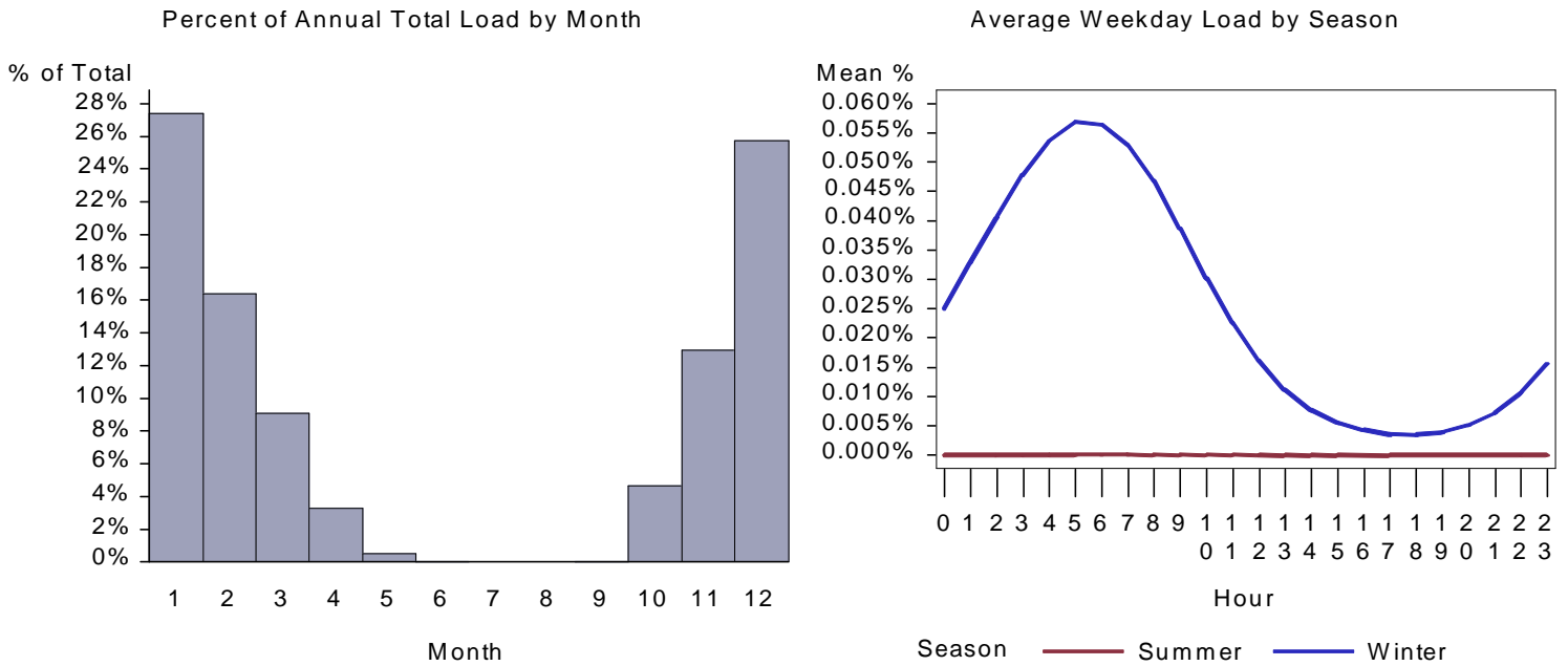
Figure 392. : CA Restaurant Space Heat Load by Month and Average Weekday
