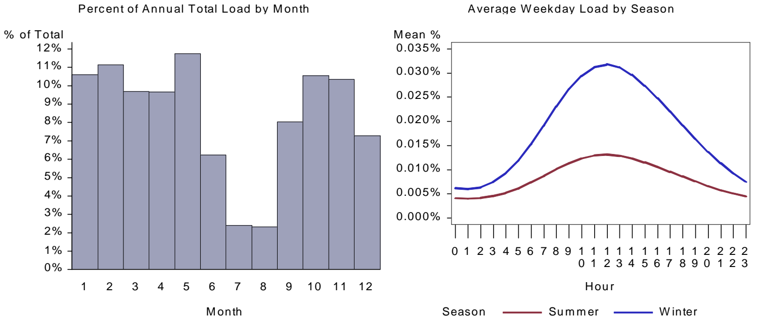
Figure 453. : CA School Water Heat Load by Month and Average Weekday
