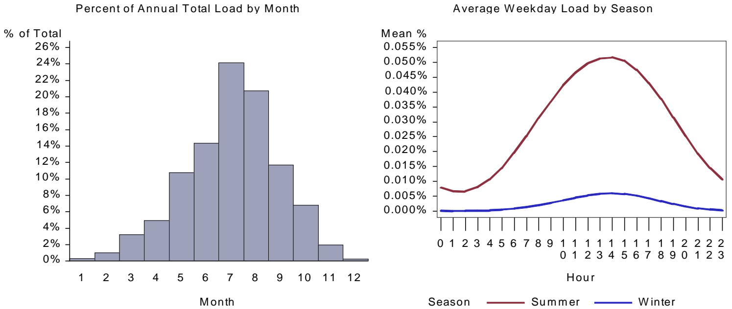
Figure 333. : UT Miscellaneous Space Cool Load by Month and Average Weekday
