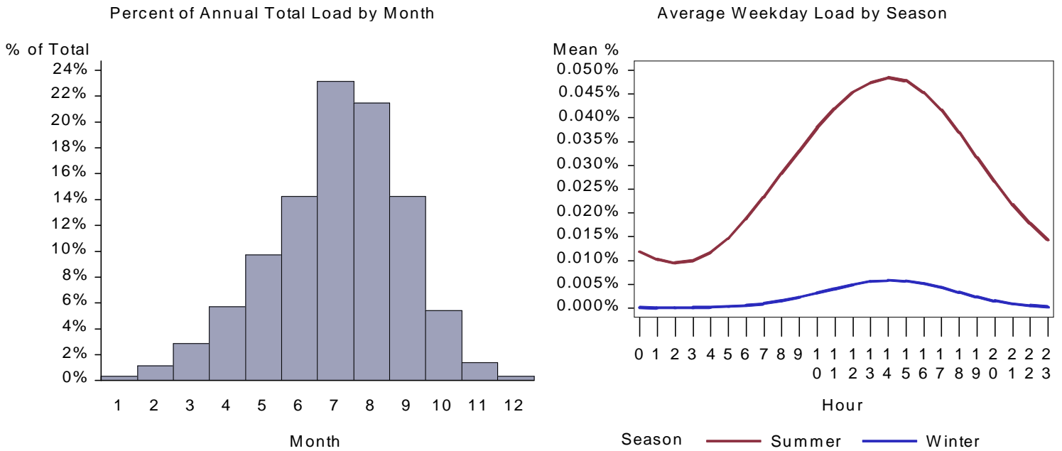
Figure 346. : CA Small Office Space Cool Load by Month and Average Weekday
