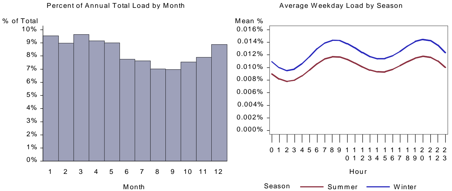
Figure 440. : UT Lodging Water Heat Load by Month and Average Weekday
