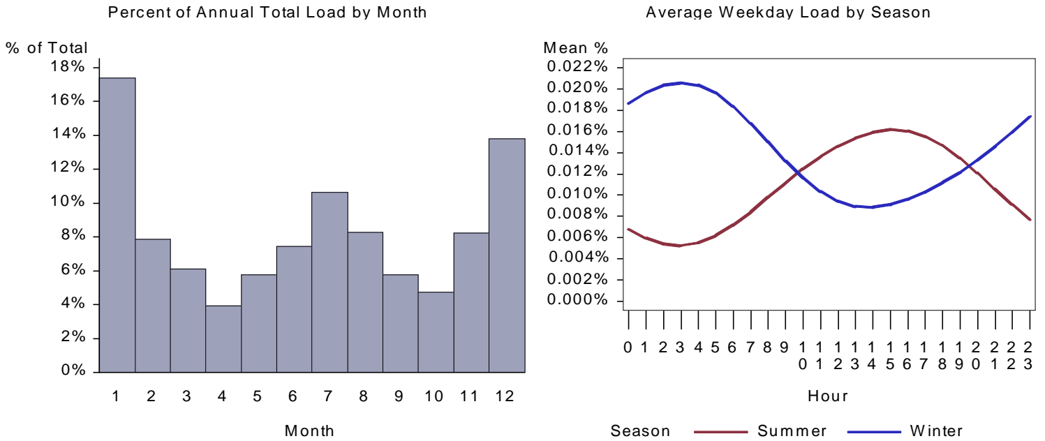
Figure 127. : WA Lodging Heat Pump Load by Month and Average Weekday
