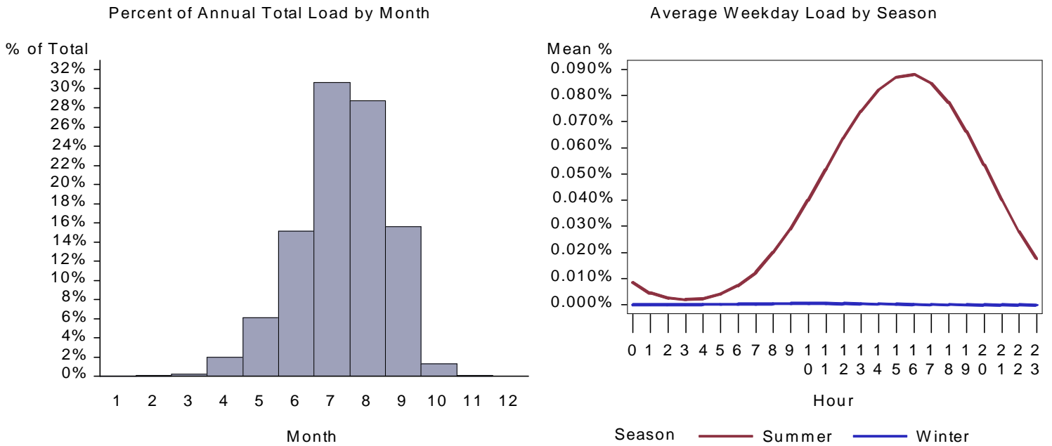
Figure 356. : CA Warehouse Space Cool Load by Month and Average Weekday
