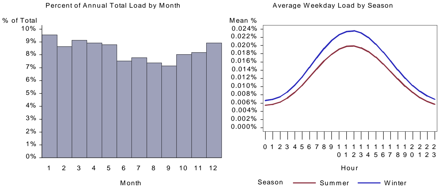
Figure 428. : CA Large Office Water Heat Load by Month and Average Weekday
