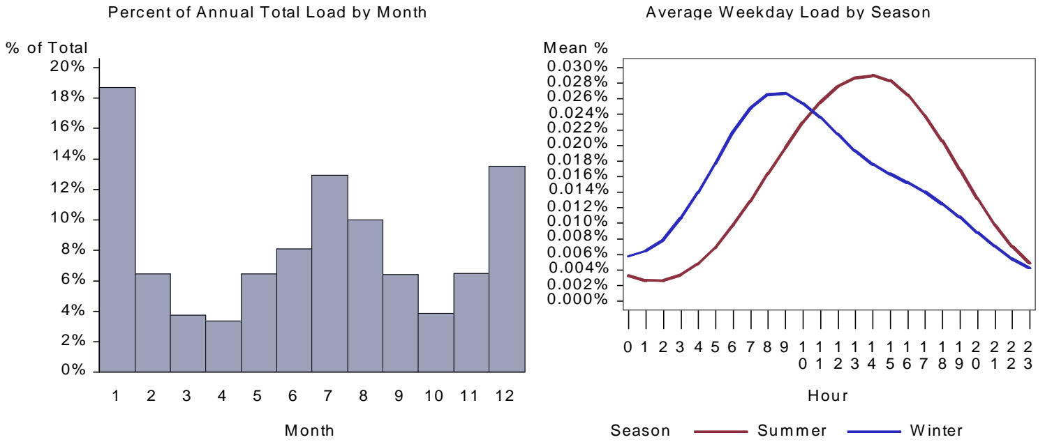
Figure 131. : WA Miscellaneous Heat Pump Load by Month and Average Weekday
