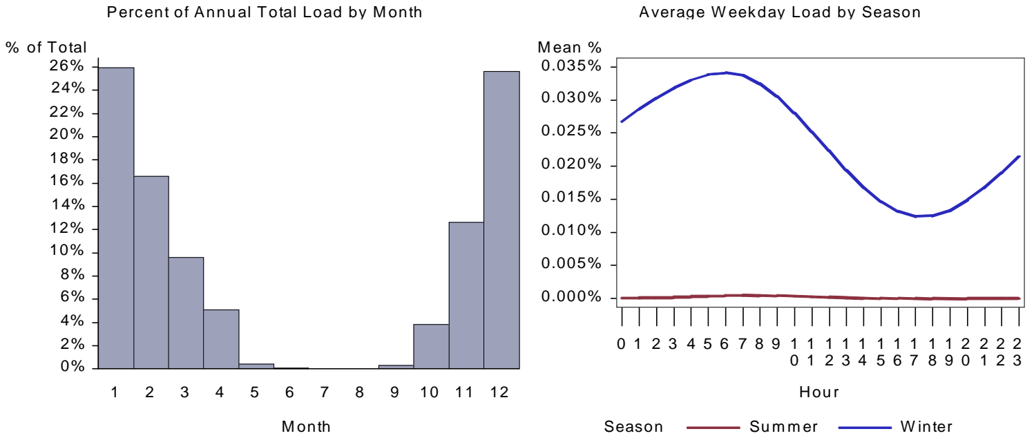
Figure 399. : UT School Space Heat Load by Month and Average Weekday
