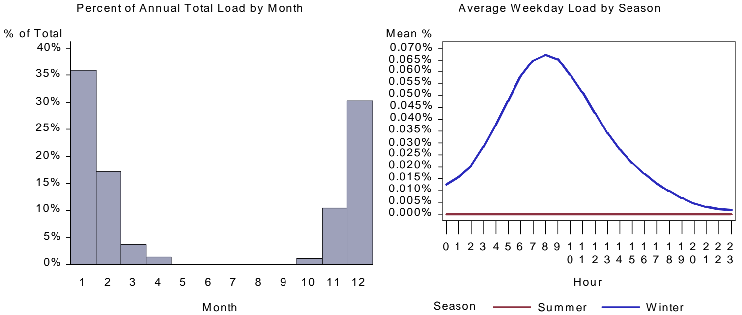
Figure 374. : UT Large Office Space Heat Load by Month and Average Weekday
