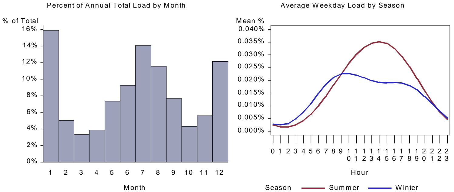
Figure 123. : WA Large Retail Heat Pump Load by Month and Average Weekday
