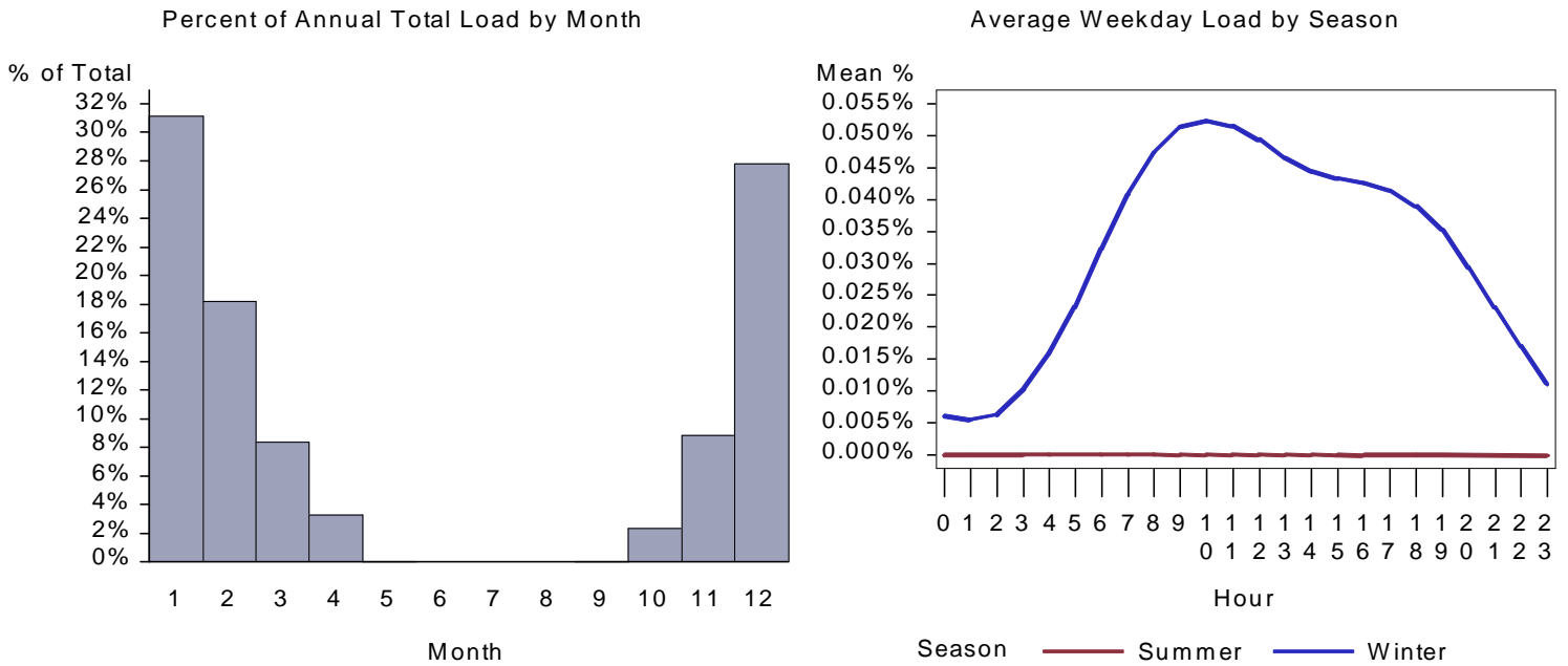
Figure 408. : ID Small Retail Space Heat Load by Month and Average Weekday
