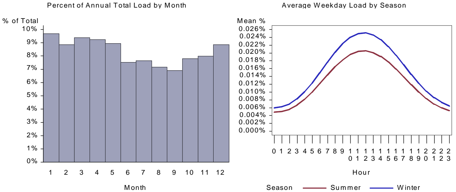
Figure 459. : ID Small Office Water Heat Load by Month and Average Weekday
