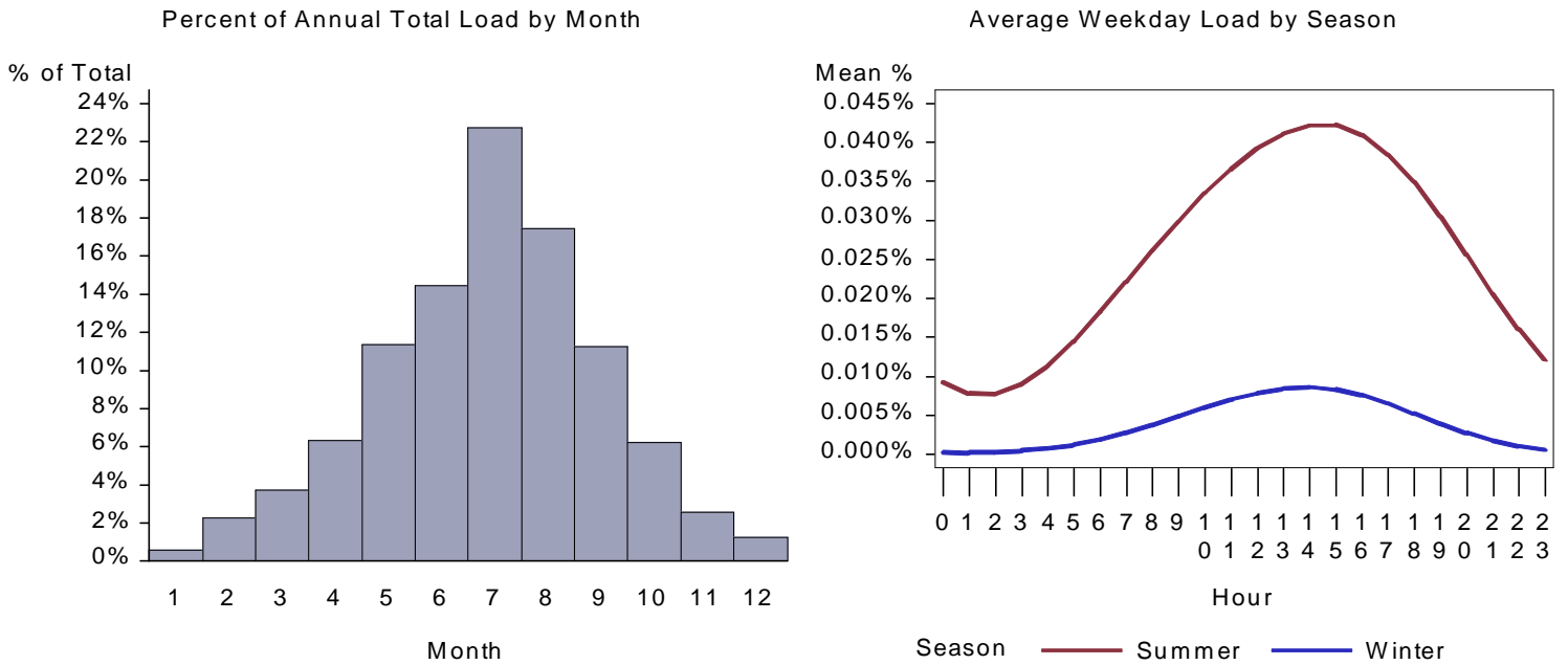
Figure 314. : WA Health Space Cool Load by Month and Average Weekday
