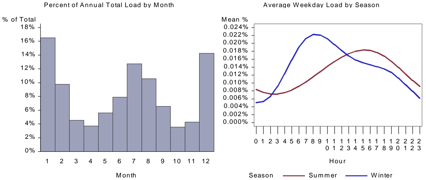
Figure 53. ID Grocery HVAC Aux Load by Month and Average Weekday
