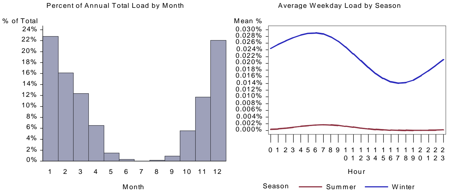
Figure 398. : ID School Space Heat Load by Month and Average Weekday
