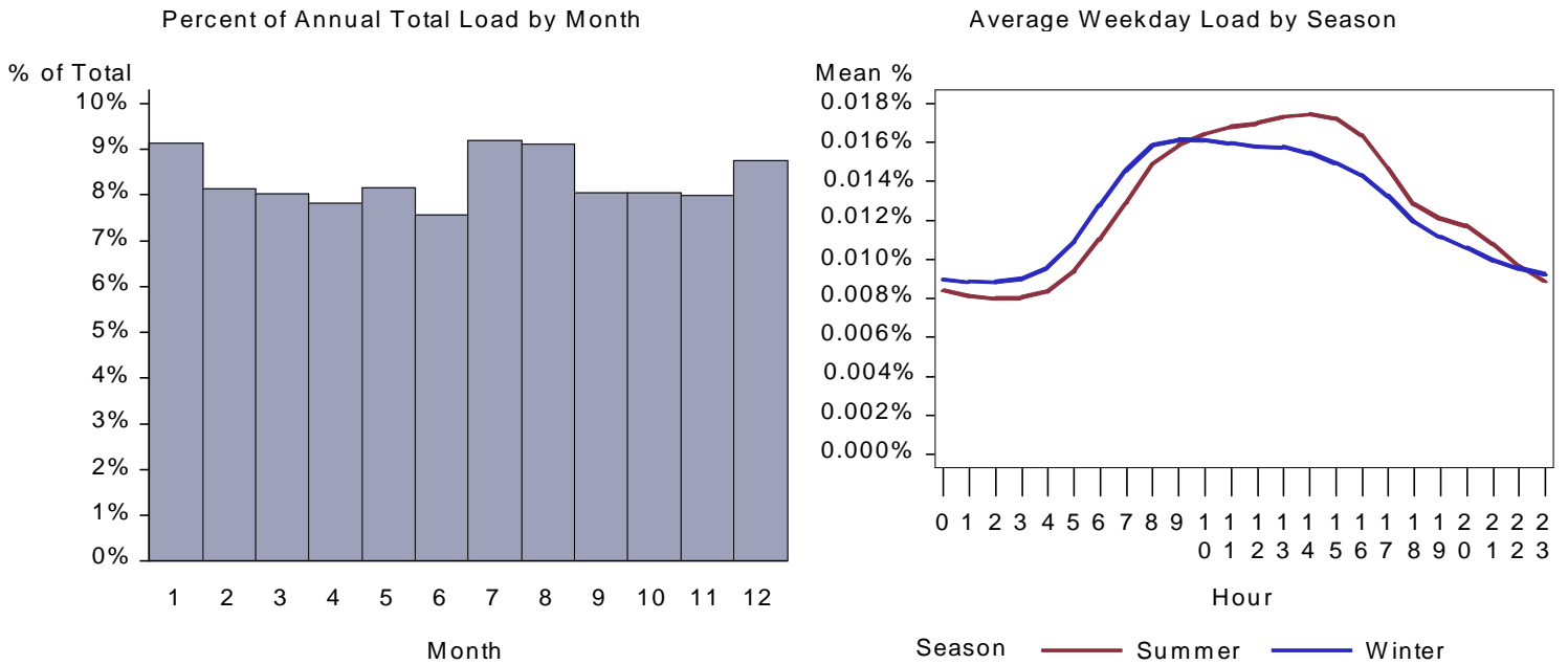
Figure 252. : ID Warehouse Plug Load Load by Month and Average Weekday
