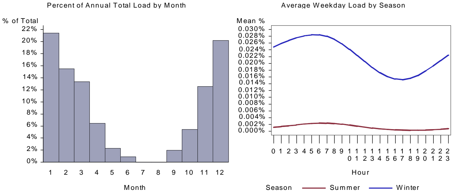
Figure 401. : WY School Space Heat Load by Month and Average Weekday
