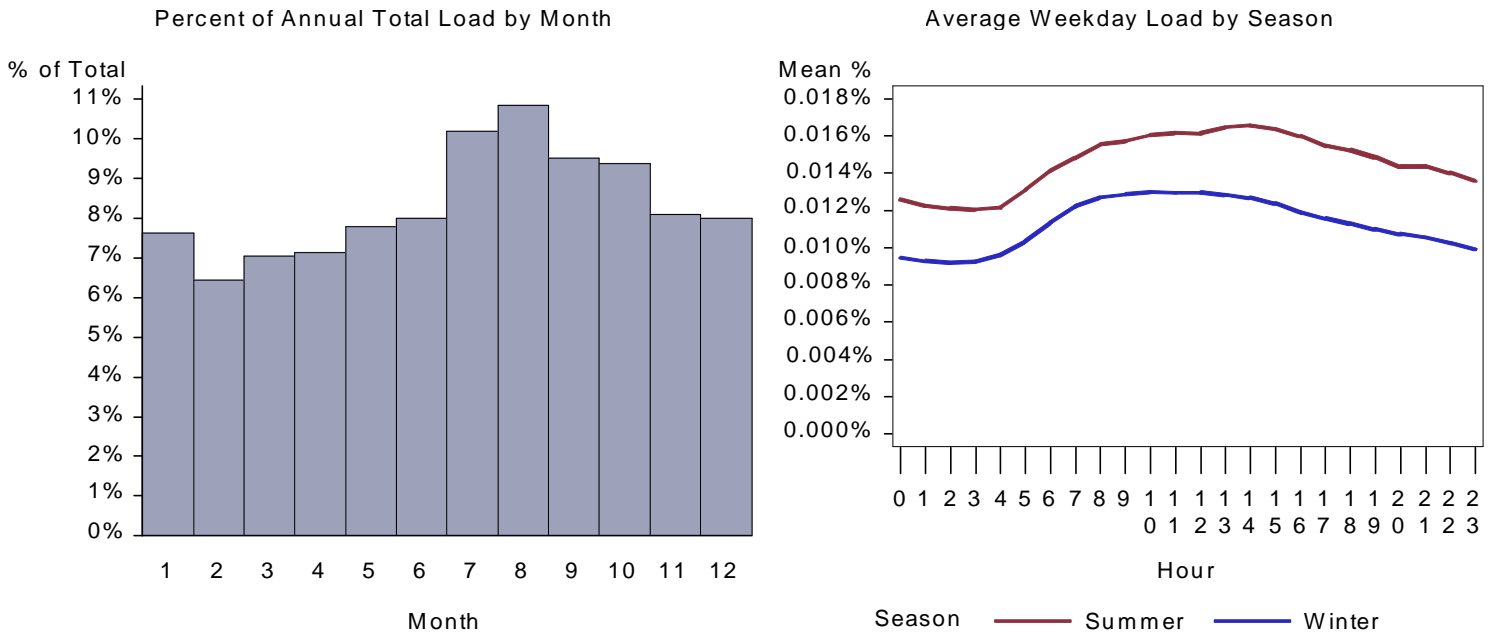
Figure 296. : ID Small Retail Refrigeration Load by Month and Average Weekday
