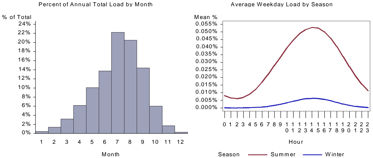
Figure 331. : CA Miscellaneous Space Cool Load by Month and Average Weekday
