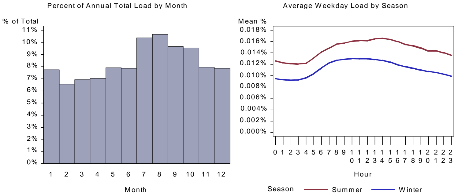
Figure 264. : UT Health Refrigeration Load by Month and Average Weekday
