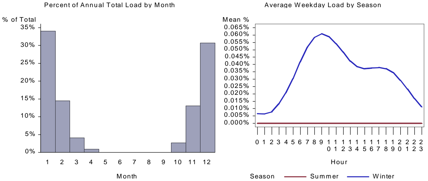
Figure 377.: CA Large Retail Space Heat Load by Month and Average Weekday
