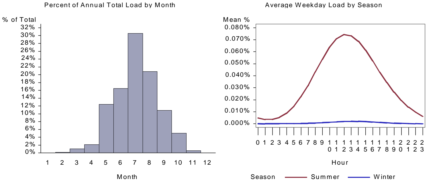
Figure 343. : UT School Space Cool Load by Month and Average Weekday
