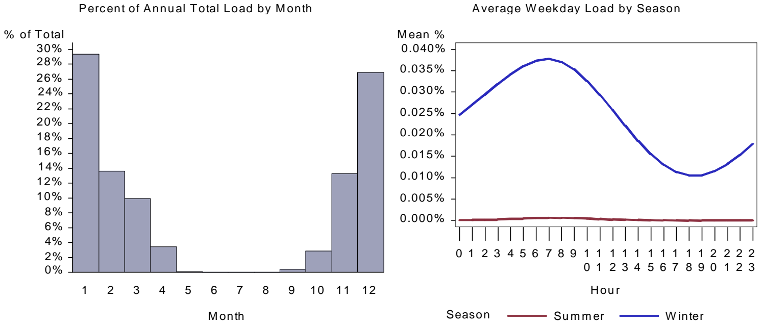
Figure 400. : WA School Space Heat Load by Month and Average Weekday
