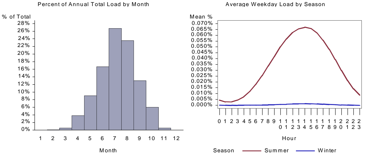
Figure 355. : WY Small Retail Space Cool Load by Month and Average Weekday
