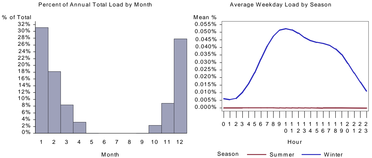
Figure 378.: ID Large Retail Space Heat Load by Month and Average Weekday
