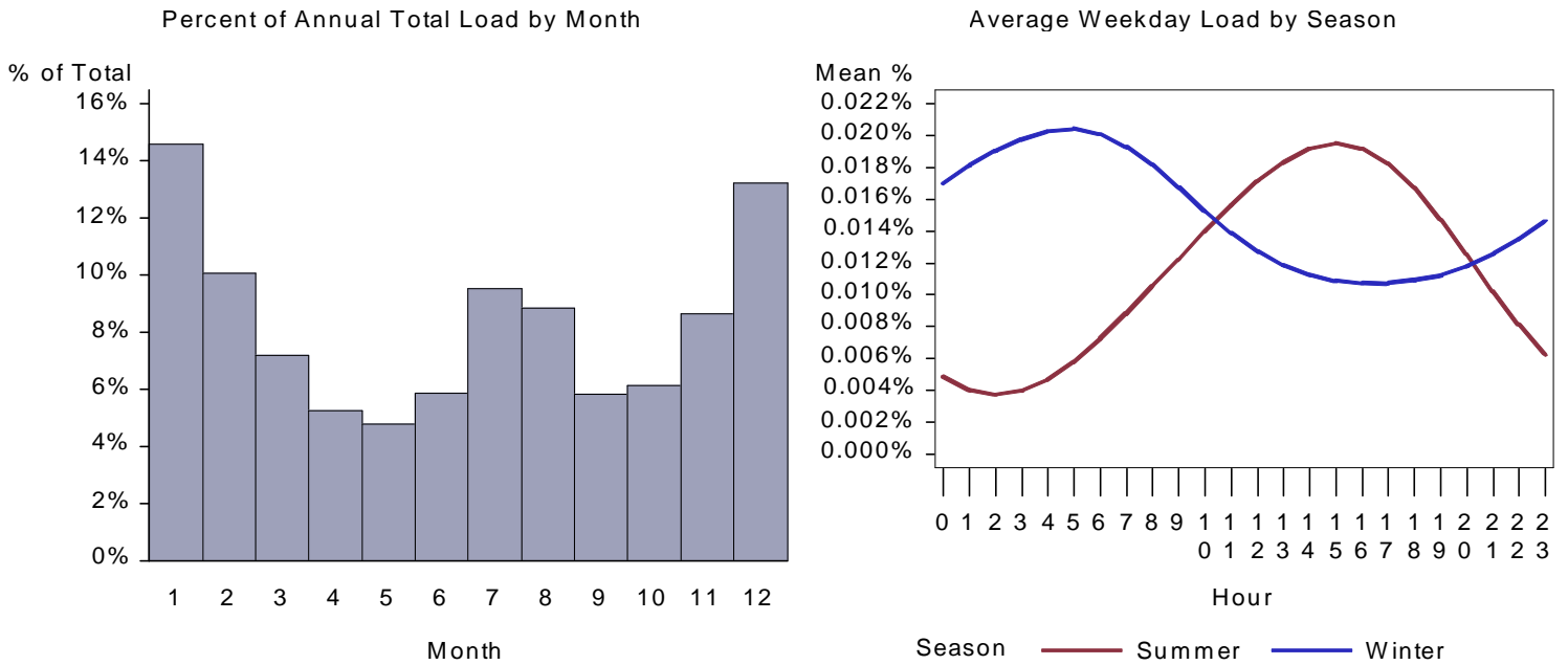
Figure 112. : CA Health Heat Pump Load by Month and Average Weekday
