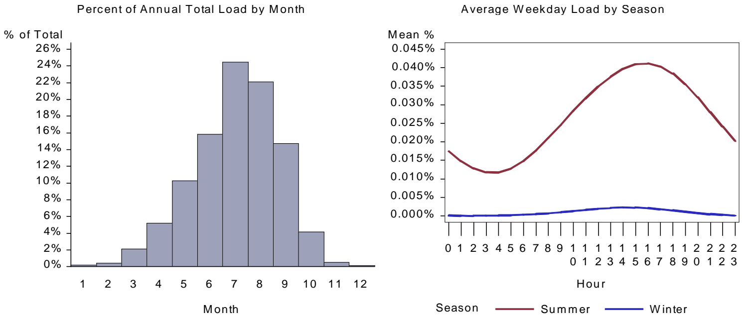
Figure 326. : CA Lodging Space Cool Load by Month and Average Weekday
