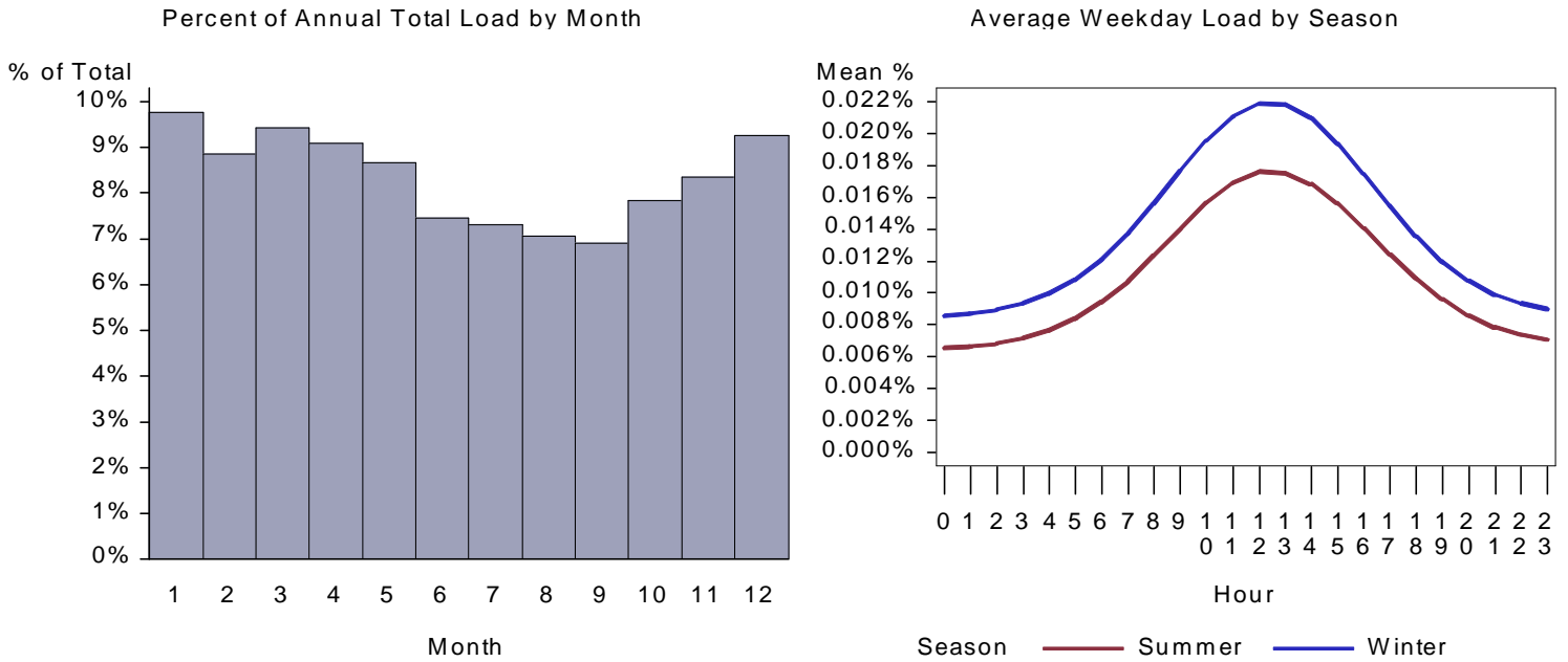
Figure 43. UT Small Retail Cooking Load by Month and Average Weekday
