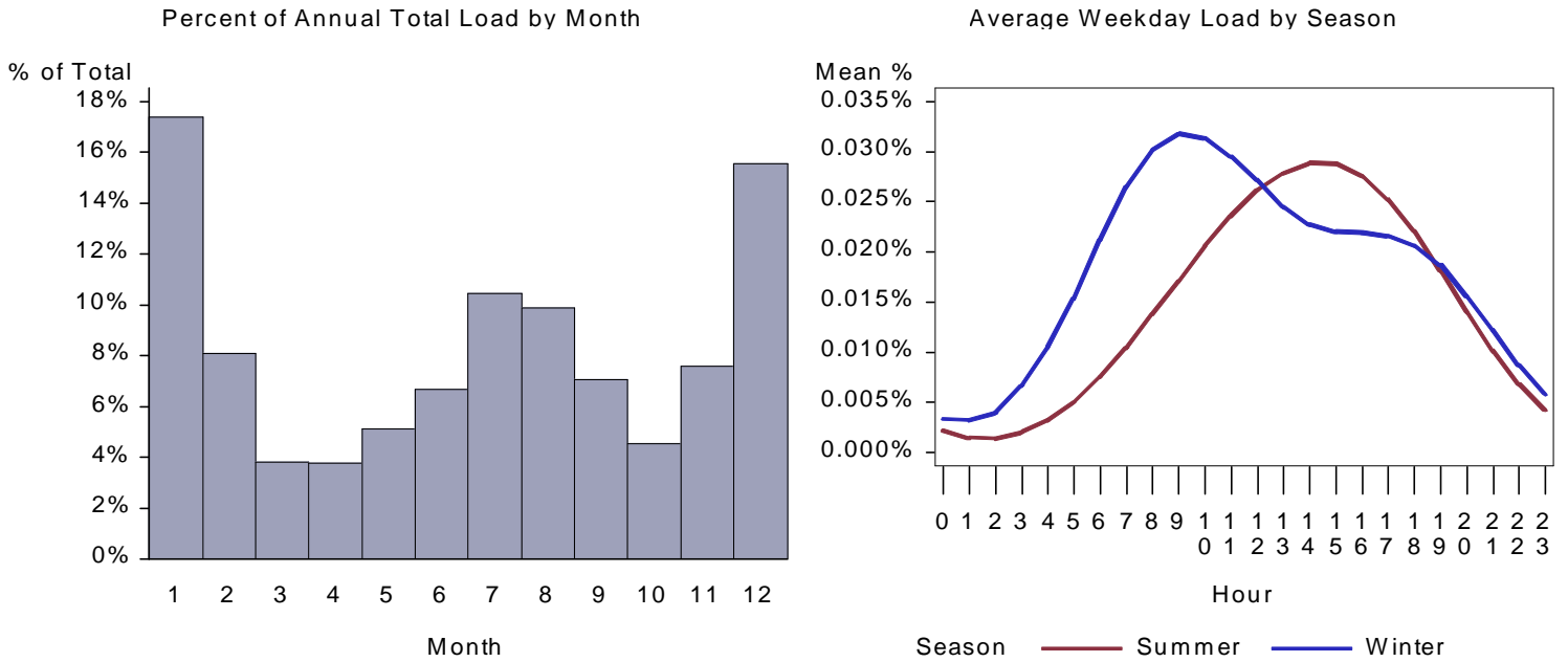
Figure 97. CA Small Retail HVAC Aux Load by Month and Average Weekday
