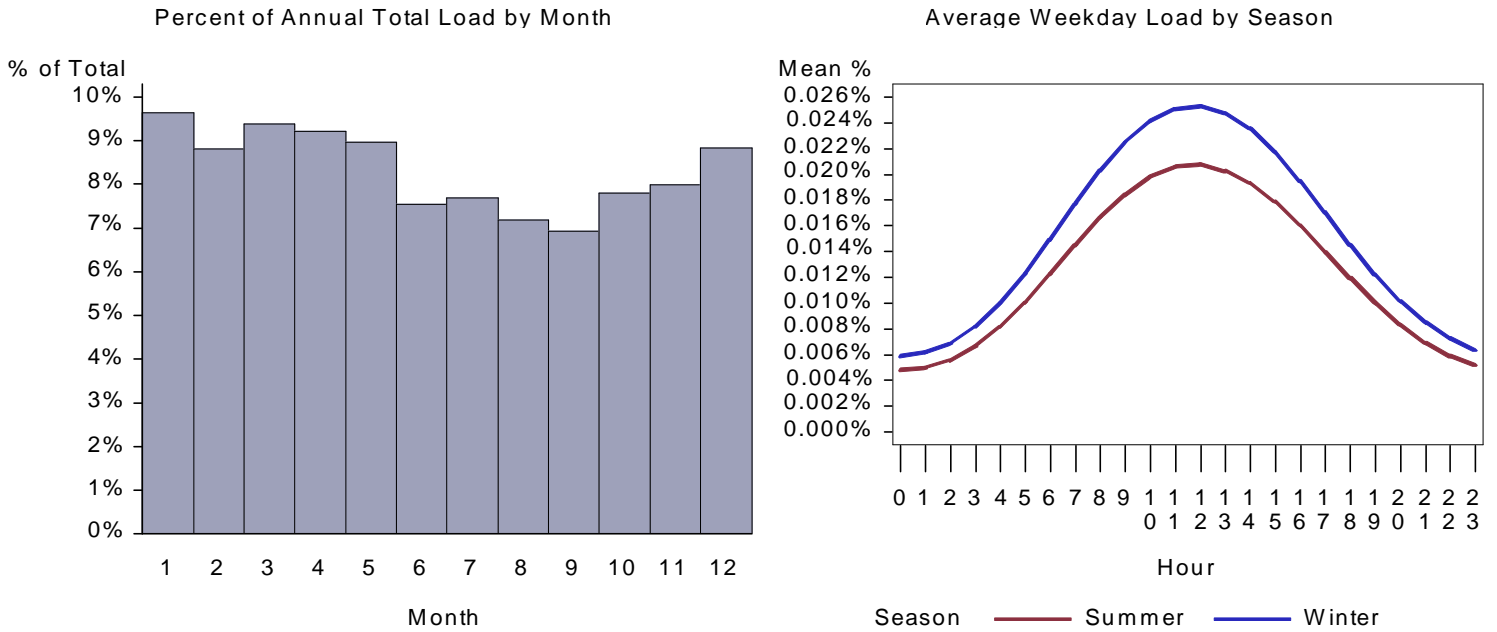
Figure 15. WY Large Office Cooking Load by Month and Average Weekday
