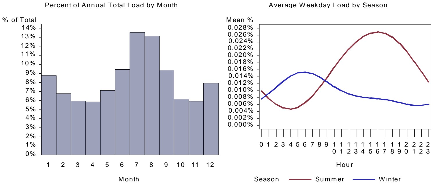
Figure 133. : CA Restaurant Heat Pump Load by Month and Average Weekday
