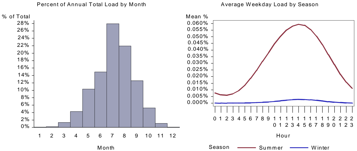
Figure 332. : ID Miscellaneous Space Cool Load by Month and Average Weekday
