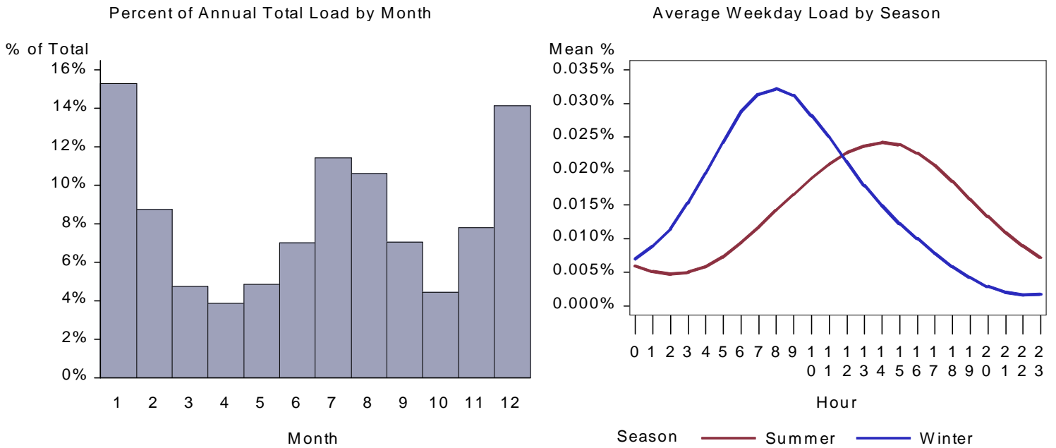
Figure 92. CA Small Office HVAC Aux Load by Month and Average Weekday
