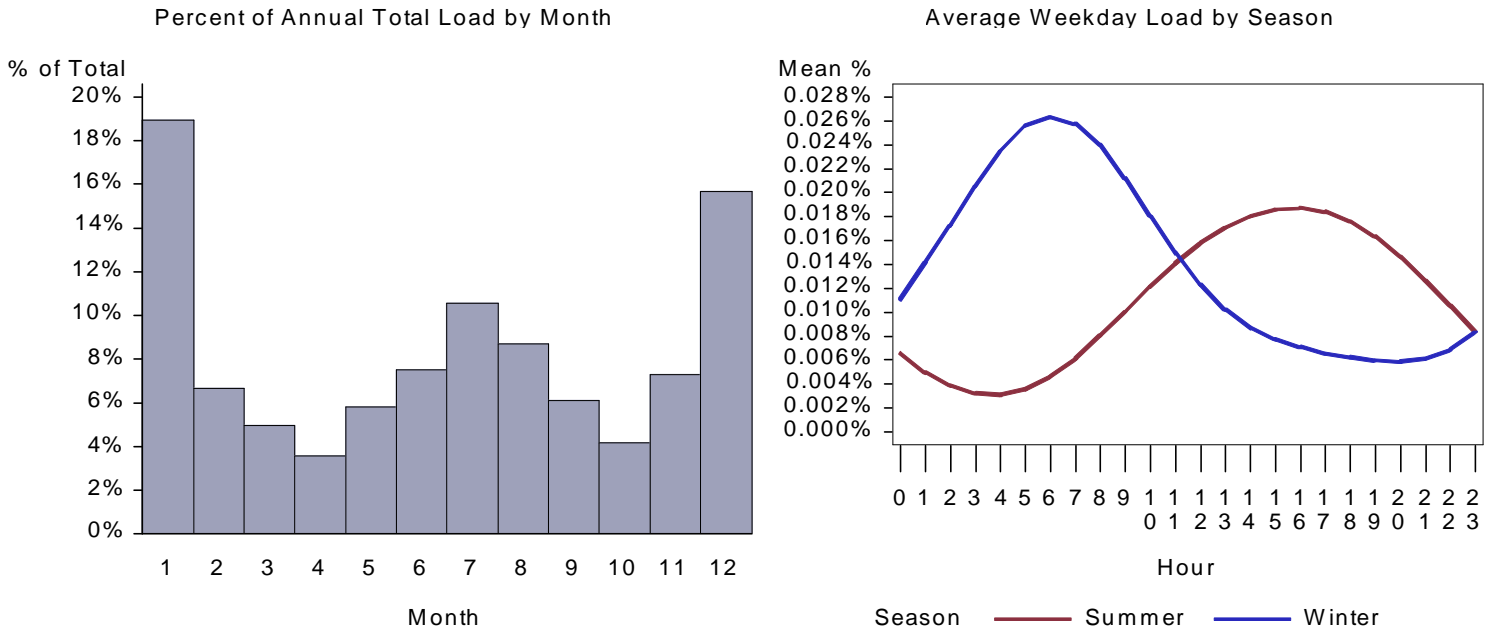
Figure 85. WA Restaurant HVAC Aux Load by Month and Average Weekday
