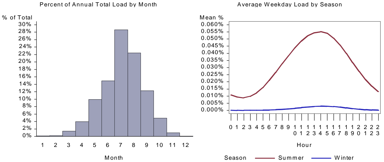
Figure 317. : ID Large Office Space Cool Load by Month and Average Weekday
