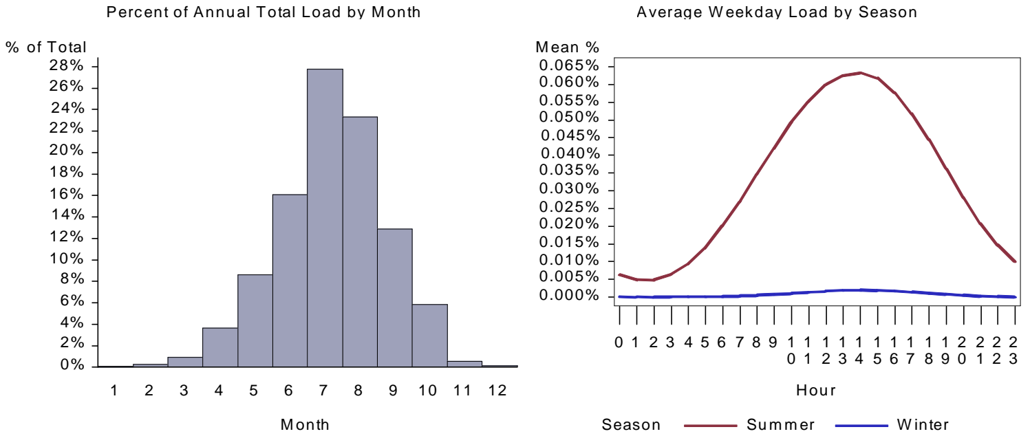
Figure 335. : WY Miscellaneous Space Cool Load by Month and Average Weekday
