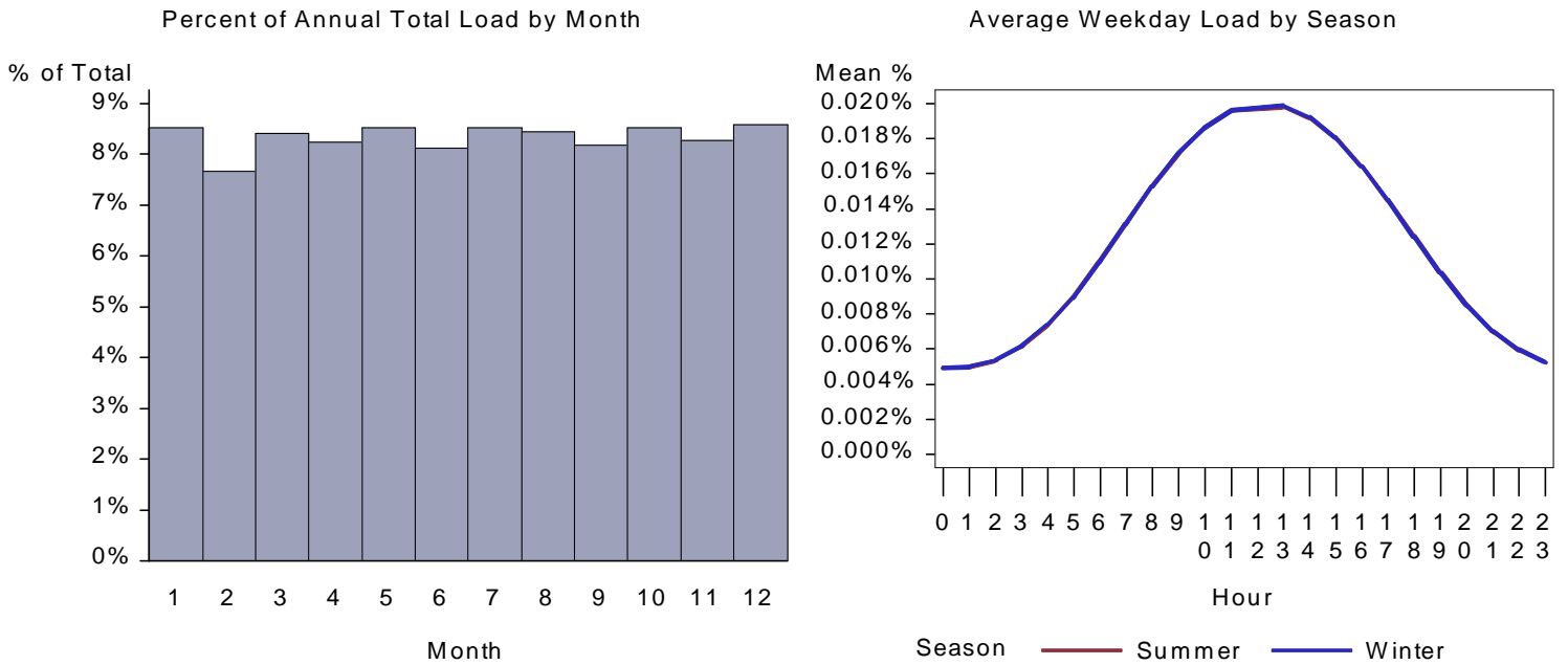
Figure 162. : CA Large Retail Lighting Load by Month and Average Weekday
