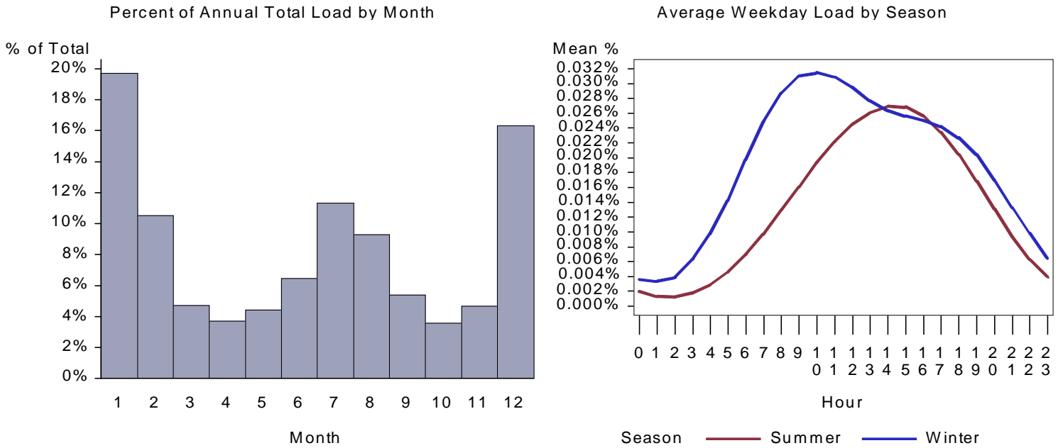
Figure 143.: ID Small Retail Heat Pump Load by Month and Average Weekday
