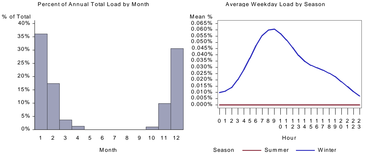
Figure 389. : UT Miscellaneous Space Heat Load by Month and Average Weekday
