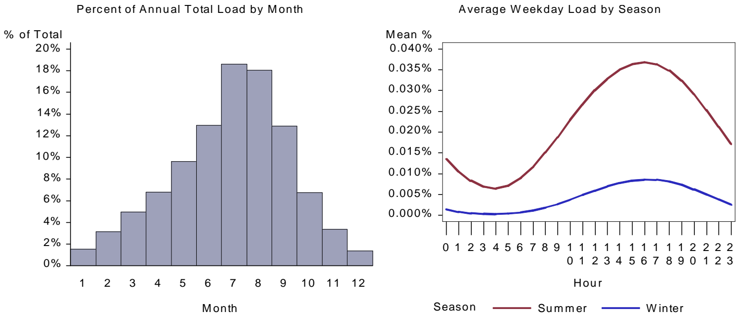
Figure 336. : CA Restaurant Space Cool Load by Month and Average Weekday
