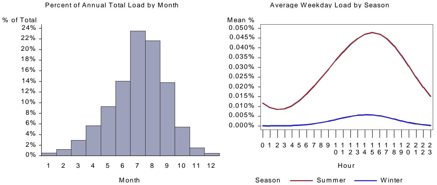
Figure 311. : CA Health Space Cool Load by Month and Average Weekday
