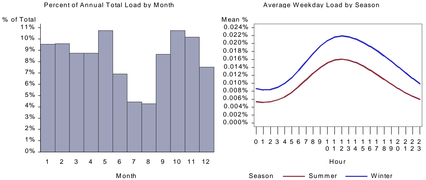
Figure 183. : ID School Lighting Load by Month and Average Weekday
