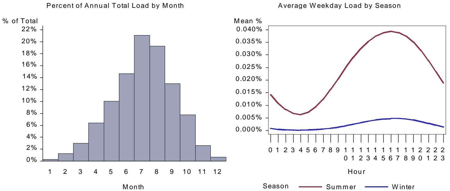
Figure 340. : WY Restaurant Space Cool Load by Month and Average Weekday
