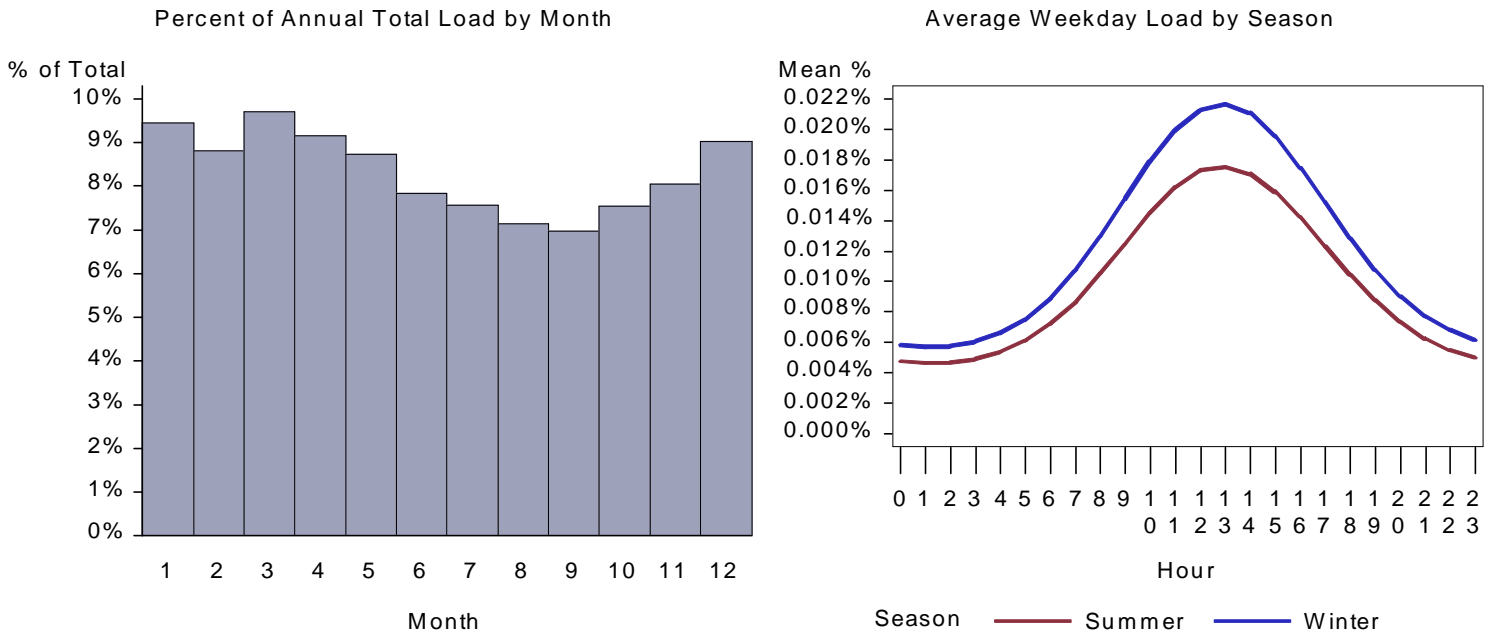
Figure 420. : UT Grocery Water Heat Load by Month and Average Weekday
