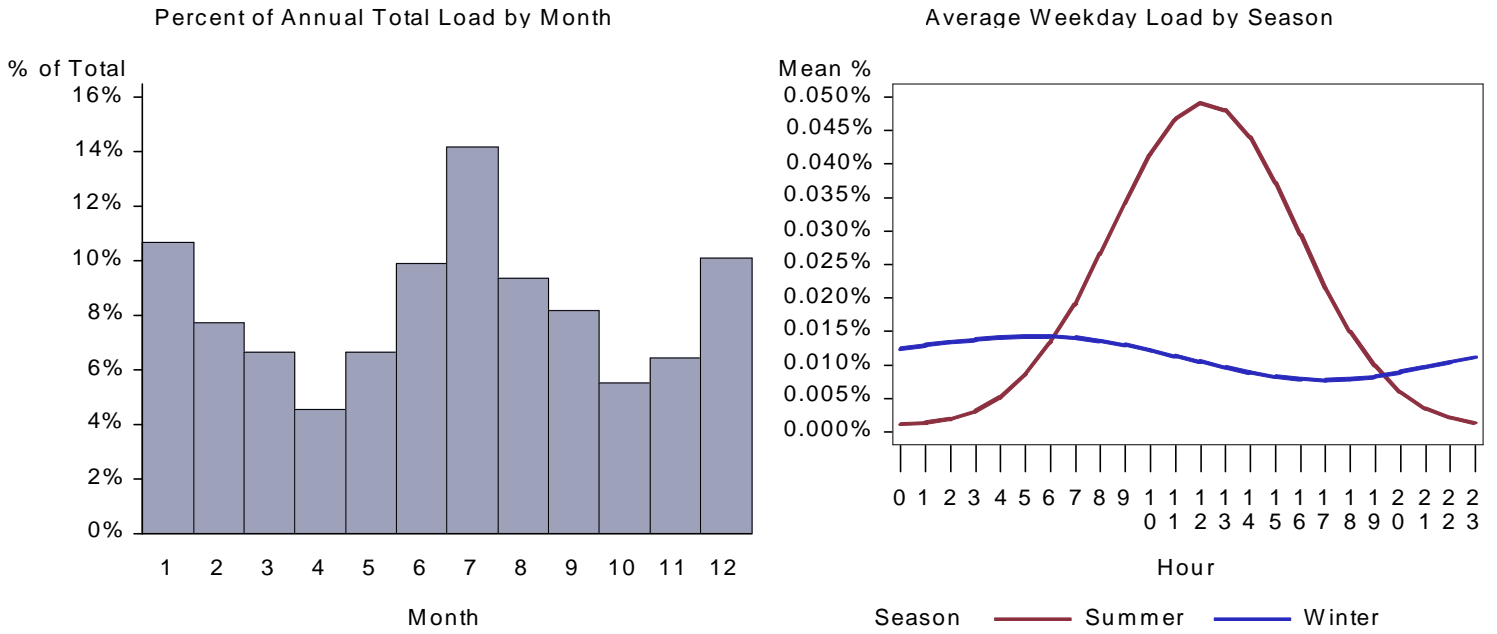
Figure 91. WY School HVAC Aux Load by Month and Average Weekday
