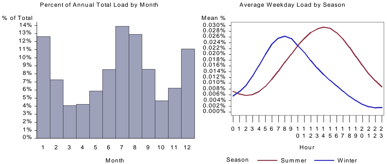
Figure 138. : CA Small Office Heat Pump Load by Month and Average Weekday
