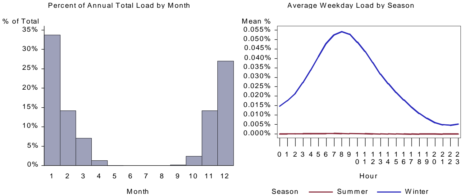
Figure 405. : WA Small Office Space Heat Load by Month and Average Weekday
