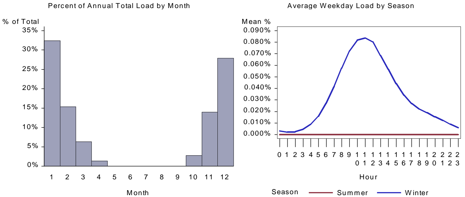
Figure 412. : CA Warehouse Space Heat Load by Month and Average Weekday
