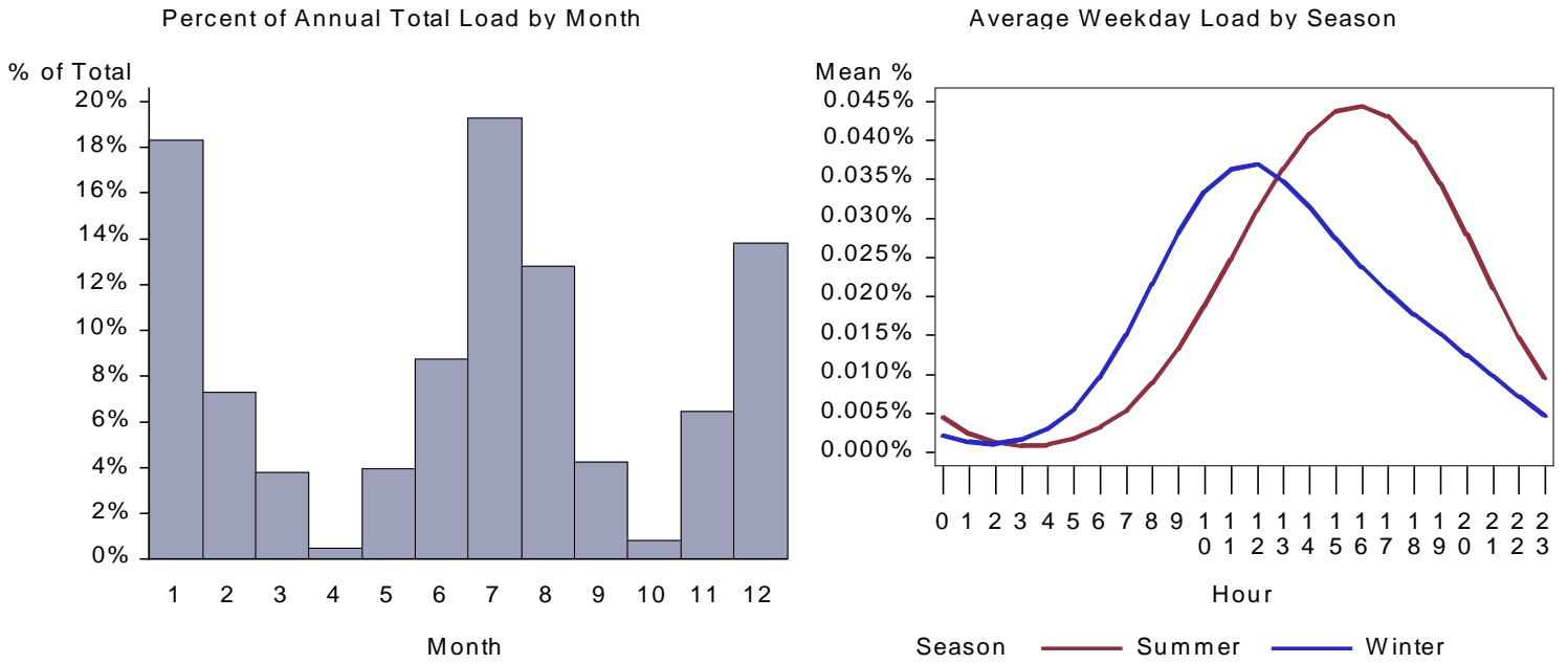
Figure 105. : WA Warehouse HVAC Aux Load by Month and Average Weekday
