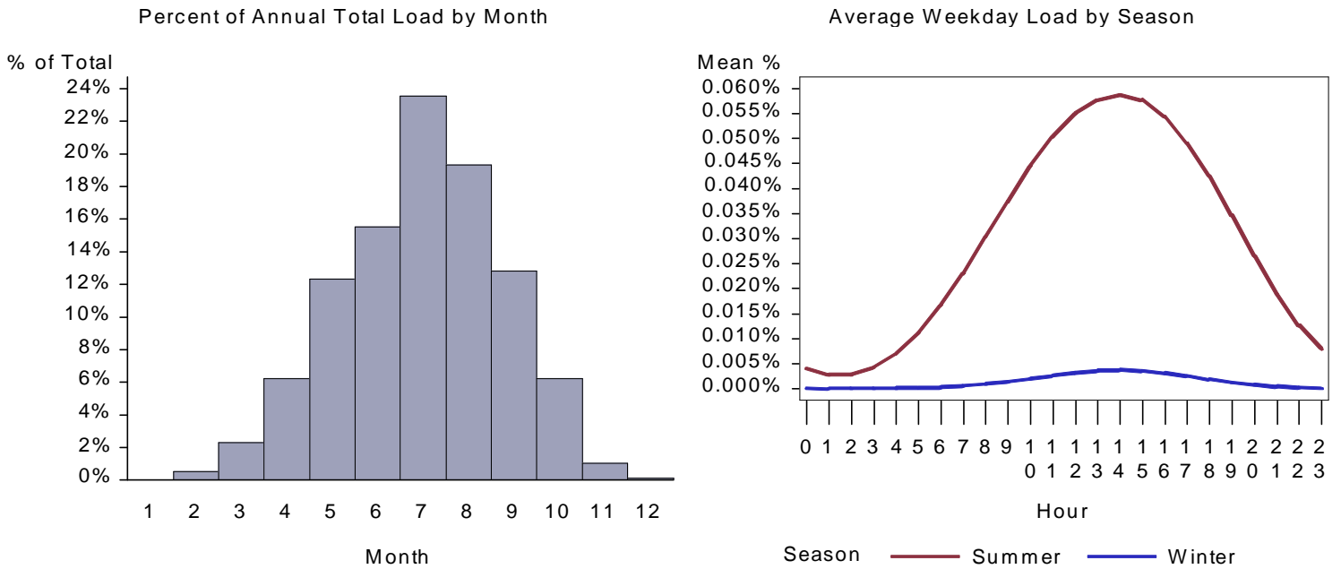
Figure 354. : WA Small Retail Space Cool Load by Month and Average Weekday
