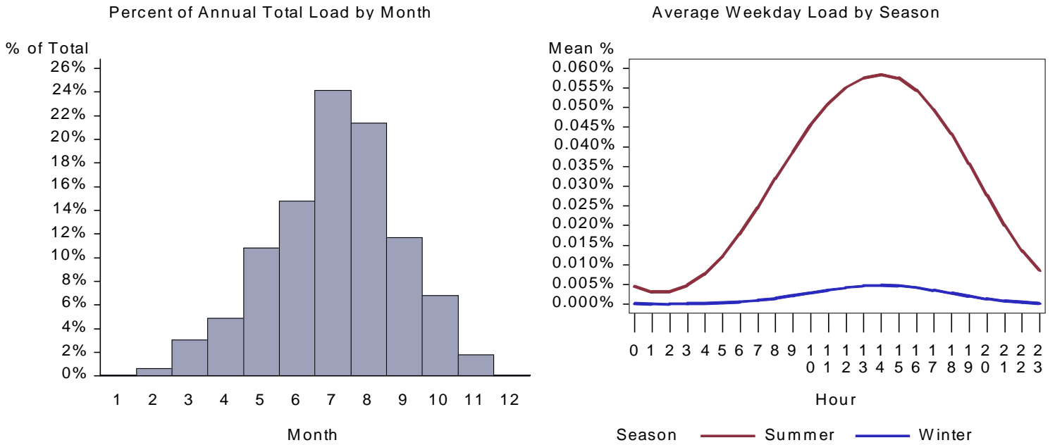
Figure 353. : UT Small Retail Space Cool Load by Month and Average Weekday
