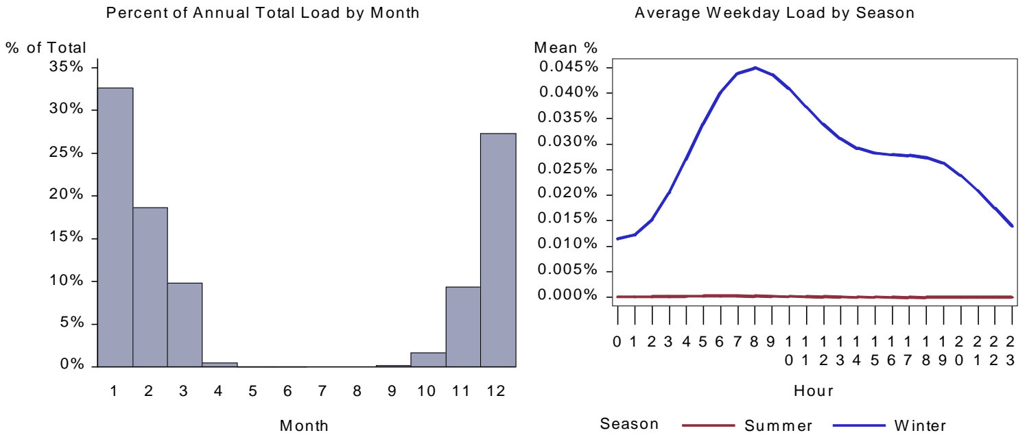
Figure 366. : WY Grocery Space Heat Load by Month and Average Weekday
