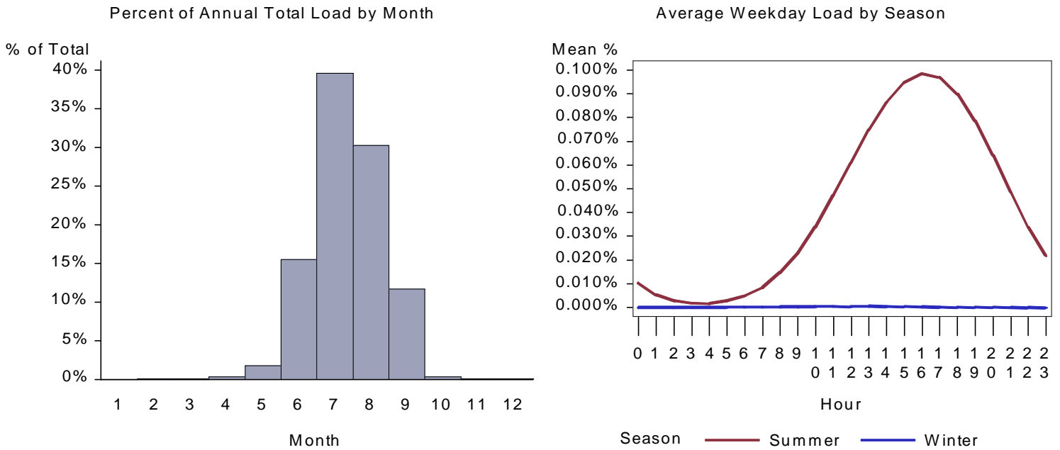
Figure 360. : WY Warehouse Space Cool Load by Month and Average Weekday
