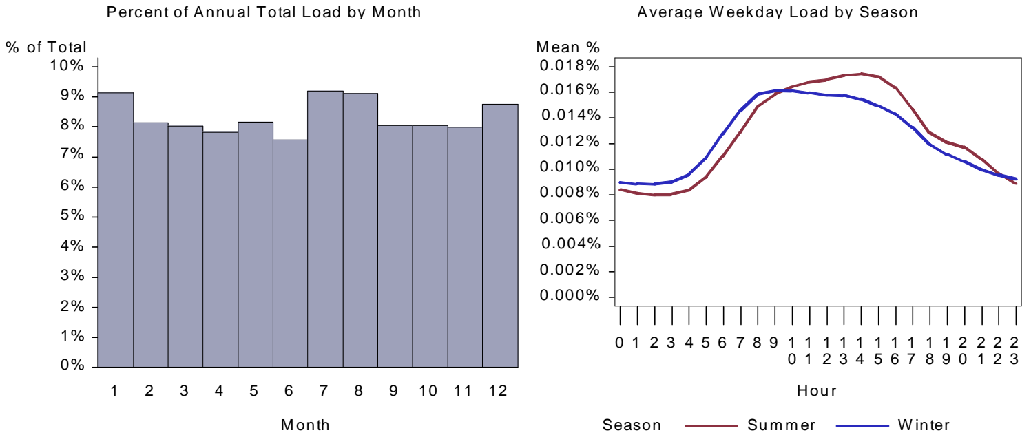
Figure 251. : CA Warehouse Plug Load Load by Month and Average Weekday
