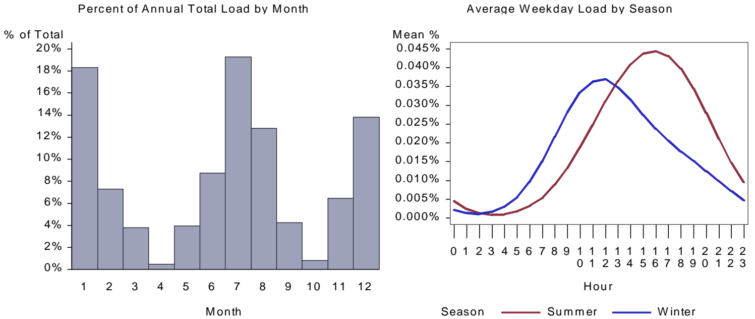
Figure 107. : WA Warehouse CA HVAC Aux Load by Month and Average Weekday
