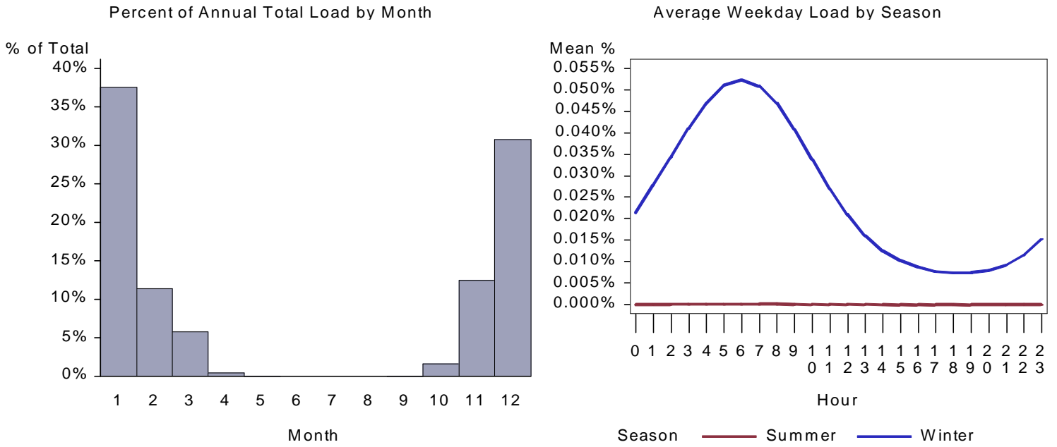
Figure 395. : WA Restaurant Space Heat Load by Month and Average Weekday
