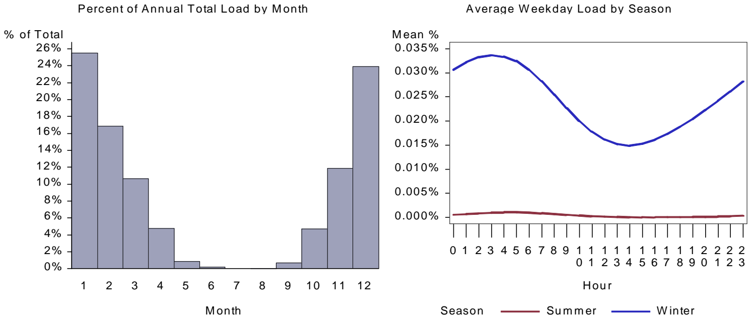
Figure 383. : ID Lodging Space Heat Load by Month and Average Weekday
