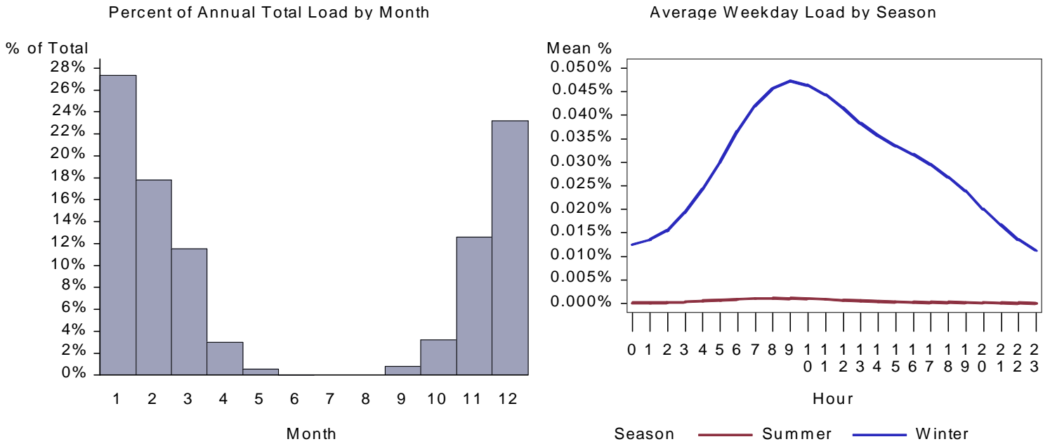
Figure 391. : WY Miscellaneous Space Heat Load by Month and Average Weekday
