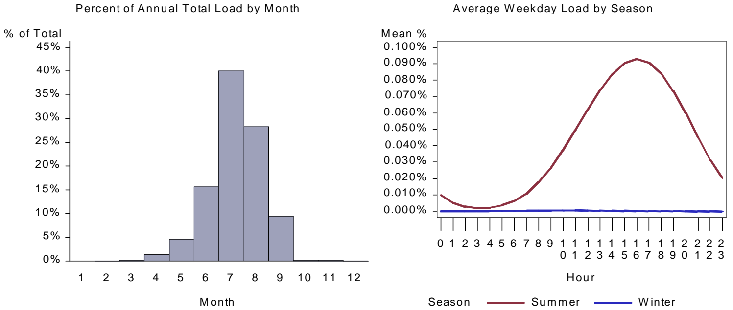
Figure 357. : ID Warehouse Space Cool Load by Month and Average Weekday
