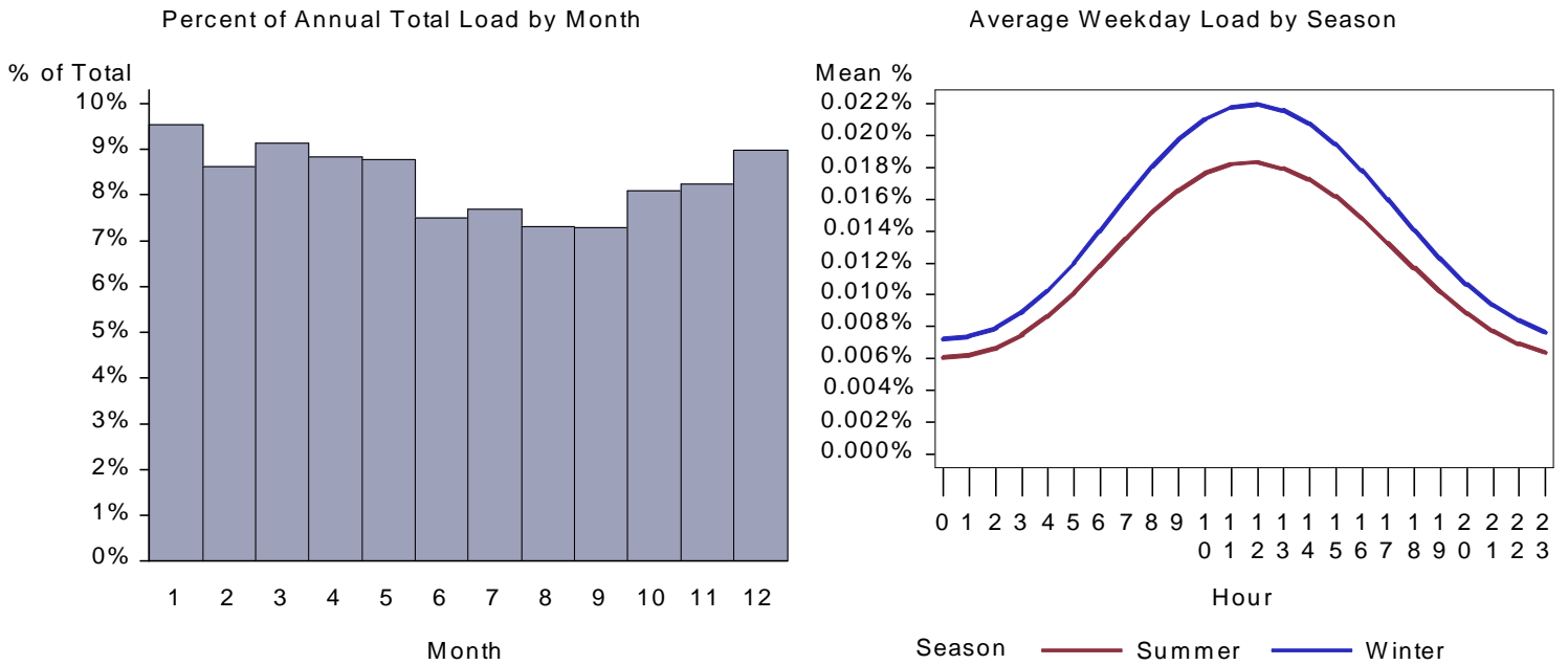
Figure 10. WY Health Cooking Load by Month and Average Weekday
