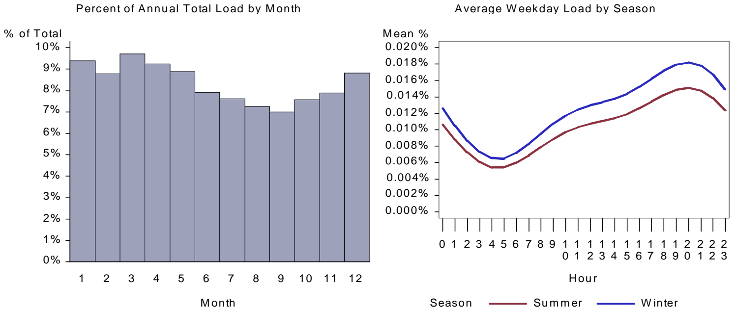
Figure 449. : ID Restaurant Water Heat Load by Month and Average Weekday
