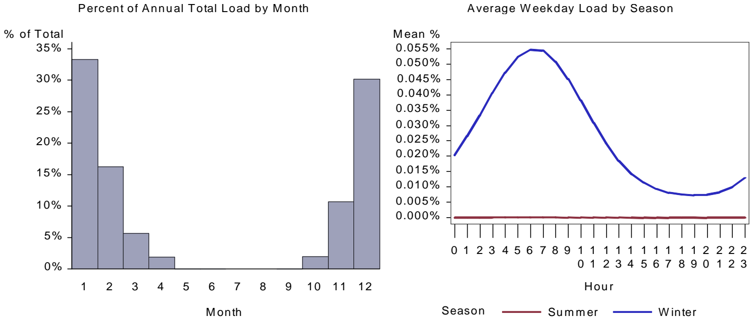
Figure 394. : UT Restaurant Space Heat Load by Month and Average Weekday
