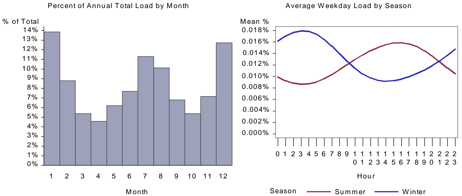
Figure 74. UT Lodging HVAC Aux Load by Month and Average Weekday
