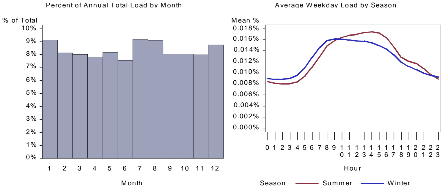
Figure 243. : UT Small Office Plug Load Load by Month and Average Weekday
