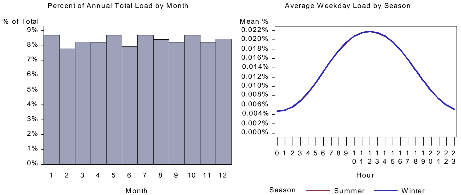
Figure 172. : CA Miscellaneous Lighting Load by Month and Average Weekday
