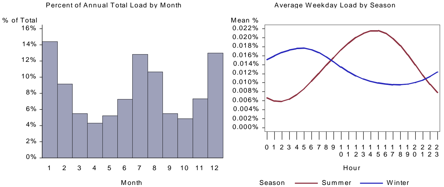
Figure 59. UT Health HVAC Aux Load by Month and Average Weekday
