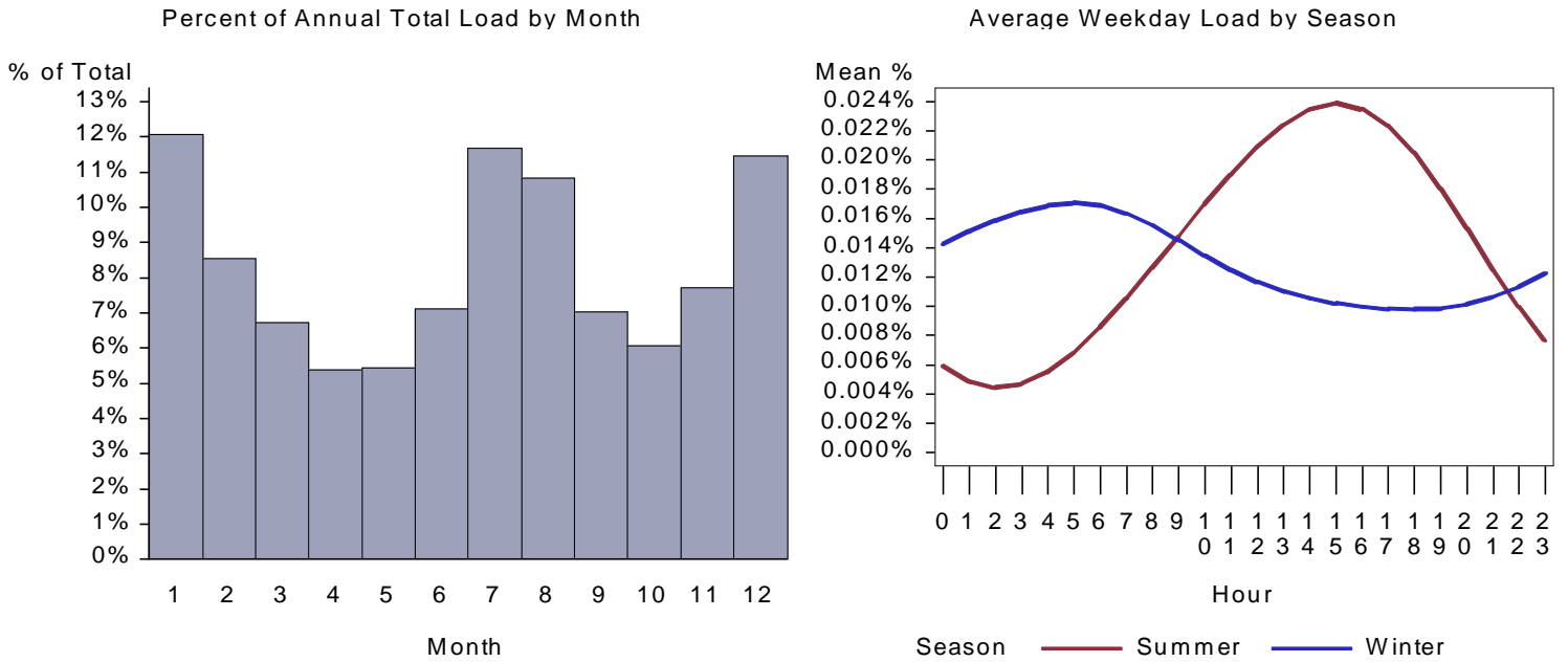
Figure 57. CA Health HVAC Aux Load by Month and Average Weekday
