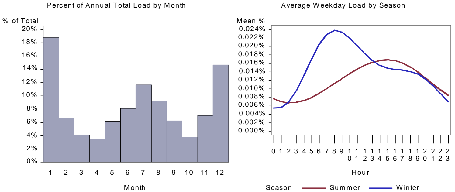
Figure 55. WA Grocery HVAC Aux Load by Month and Average Weekday
