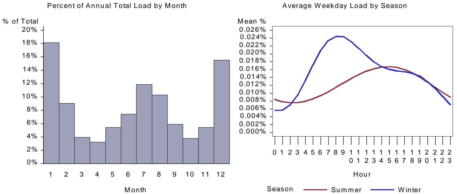
Figure 54. UT Grocery HVAC Aux Load by Month and Average Weekday
