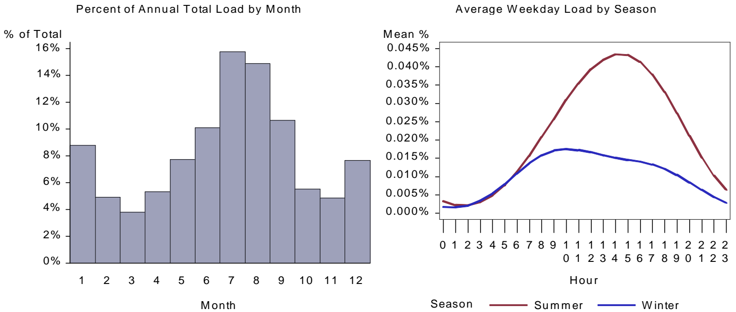
Figure 142. : CA Small Retail Heat Pump Load by Month and Average Weekday
