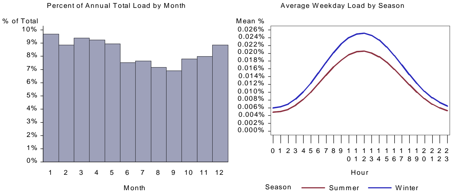
Figure 12. ID Large Office Cooking Load by Month and Average Weekday
