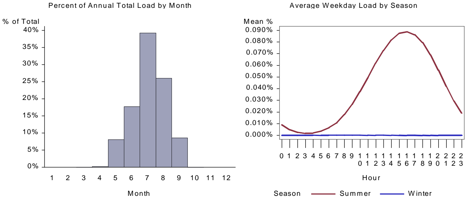
Figure 359. : WA Warehouse Space Cool Load by Month and Average Weekday
