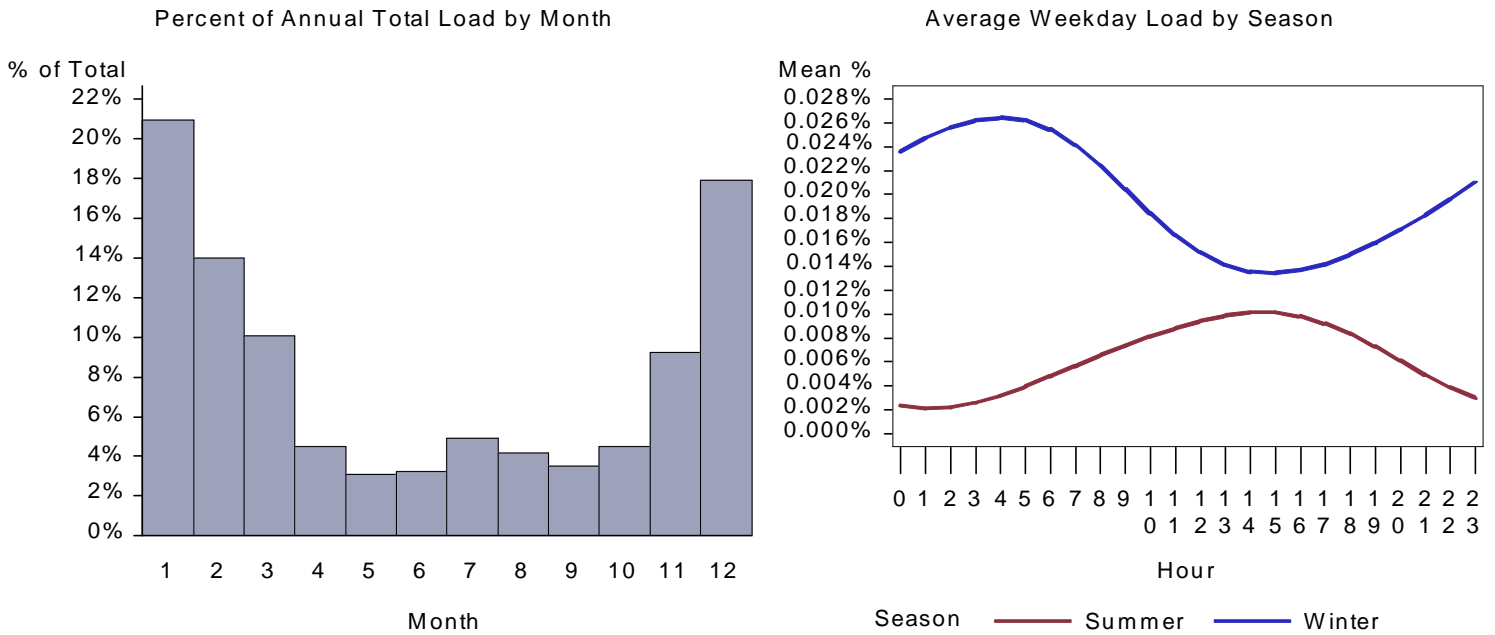
Figure 116. : WY Health Heat Pump Load by Month and Average Weekday
