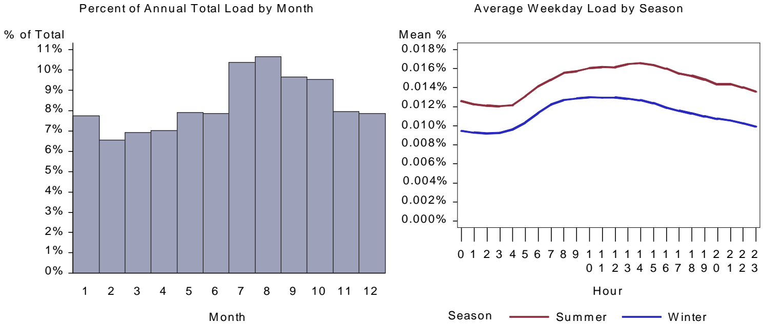
Figure 278. : WA Lodging Refrigeration Load by Month and Average Weekday
