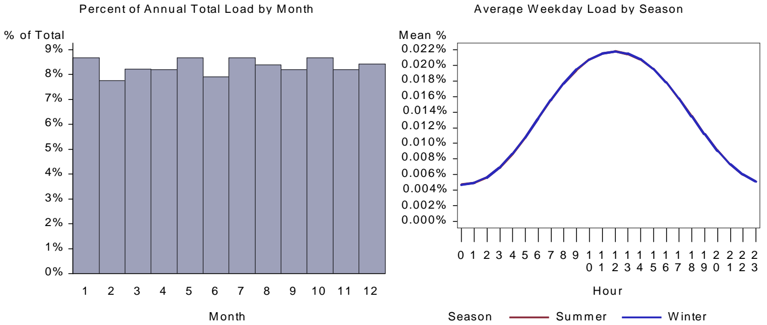
Figure 173. : ID Miscellaneous Lighting Load by Month and Average Weekday
