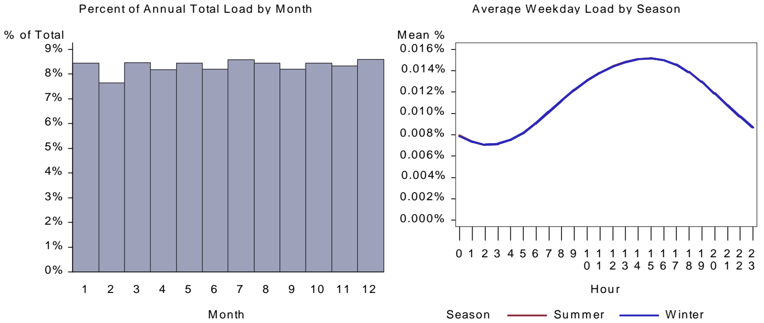
Figure 149. : UT Grocery Lighting Load by Month and Average Weekday
