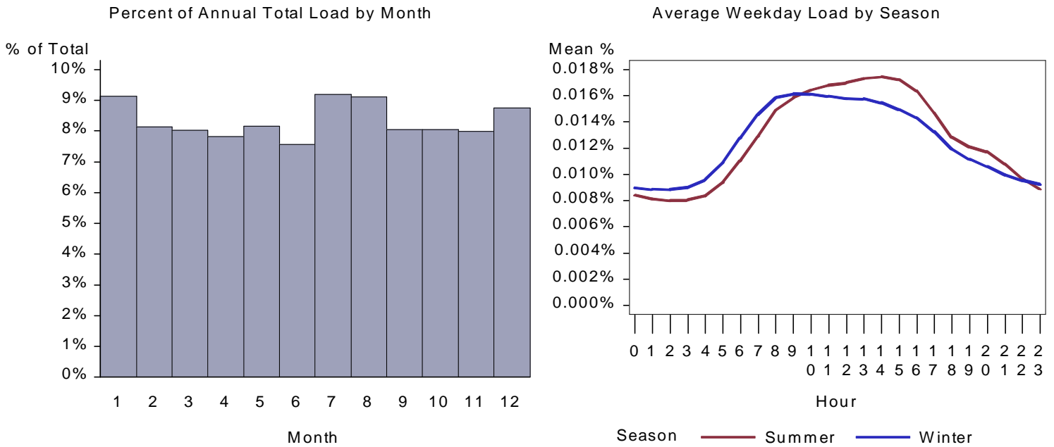
Figure 226. : CA Miscellaneous Plug Load Load by Month and Average Weekday
