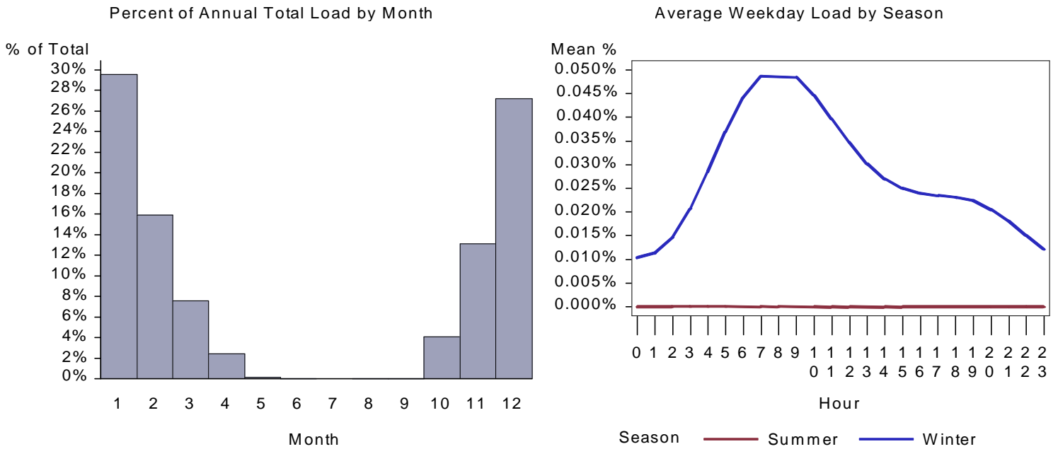
Figure 362. : CA Grocery Space Heat Load by Month and Average Weekday
