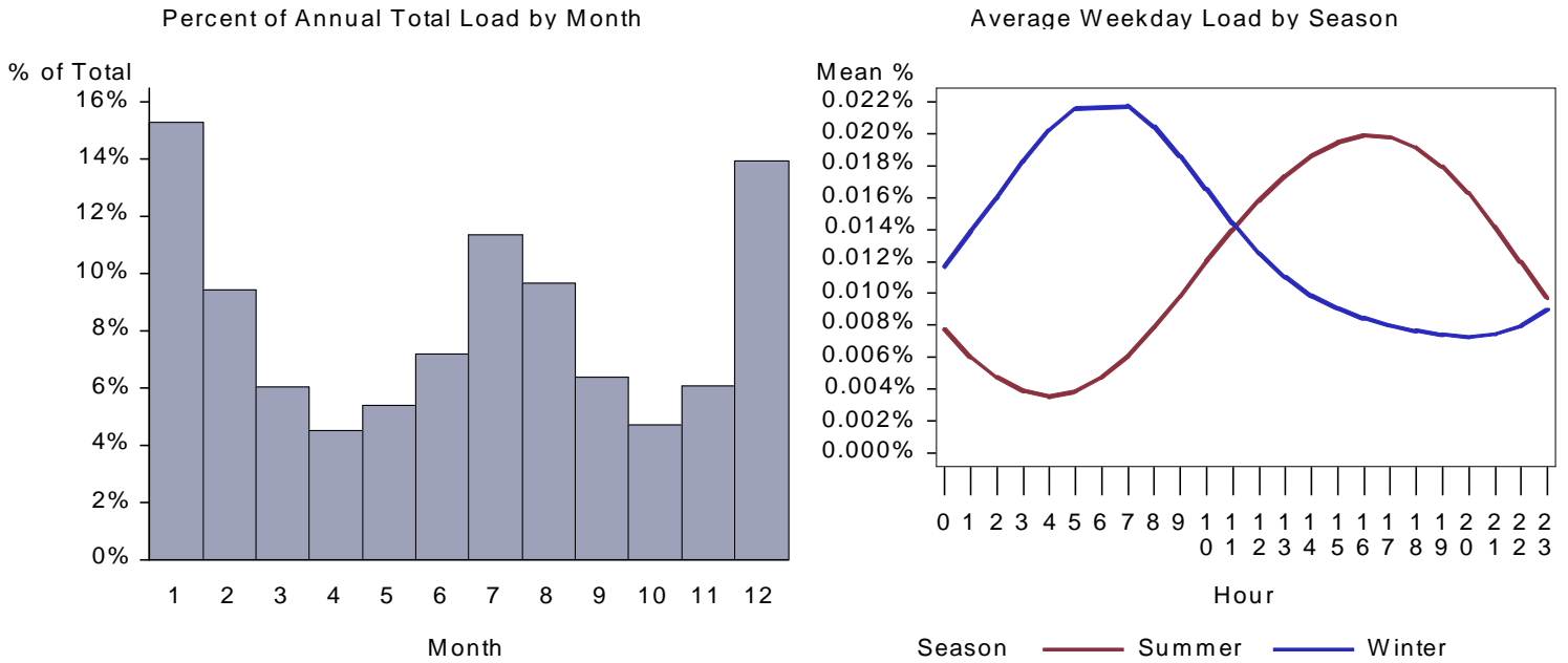
Figure 83. ID Restaurant HVAC Aux Load by Month and Average Weekday
