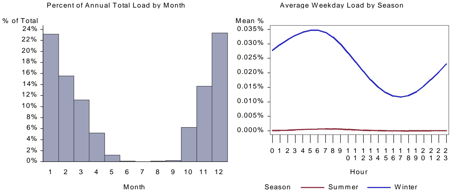
Figure 397. : CA School Space Heat Load by Month and Average Weekday
