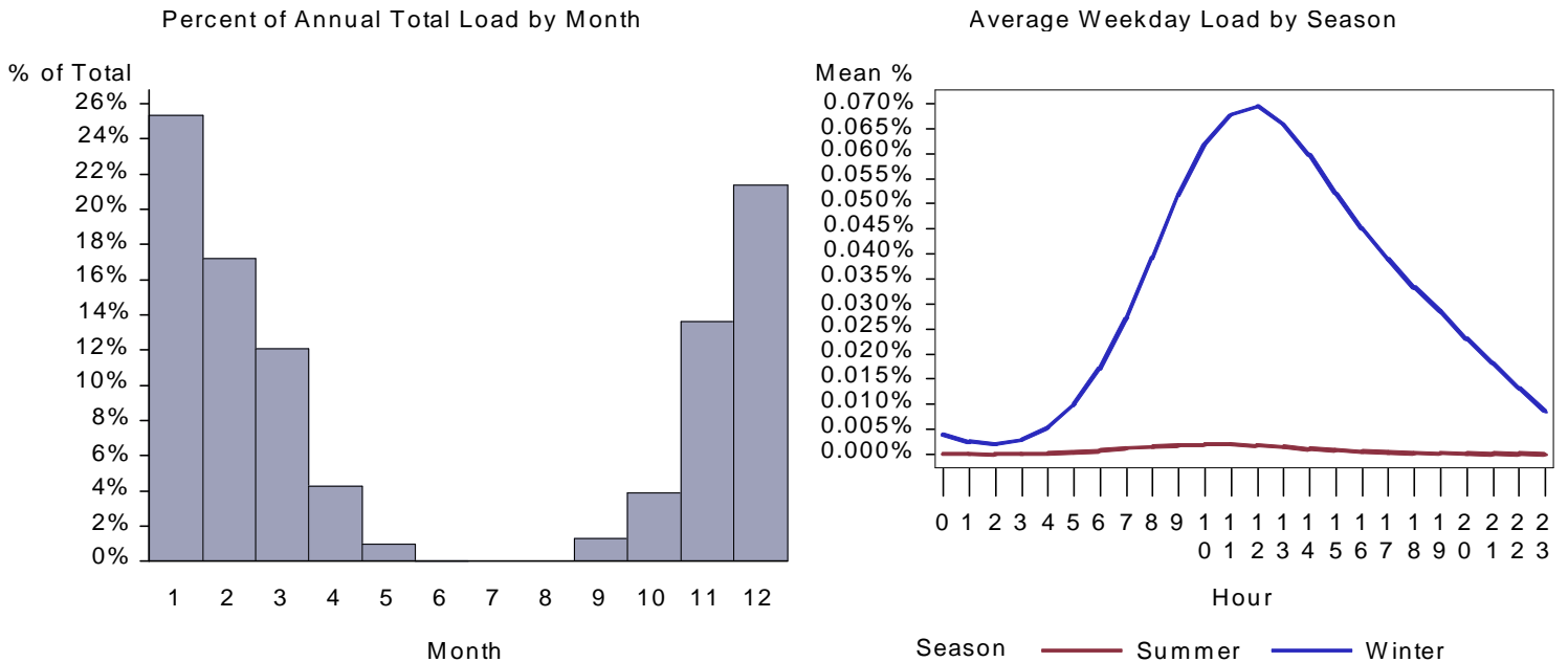
Figure 416. : WY Warehouse Space Heat Load by Month and Average Weekday
