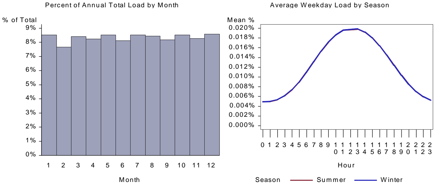
Figure 163. : ID Large Retail Lighting Load by Month and Average Weekday
