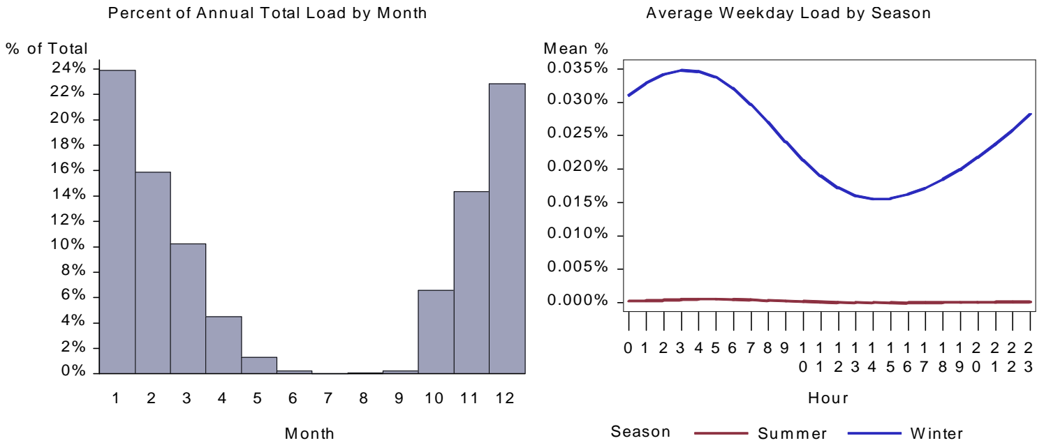
Figure 382. : CA Lodging Space Heat Load by Month and Average Weekday
