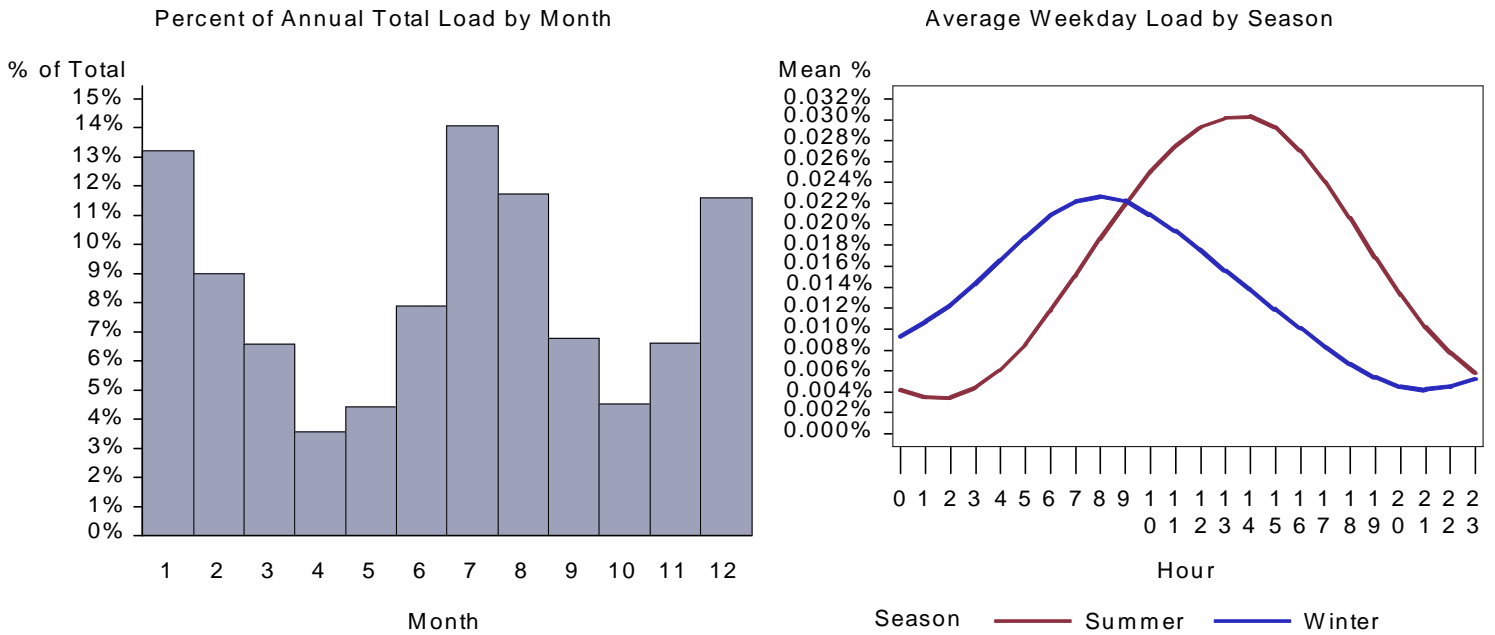
Figure 96. WY Small Office HVAC Aux Load by Month and Average Weekday
