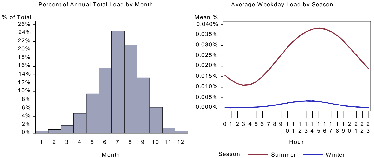
Figure 330. : WY Lodging Space Cool Load by Month and Average Weekday
