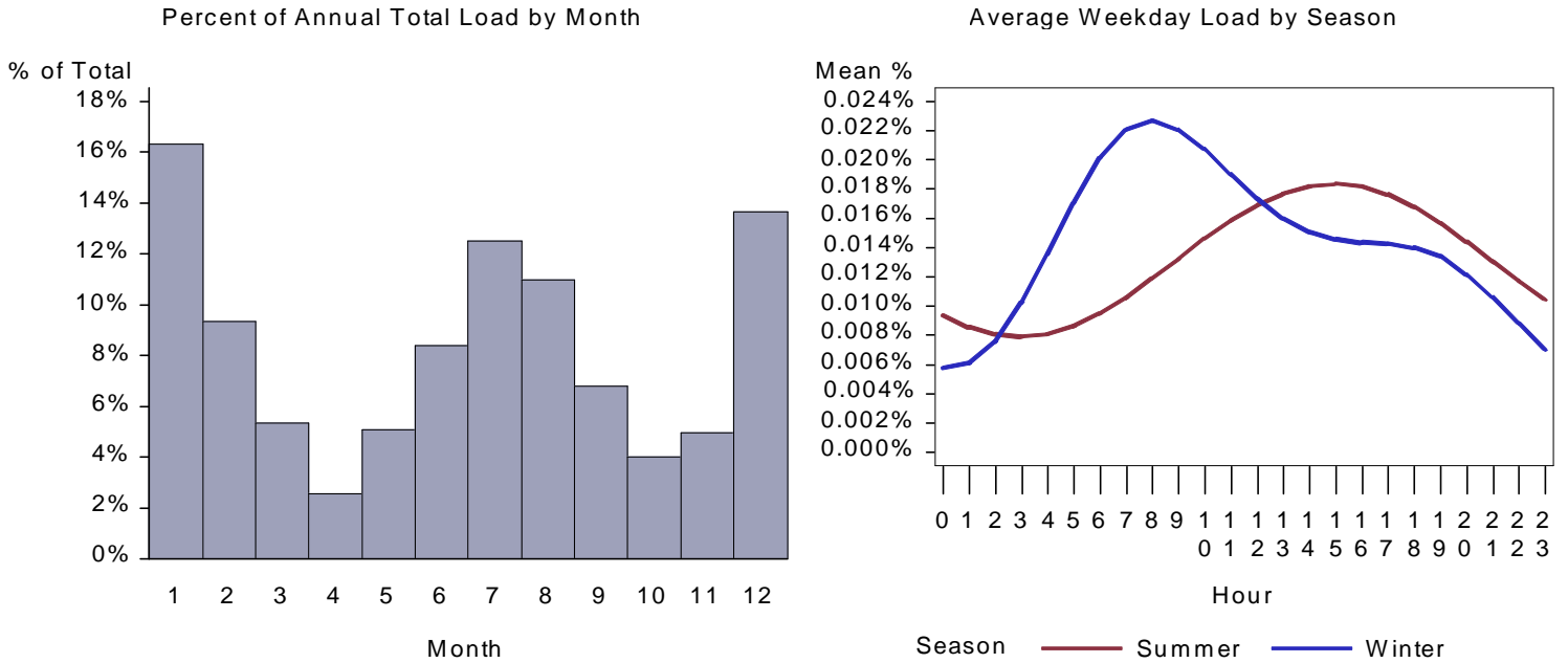
Figure 56. WY Grocery HVAC Aux Load by Month and Average Weekday
