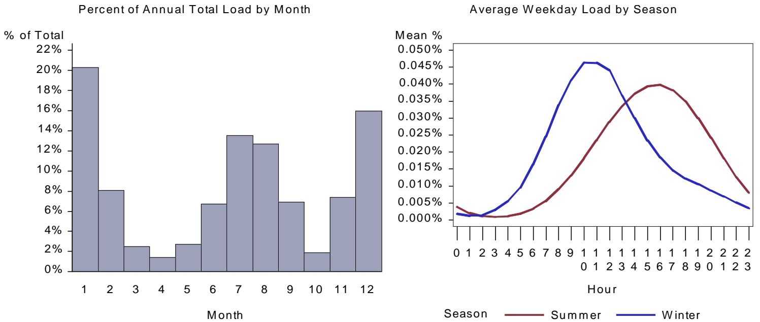
Figure 146. : CA Warehouse Heat Pump Load by Month and Average Weekday
