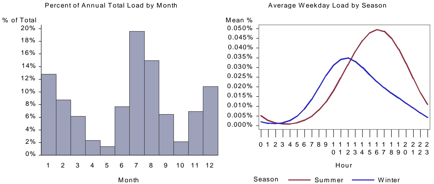
Figure 106. : WY Warehouse HVAC Aux Load by Month and Average Weekday
