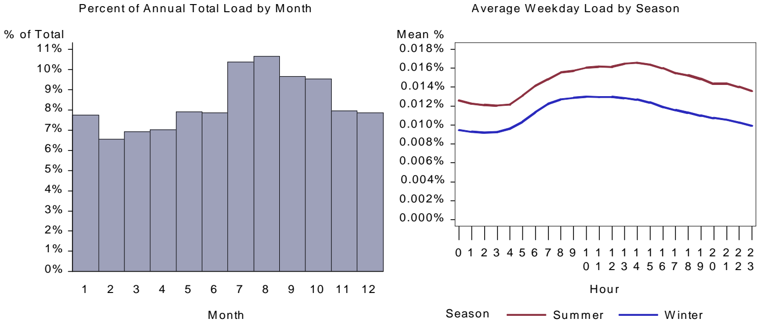
Figure 270. : WY Large Office Refrigeration Load by Month and Average Weekday
