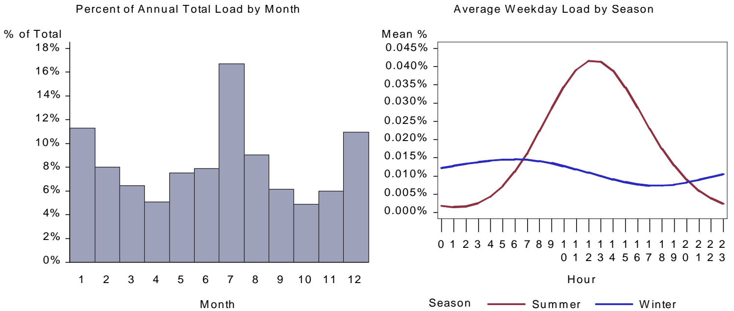
Figure 88. ID School HVAC Aux Load by Month and Average Weekday
