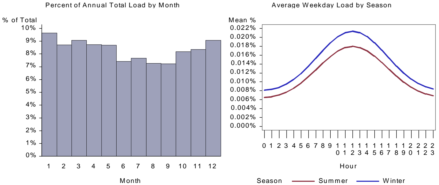
Figure 443. : CA Miscellaneous Water Heat Load by Month and Average Weekday
