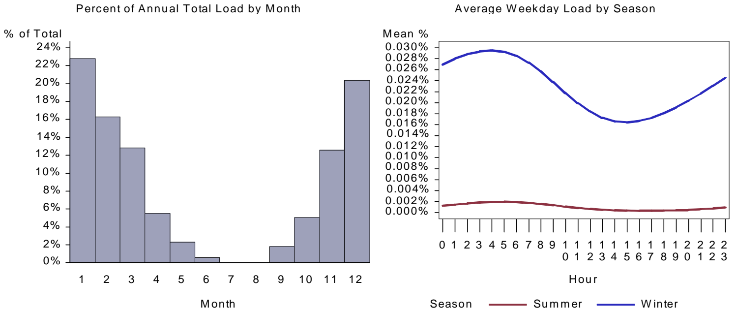
Figure 371. : WY Health Space Heat Load by Month and Average Weekday
