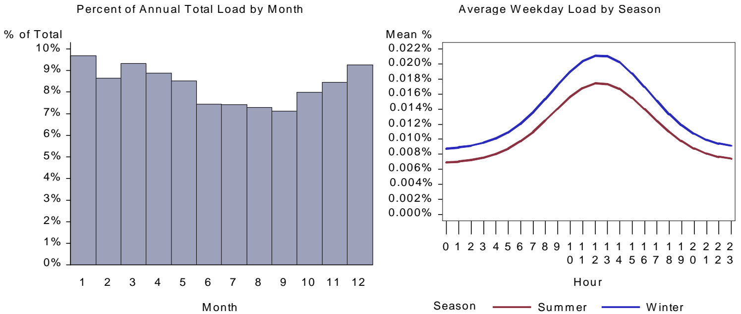
Figure 44. WA Small Retail Cooking Load by Month and Average Weekday
