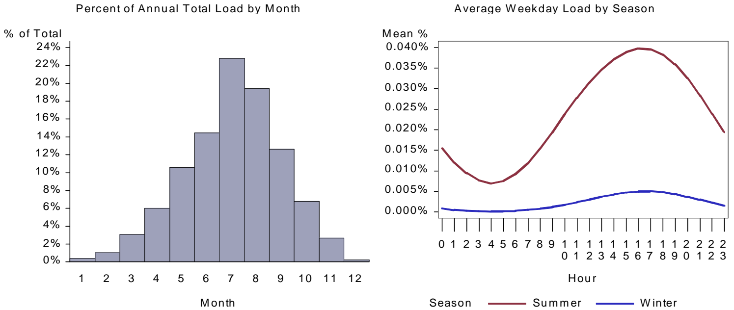
Figure 337. : ID Restaurant Space Cool Load by Month and Average Weekday
