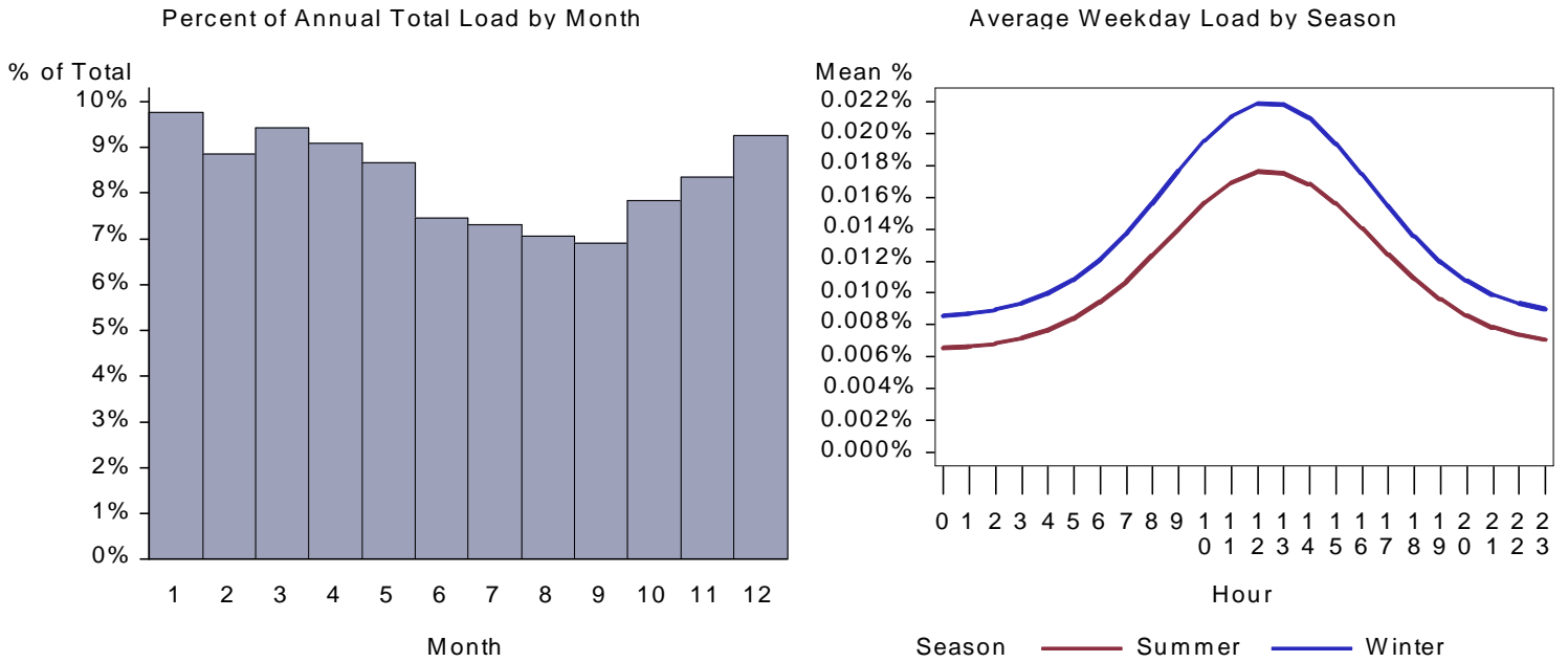
Figure 435. : UT Large Retail Water Heat Load by Month and Average Weekday
