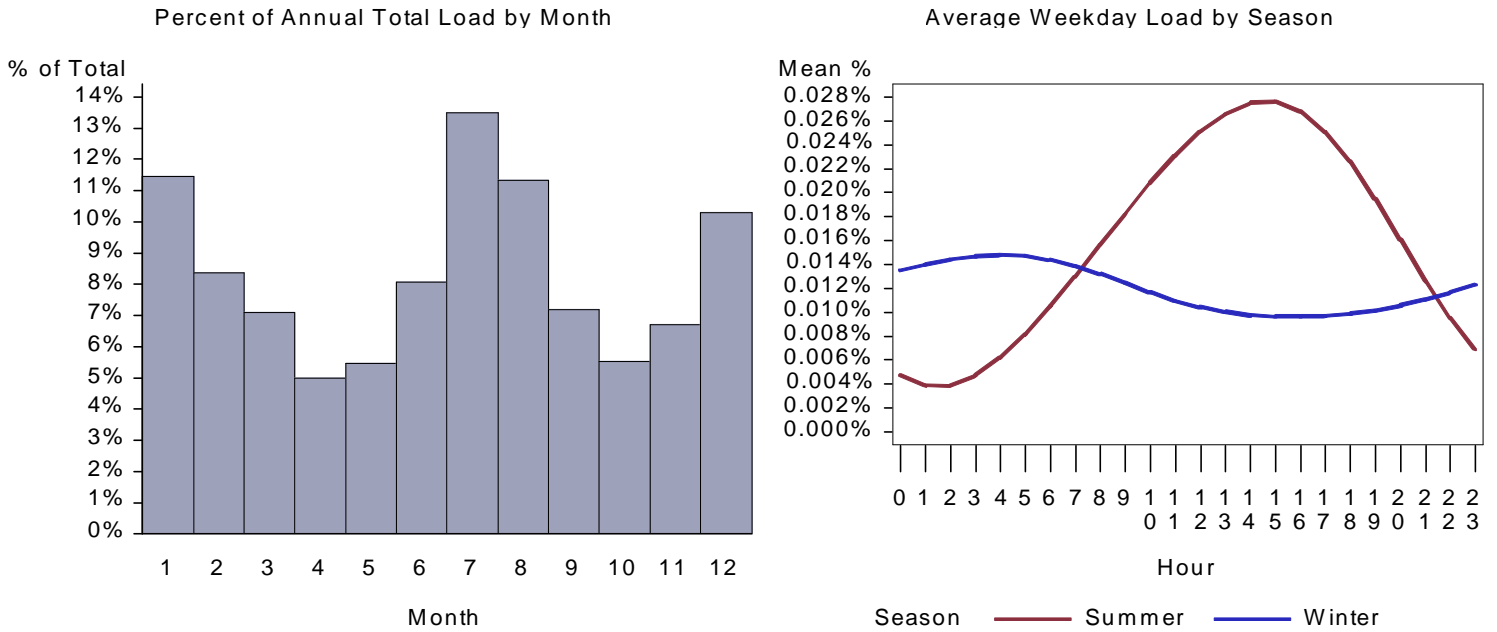
Figure 61. WY Health HVAC Aux Load by Month and Average Weekday
