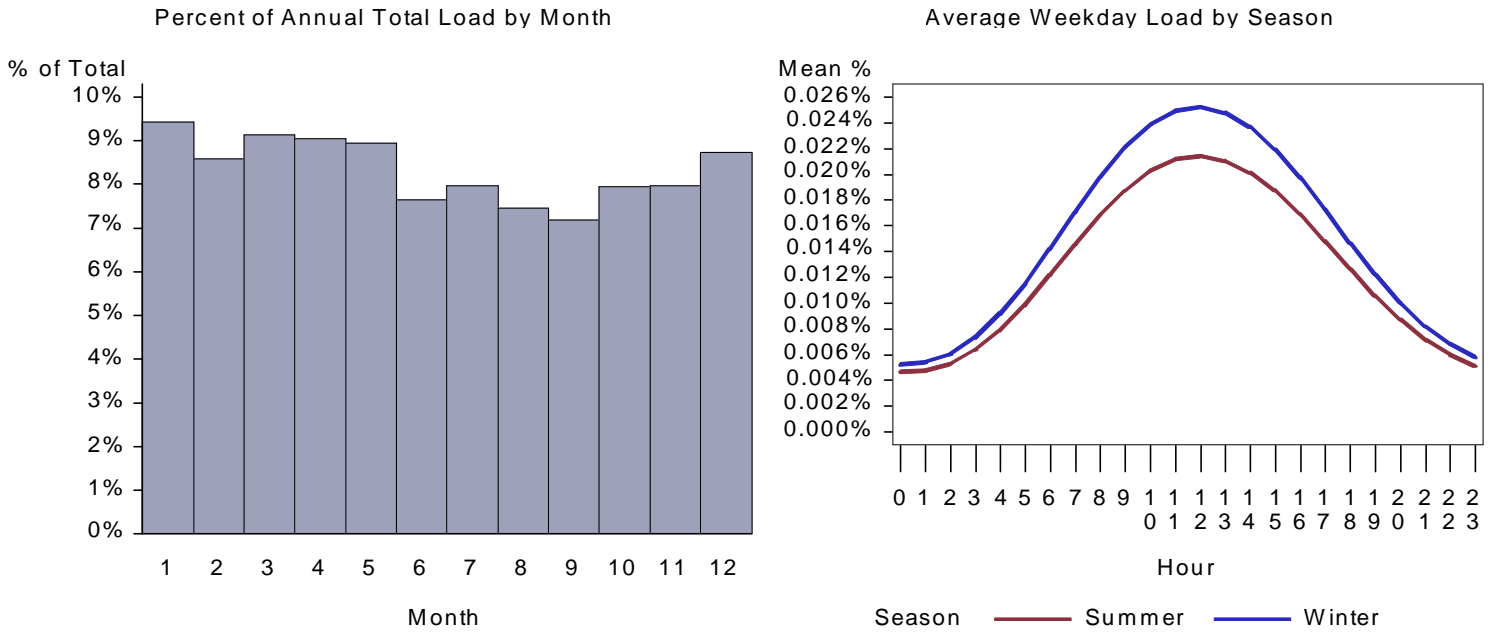
Figure 9. WA Health Cooking Load by Month and Average Weekday
