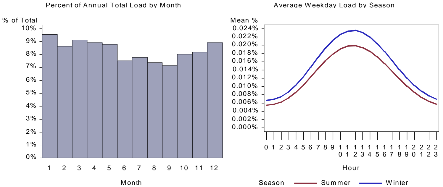
Figure 11. CA Large Office Cooking Load by Month and Average Weekday
