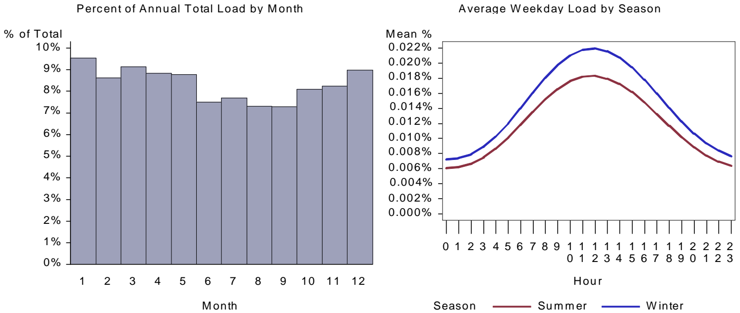
Figure 427. : WY Health Water Heat Load by Month and Average Weekday
