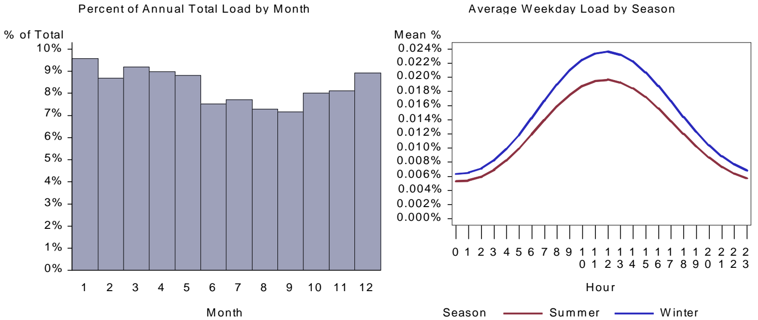
Figure 7. ID Health Cooking Load by Month and Average Weekday
