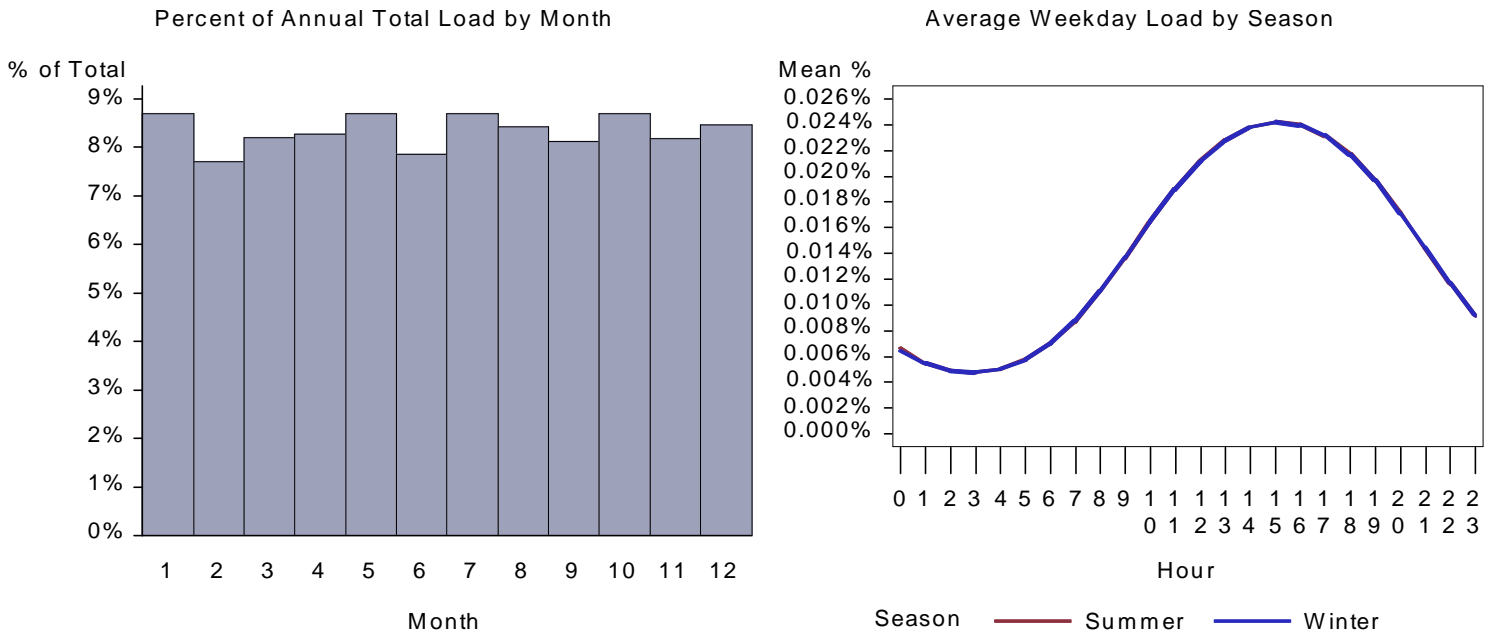
Figure 202. : WA Warehouse CA Lighting Load by Month and Average Weekday
