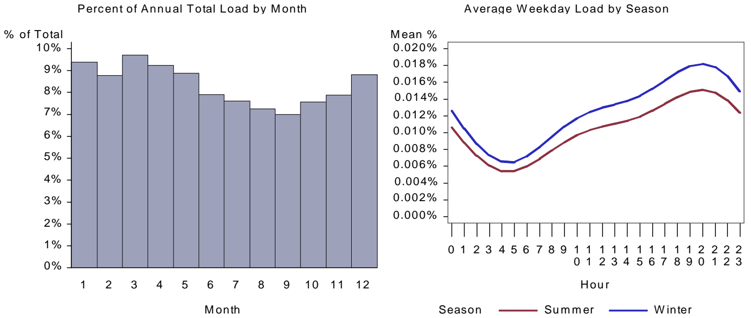
Figure 27. ID Restaurant Cooking Load by Month and Average Weekday
