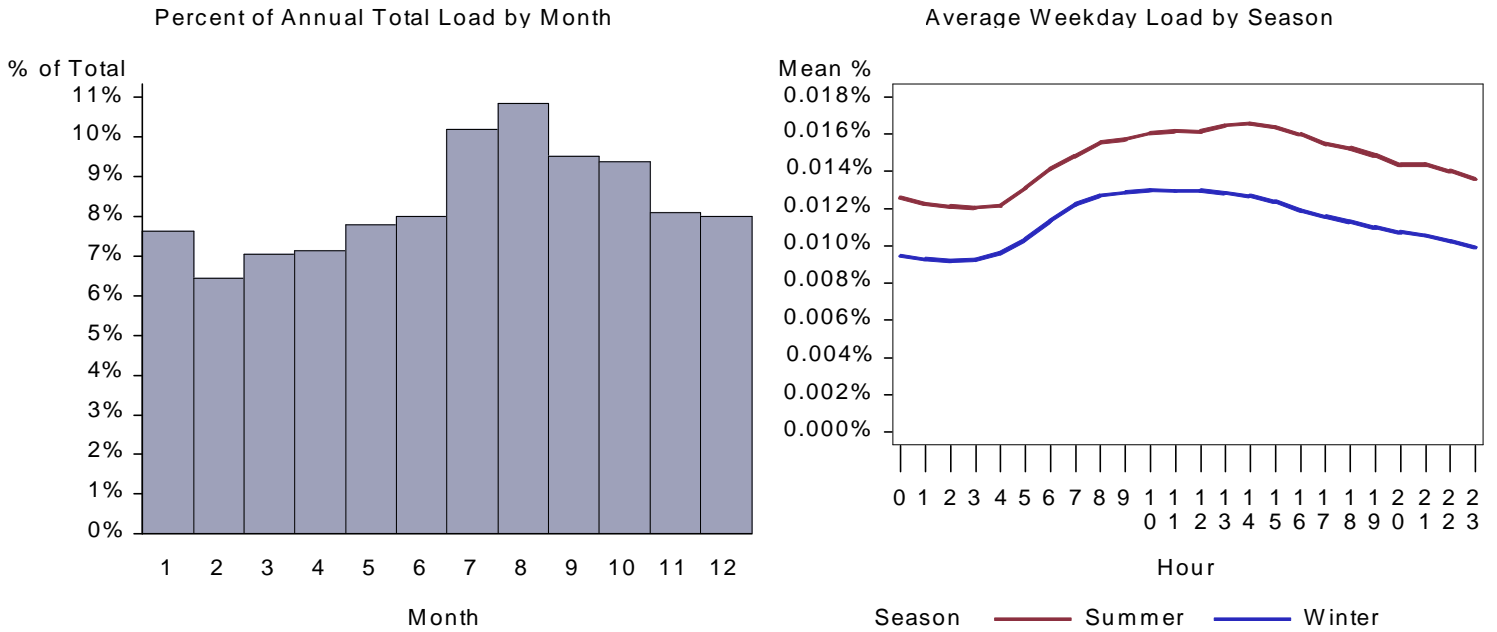
Figure 283. : WA Restaurant Refrigeration Load by Month and Average Weekday
