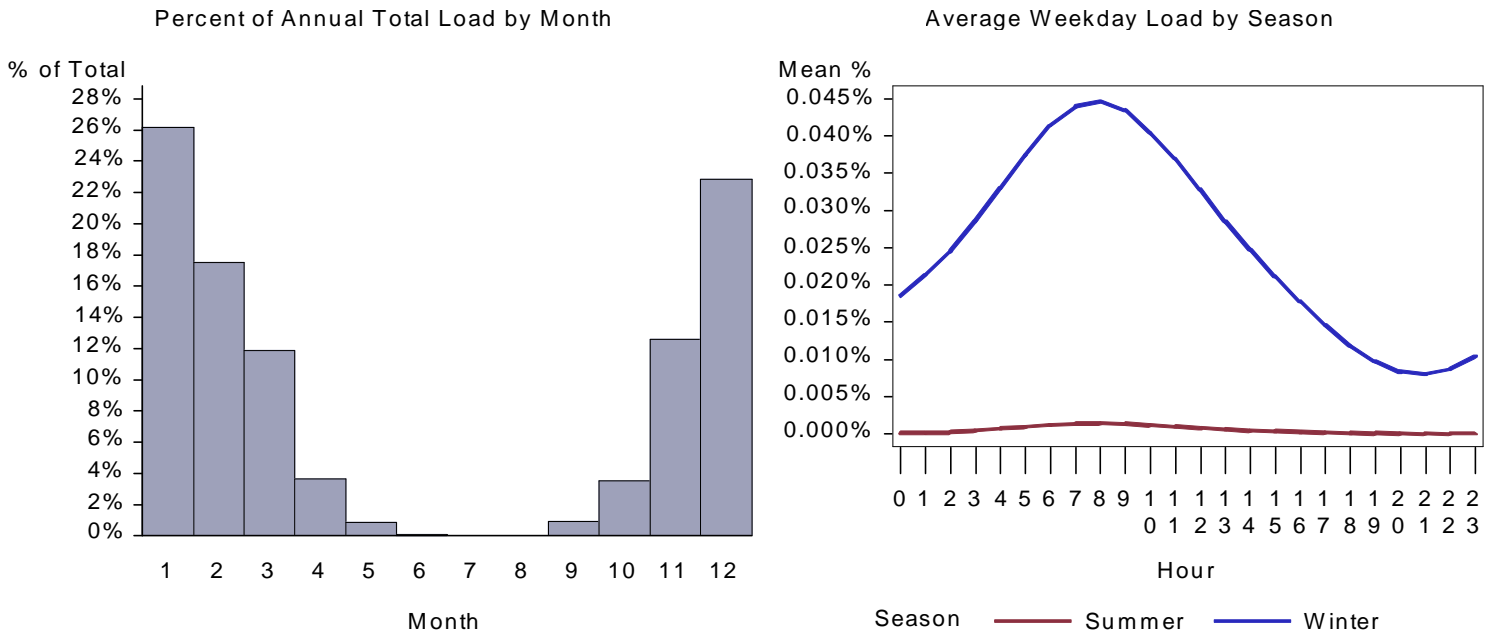
Figure 406. : WY Small Office Space Heat Load by Month and Average Weekday
