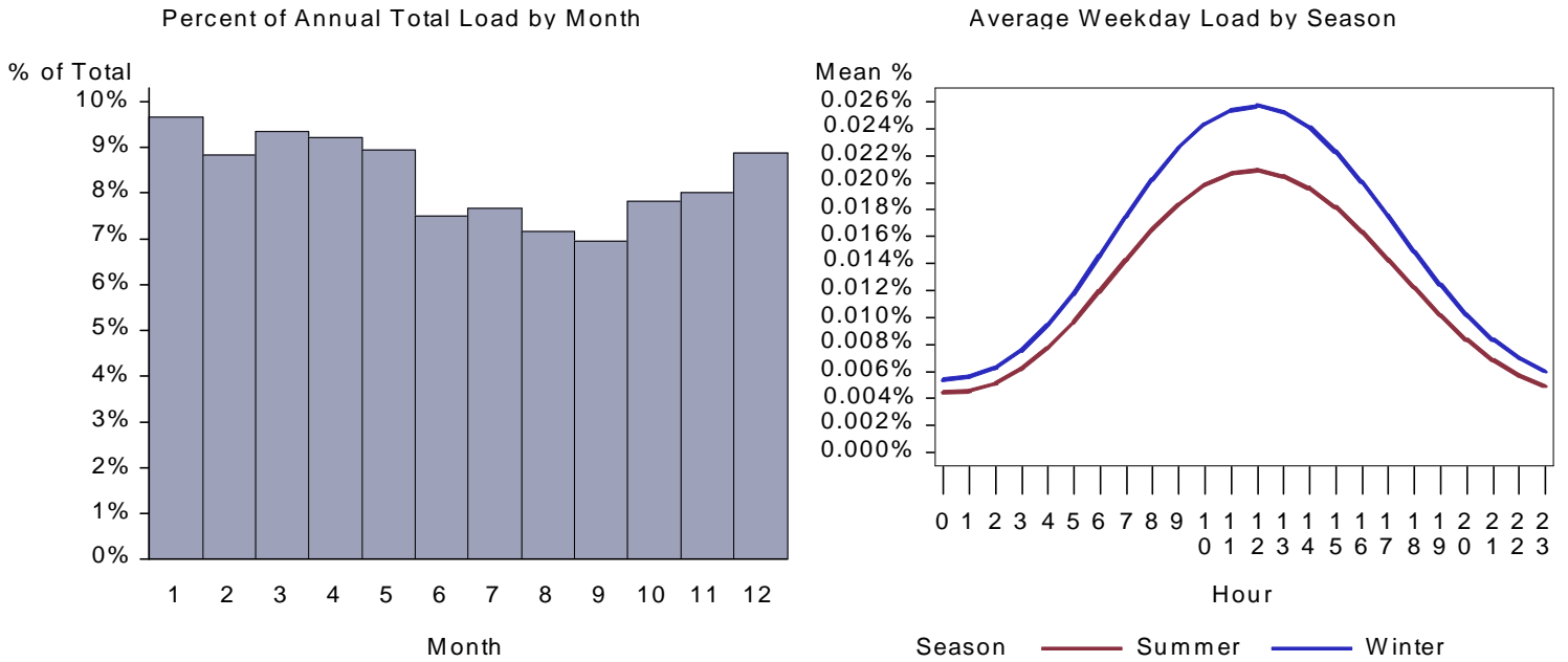
Figure 425. : UT Health Water Heat Load by Month and Average Weekday
