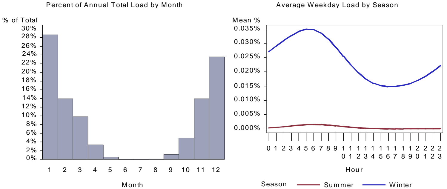
Figure 370. : WA Health Space Heat Load by Month and Average Weekday
