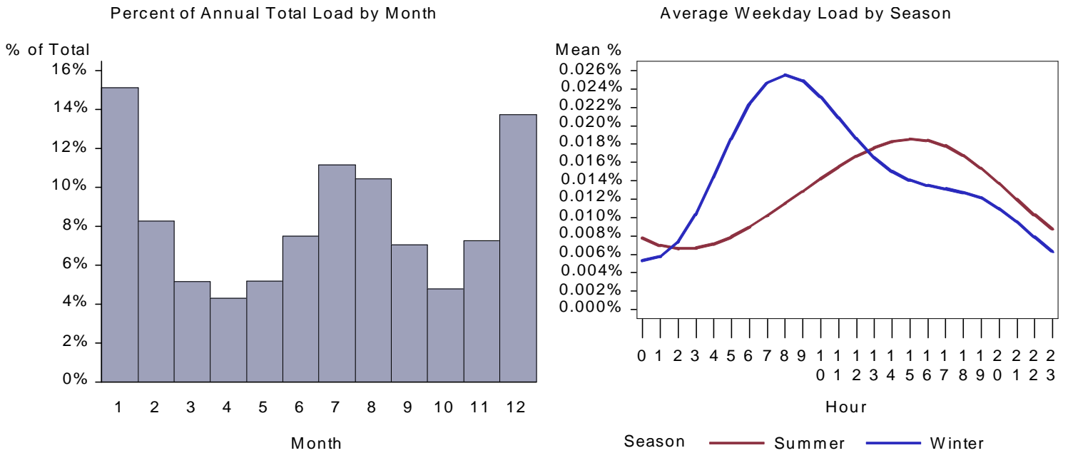
Figure 52. CA Grocery HVAC Aux Load by Month and Average Weekday
