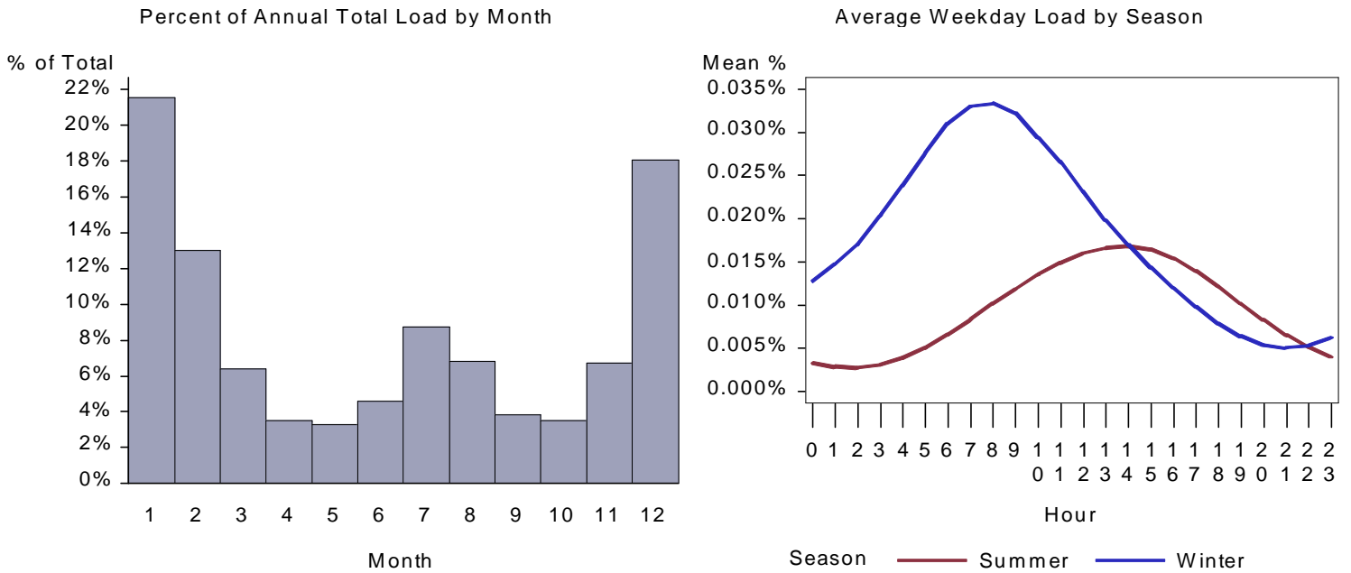
Figure 118. : ID Large Office Heat Pump Load by Month and Average Weekday
