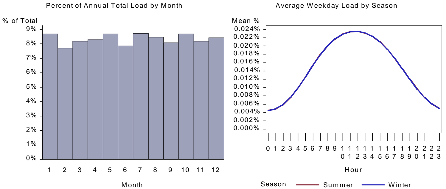
Figure 158. : ID Large Office Lighting Load by Month and Average Weekday
