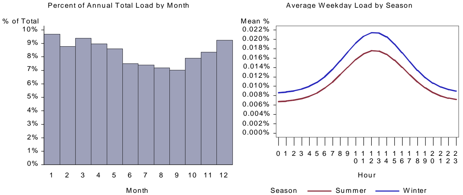
Figure 17. ID Large Retail Cooking Load by Month and Average Weekday
