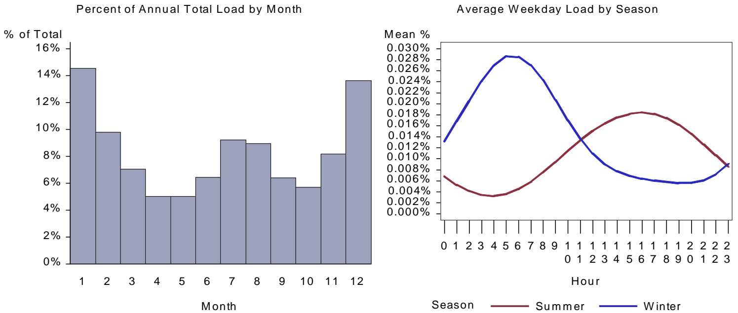
Figure 82. CA Restaurant HVAC Aux Load by Month and Average Weekday
