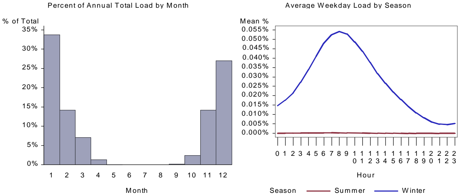
Figure 375. : WA Large Office Space Heat Load by Month and Average Weekday
