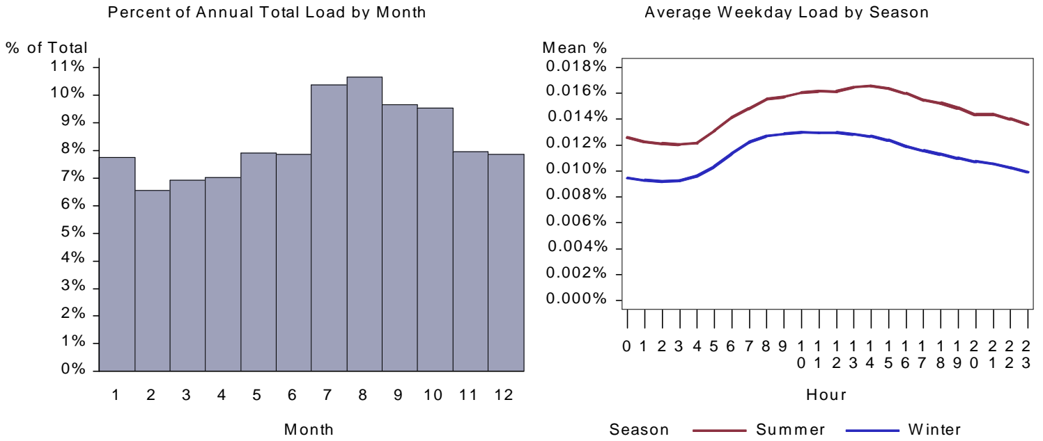
Figure 291. : ID Small Office Refrigeration Load by Month and Average Weekday
