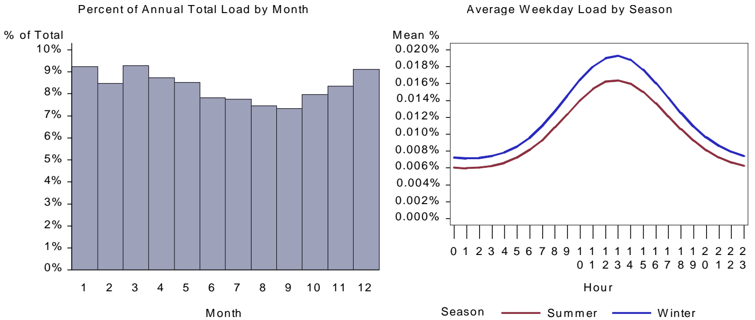
Figure 418.: CA Grocery Water Heat Load by Month and Average Weekday
