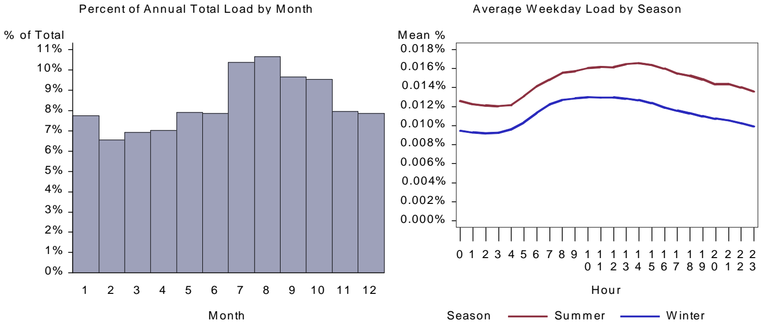
Figure 289. : WY School Refrigeration Load by Month and Average Weekday
