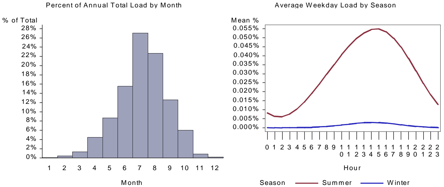
Figure 315.: WY Health Space Cool Load by Month and Average Weekday
