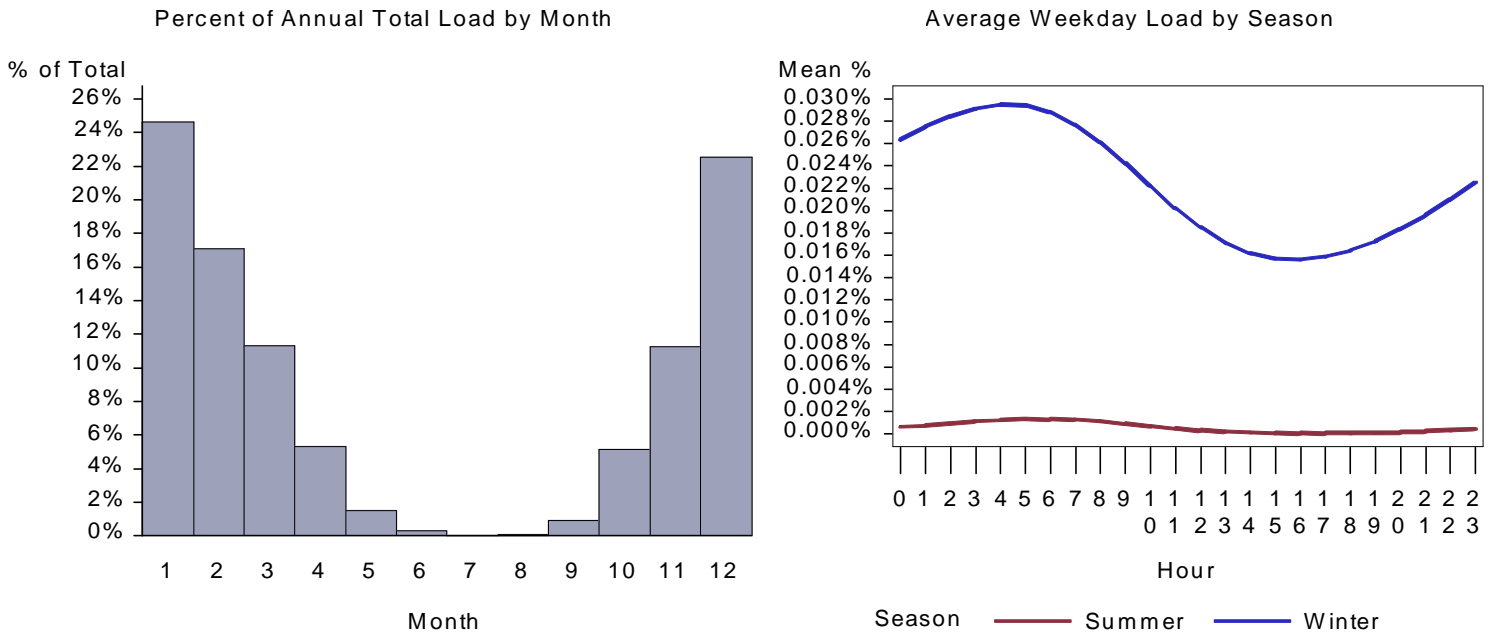
Figure 368.: ID Health Space Heat Load by Month and Average Weekday
