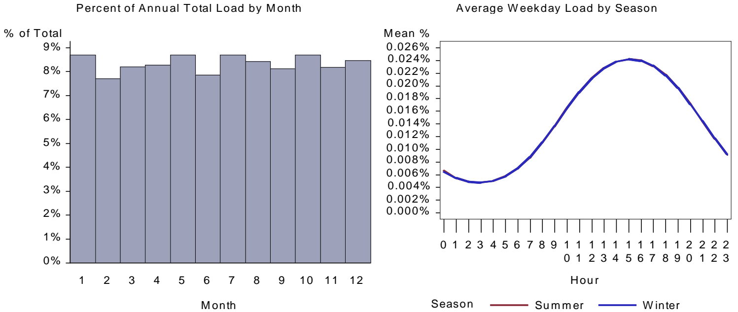
Figure 200. : WA Warehouse Lighting Load by Month and Average Weekday
