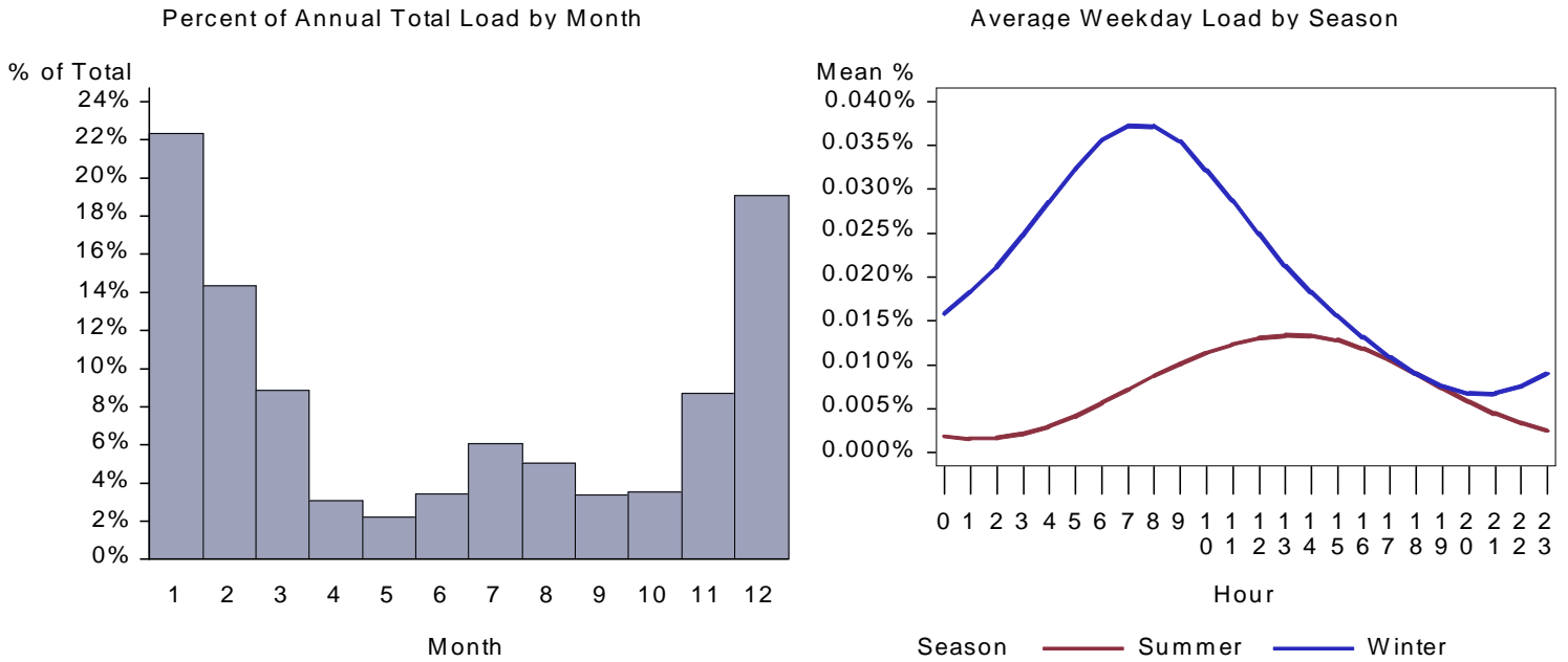
Figure 141. : WY Small Office Heat Pump Load by Month and Average Weekday
