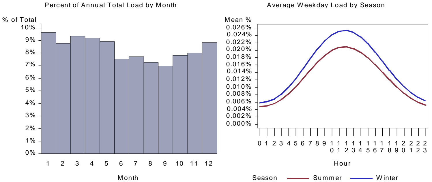
Figure 461. : WA Small Office Water Heat Load by Month and Average Weekday
