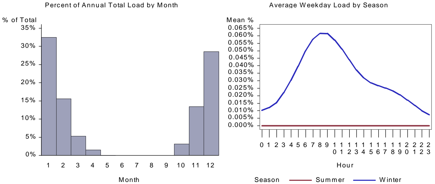
Figure 387. : CA Miscellaneous Space Heat Load by Month and Average Weekday
