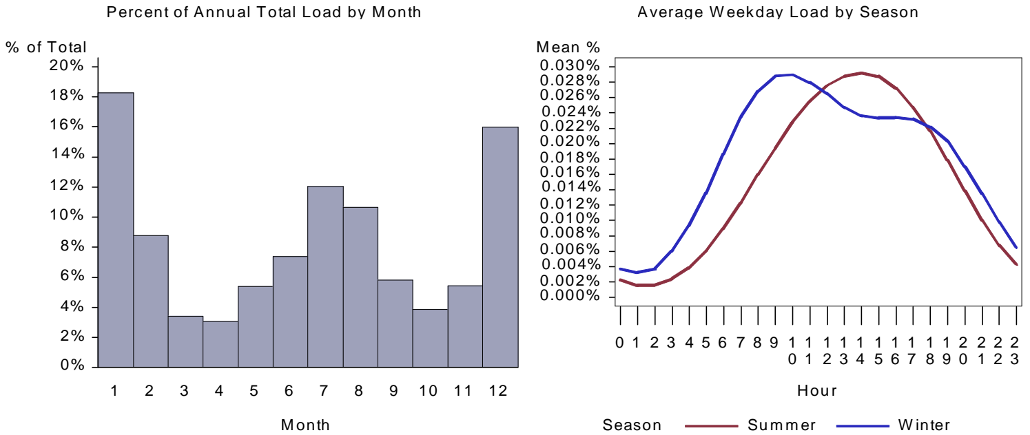
Figure 69. UT Large Retail HVAC Aux Load by Month and Average Weekday
