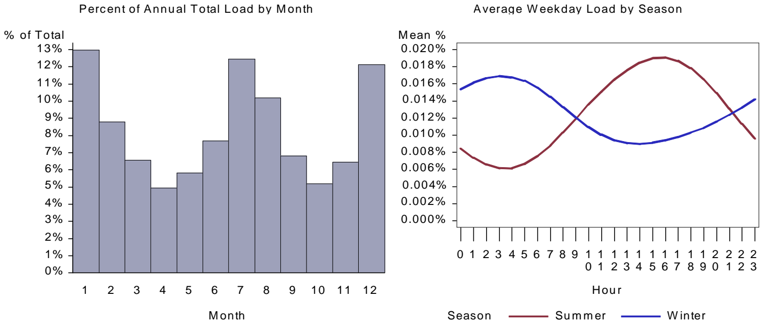
Figure 73. ID Lodging HVAC Aux Load by Month and Average Weekday
