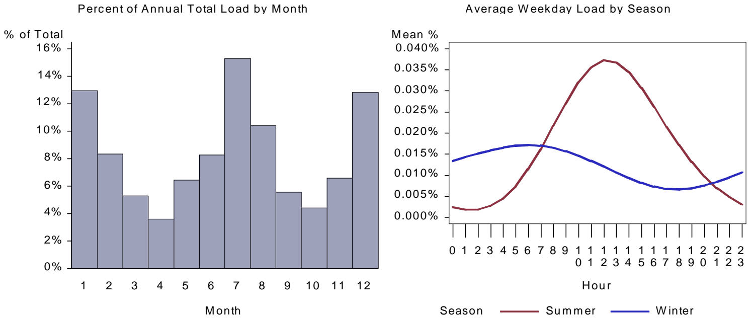
Figure 89. UT School HVAC Aux Load by Month and Average Weekday
