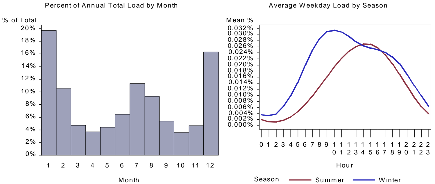
Figure 122. : ID Large Retail Heat Pump Load by Month and Average Weekday
