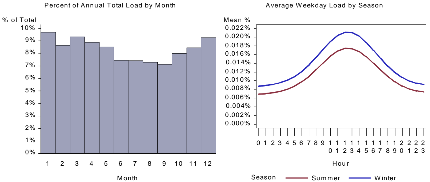
Figure 466. : WA Small Retail Water Heat Load by Month and Average Weekday
