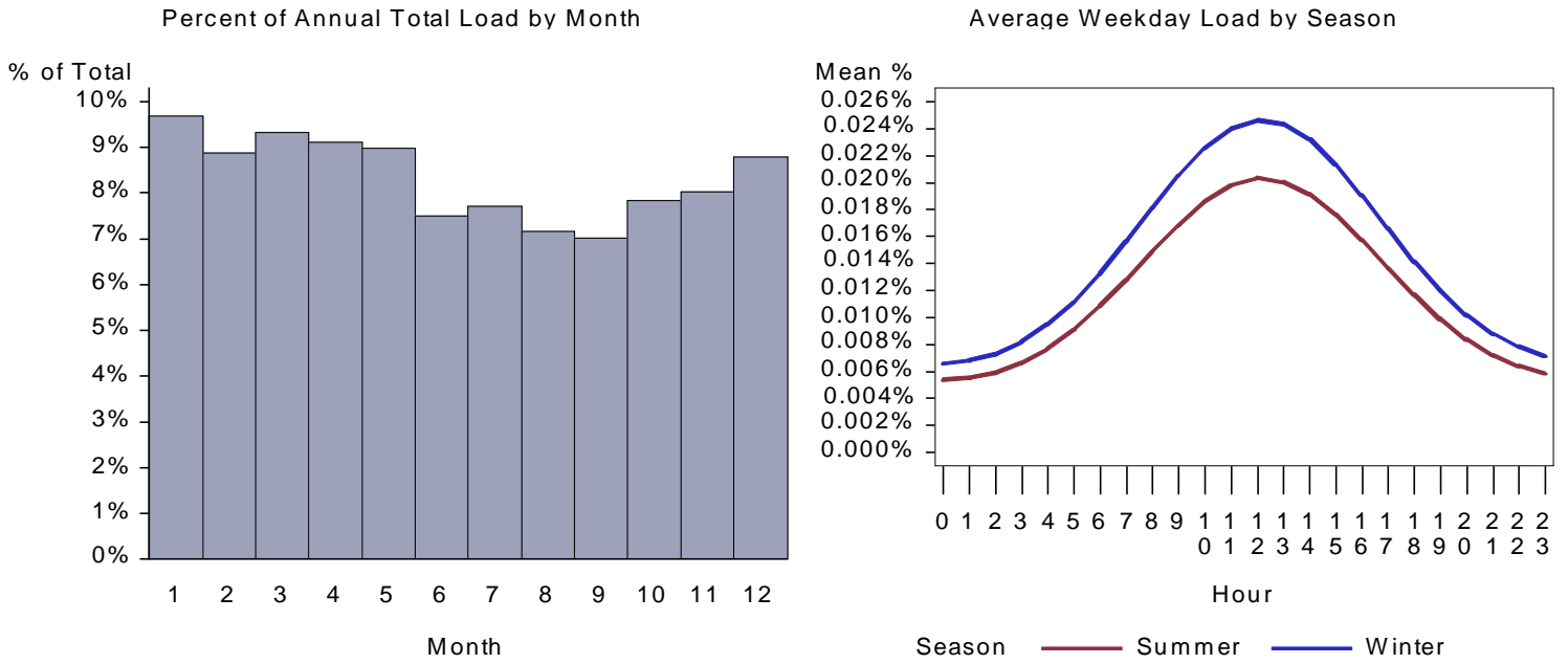
Figure 447. : WY Miscellaneous Water Heat Load by Month and Average Weekday
