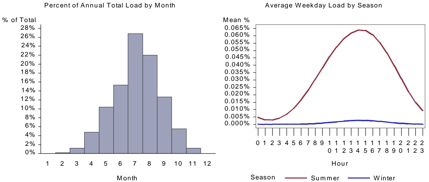
Figure 352. : ID Small Retail Space Cool Load by Month and Average Weekday
