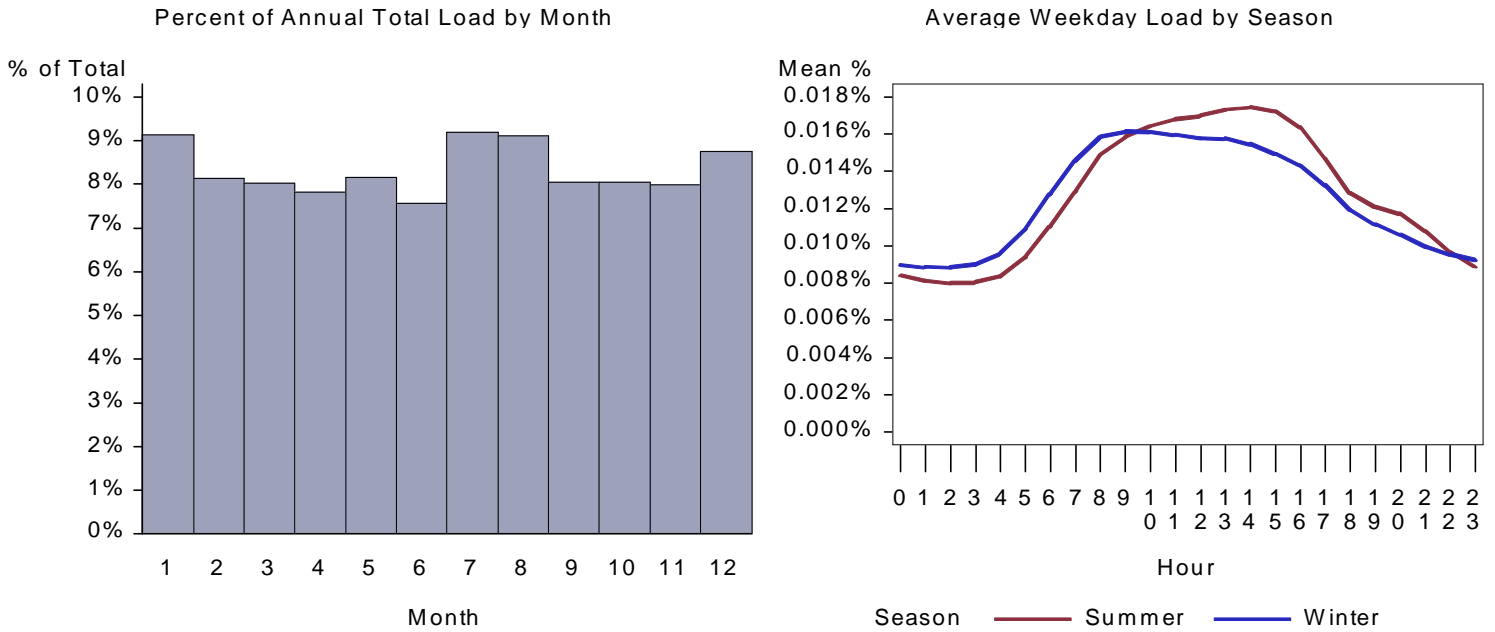
Figure 255. : WY Warehouse Plug Load Load by Month and Average Weekday
