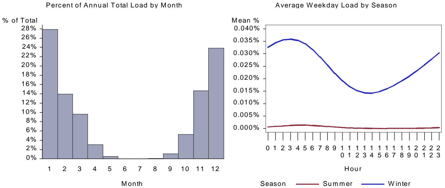
Figure 385. : WA Lodging Space Heat Load by Month and Average Weekday
