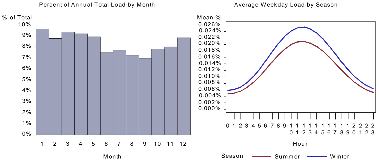
Figure 14. WA Large Office Cooking Load by Month and Average Weekday
