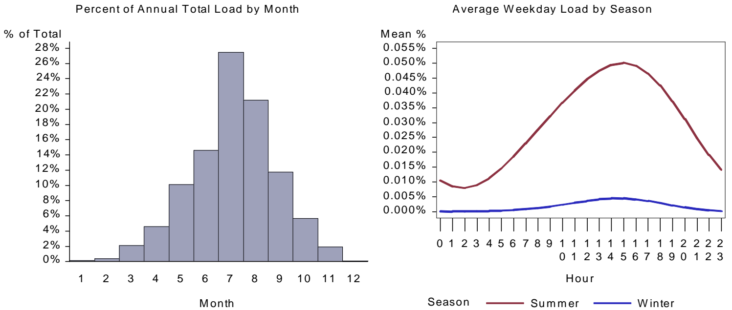
Figure 312. : ID Health Space Cool Load by Month and Average Weekday
