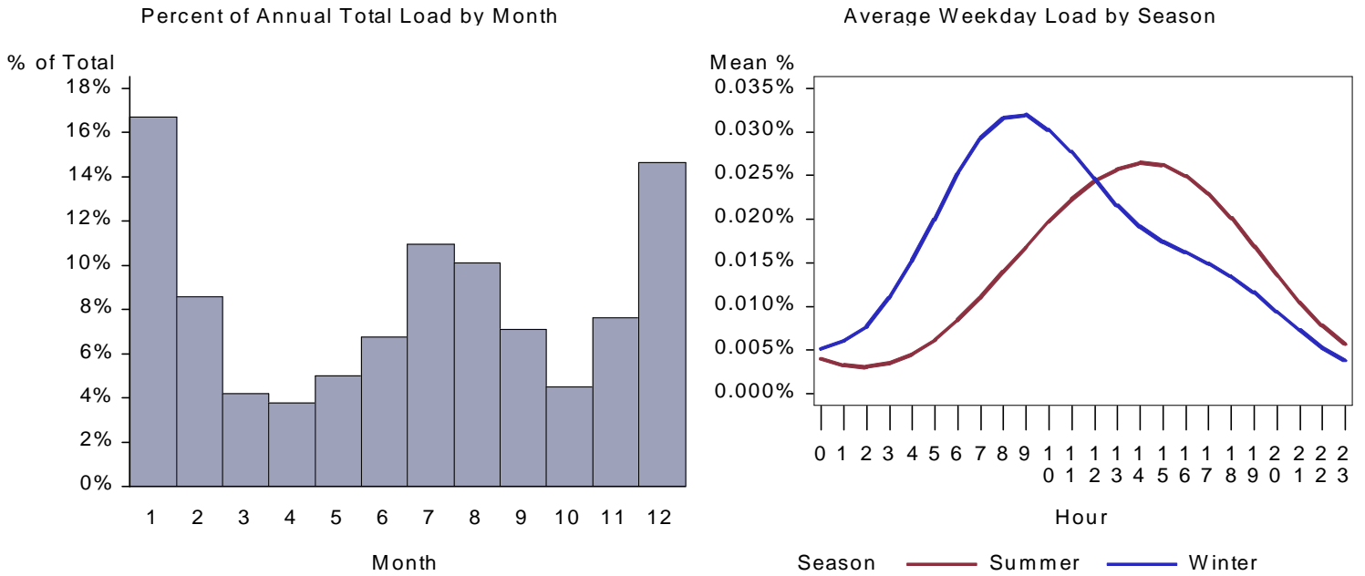
Figure 77. CA Miscellaneous HVAC Aux Load by Month and Average Weekday
