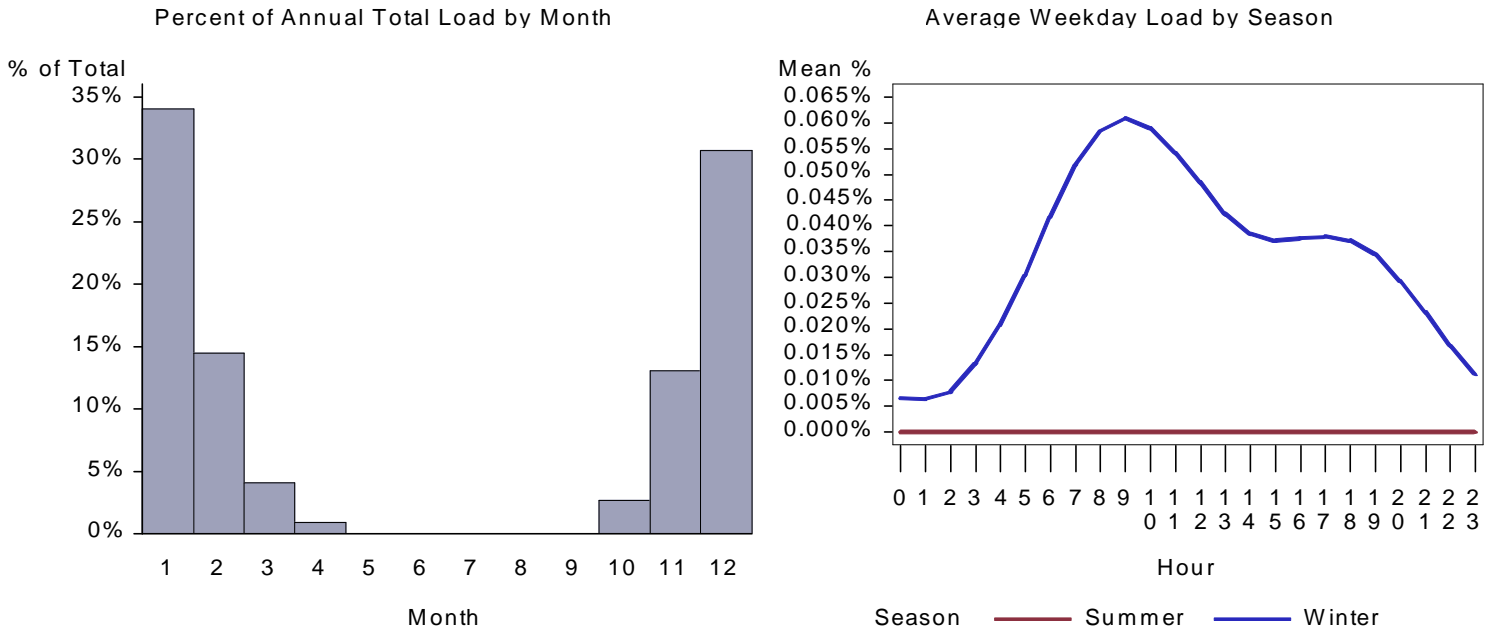
Figure 407. : CA Small Retail Space Heat Load by Month and Average Weekday
