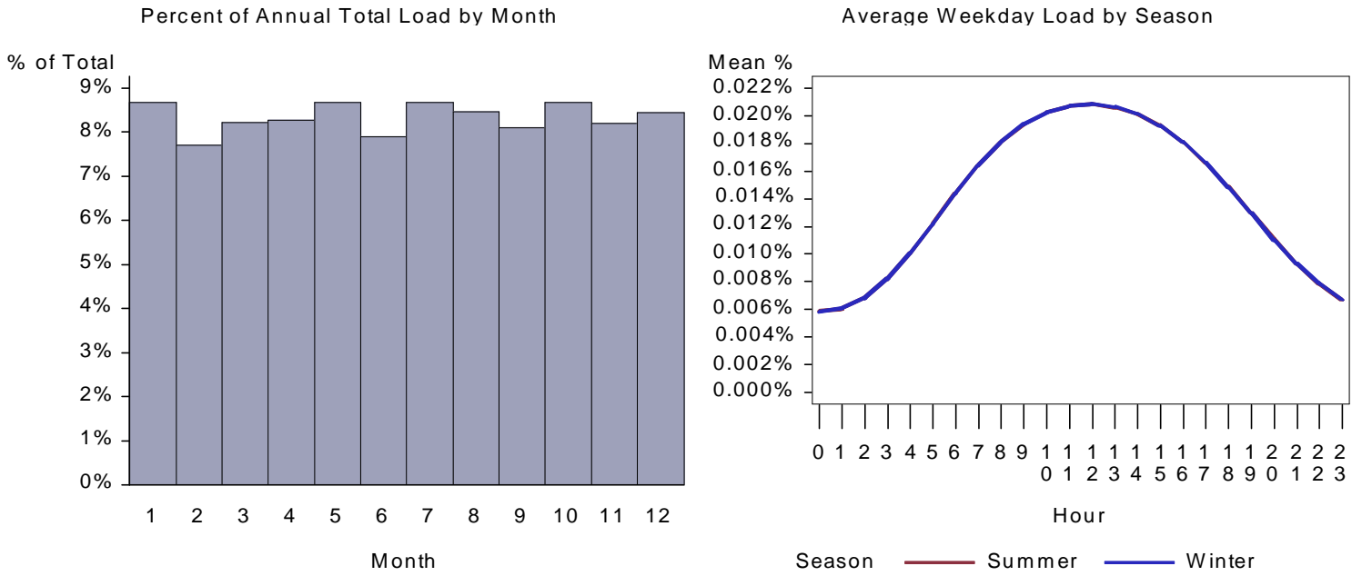
Figure 155. : WA Health Lighting Load by Month and Average Weekday
