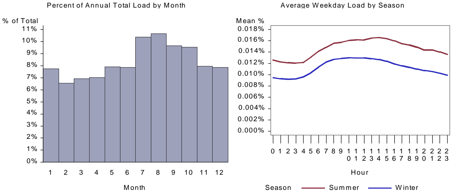
Figure 285. : CA School Refrigeration Load by Month and Average Weekday
