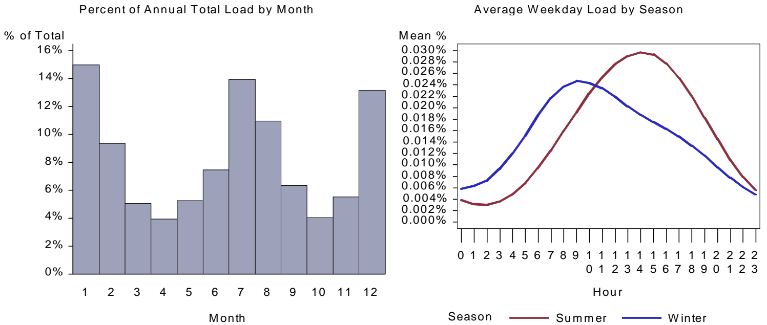
Figure 78. ID Miscellaneous HVAC Aux Load by Month and Average Weekday
