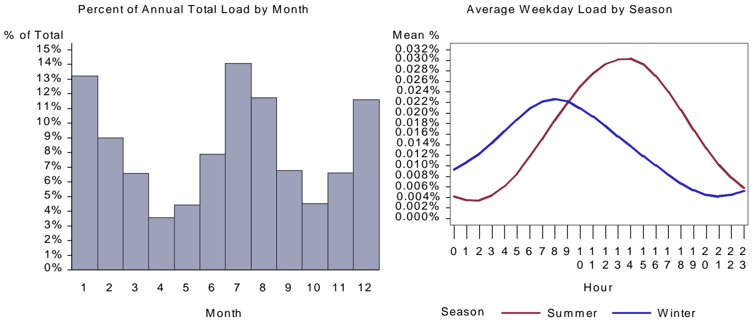
Figure 66. WY Large Office HVAC Aux Load by Month and Average Weekday
