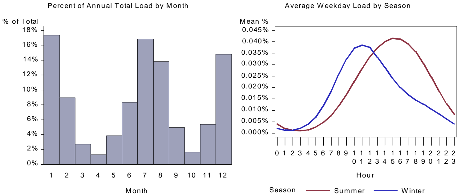
Figure 104. : UT Warehouse HVAC Aux Load by Month and Average Weekday
