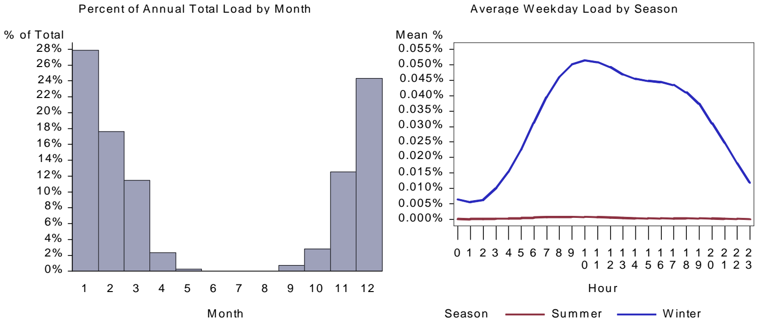
Figure 411. : WY Small Retail Space Heat Load by Month and Average Weekday
