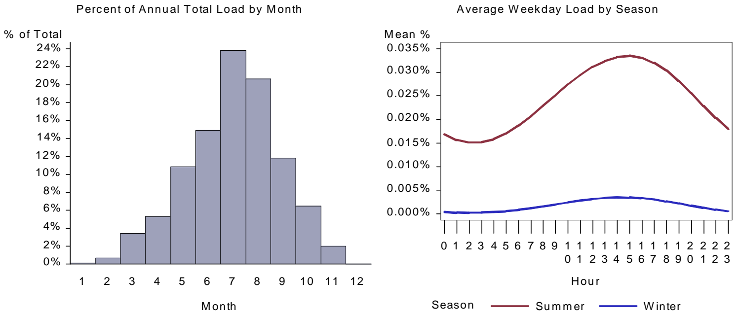
Figure 308. : UT Grocery Space Cool Load by Month and Average Weekday
