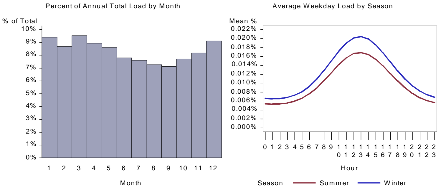
Figure 2. ID Grocery Cooking Load by Month and Average Weekday
