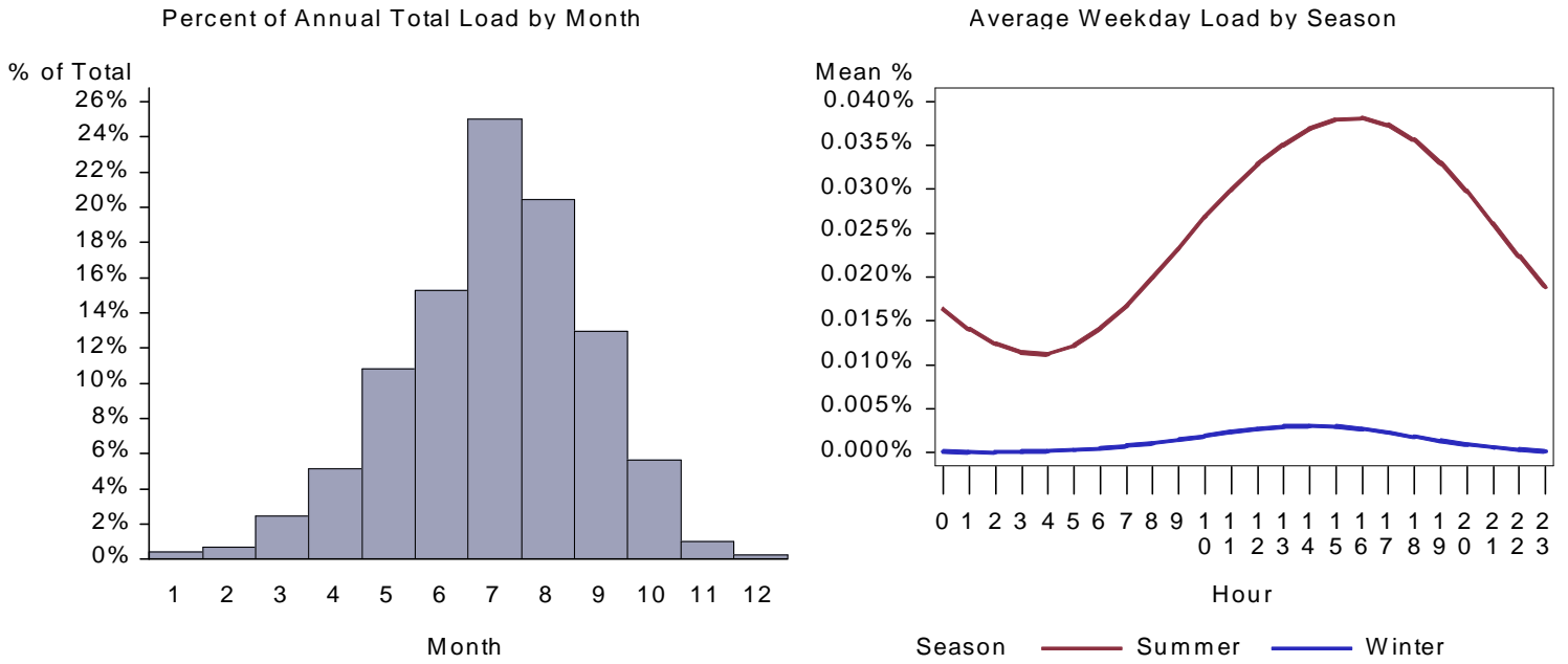
Figure 327. : ID Lodging Space Cool Load by Month and Average Weekday
