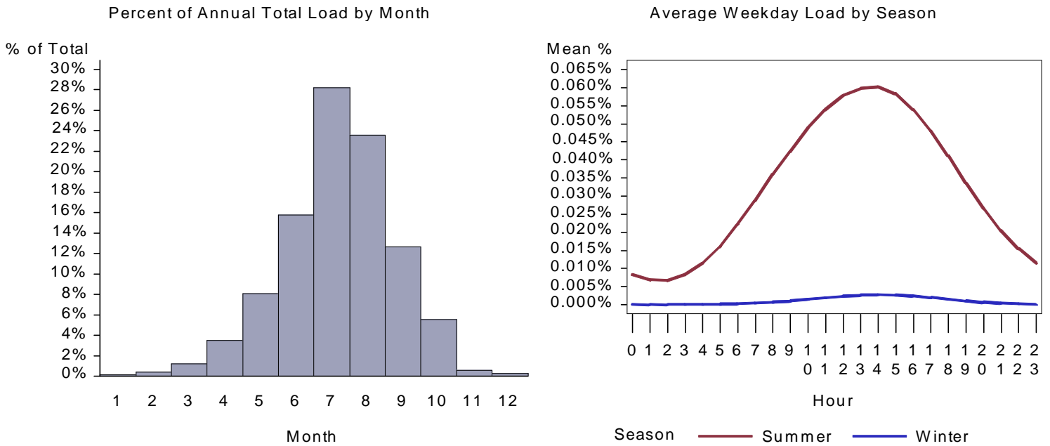
Figure 350. : WY Small Office Space Cool Load by Month and Average Weekday
