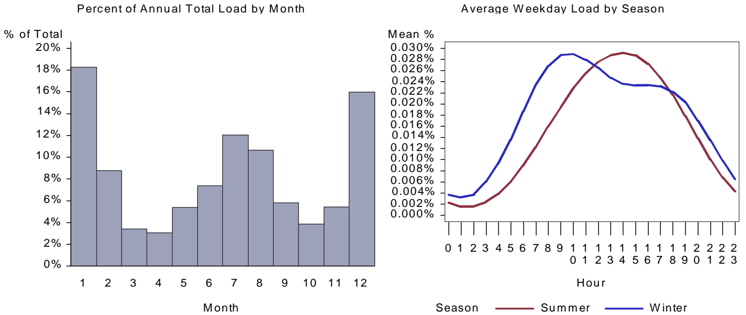
Figure 99. UT Small Retail HVAC Aux Load by Month and Average Weekday
