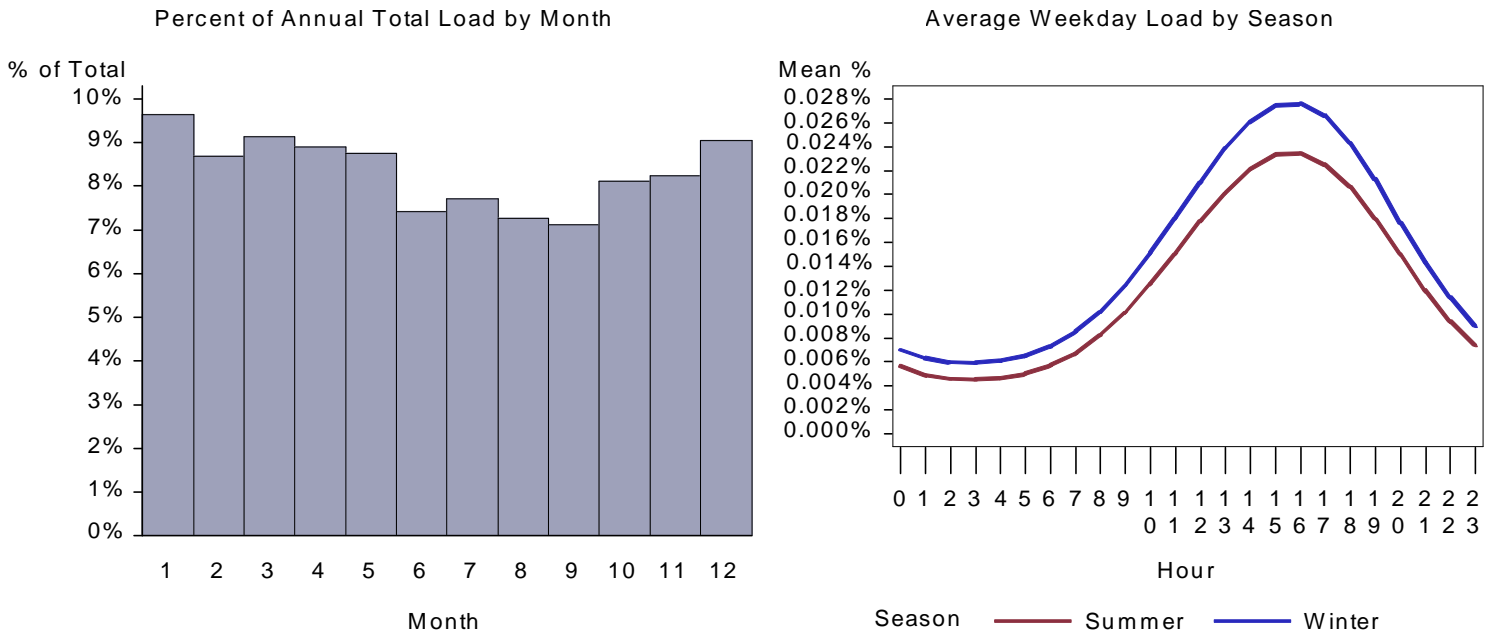
Figure 468. : CA Warehouse Water Heat Load by Month and Average Weekday
