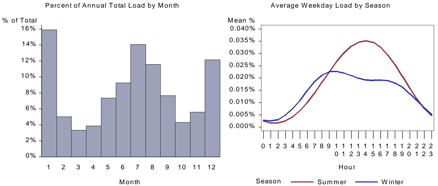
Figure 144.: WA Small Retail Heat Pump Load by Month and Average Weekday
