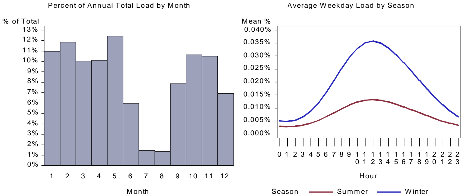
Figure 35. WY School Cooking Load by Month and Average Weekday
