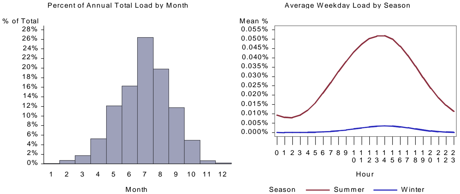
Figure 349. : WA Small Office Space Cool Load by Month and Average Weekday
