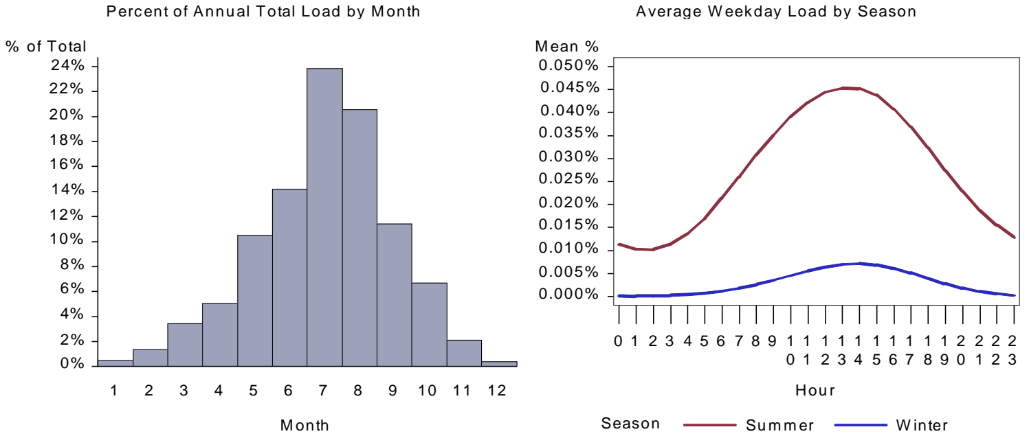
Figure 348. : UT Small Office Space Cool Load by Month and Average Weekday
