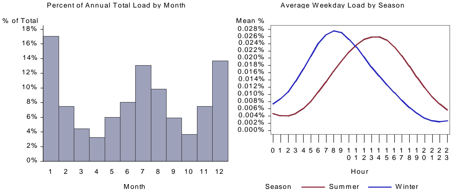
Figure 65. WA Large Office HVAC Aux Load by Month and Average Weekday
