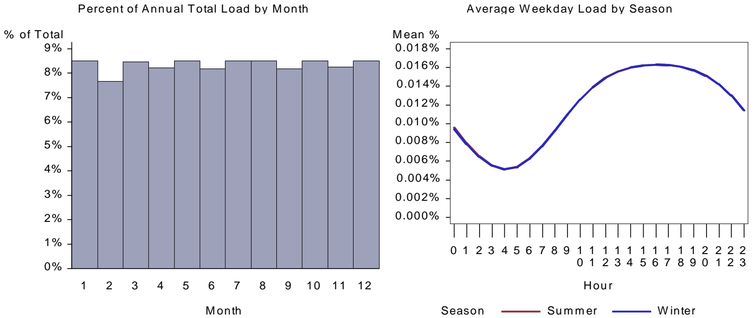
Figure 179. : UT Restaurant Lighting Load by Month and Average Weekday
