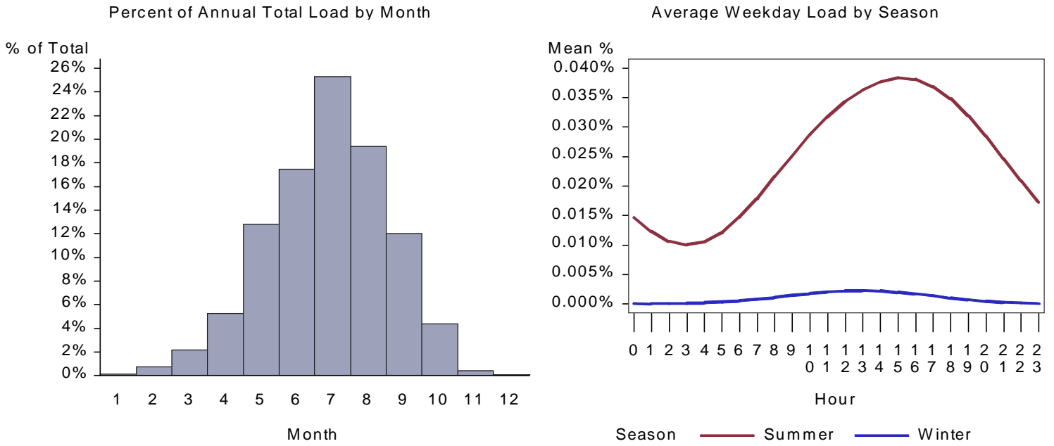
Figure 329. : WA Lodging Space Cool Load by Month and Average Weekday
