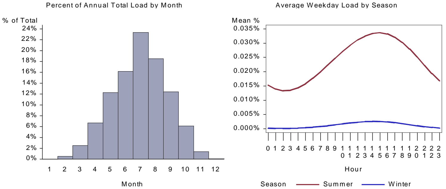
Figure 309. : WA Grocery Space Cool Load by Month and Average Weekday
