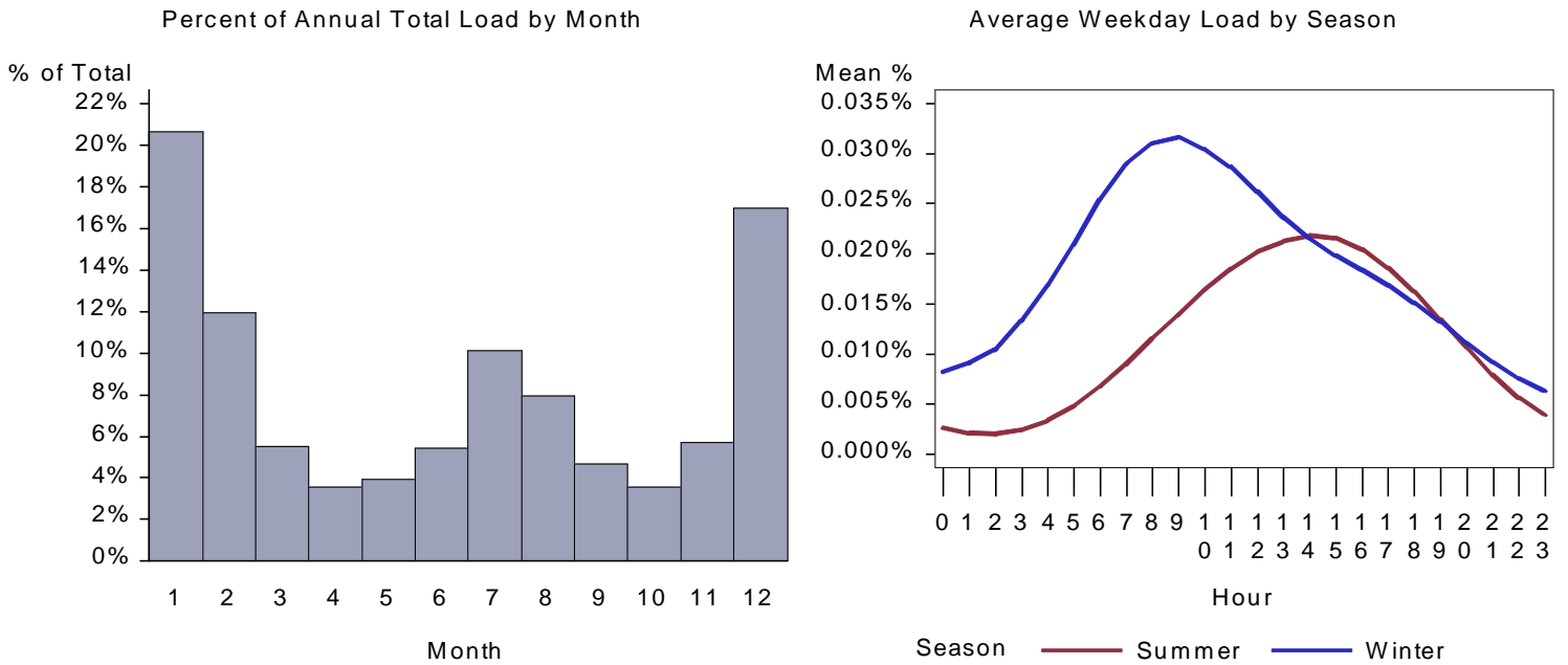
Figure 130. : ID Miscellaneous Heat Pump Load by Month and Average Weekday
