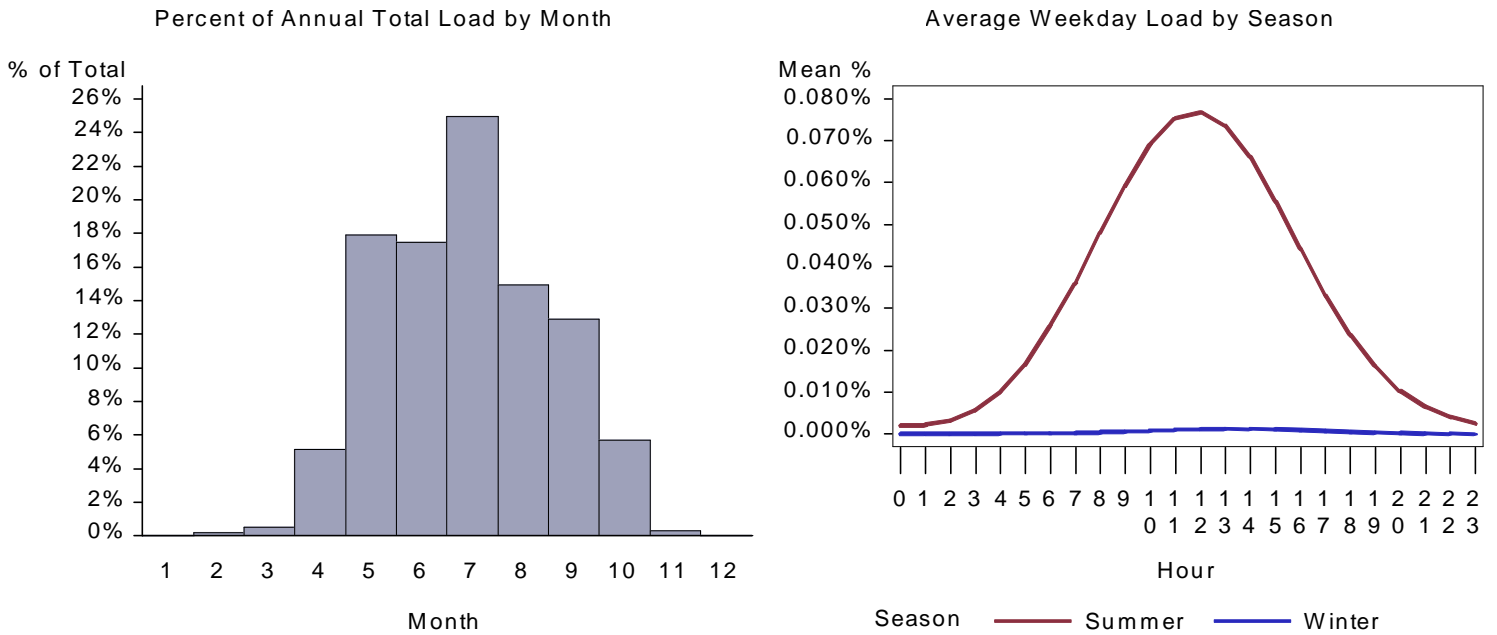
Figure 344. : WA School Space Cool Load by Month and Average Weekday
