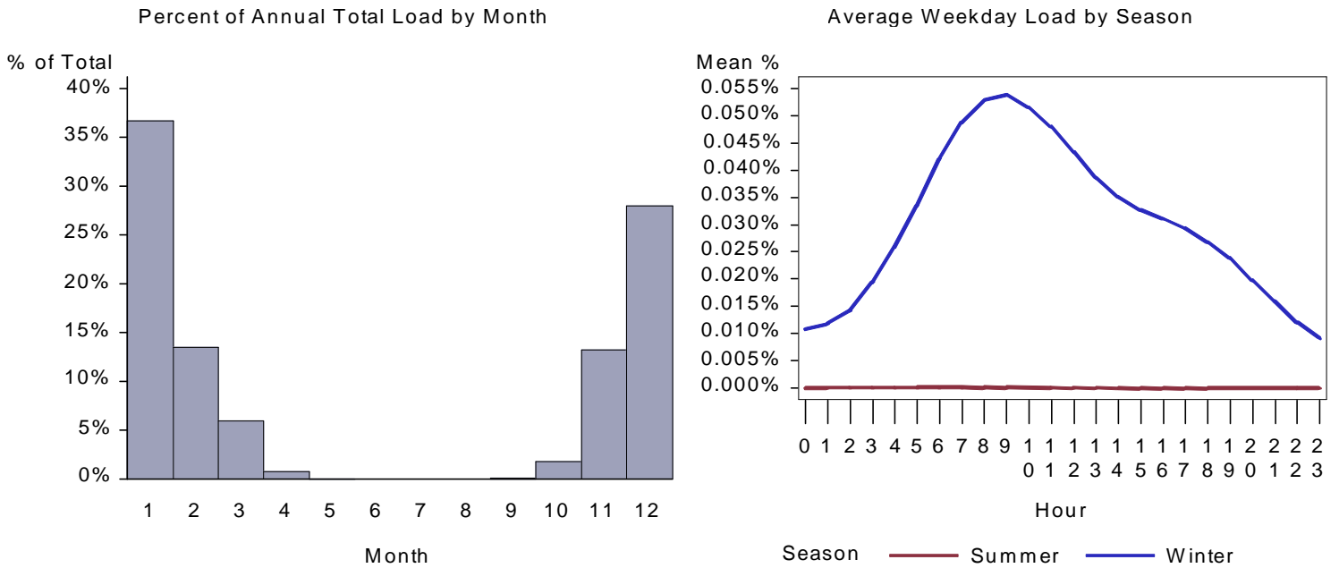
Figure 390. : WA Miscellaneous Space Heat Load by Month and Average Weekday
