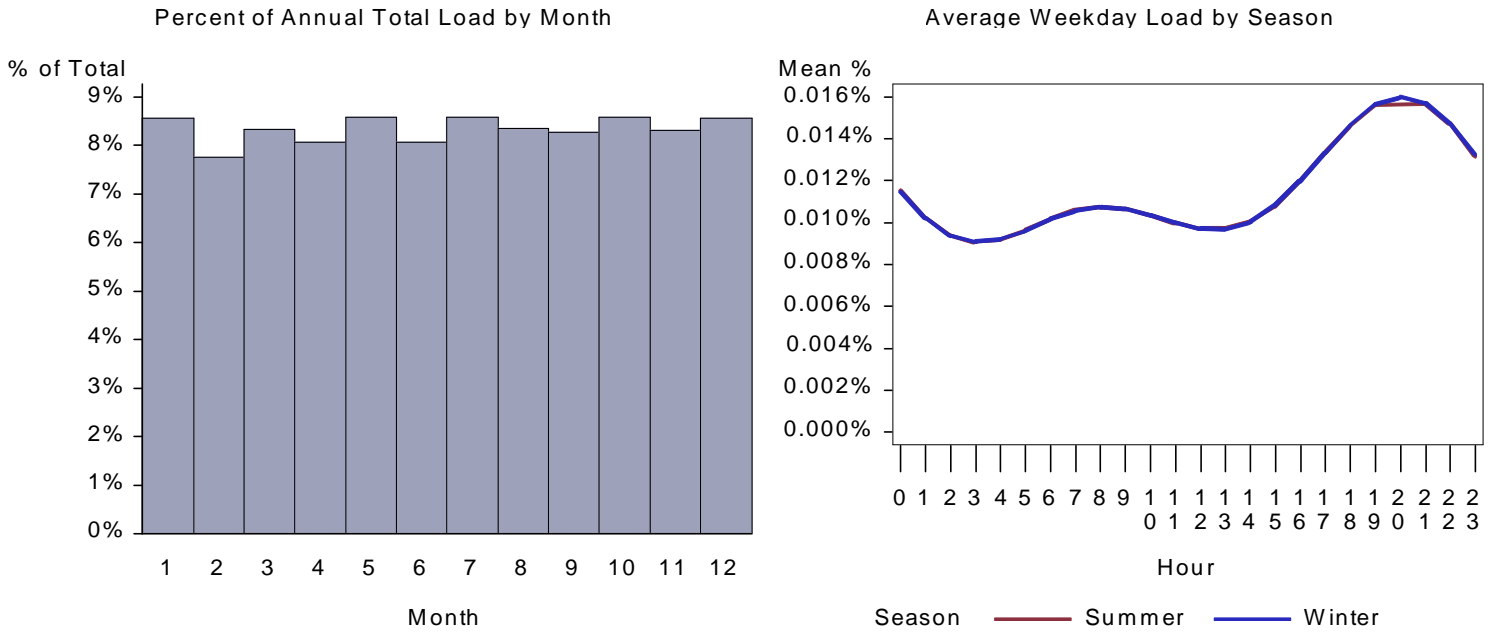
Figure 169. : UT Lodging Lighting Load by Month and Average Weekday
