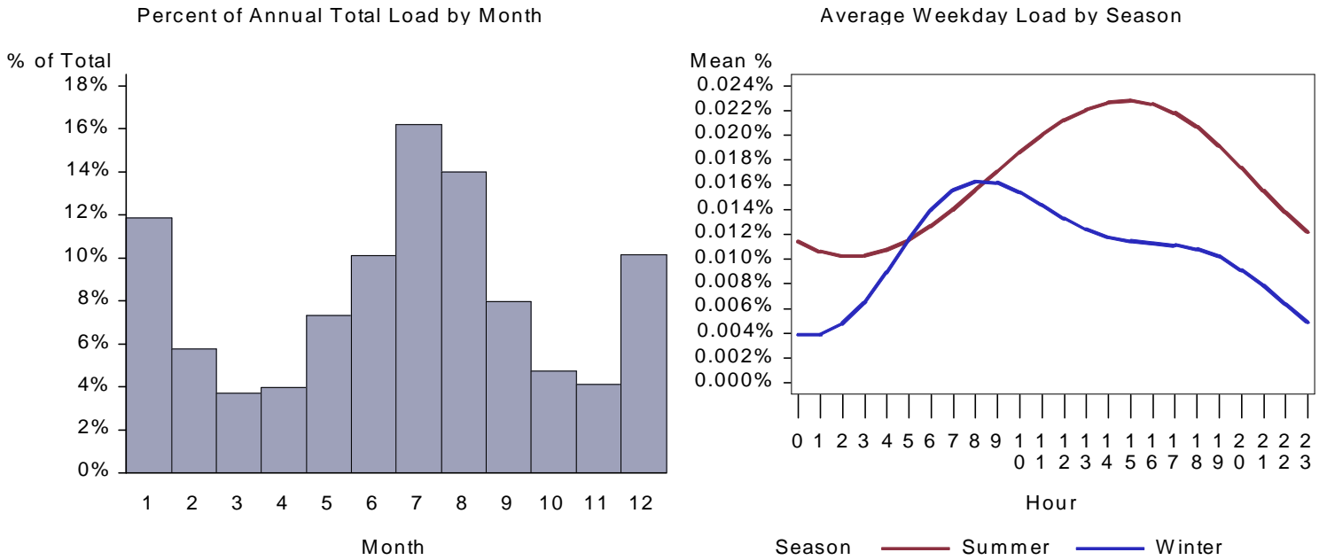
Figure 109. : UT Grocery Heat Pump Load by Month and Average Weekday
