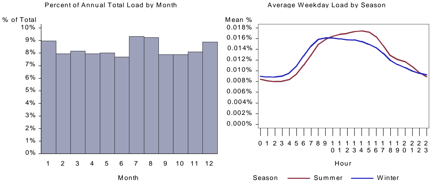
Figure 207. : WY Grocery Plug Load Load by Month and Average Weekday
