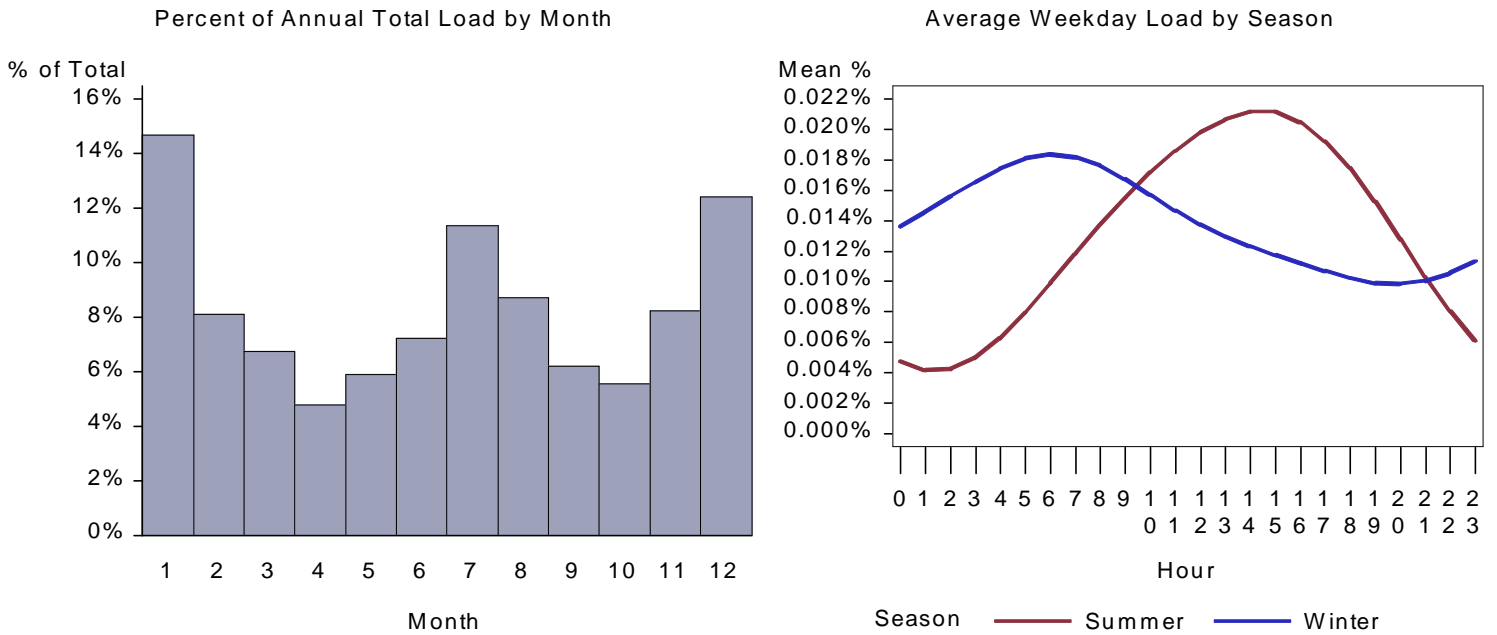
Figure 60. WA Health HVAC Aux Load by Month and Average Weekday
