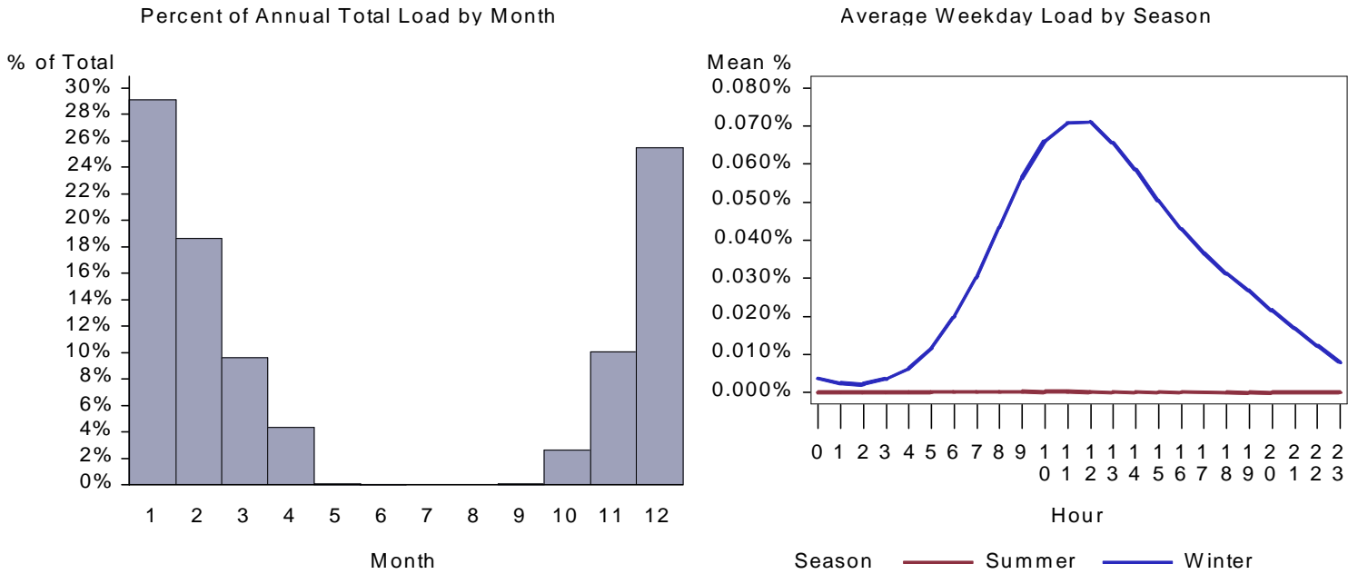
Figure 413. : ID Warehouse Space Heat Load by Month and Average Weekday
