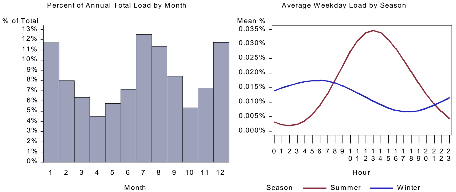
Figure 87. CA School HVAC Aux Load by Month and Average Weekday
