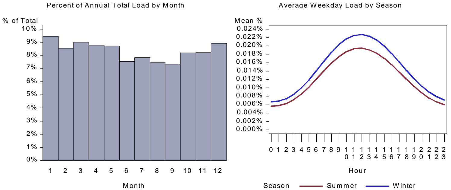
Figure 423. : CA Health Water Heat Load by Month and Average Weekday
