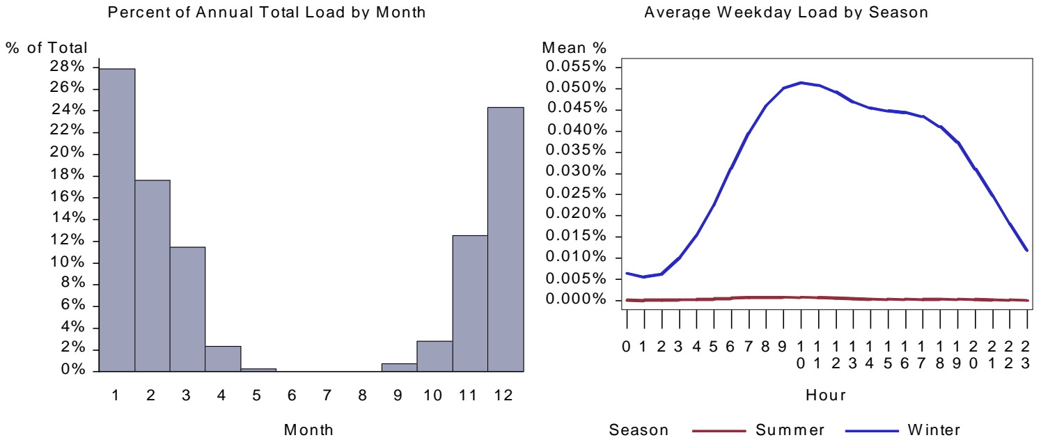
Figure 381. : WY Large Retail Space Heat Load by Month and Average Weekday
