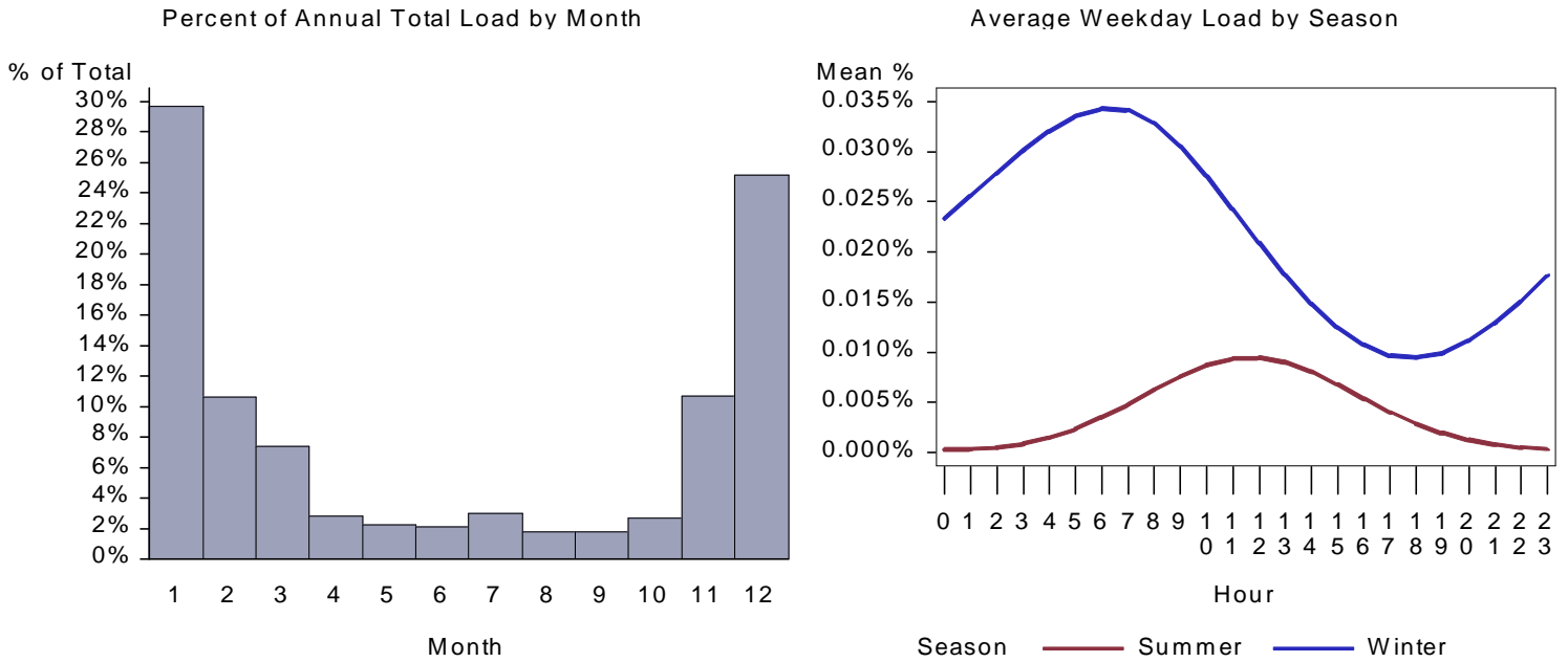
Figure 137. : WA School Heat Pump Load by Month and Average Weekday
