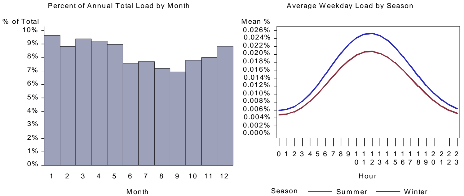
Figure 40. WY Small Office Cooking Load by Month and Average Weekday
