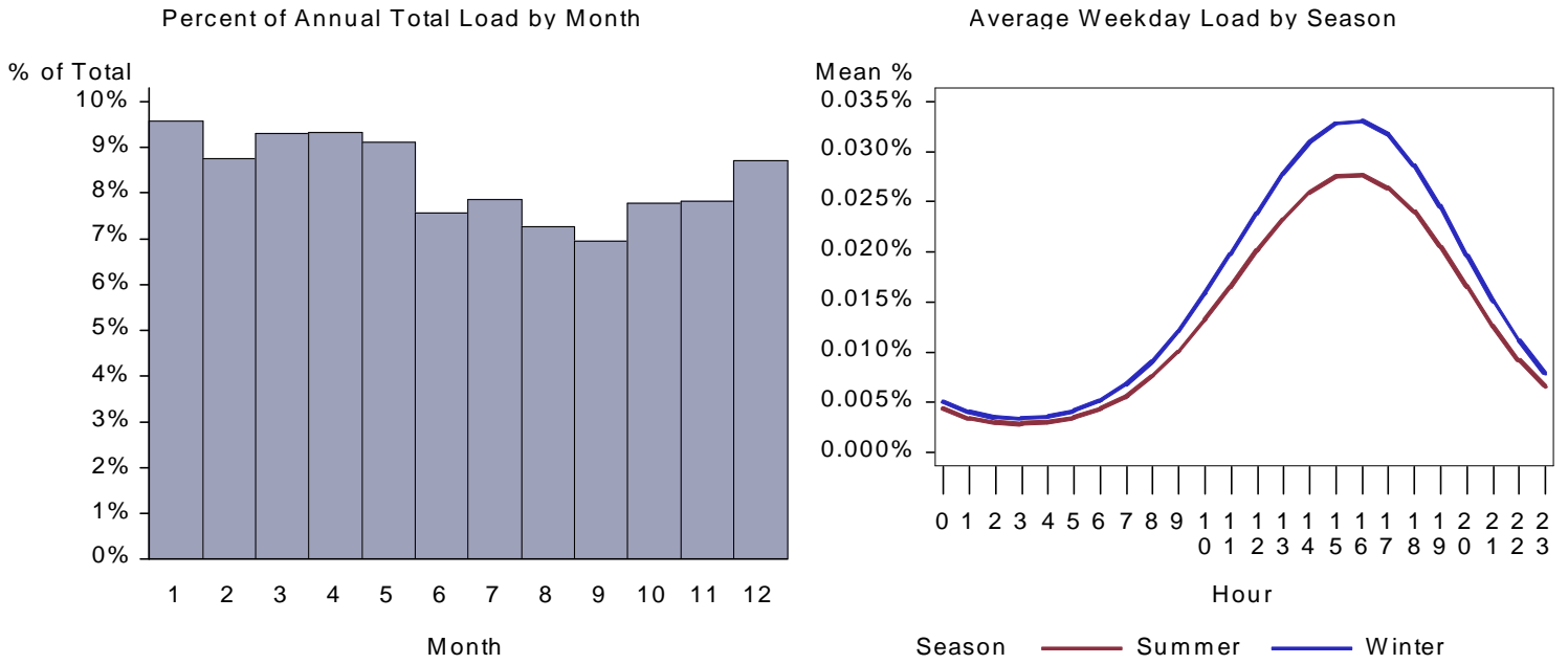
Figure 473. : WA Warehouse CA Water Heat Load by Month and Average Weekday
