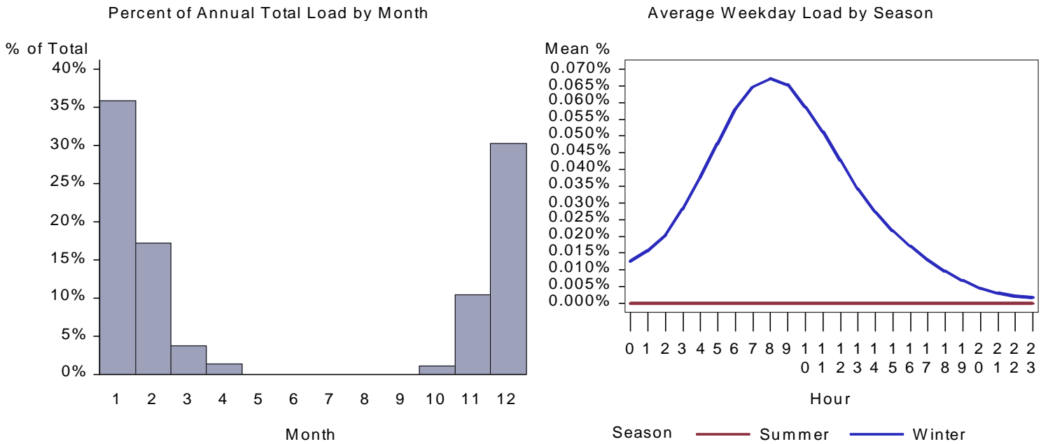
Figure 404. : UT Small Office Space Heat Load by Month and Average Weekday
