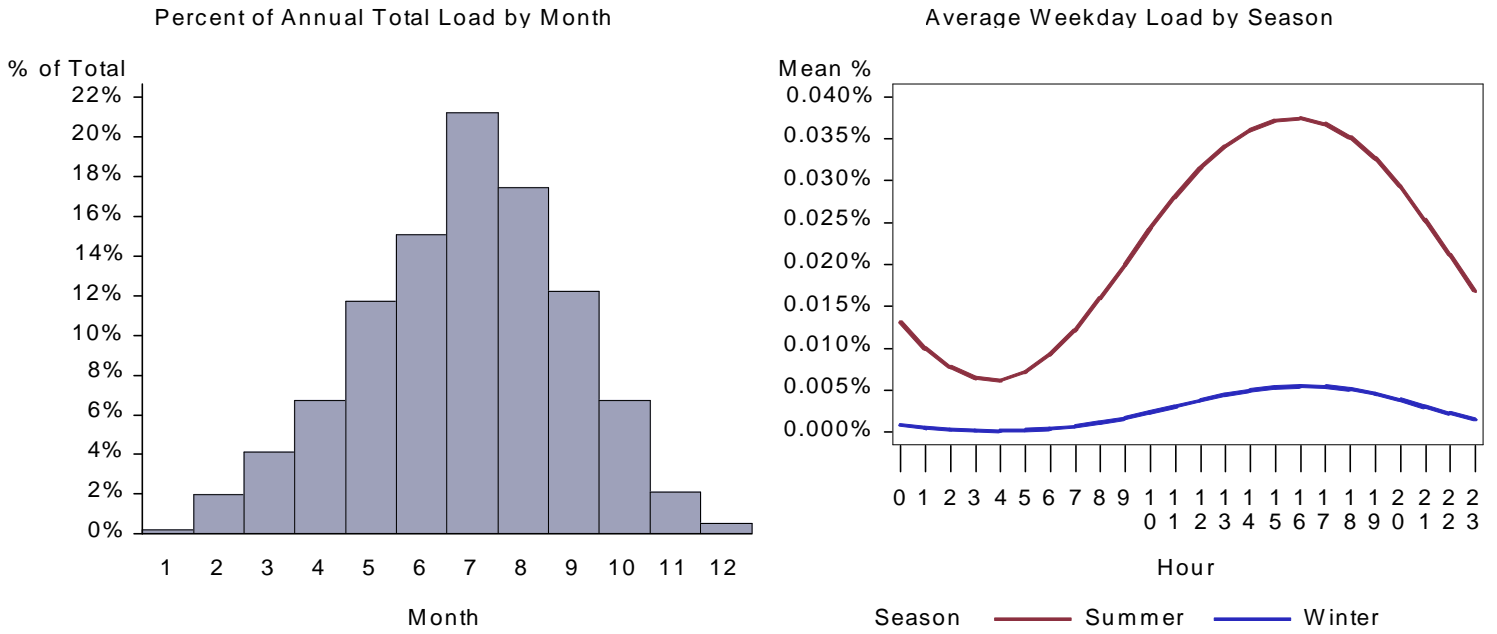
Figure 339. : WA Restaurant Space Cool Load by Month and Average Weekday
