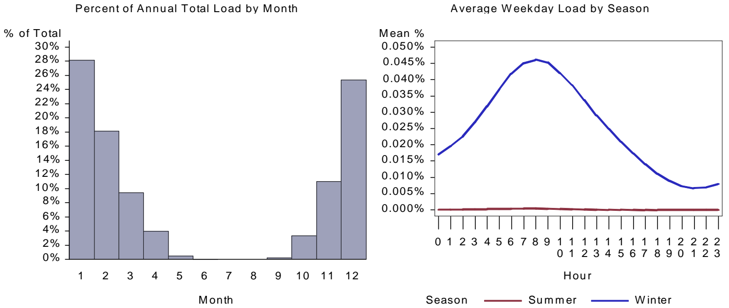
Figure 373. : ID Large Office Space Heat Load by Month and Average Weekday
