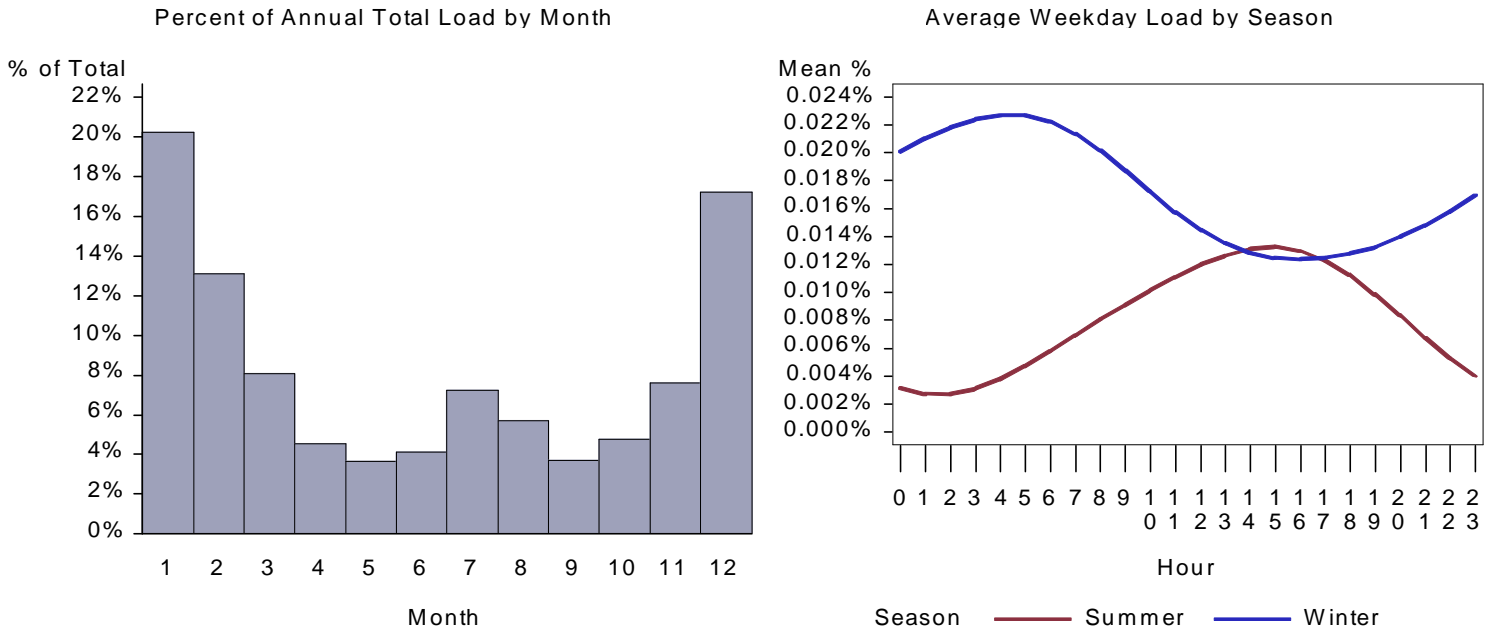
Figure 113. : ID Health Heat Pump Load by Month and Average Weekday
