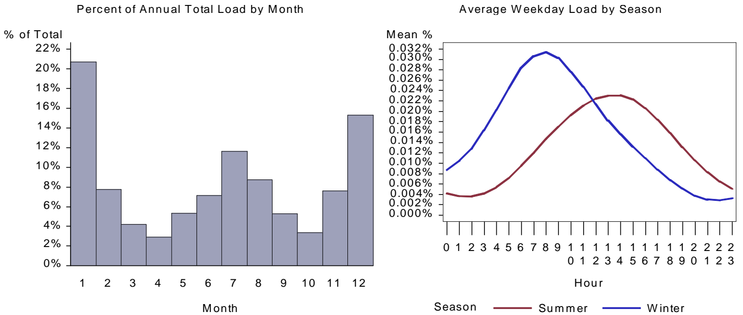
Figure 140. : WA Small Office Heat Pump Load by Month and Average Weekday
