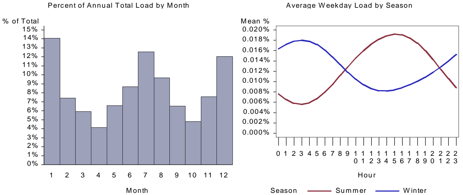
Figure 75. WA Lodging HVAC Aux Load by Month and Average Weekday
