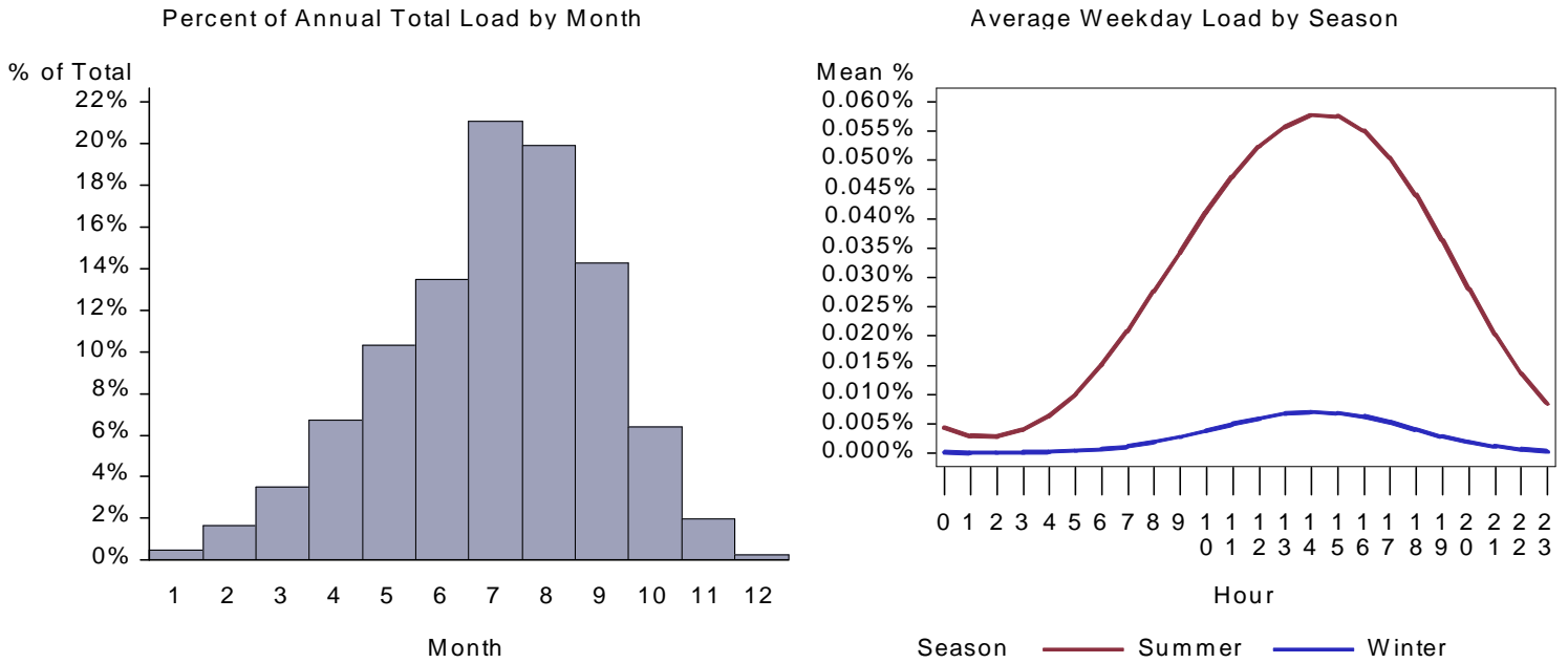
Figure 321. : CA Large Retail Space Cool Load by Month and Average Weekday
