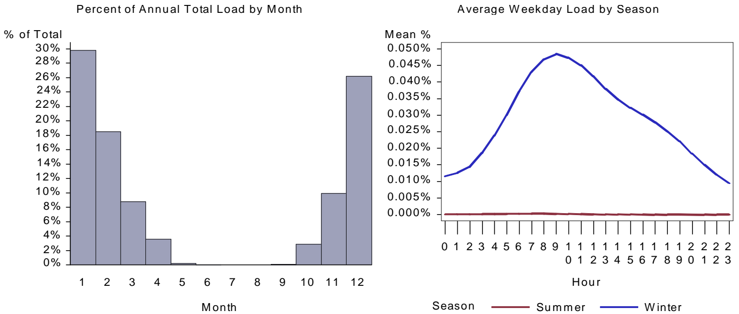
Figure 388. : ID Miscellaneous Space Heat Load by Month and Average Weekday
