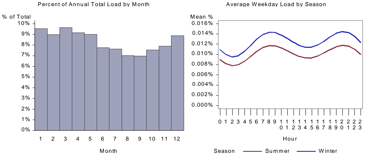
Figure 23. UT Lodging Cooking Load by Month and Average Weekday
