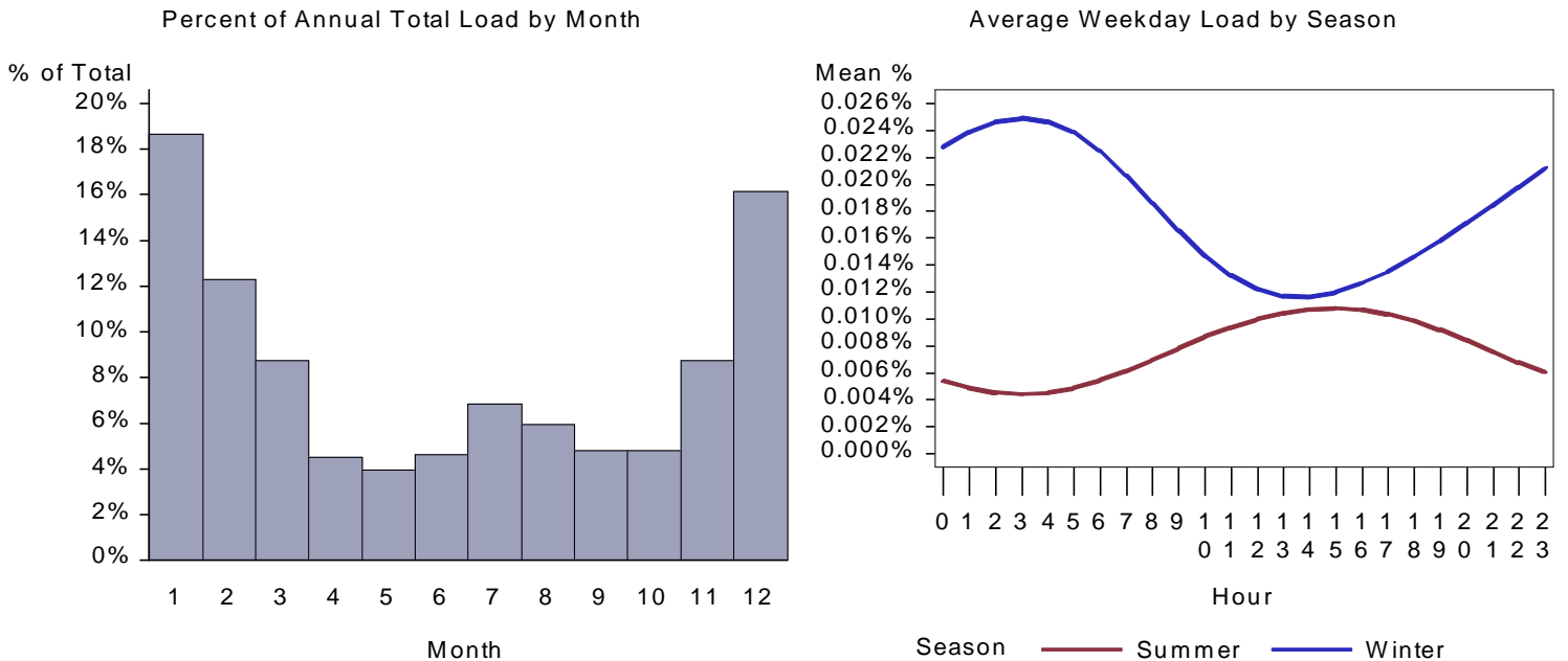
Figure 128. : WY Lodging Heat Pump Load by Month and Average Weekday
