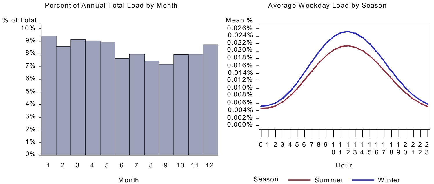
Figure 426. : WA Health Water Heat Load by Month and Average Weekday
