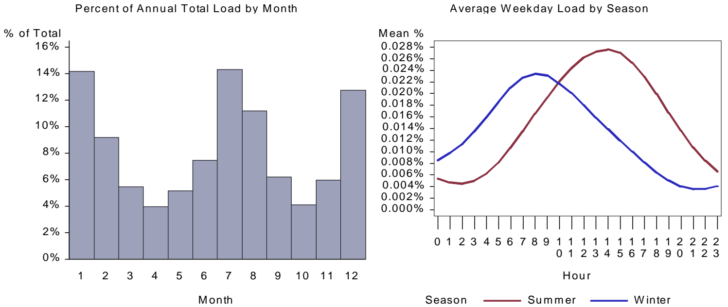
Figure 93. ID Small Office HVAC Aux Load by Month and Average Weekday
