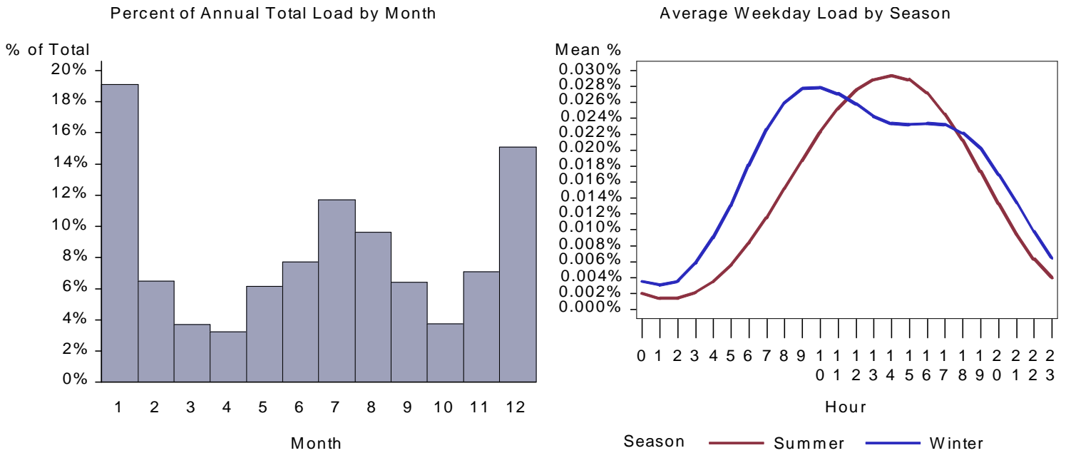
Figure 70. WA Large Retail HVAC Aux Load by Month and Average Weekday
