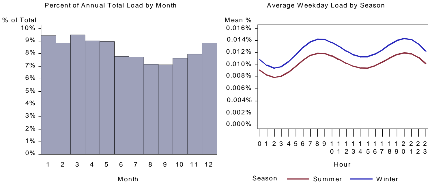
Figure 442. : WY Lodging Water Heat Load by Month and Average Weekday
