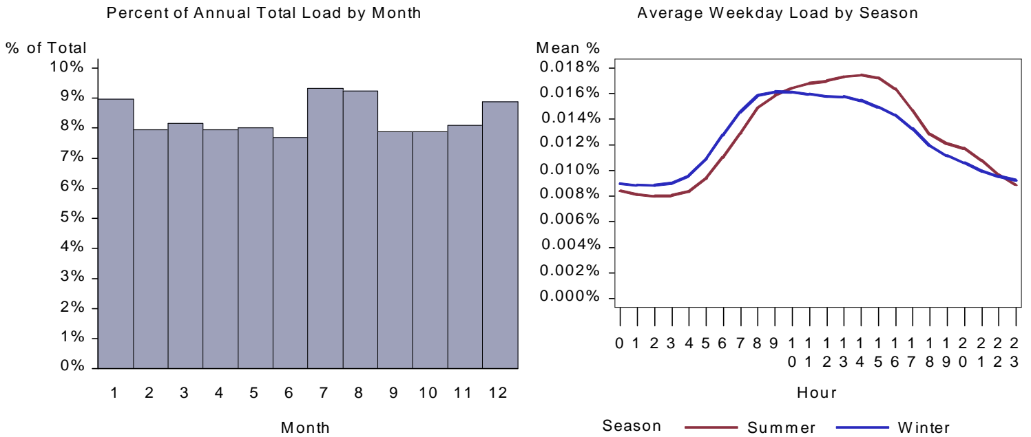
Figure 204. : ID Grocery Plug Load Load by Month and Average Weekday
