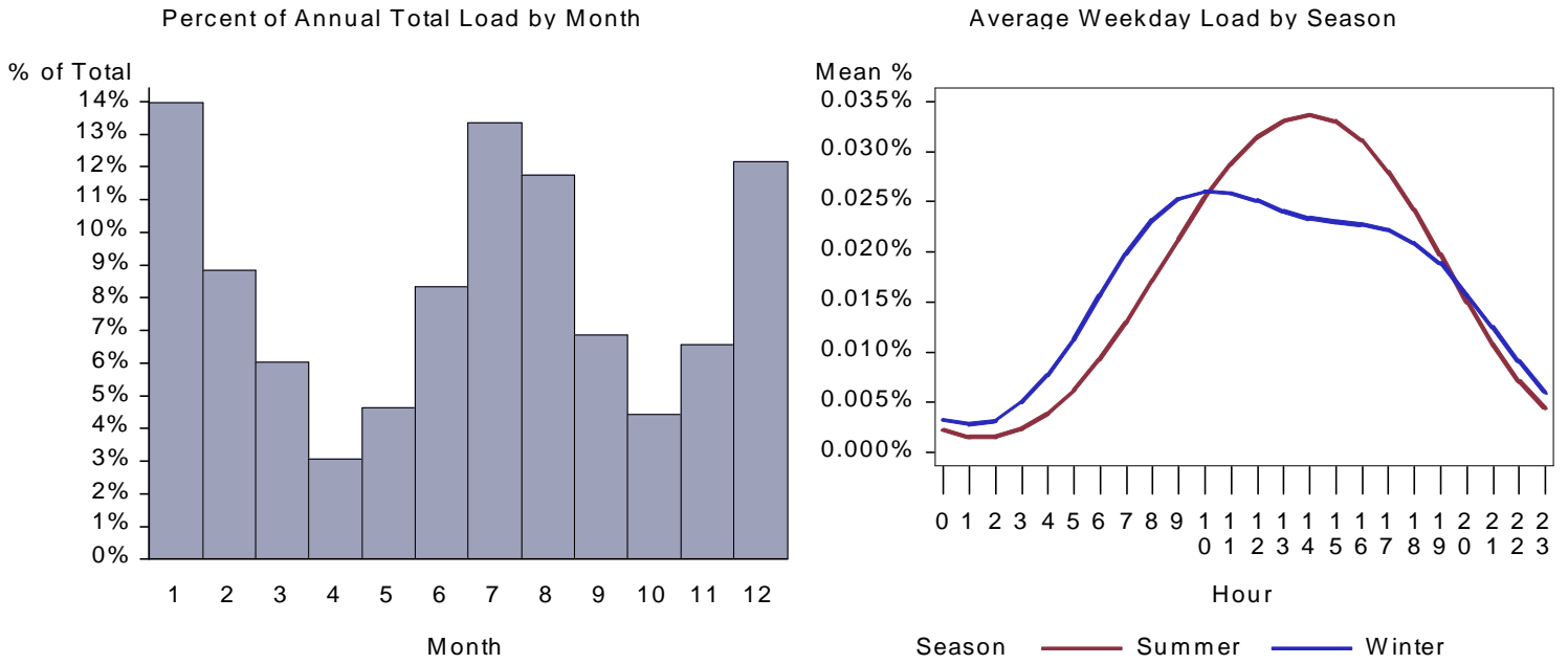
Figure 71. WY Large Retail HVAC Aux Load by Month and Average Weekday
