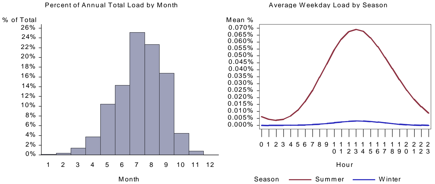
Figure 341. : CA School Space Cool Load by Month and Average Weekday
