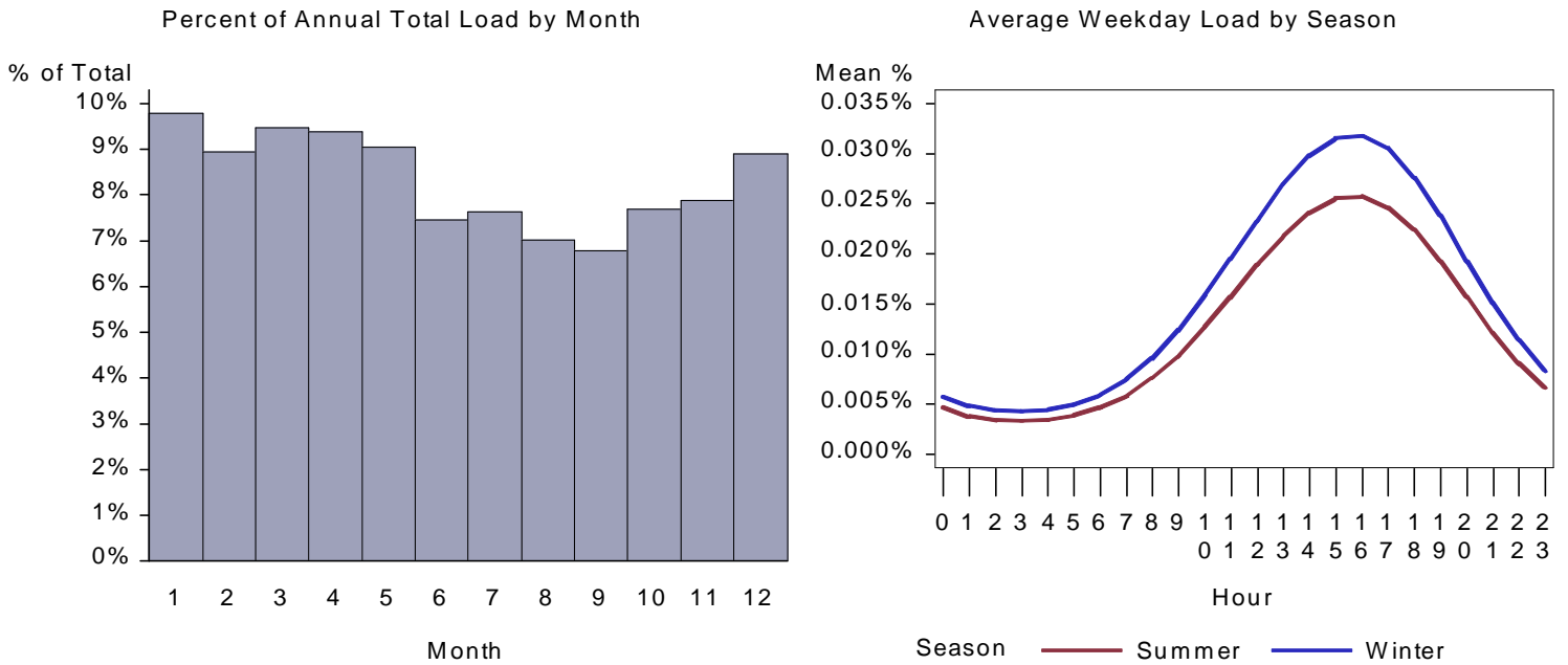
Figure 470. : UT Warehouse Water Heat Load by Month and Average Weekday
