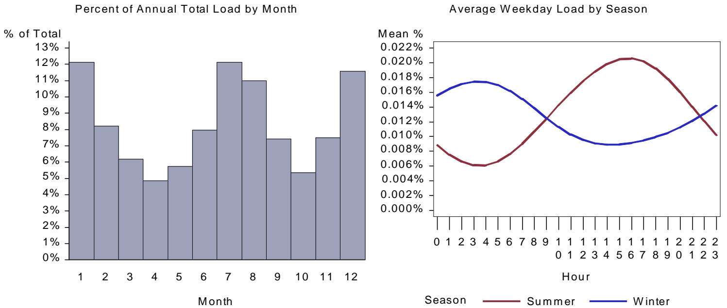
Figure 72. CA Lodging HVAC Aux Load by Month and Average Weekday
