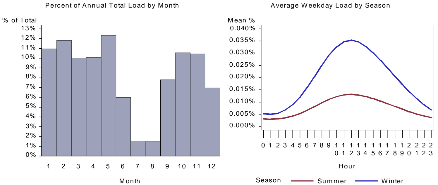
Figure 32. ID School Cooking Load by Month and Average Weekday
