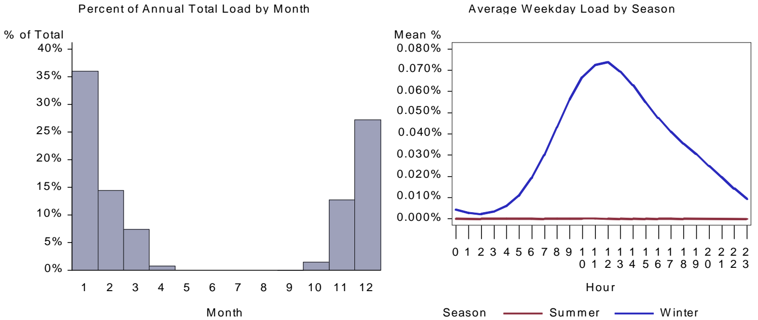
Figure 415. : WA Warehouse Space Heat Load by Month and Average Weekday
