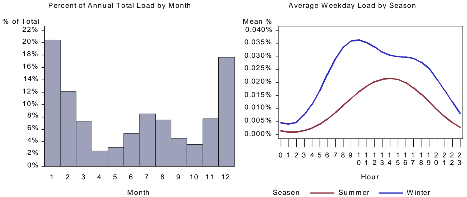
Figure 145. : WY Small Retail Heat Pump Load by Month and Average Weekday
