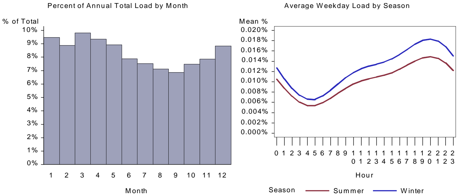
Figure 28. UT Restaurant Cooking Load by Month and Average Weekday
