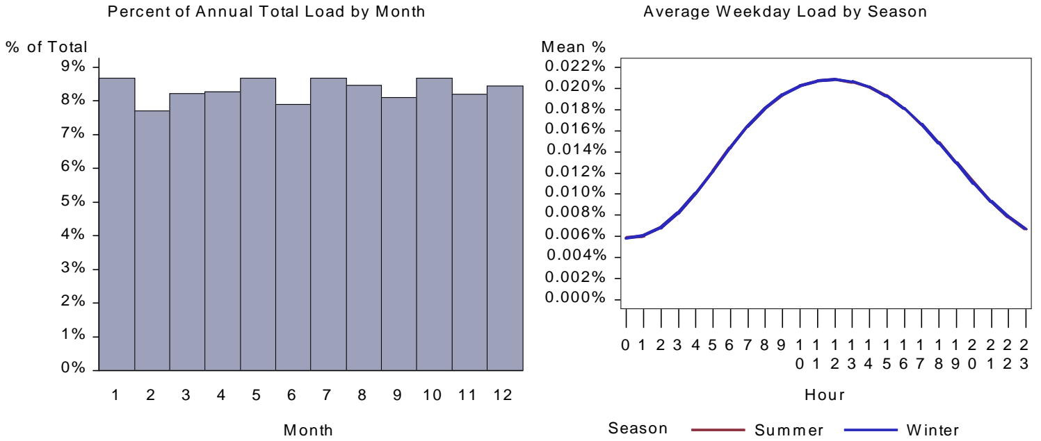
Figure 154. : UT Health Lighting Load by Month and Average Weekday
