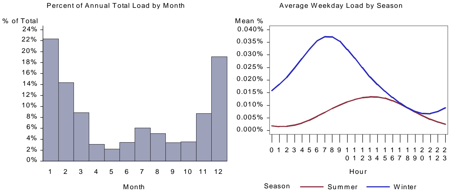
Figure 120. : WY Large Office Heat Pump Load by Month and Average Weekday
