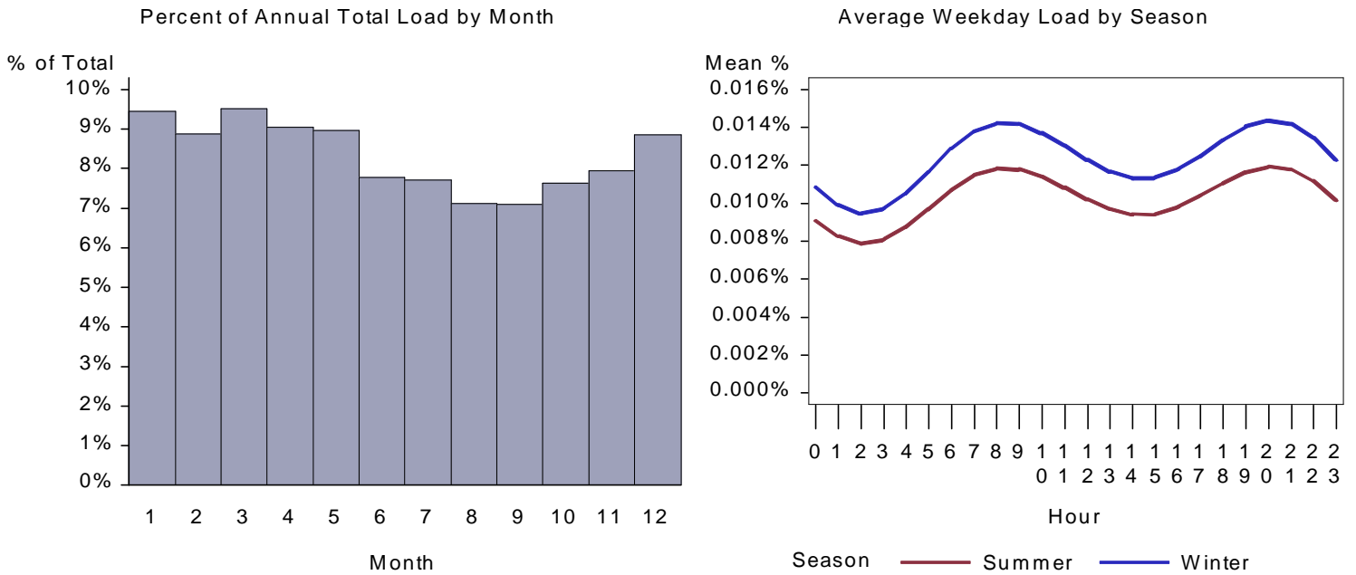
Figure 22. ID Lodging Cooking Load by Month and Average Weekday
