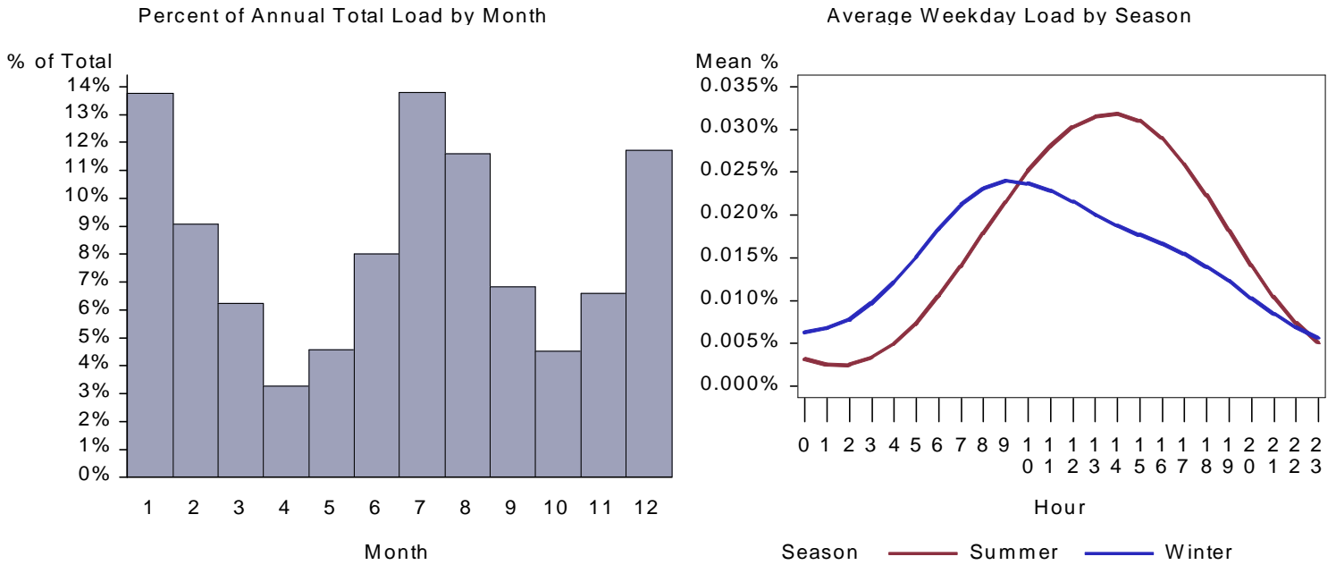
Figure 81. WY Miscellaneous HVAC Aux Load by Month and Average Weekday
