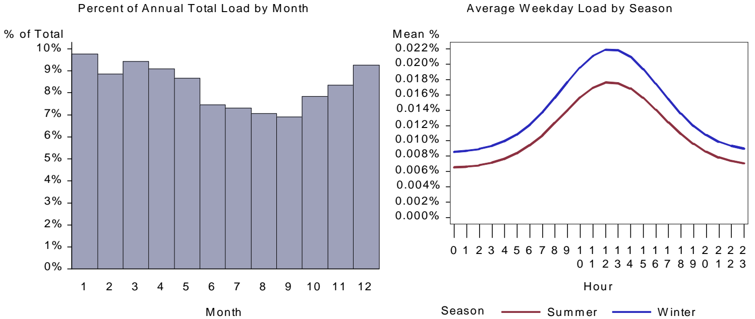
Figure 18. UT Large Retail Cooking Load by Month and Average Weekday
