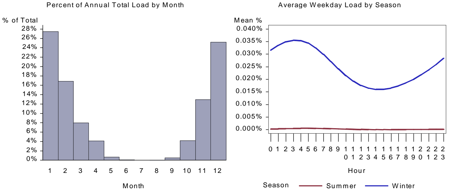
Figure 384. : UT Lodging Space Heat Load by Month and Average Weekday
