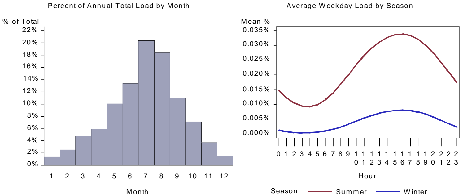
Figure 338. : UT Restaurant Space Cool Load by Month and Average Weekday
