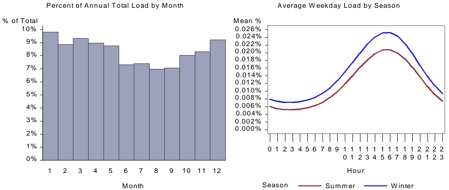
Figure 472. : WY Warehouse Water Heat Load by Month and Average Weekday
