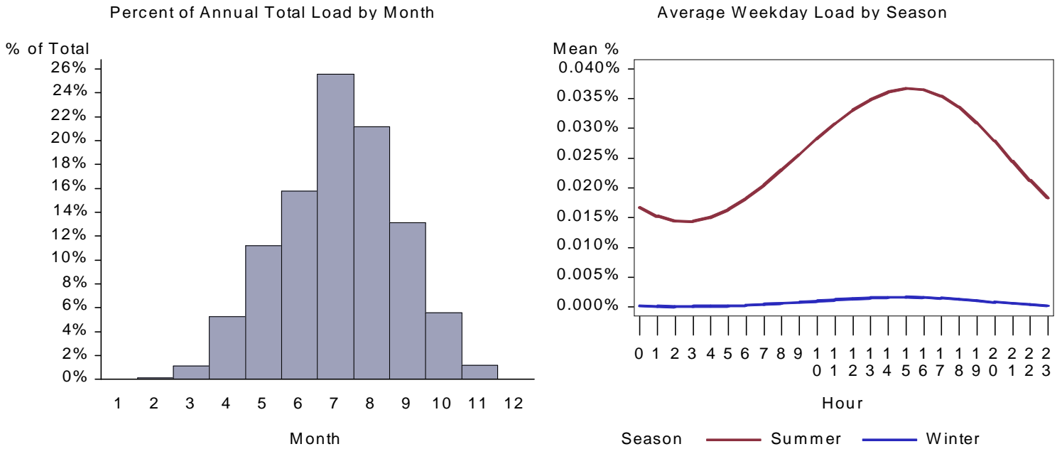
Figure 307. : ID Grocery Space Cool Load by Month and Average Weekday
