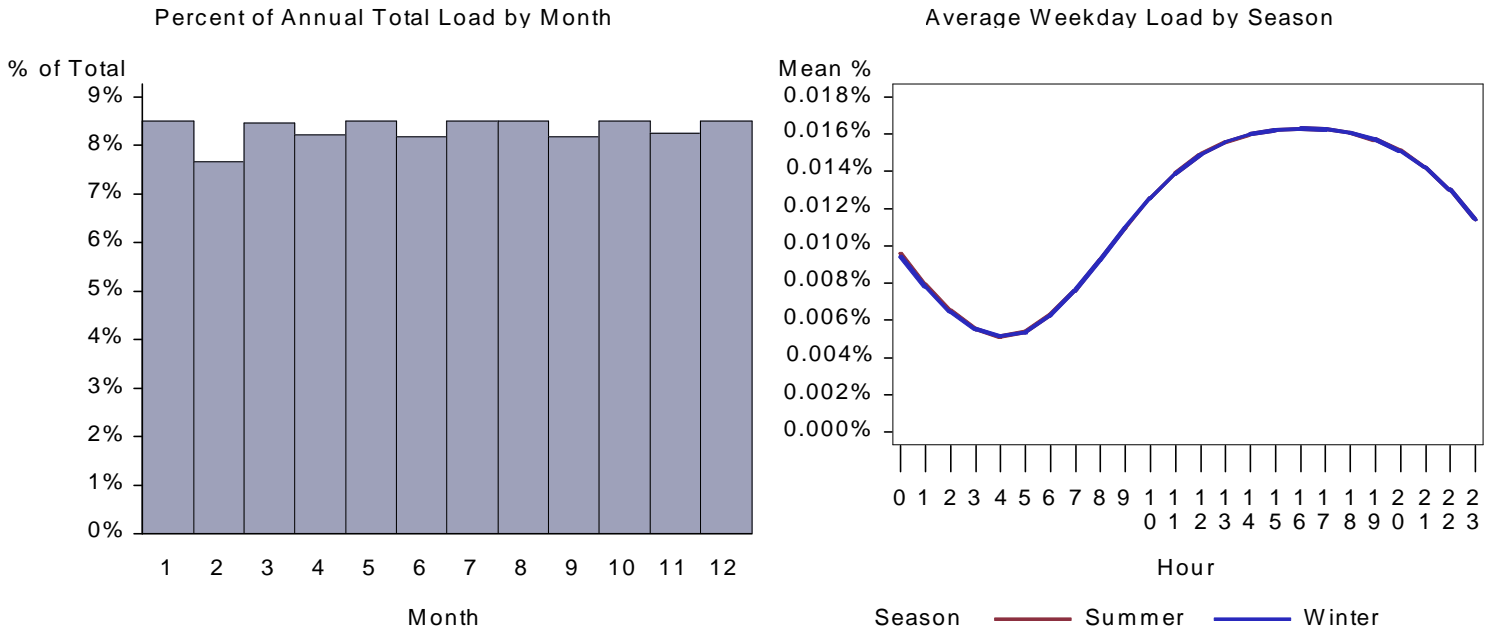
Figure 177. : CA Restaurant Lighting Load by Month and Average Weekday
