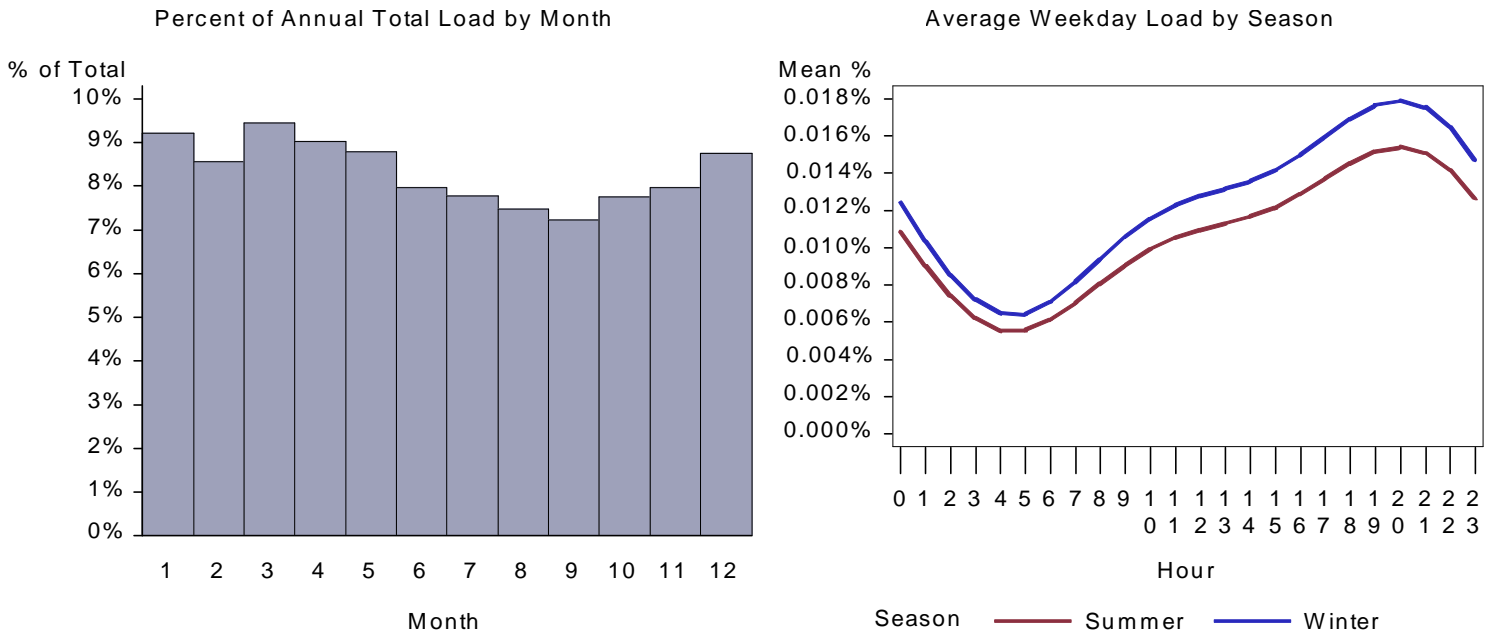
Figure 26. CA Restaurant Cooking Load by Month and Average Weekday
