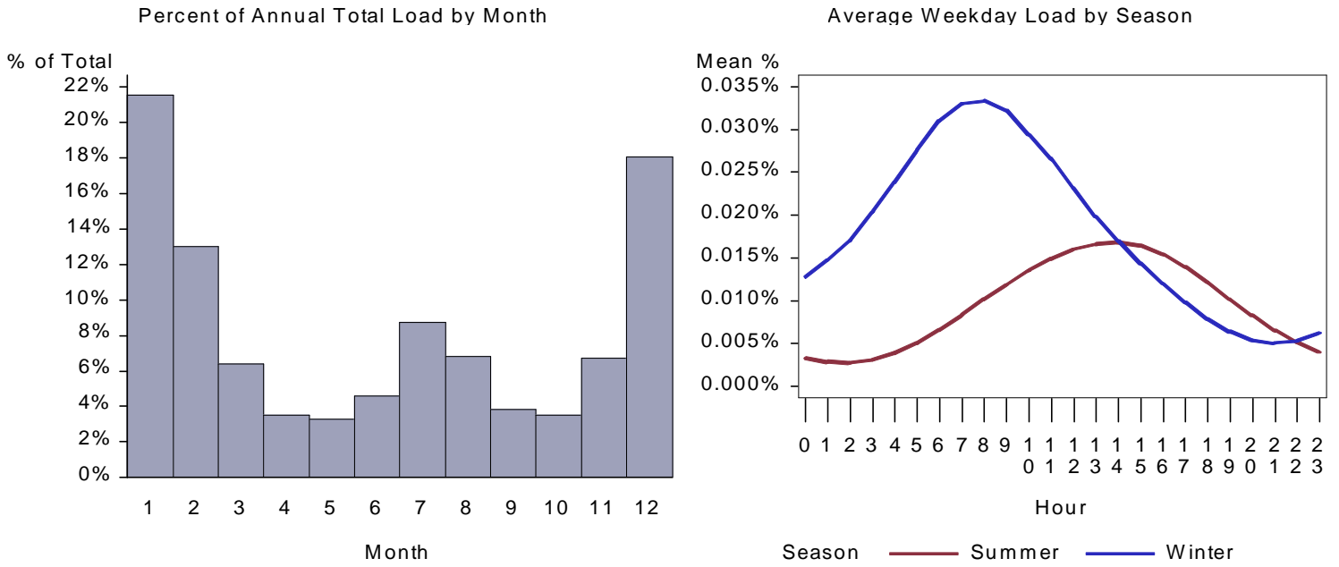
Figure 139. : ID Small Office Heat Pump Load by Month and Average Weekday
