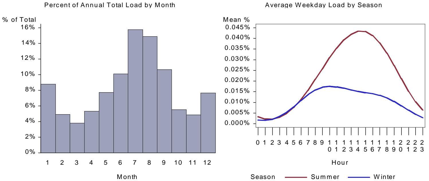
Figure 121. : CA Large Retail Heat Pump Load by Month and Average Weekday
