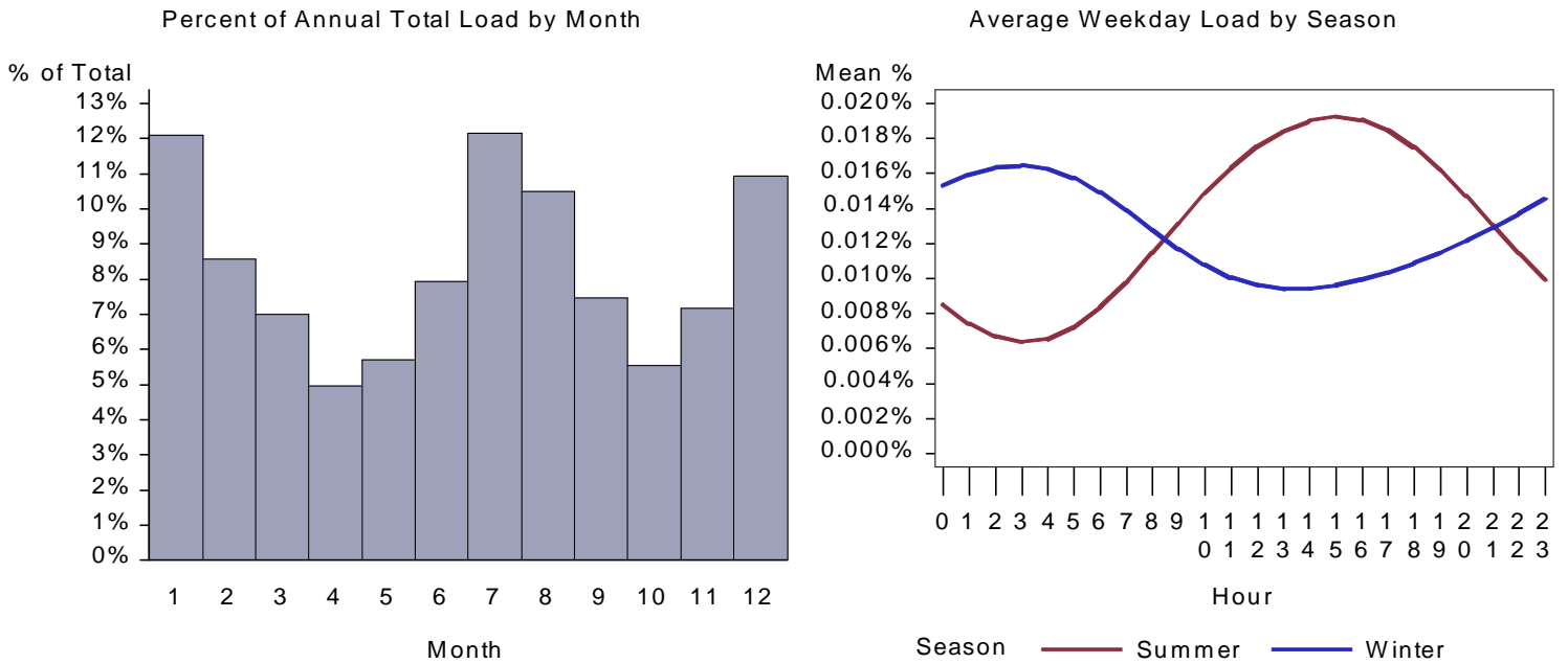
Figure 76. WY Lodging HVAC Aux Load by Month and Average Weekday
