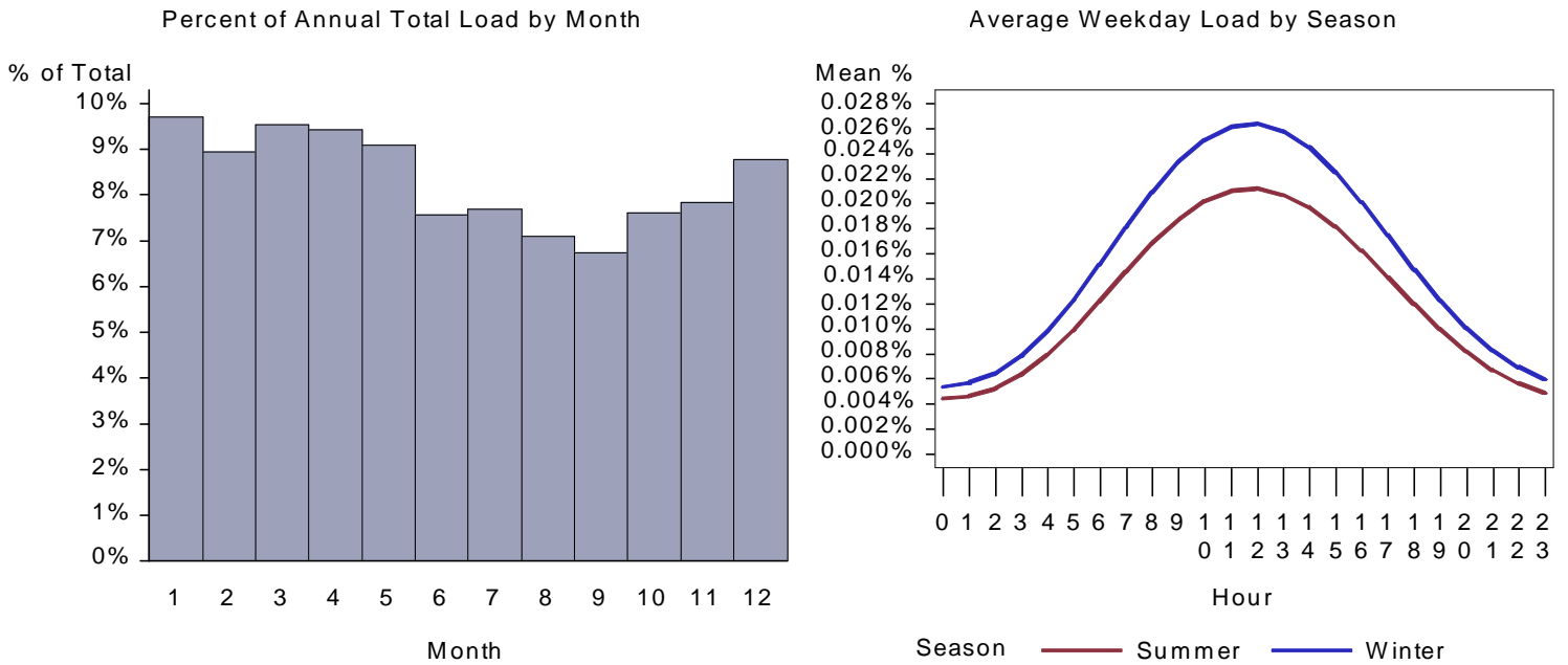
Figure 430. : UT Large Office Water Heat Load by Month and Average Weekday
