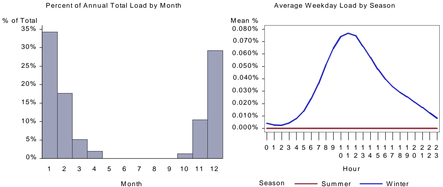
Figure 414. : UT Warehouse Space Heat Load by Month and Average Weekday
