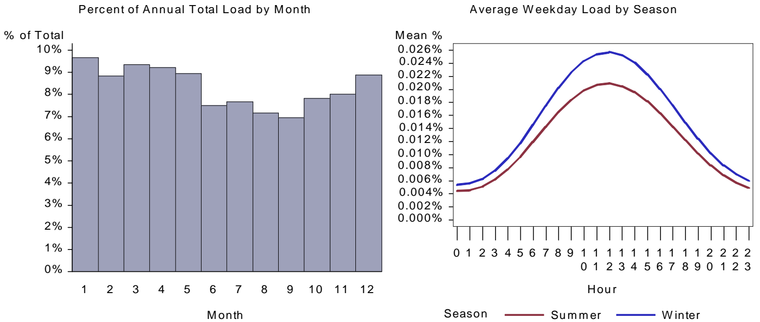
Figure 8. UT Health Cooking Load by Month and Average Weekday
