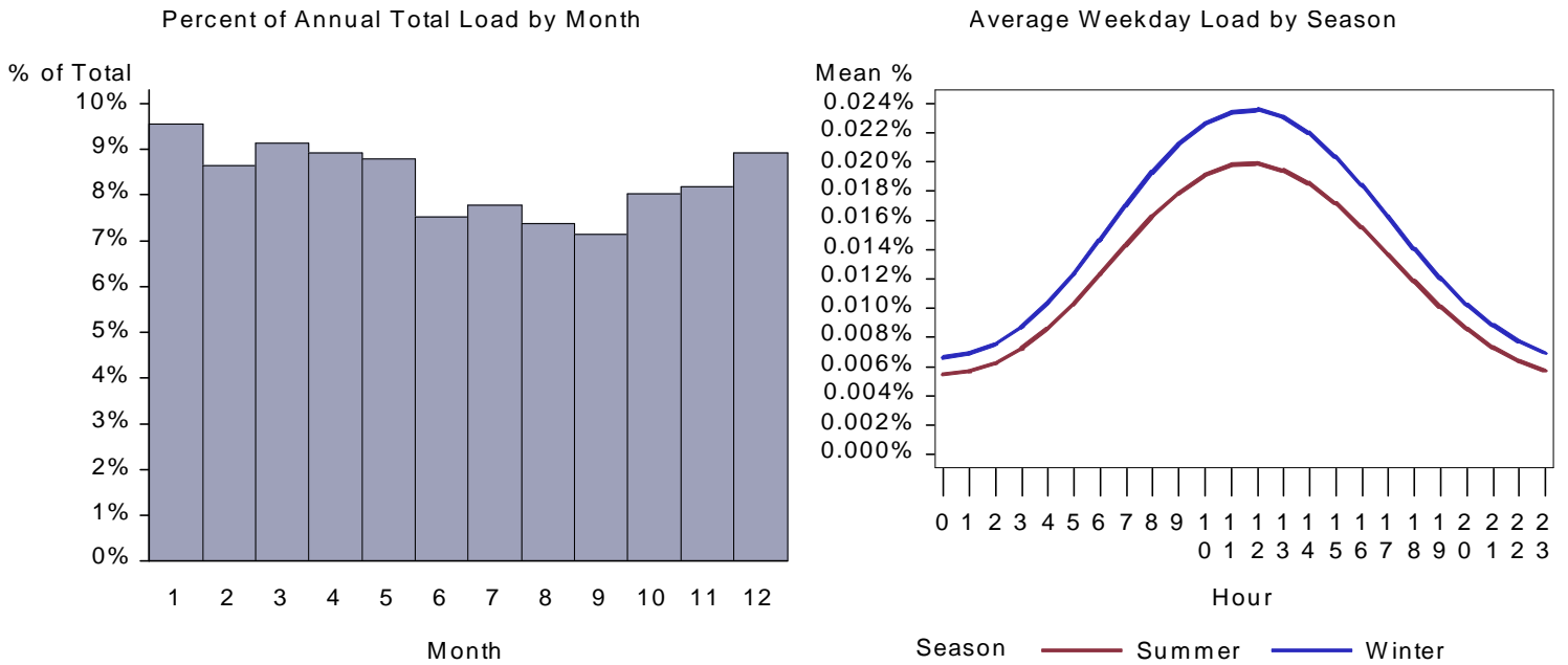
Figure 36. CA Small Office Cooking Load by Month and Average Weekday
