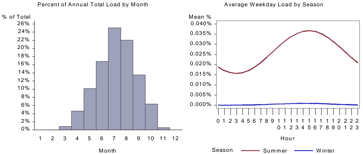
Figure 310. : WY Grocery Space Cool Load by Month and Average Weekday
