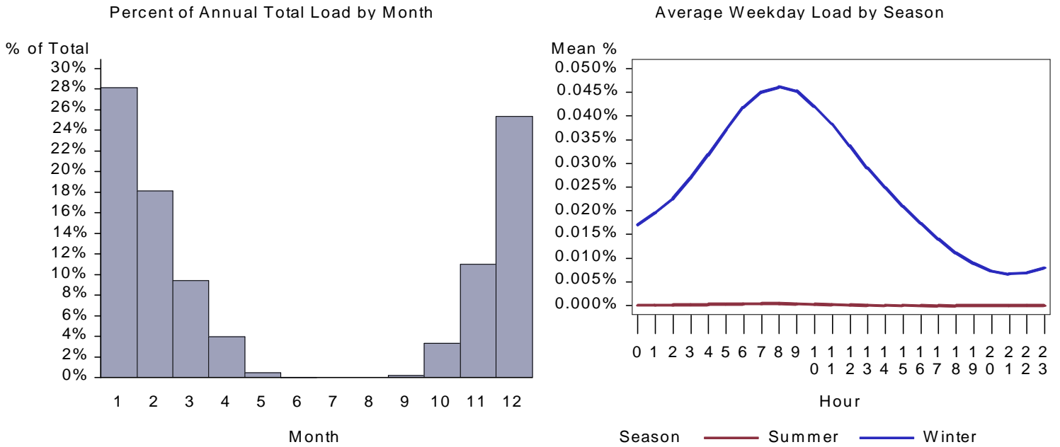
Figure 403. : ID Small Office Space Heat Load by Month and Average Weekday
