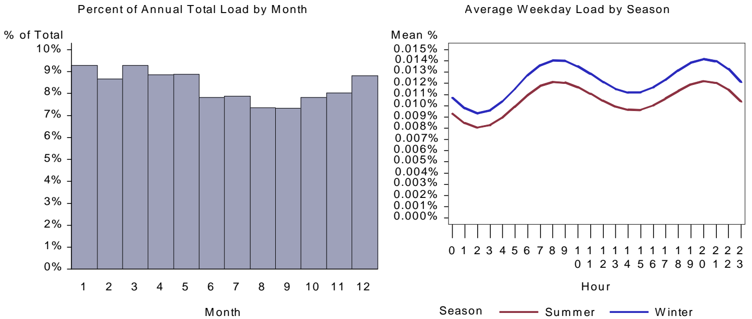
Figure 438. : CA Lodging Water Heat Load by Month and Average Weekday
