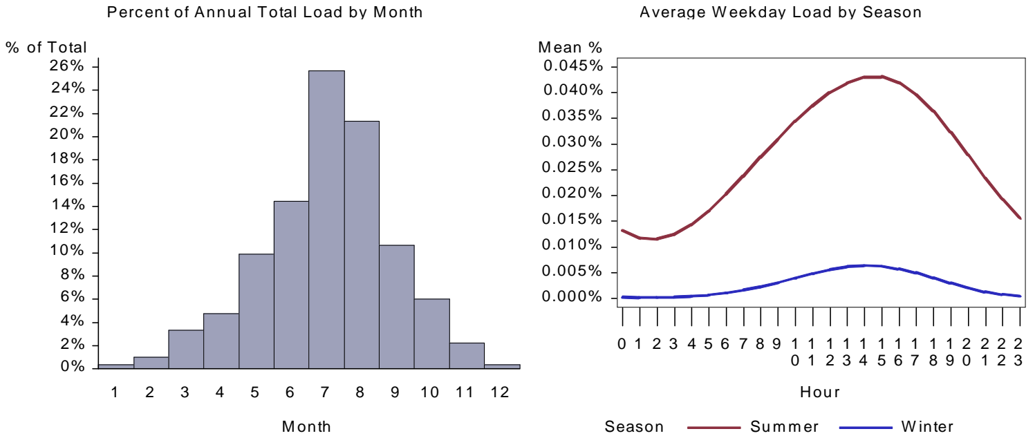
Figure 313. : UT Health Space Cool Load by Month and Average Weekday
