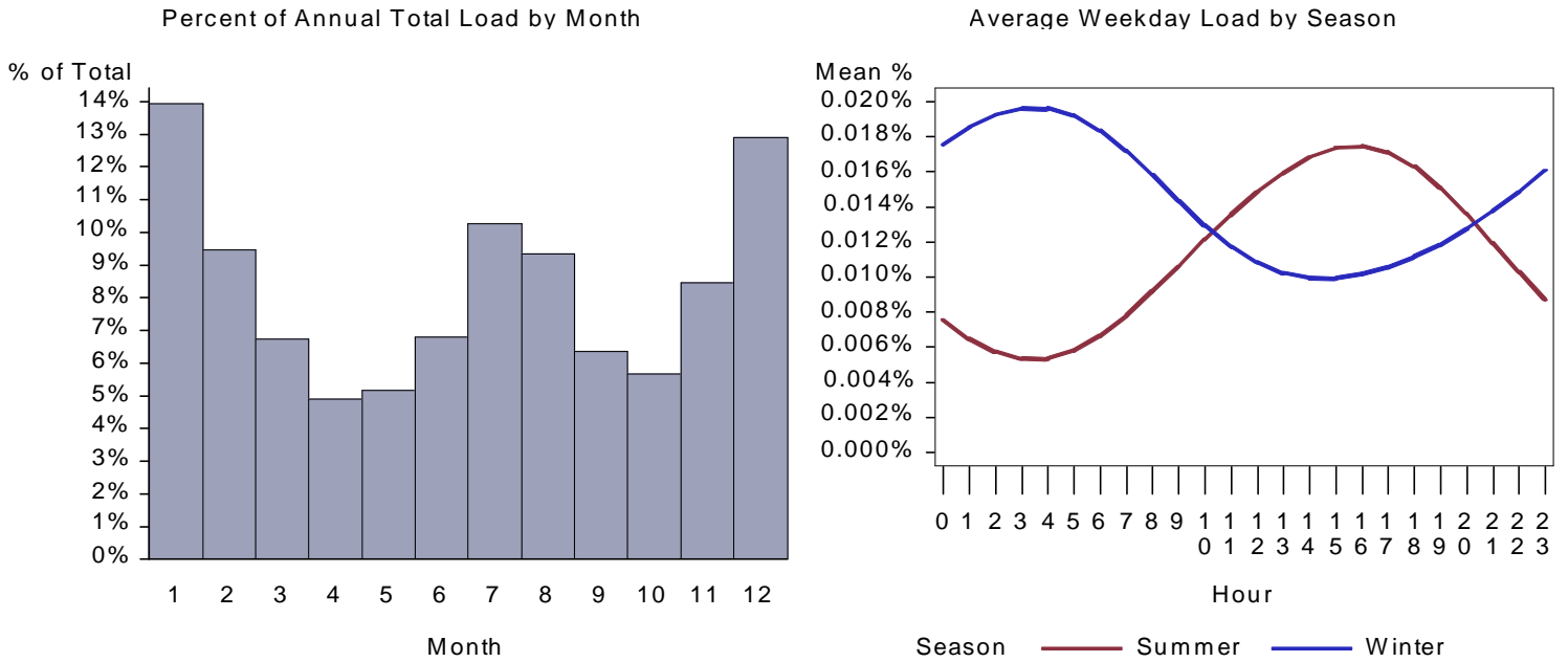
Figure 125. : CA Lodging Heat Pump Load by Month and Average Weekday
