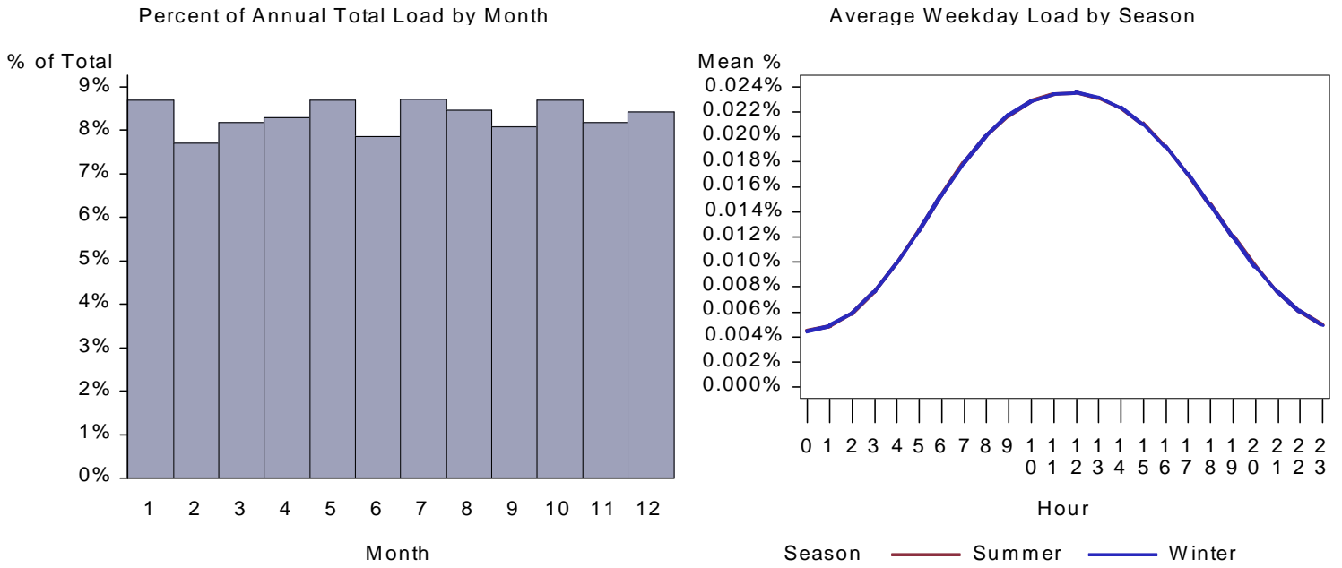
Figure 159. : UT Large Office Lighting Load by Month and Average Weekday
