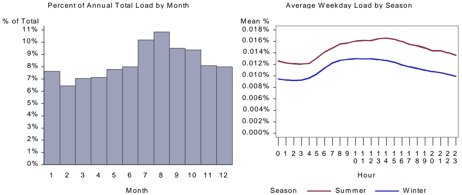
Figure 299. : WY Small Retail Refrigeration Load by Month and Average Weekday
