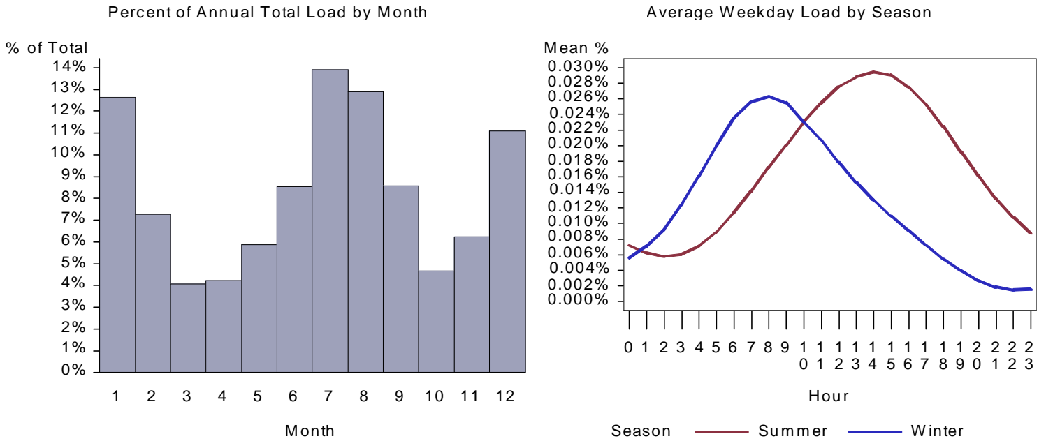
Figure 117. : CA Large Office Heat Pump Load by Month and Average Weekday
