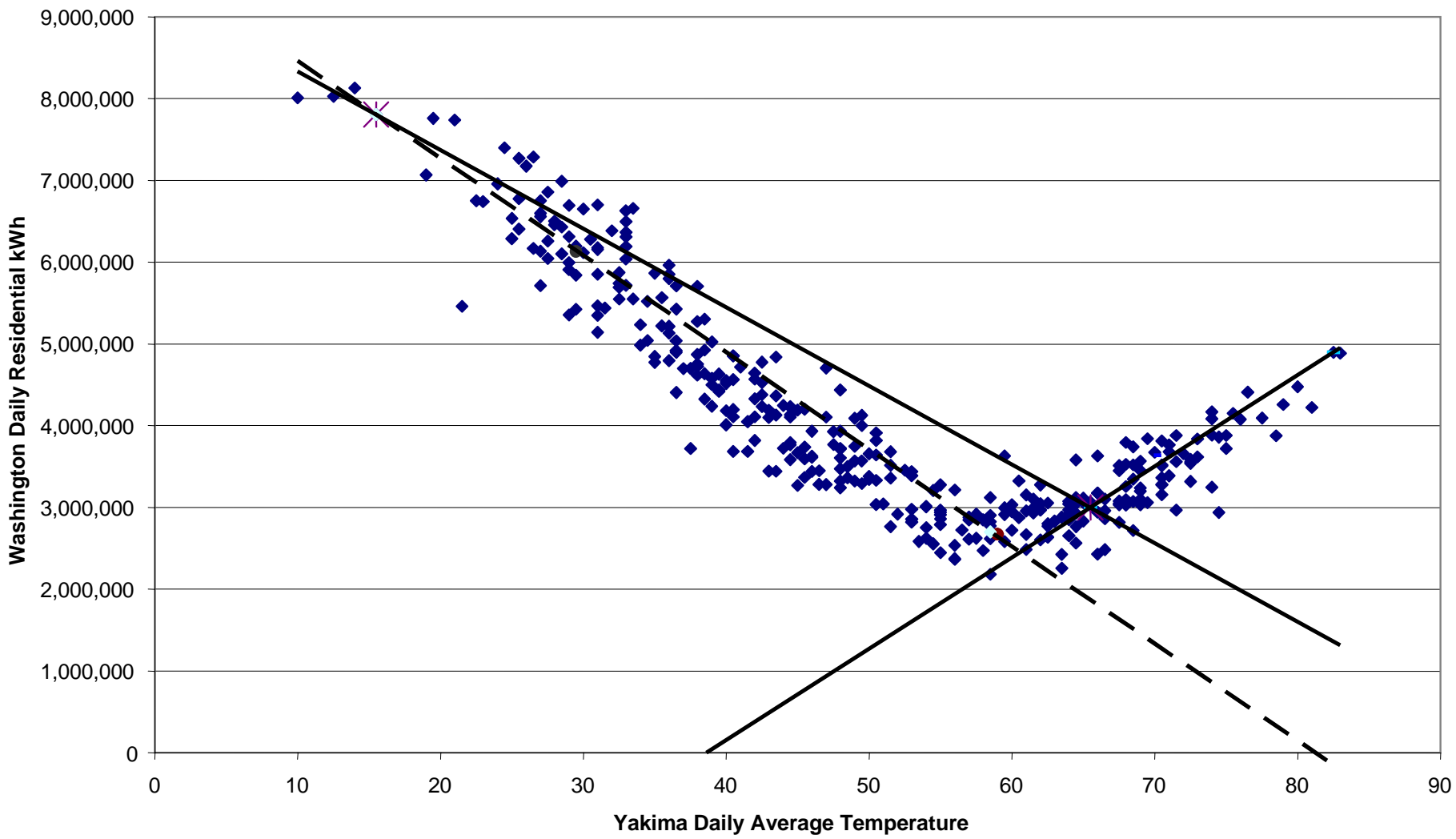
Washington State Residential Load vs. Daily Average Temperatures
