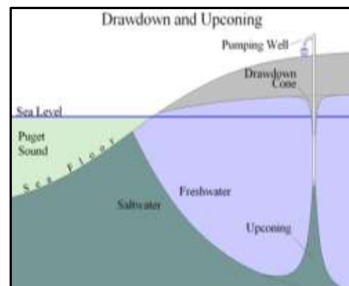
Figure 1 Seawater Upconing
