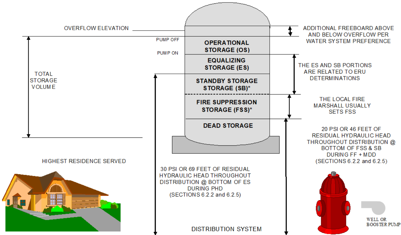
Figure 7-1: Reservoir Storage Components
