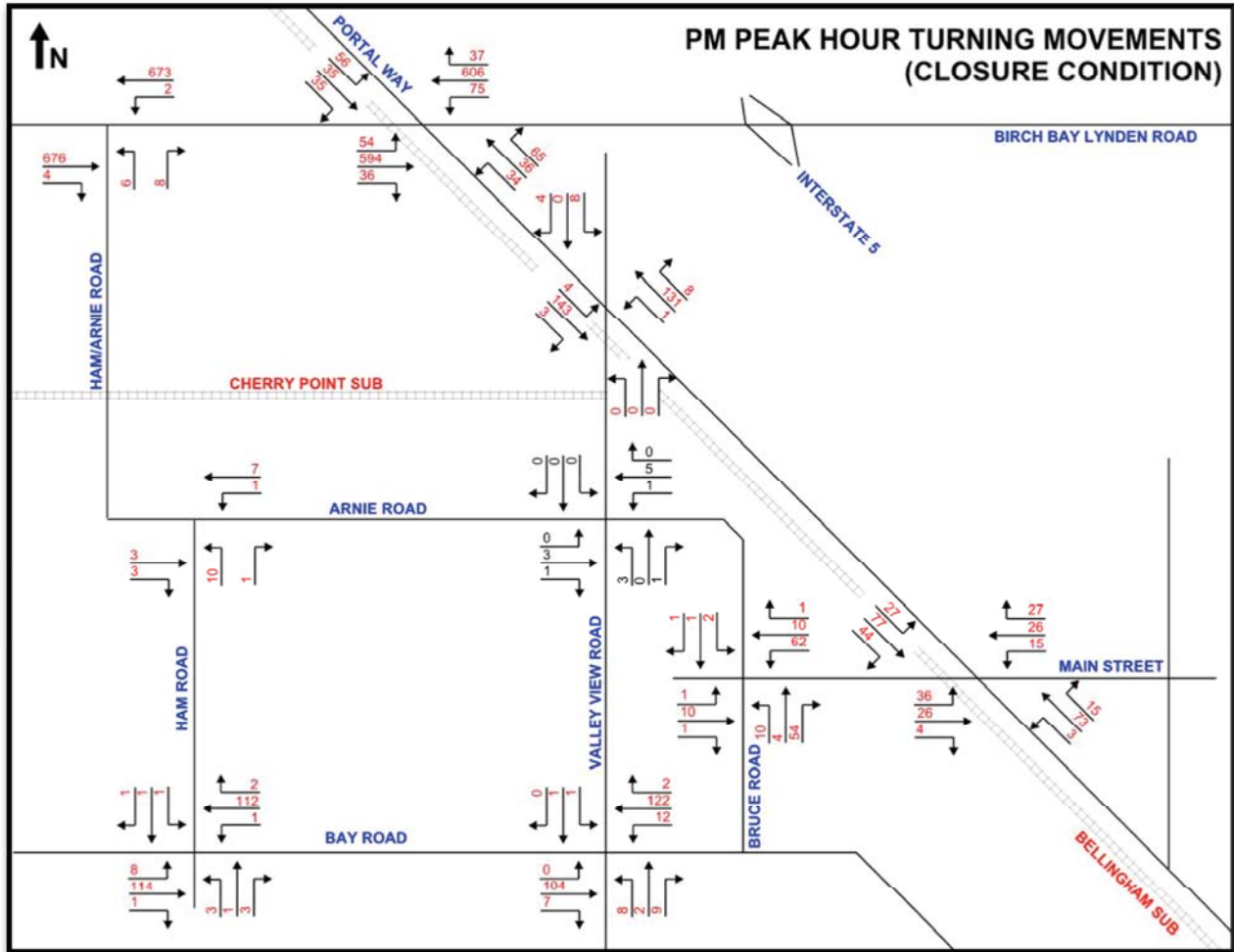
Figure 5: 2015 Peak Hour Turning Movements - Closed Condition
