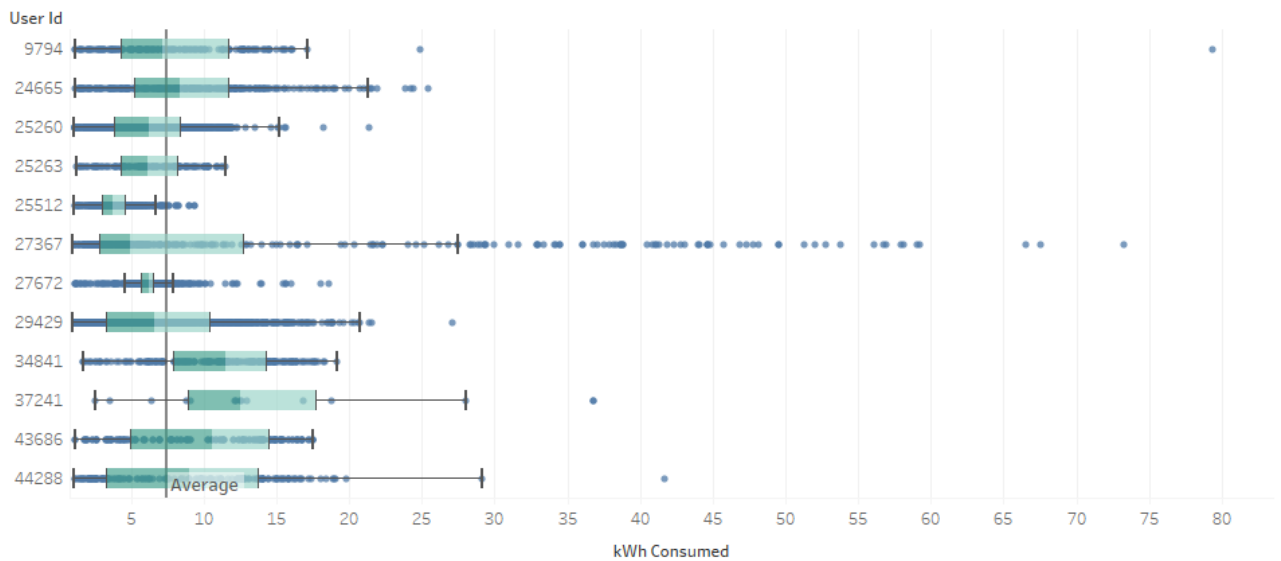
Figure 102. Workplace Charger Sample Group: Residential EVSE Session Energy Usage
