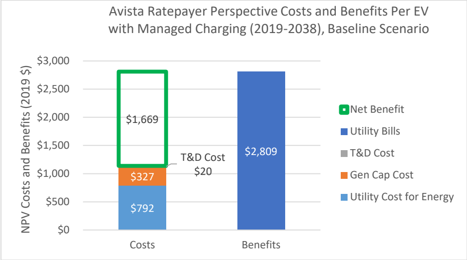
Figure 93. Ratepayer Perspective costs and benefits per EV, with managed charging 2019-2038
