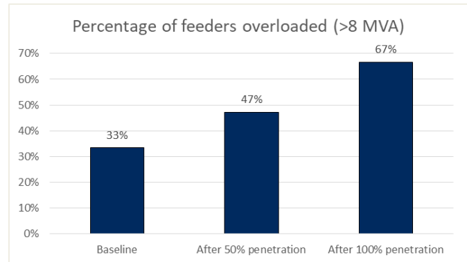
Figure 87: Distribution feeder overloads from EV loads, assuming all other loads held constant
