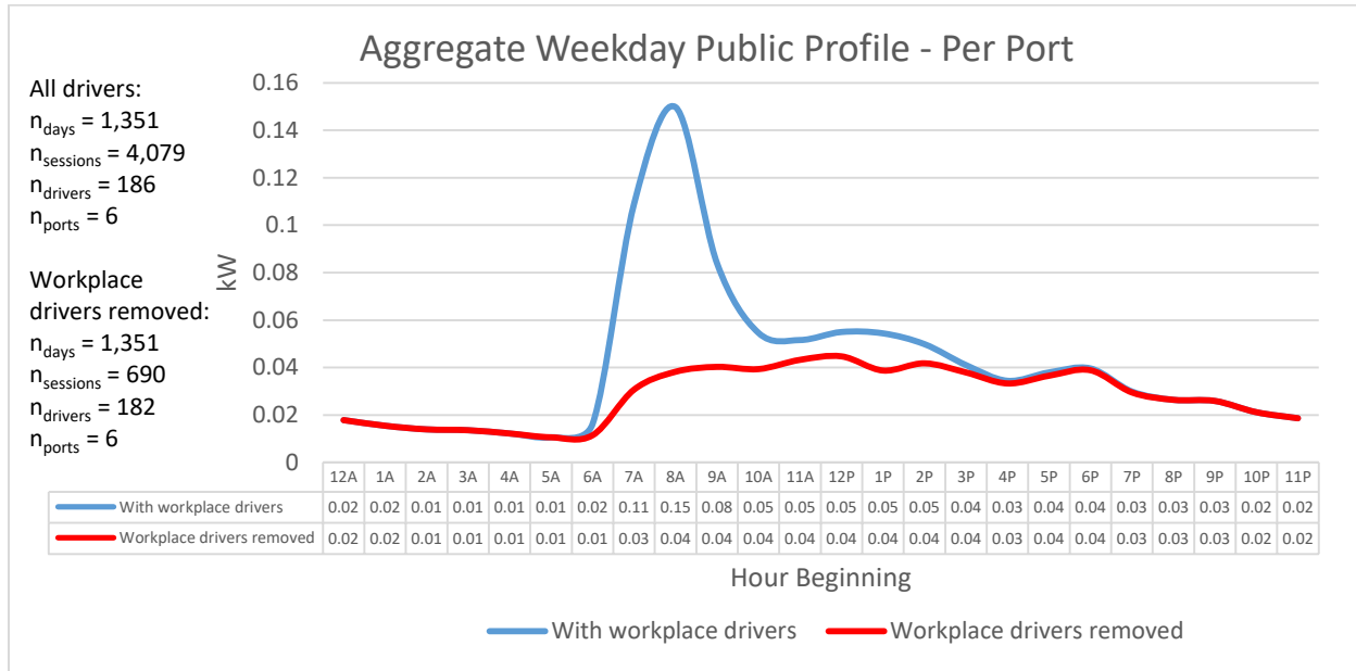
Figure 65. Workplace driver charging impact at public station
