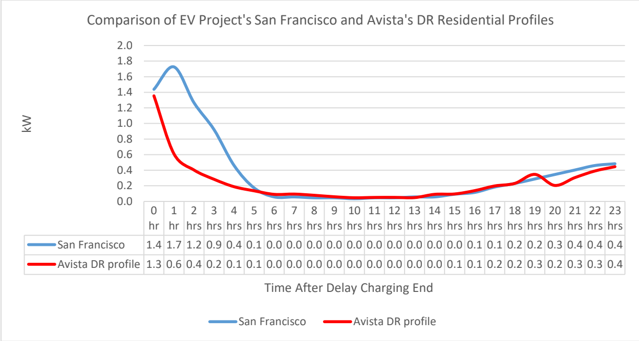
Figure 79. Comparison of Avista and the EV Project's Profiles with Delayed Charging
