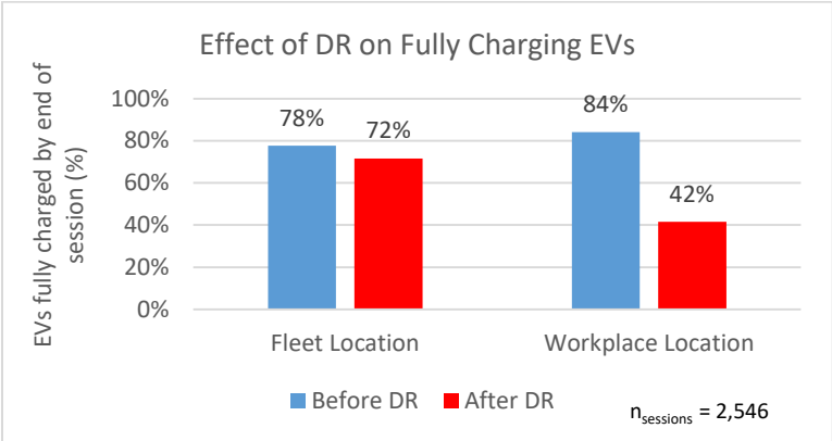
Figure 83. Comparison of fully charged batteries before and after DR at workplace and fleet locations
