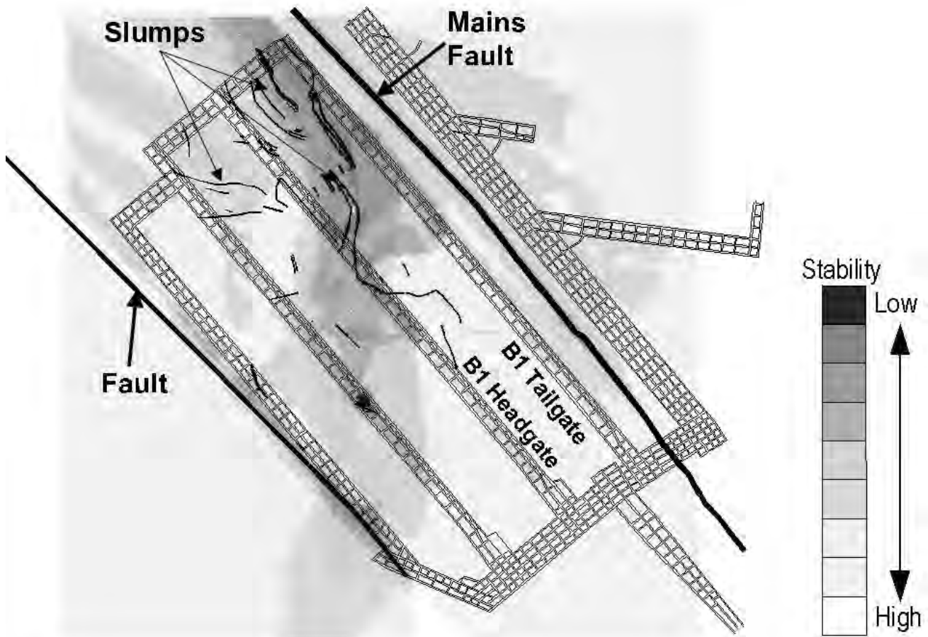
Figure 3. "Stability Map" generated from CMRR and underground mapping data.
