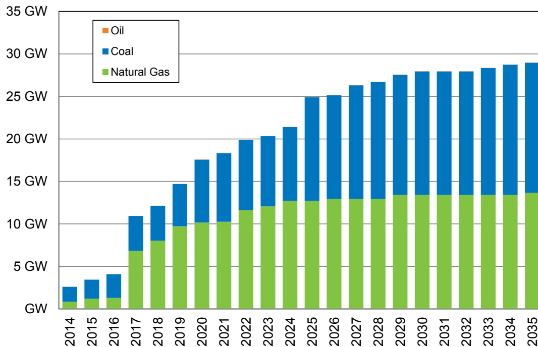
Figure 10.3: Resource Retirements (Nameplate Capacity)
