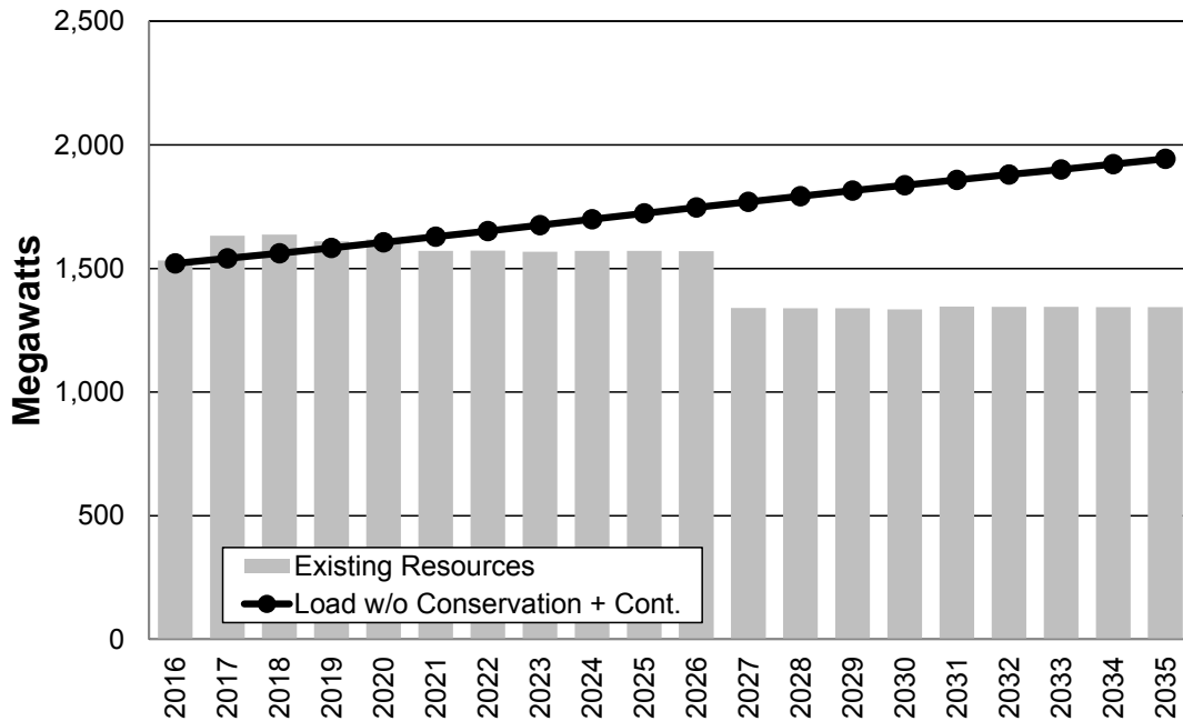
Figure 6.7: Summer 18-Hour Capacity Load and Resources
