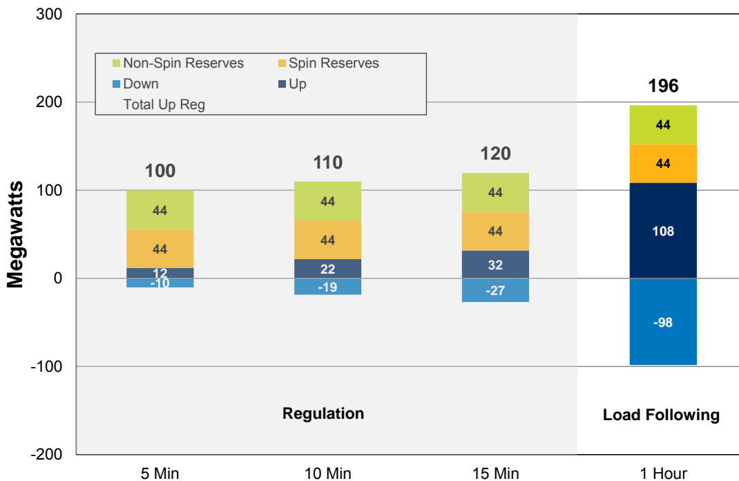
Figure 6.4: 95th Percentile Capacity Requirements
