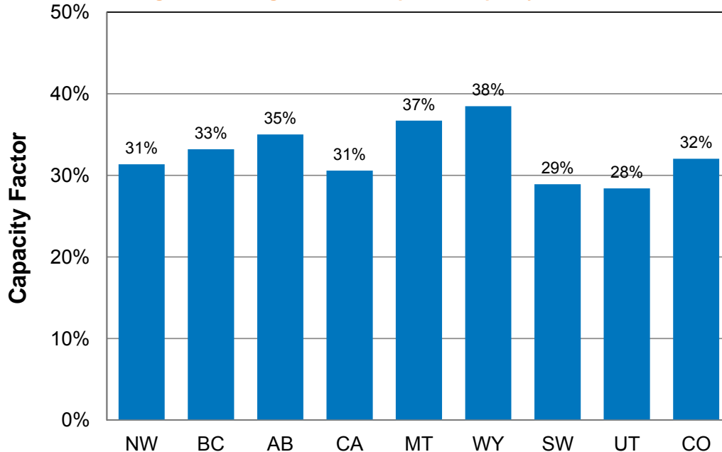
Figure 10.7: Regional Wind Expected Capacity Factors
