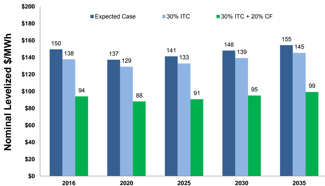
Figure 9.2: Solar Nominal Levelized Cost ($/MWh)
