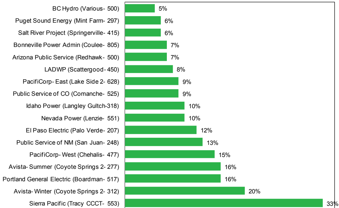
Figure 6.3: Single Largest Contingency Survey Results (2014 Peak Load)
