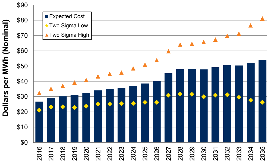
Figure 11.9: Power Supply Expense Range
