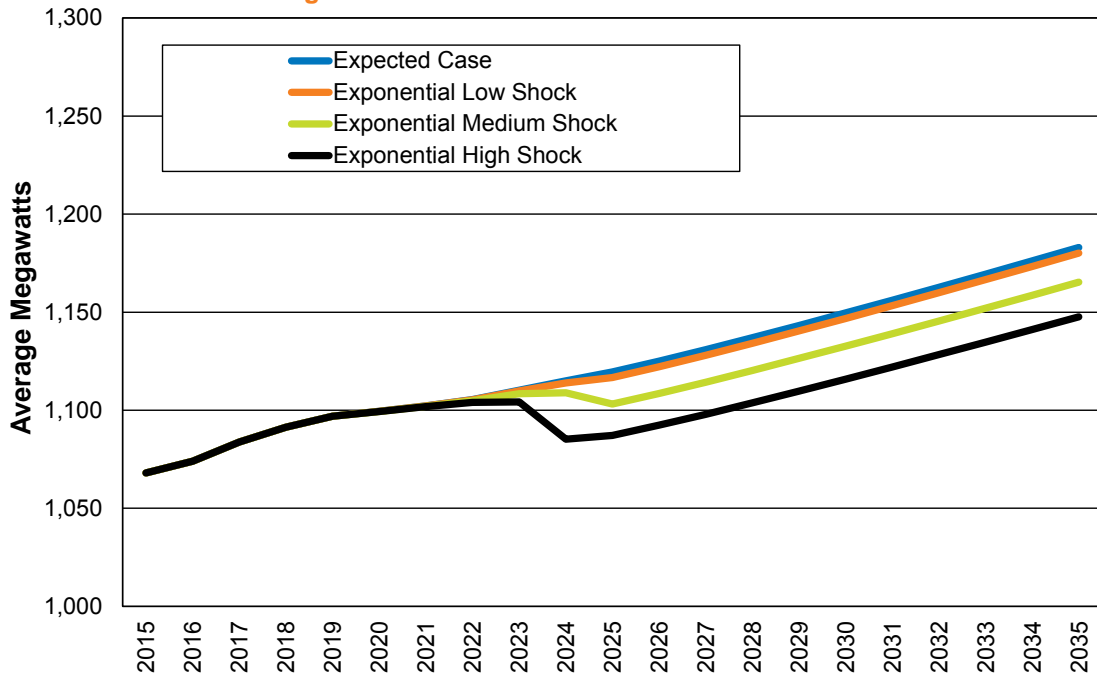
Figure 3.12: Load Scenarios with PV Shocks
