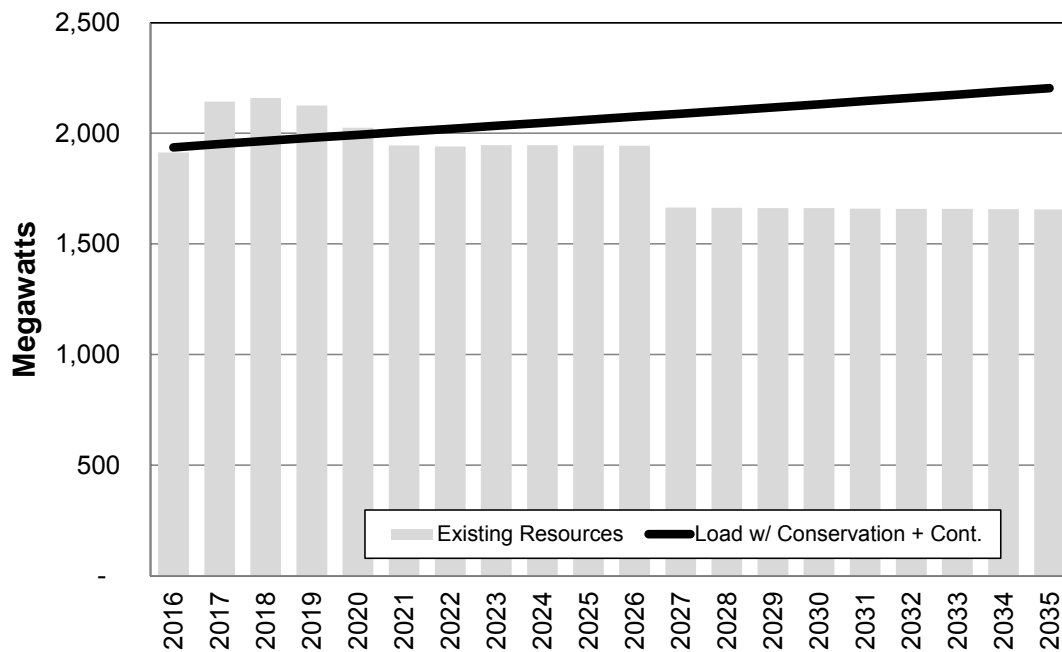
Figure 1.1: Load-Resource Balance—Winter Peak Load & Resource Availability
