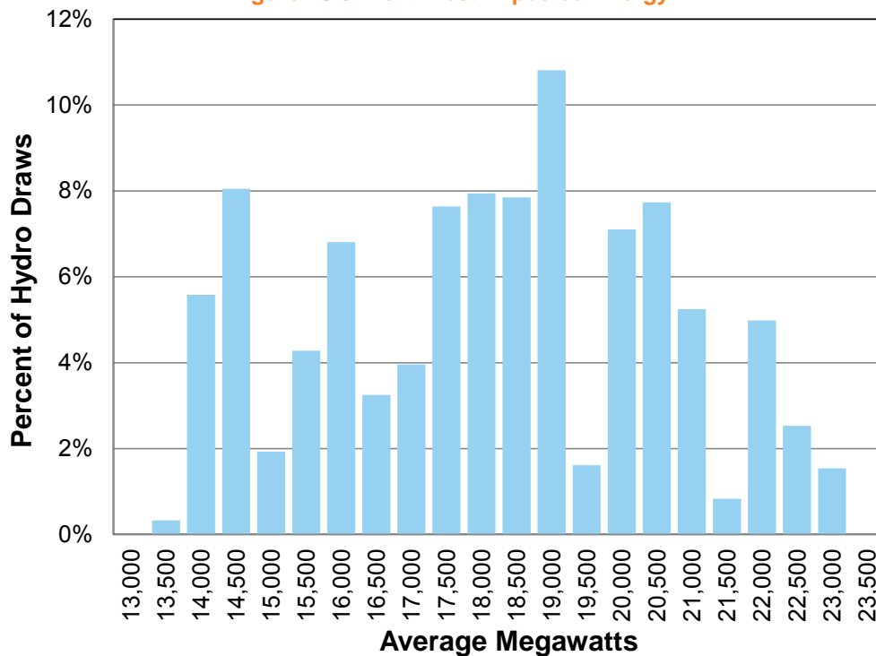
Figure 10.6: Northwest Expected Energy
