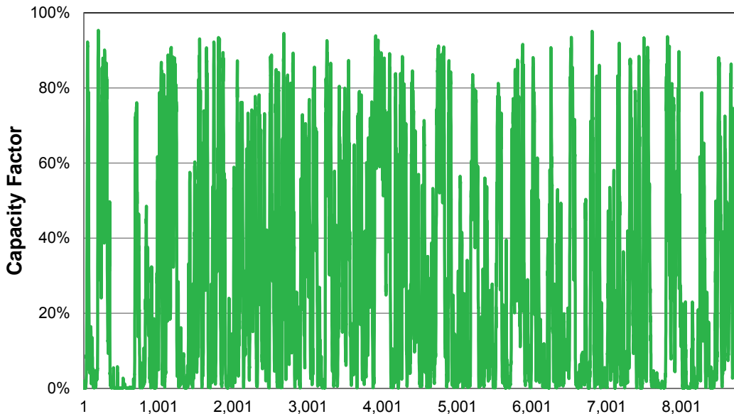
Figure 10.13: 2014 Actual Wind Output BPA Balancing Authority 3
