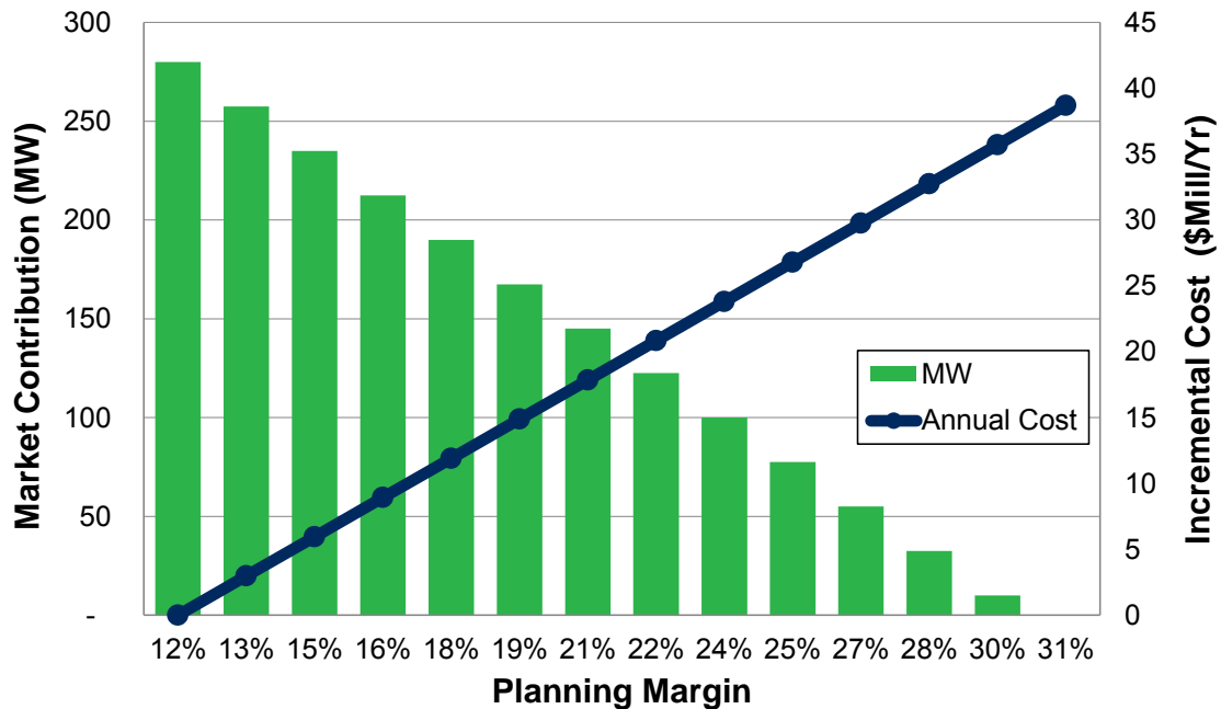
Figure 6.1: 2020 Market Reliance & Capacity Cost Tradeoffs
