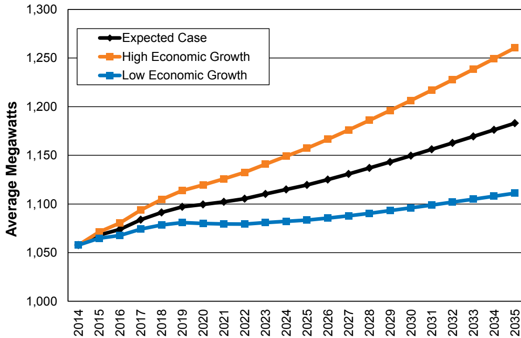
Figure 3.14: Average Megawatts, High/Low Economic Growth Scenarios
