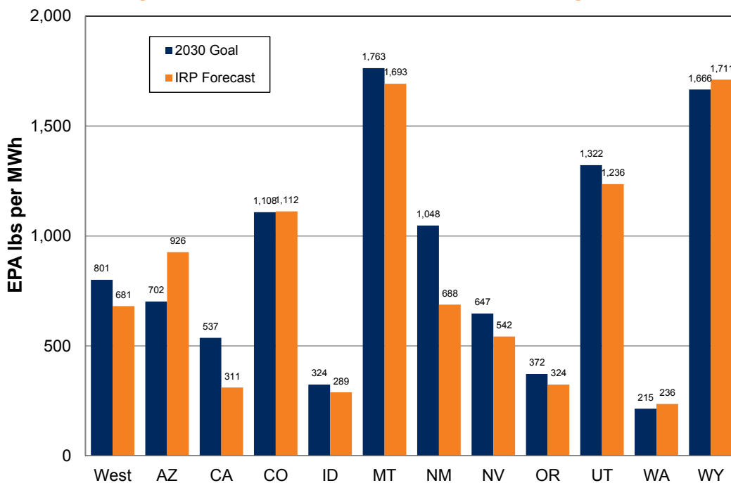
Figure 10.17: EPA's CPP 2030 State Goal vs. Modeling Result
