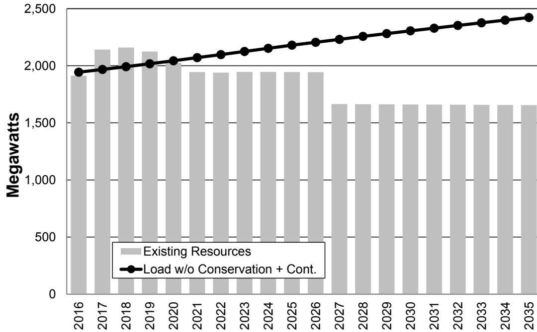
Figure 6.6: Winter 1 Hour Capacity Load and Resources
