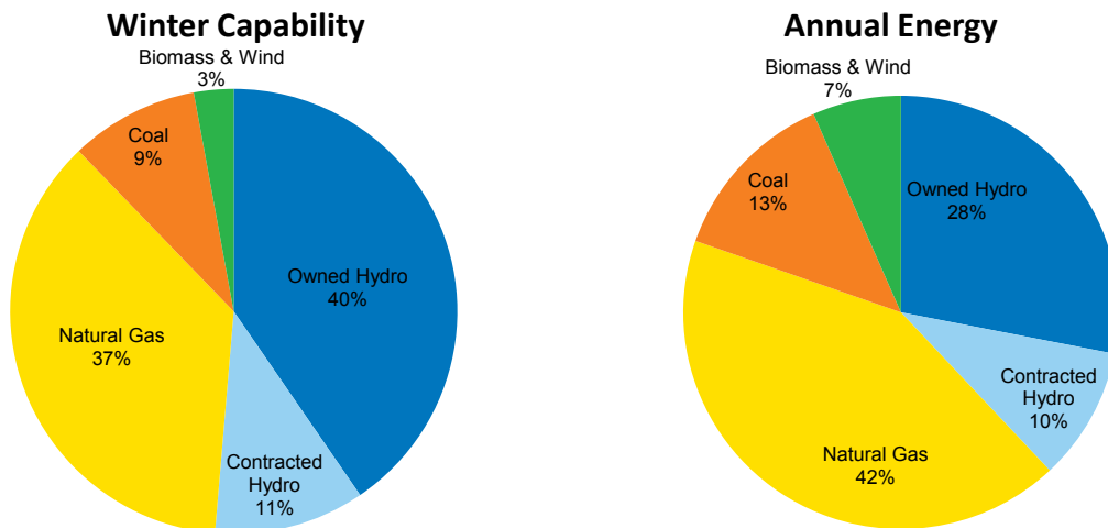
Figure 4.1: 2016 Avista Capacity & Energy Fuel Mix
