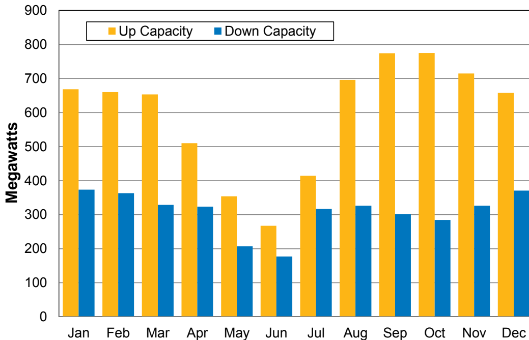
Figure 9.5: Avista’s Monthly Up/Down Regulation Surplus
