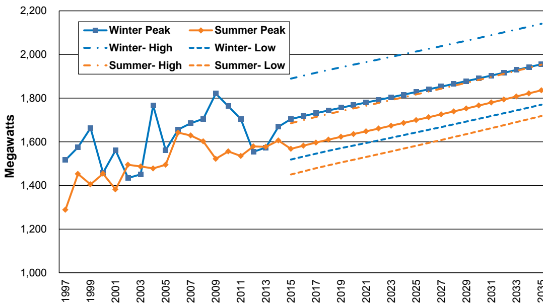
Figure 3.18: Peak Load Forecast with 1 in 20 High/Low Bounds, 2015-2035
