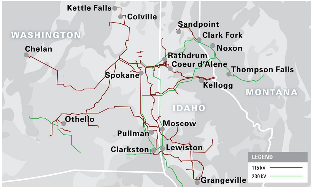
Figure 8.2: Avista Transmission Map
