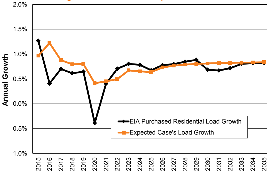
Figure 3.16: Load Growth Comparison to EIA
