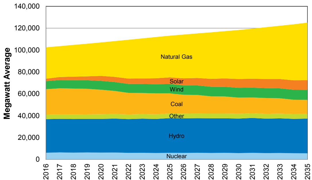
Figure 10.18: Base Case Western Interconnect Resource Mix
