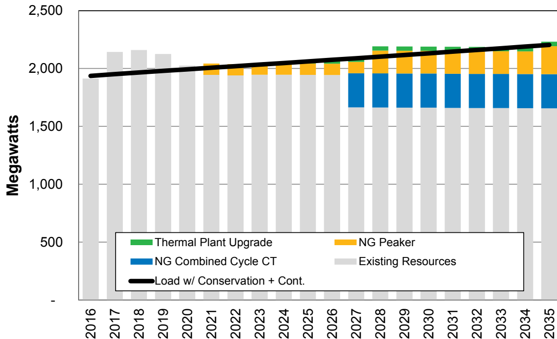
Figure 11.5: New Resources Meets Winter Peak Loads
