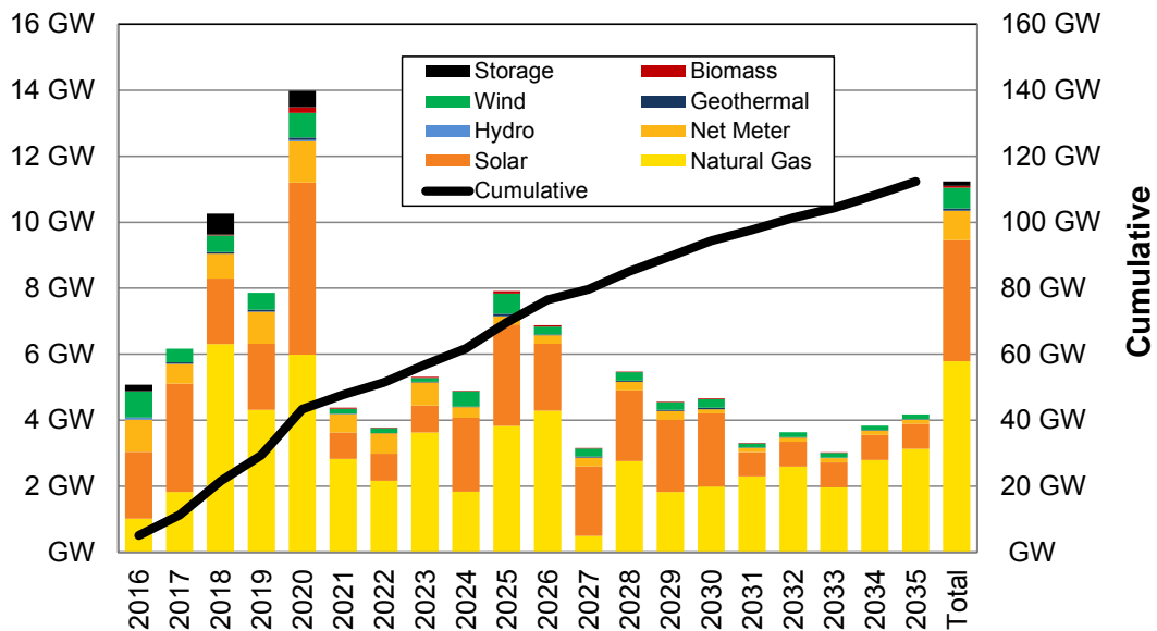
Figure 10.4: Cumulative Generation Resource Additions (Nameplate Capacity)
