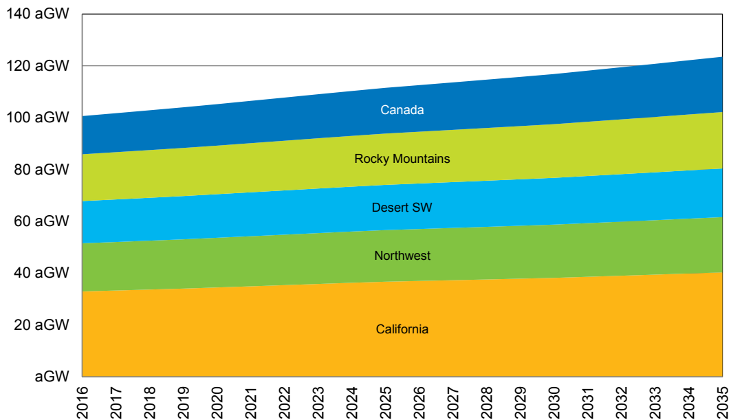
Figure 10.2: 20-Year Annual Average Western Interconnect Energy
