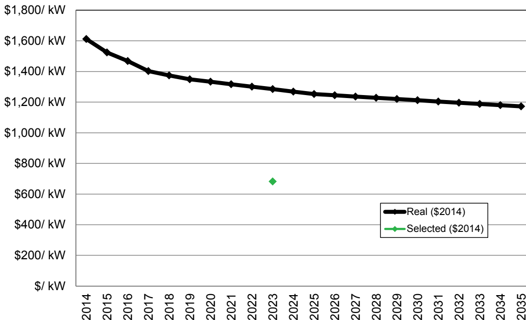
Figure 12.12: Utility Scale Solar Tipping Point Analysis (2014 $)
