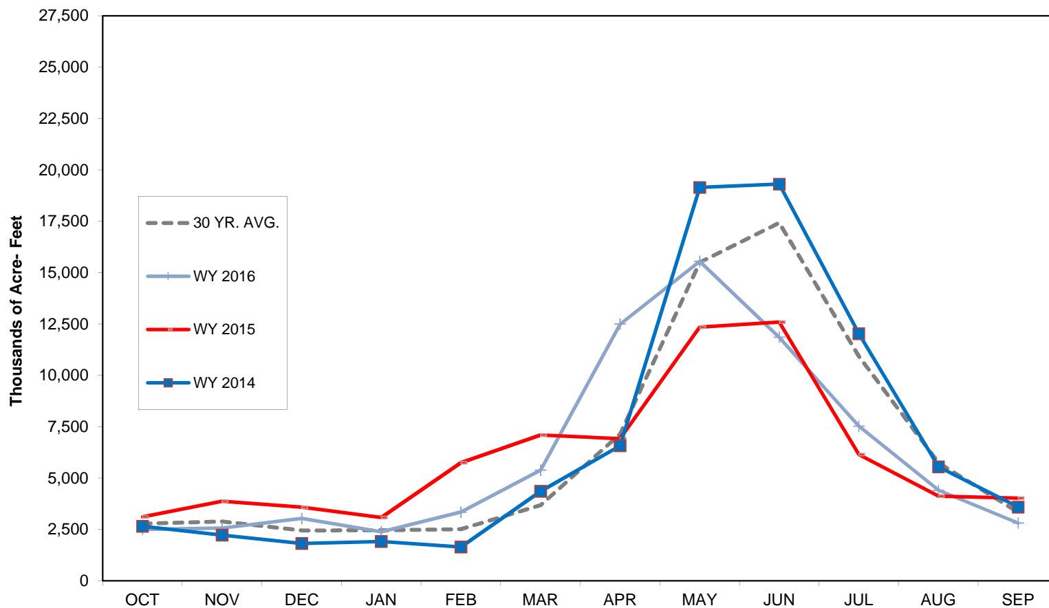
Grand Coulee Monthly Runoff Volumes Water Years 2014-2016 (Oct-Sep) Actuals and 30 Yr Average 1981-2010
