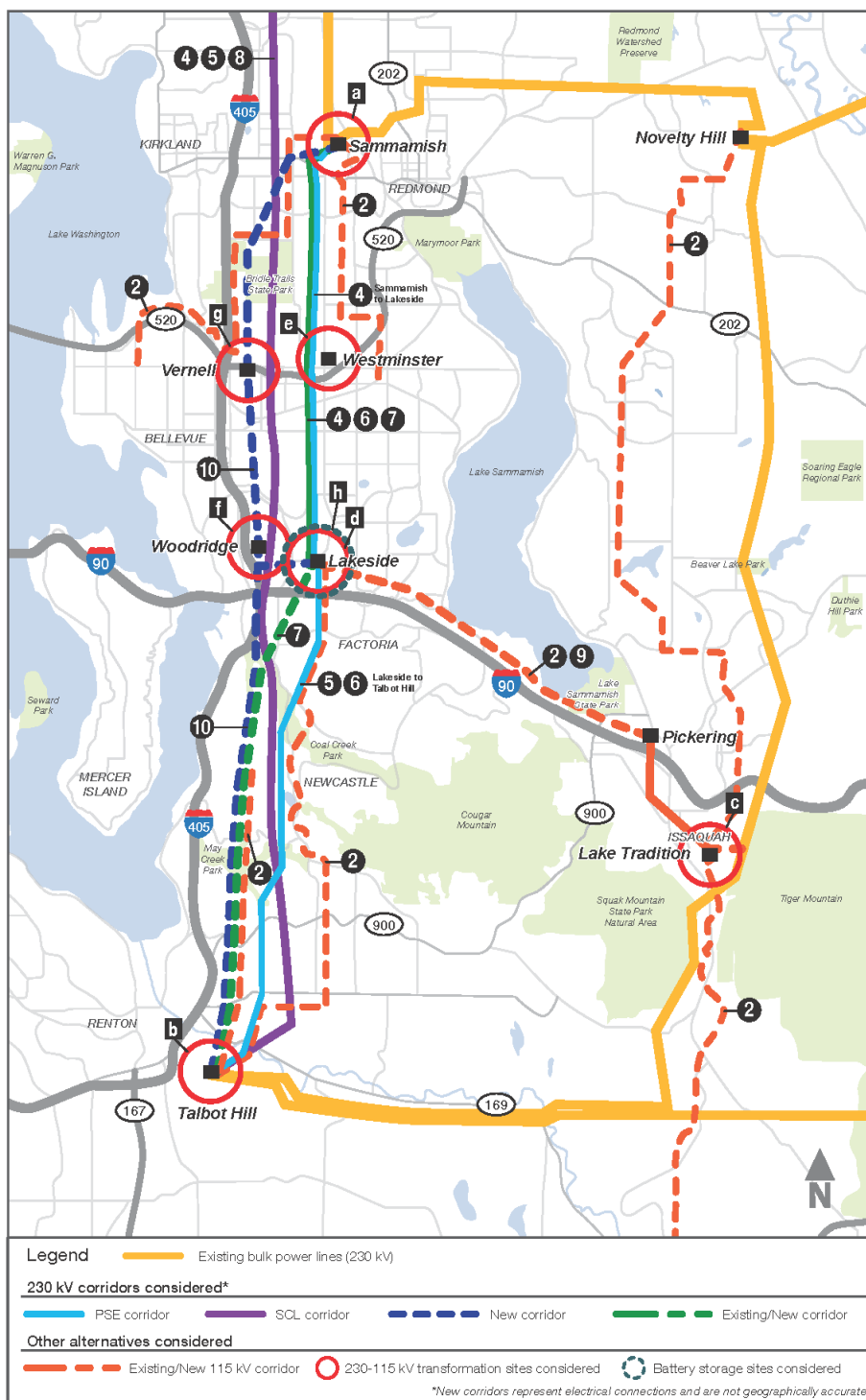
Figure 3: Graphic Showing all 10 Alternatives with Options
