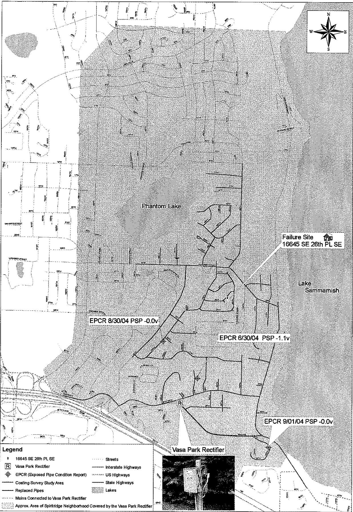
Approximation of Area Covered by the Vasa Park Rectifier; Coating Survey Study Area; Replaced Pipes; And Other Information
