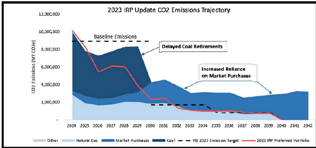
Figure 2 – 2023 IRP Update CO2 Emissions Trajectory
