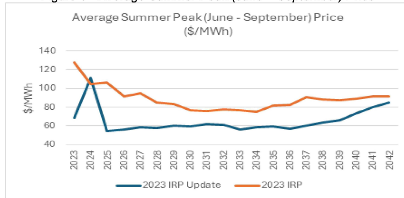
Figure 3 - Average Summer Peak (June – September) Price
