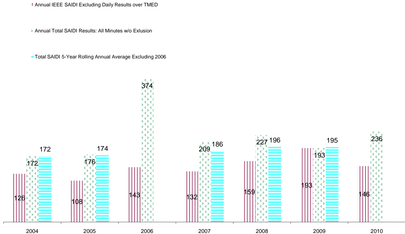
Chart 1: 20XX-20XX AVA SAIDI Performance in Different Measurements by Year
