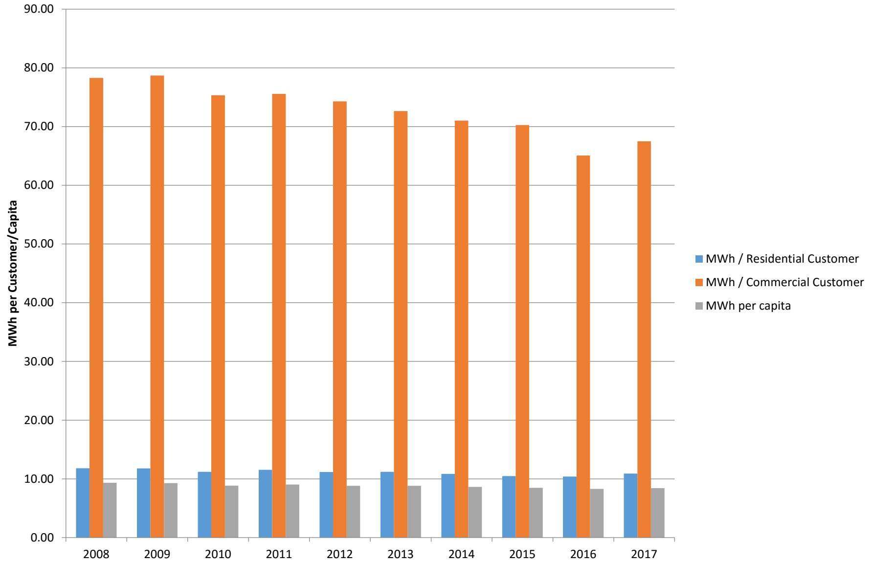
Figure 2. Energy Intensity Metrics 2008 - 2017
