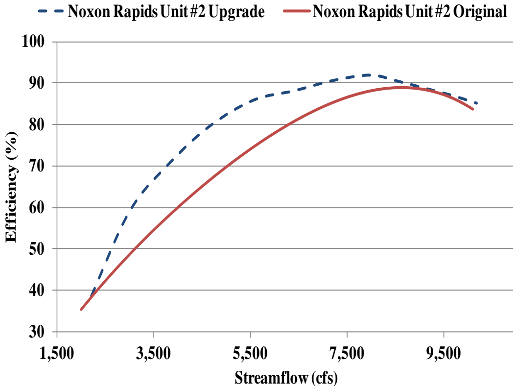
Illustration 5: Noxon Rapids Unit #2 Turbine Curves
